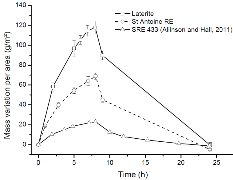
Figure 7-5: Moisture buffering test
