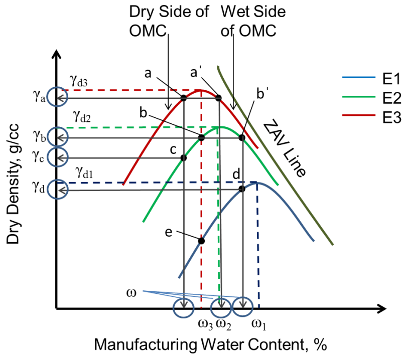
Figure 2-5 Concept of Manufacturing water content and achieved dry density
