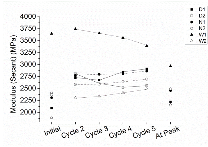
Figure 7-11: Variation of Modulus at each cycle
