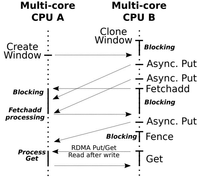
Figure 5.3 – RDMA Put and Get Operations with Remote Atomics on Window Memory Segments
