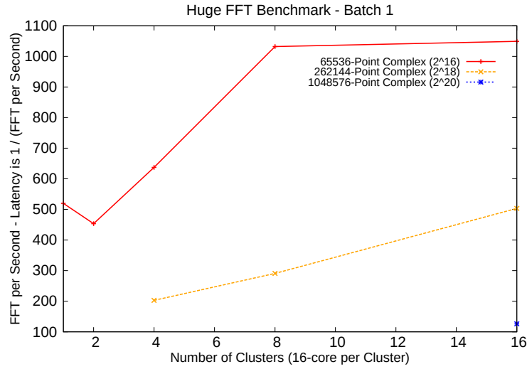
Figure 10.9 – Execution Time of Distributed Multi-Cluster FFT. The Higher, The Better.
