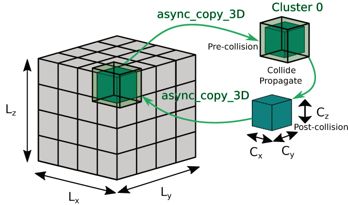
Figure 10.2 – 3D LBM/stencil decomposition where a Main-node subdomain (green) is copied with its surrounding halo layers (if exists) and one extra subdomain (blue) is needed to store the post-collision state.
