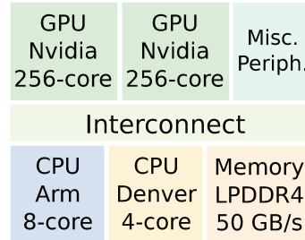
Figure 2.3 – Nvidia Drive PX 2: A Complex and Highly Parallel Heterogeneous Embedded System for Autonomous Driving
