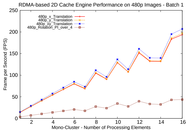
Figure 9.15 – Mono-Cluster RDMA-based 2D Explicit Cache of Tiles Performance. VGA Images.
