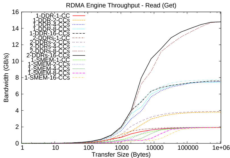
Figure 5.7 – RDMA Get (Read) Throughput GB/s (Asynchronous)
