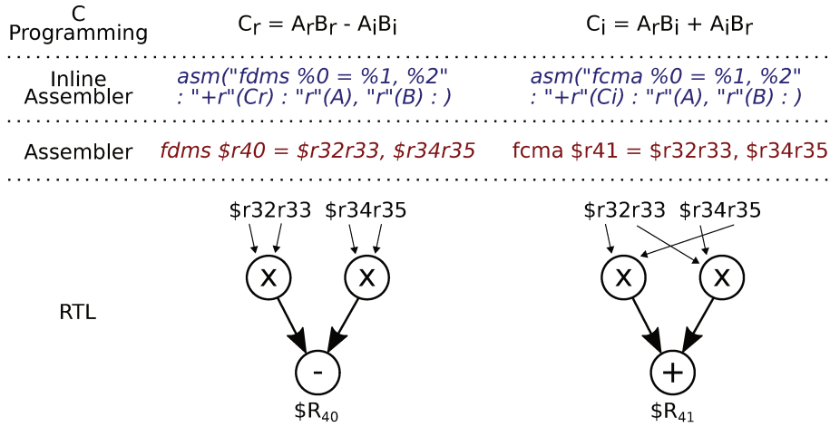
Figure 10.7 – Example of a Vectorization (pair of registers) in the k1 VLIW PE.
