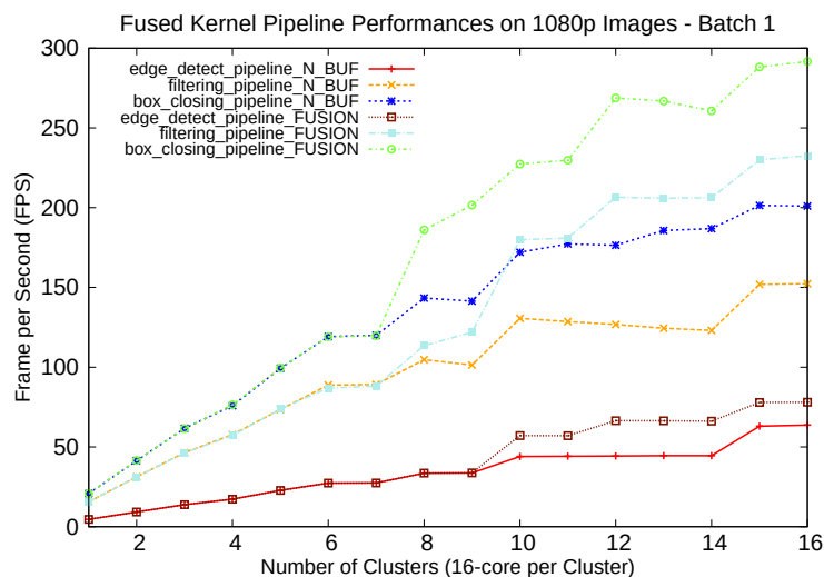
Figure 9.12 – Automatic RDMA -based Kernel Fusion Performance. Full HD Images. Tiling with N-Buffering ( N_BUF = N-Buffering = Prefetch) vs Kernel Fusing ( FUSION ).
