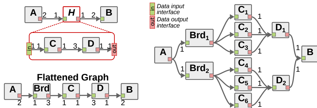
Figure 3.9 – Flattening and Single-Rate Transformation of IBSDF (left) to Single-Rate DAG (SRDAG) (right)
