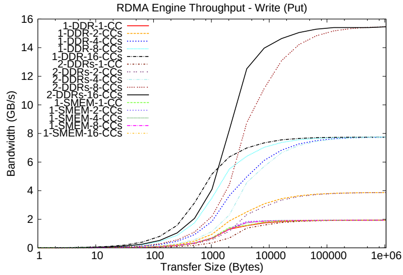
Figure 5.8 – RDMA Put (Write) Throughput GB/s (Asynchronous)
