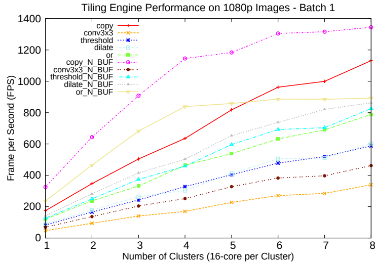
Figure 9.10 – Automatic Tiling Engine Performance. Full HD Images. Simple Tiling vs Tiling with N-Buffering ( N\_BUF = N\text{-Buffering} = \text{Prefetch} ).
