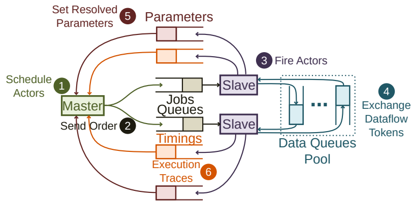
Figure 3.13 – Internal Structure of the SPIDER Runtime
