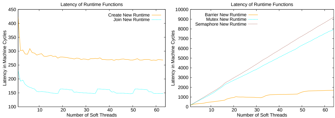
Figure 6.5 – Performance Comparisons of Thread Creation, Join and Basic Synchronization Primitives on 64 Threads
