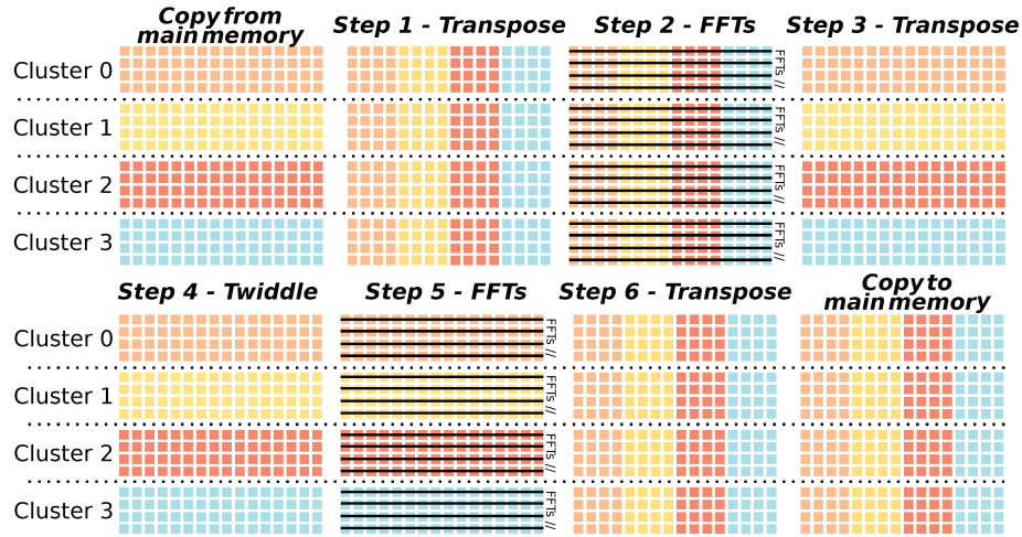
Figure 10.6 – Architecture of the Distributed FFT for Low-Latency Execution over Several Compute Clusters (CCs).
