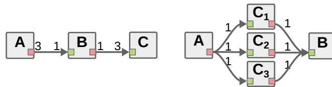
Figure 3.6 – Single-Rate Transformation SDF (left) to Single-Rate DAG (SRDAG) (right)
