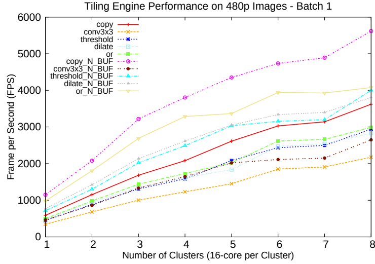
Figure 9.9 – Automatic Tiling Engine Performance. VGA Images. Simple Tiling vs Tiling with N-Buffering ( N\_BUF = N\text{-Buffering} = \text{Prefetch} ).
