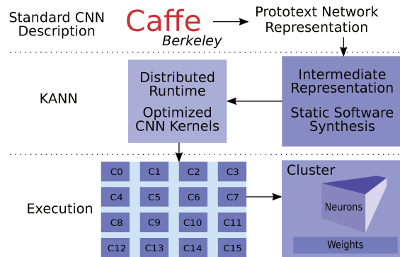
Figure 10.10 – Architecture of the KANN Framework.
