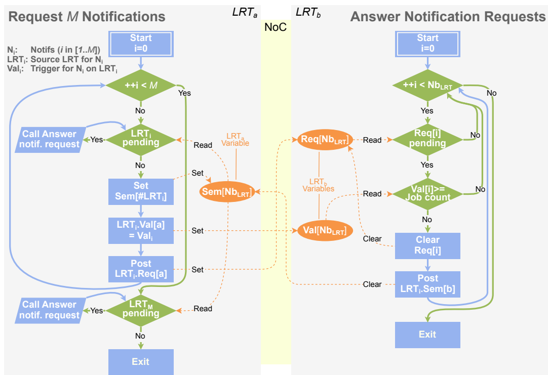
Figure 8.2 – Algorithms for Distributed Synchronizations for the Actor Firings. The number of requests is the number of input First-In-First-Out queues (FIFOs) of the next actor.
