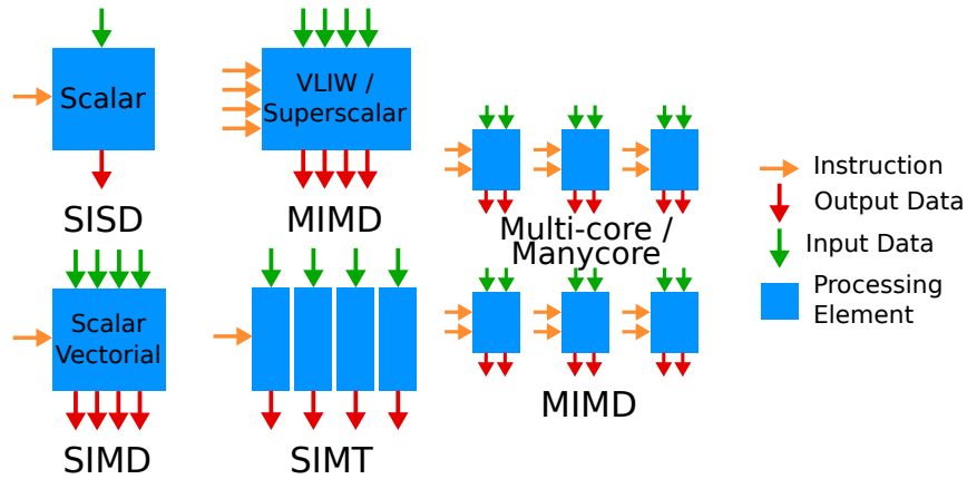
Figure 2.2 – Examples of Multiple Levels of Parallelism
