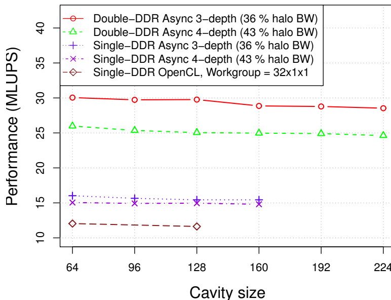
Figure 10.4 – OPAL_async vs. OPAL OpenCL on MPPA ® for duration = 1000 steps.
