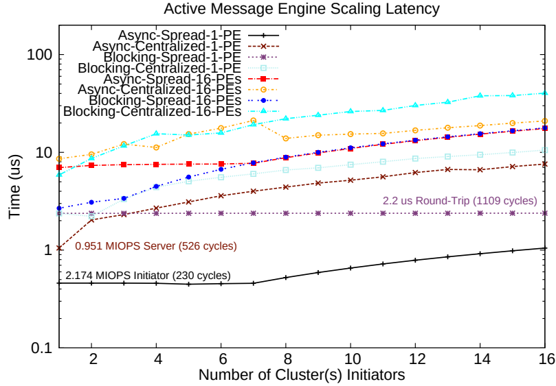
Figure 5.11 – Active Message Latency
