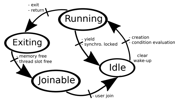
Figure 6.1 — Specific States & Transitions of Threads in the NMTR
