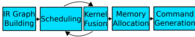
Figure 9.4 – OpenVX Verify Graph Workflow - vxVerifyGraph [G+ 17]
