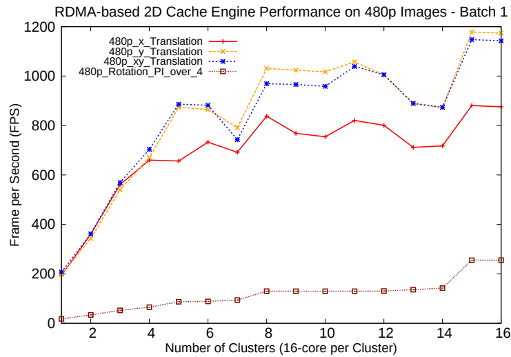
Figure 9.13 – RDMA-based 2D Explicit Cache of Tiles Performance. VGA Images.
