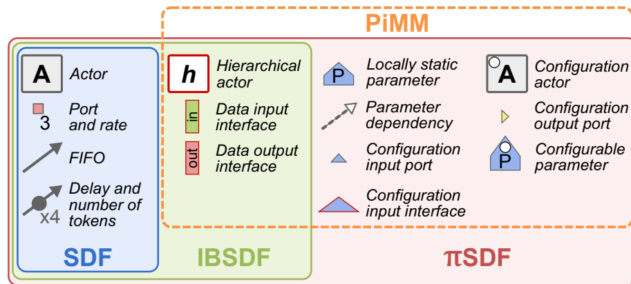
Figure 3.10 – PiMM Semantics (Source [Des14])
