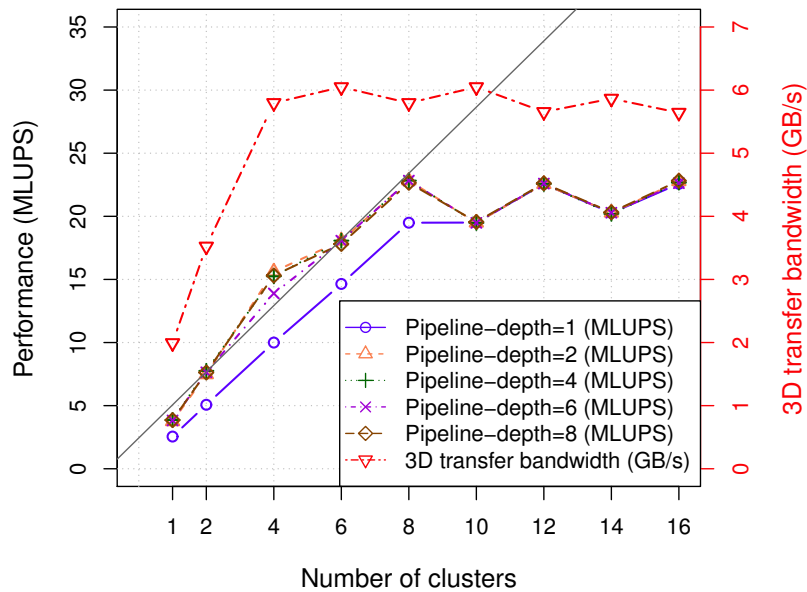
Figure 10.5 – Performance extrapolation of OPAL_async with 8 \times 8 \times 8 subdomains with the first eight CCs correlation represented by a gray line for 1000 timesteps and cavity size 128.
