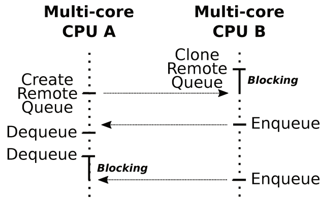
Figure 5.4 – Enqueue and Dequeue Operation using Remote Queue Memory Segments
