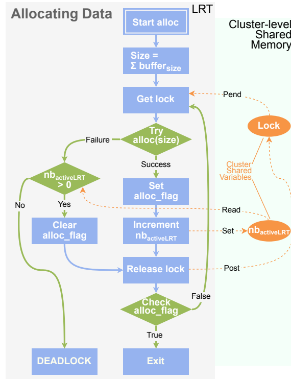
Figure 8.3 – Algorithm for the Local Memory Allocation in the CC .
