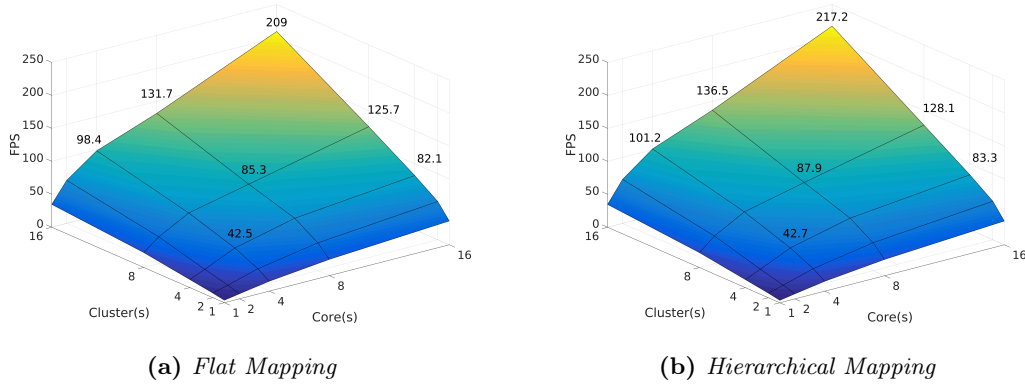
Figure 7.6 – MPPA ® Matrix Result in fps
