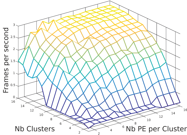
Figure 8.5 – Application Performance on a 4K Video
