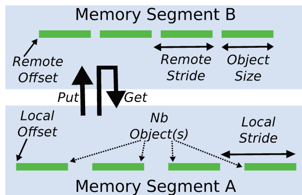
Figure 5.5 – RDMA Put/Get Data Transfer Restructuring Pattern
