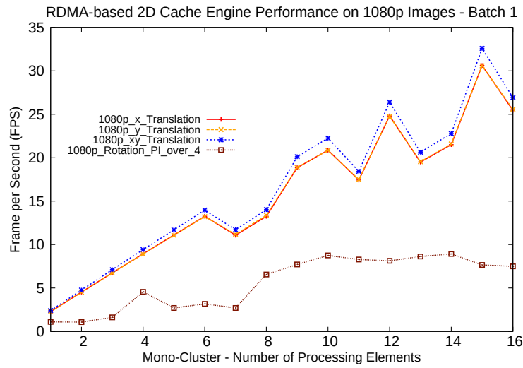
Figure 9.16 – Mono-Cluster RDMA -based 2D Explicit Cache of Tiles Performance. Full HD Images.
