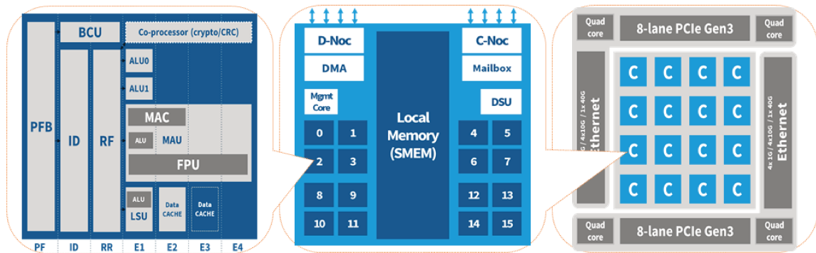
Figure 2.4 – MPPA ® Processor
