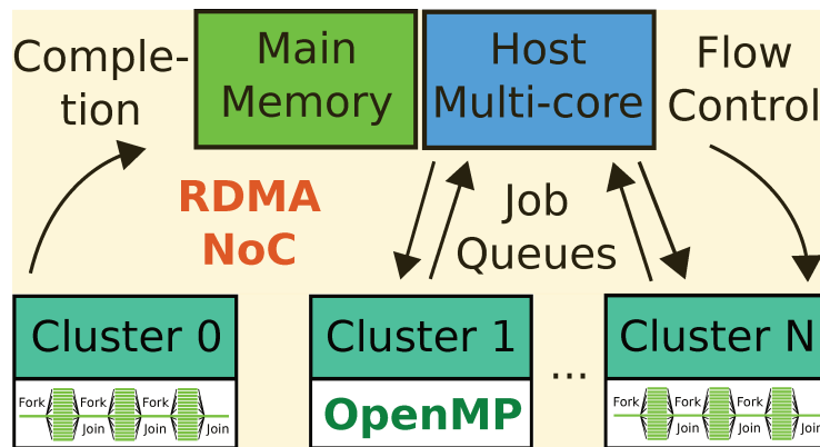
Figure 9.2 – OpenVX Offloading Engine Architecture
