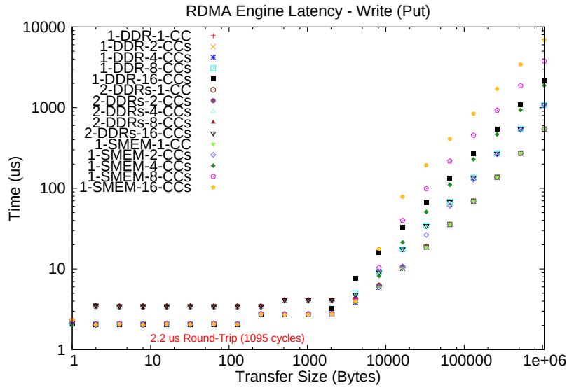
Figure 5.10 – RDMA Put (Write) Latency \mu s (Blocking)
