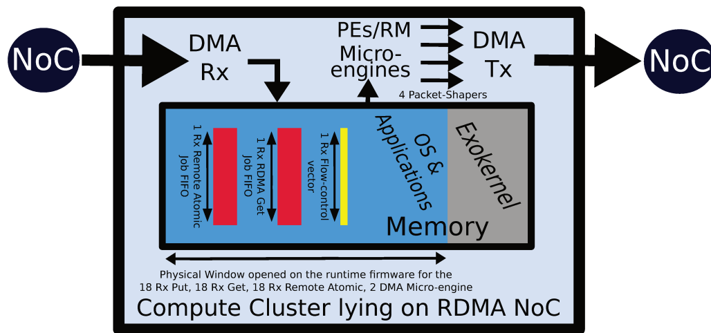
Figure 5.6 – Architecture of AOS in a Compute Cluster
