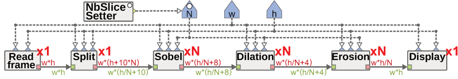
Figure 8.4 – Parametrized Image Filtering Application.
