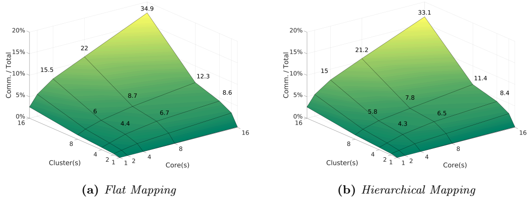
Figure 7.7 – MPPA ® Matrix Results Ratios between NoC Communications and Processing Time (lower is better, lower means more PEs efficiency). Communication Overheads Relative to Total Execution Time.
