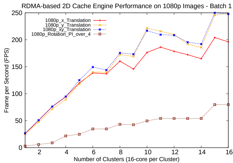
Figure 9.14 – RDMA-based 2D Explicit Cache of Tiles Performance. Full HD Images.
