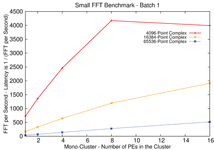
Figure 10.8 – Execution Time of the Mono-Cluster FFT. The Higher, The Better.
