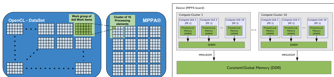
Figure 3.4 – OpenCL Mapping of Applications and Memory Model Source: Kalray's OpenCL User Manual
