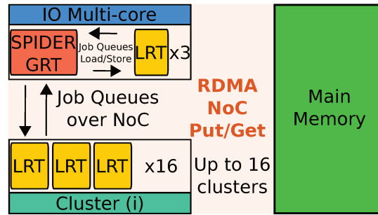
Figure 8.1 – Architecture of the Reconfigurable Dataflow Runtime onto a DMA-Enabled Clustered Manycore Processor
