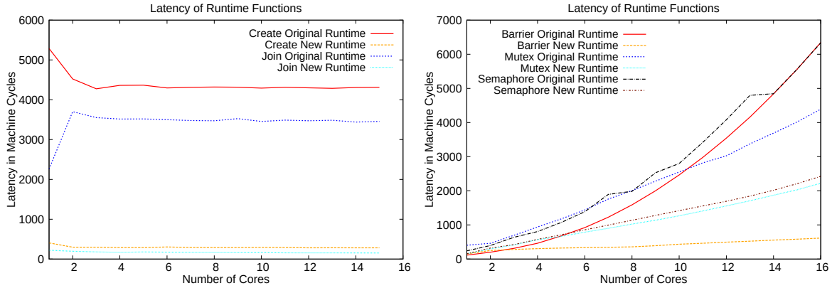
Figure 6.4 – Performance Comparisons of Thread Creation, Join and Basic Synchronization Primitives on 16 Cores
