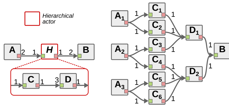
Figure 3.8 – Flattening and the Single-Rate Transformation Hierarchical SDF (left) to Single-Rate DAG (SRDAG) (right)
