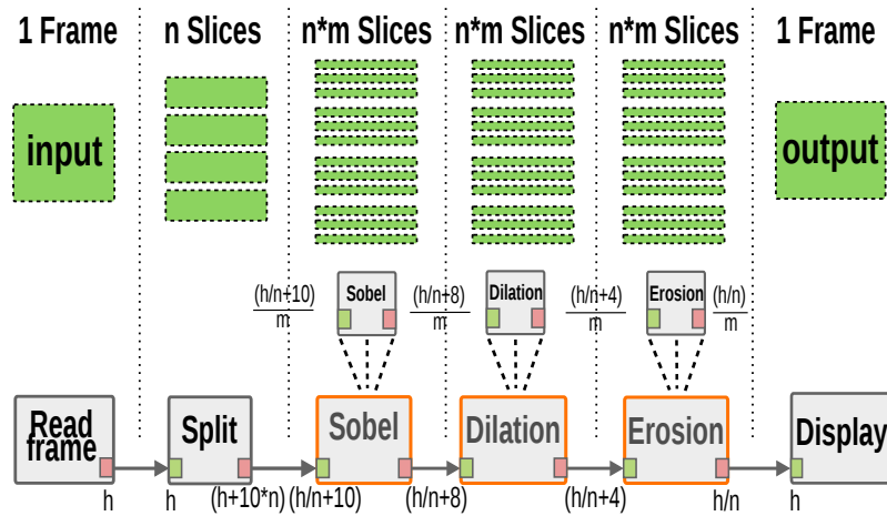
Figure 7.1 – IBSDF Graph: Edges Detection and Denoising
