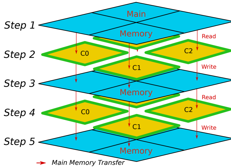
Figure 9.6 – Automated Multi-clusters Tiling
