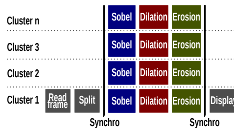
Figure 7.3 – Gantt Chart of the Hierarchic Scheduling
