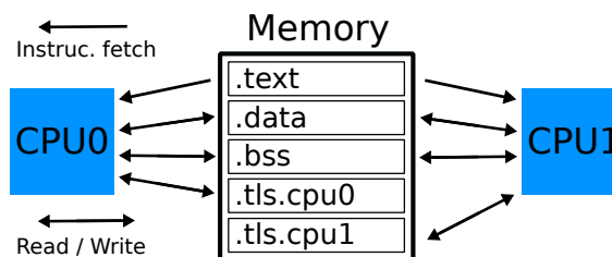
Figure 2.5 – Typical CPU Cores Linked to a Memory with Memory Access examples
