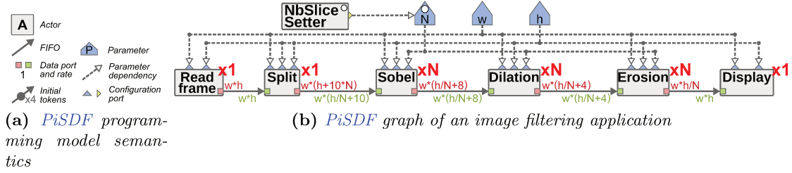
Figure 3.11 – PiSDF Programming Model Semantics and Example
