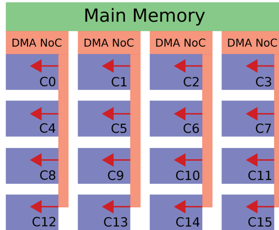
Figure 10.11 – Broadcast Operation From the Main DDR3 Memory to the CCs .
