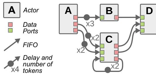
Figure 3.5 – DPN Programming Model Example and Semantic
