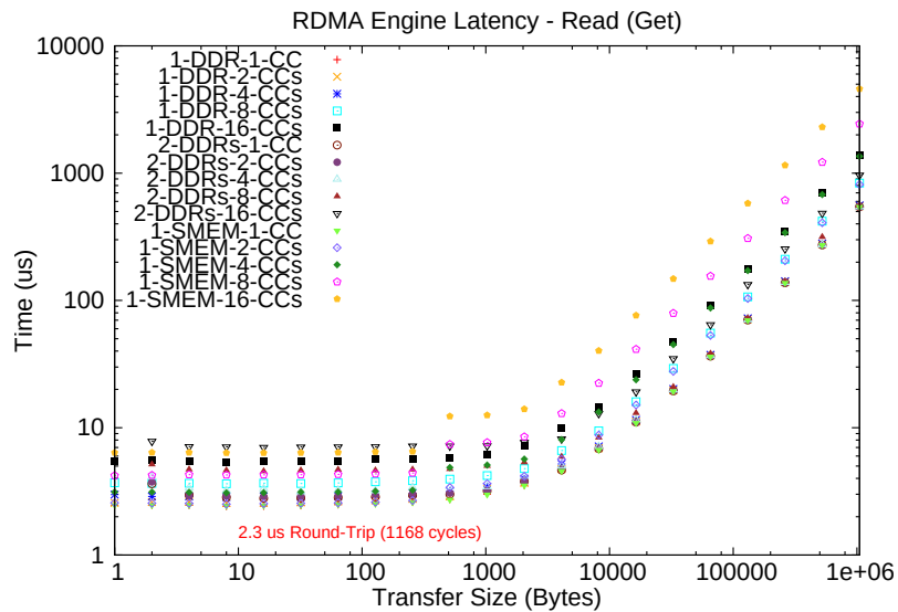
Figure 5.9 – RDMA Get (Read) Latency \mu s (Blocking)
