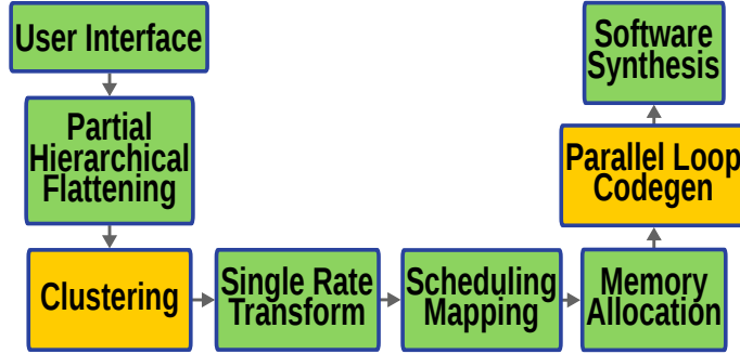
Figure 7.2 – New PREESM Workflow for Clustering and Parallel Loop Generation
