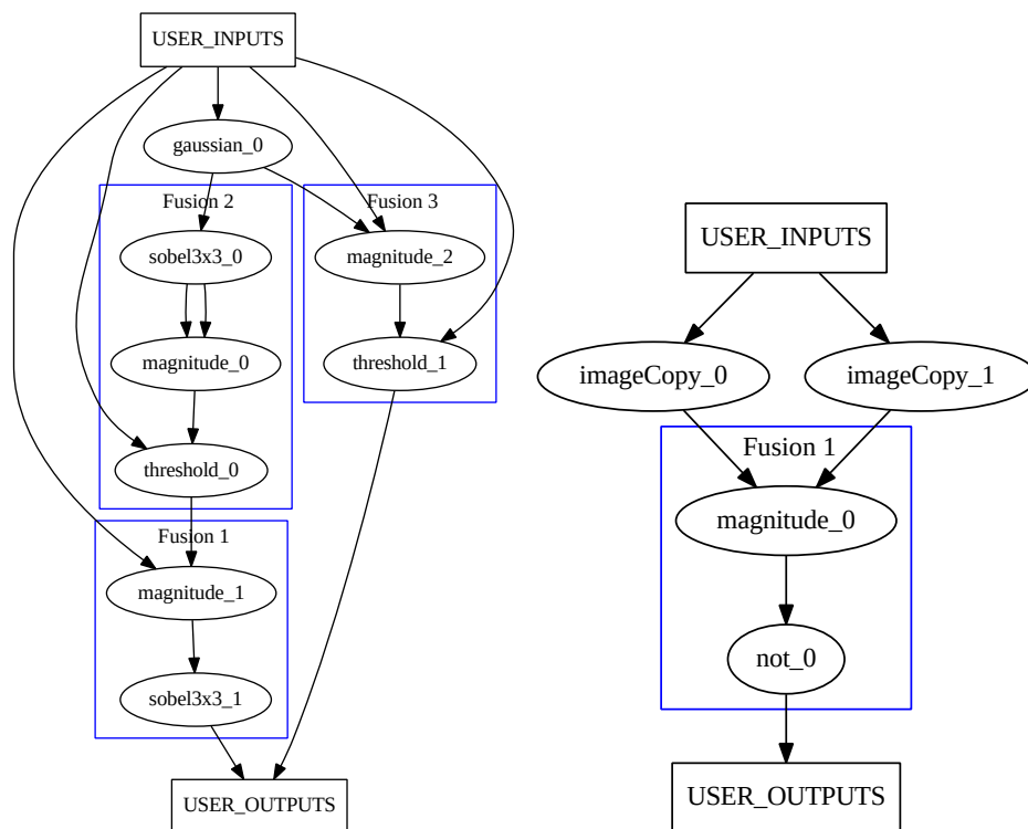
Figure 9.5 – Example of a Graph Display from the IO , Schedule and Fusion Optimizations
