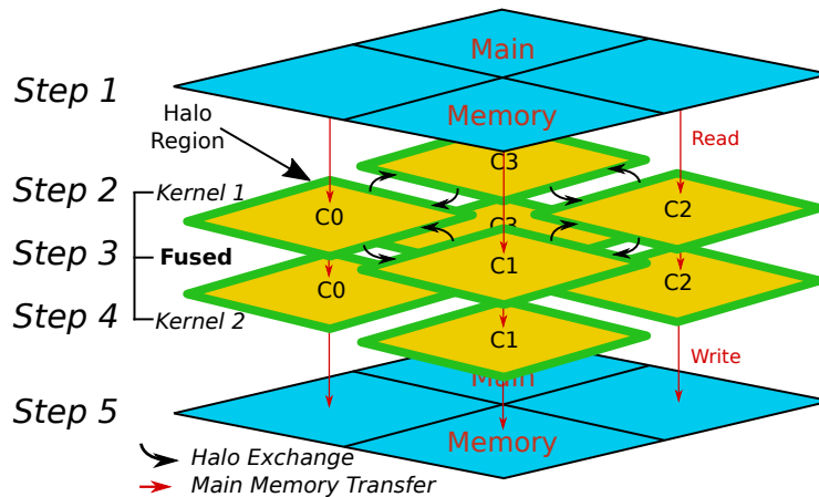
Figure 9.7 – Automated Multi-clusters Tiling Combined with Fusion
