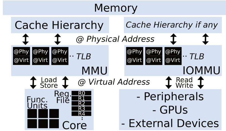
Figure 2.6 – (IO)MMU Role in a Heterogeneous Computer System
