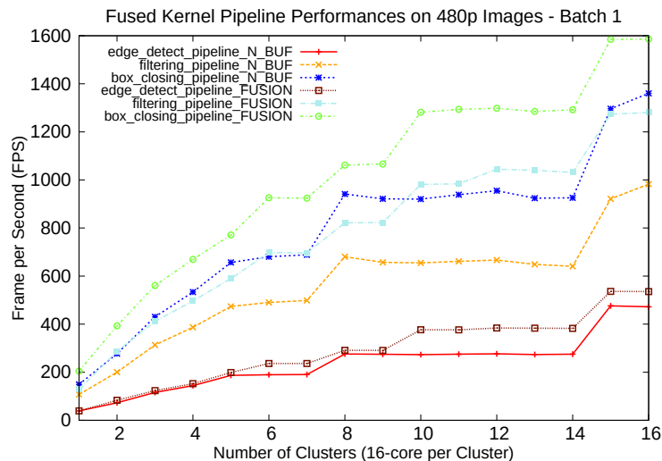
Figure 9.11 – Automatic RDMA -based Kernel Fusion Performance. VGA Images. Tiling with N-Buffering ( N_BUF = N-Buffering = Prefetch) vs Kernel Fusing ( FUSION ).
