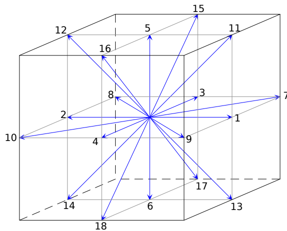
Figure 10.1 – LBM D3Q19 Stencil
