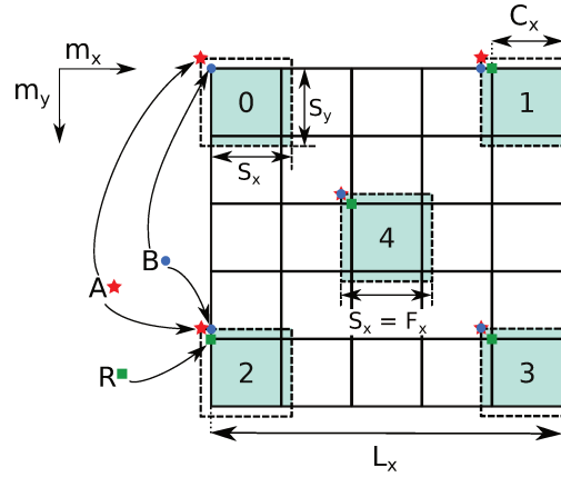
Figure 10.3 – Local/Remote copied index in 2D (in lattice node) with A : beginning of the local buffer = (0,0) ; R : beginning of the remote main node 3D tile (without halo); B : beginning of the copied 3D tile ( S ), represented by: B_a : index of S on local memory (from A ) and B_r : index of S on main memory (from R ).
