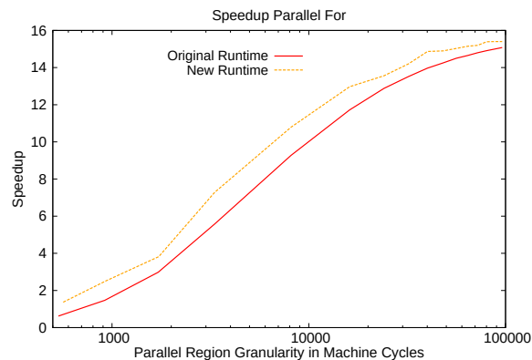
Figure 6.6 – Performance of the OpenMP GCC libgomp, Based on our New Multi-threading Runtime with 16 Threads Running
