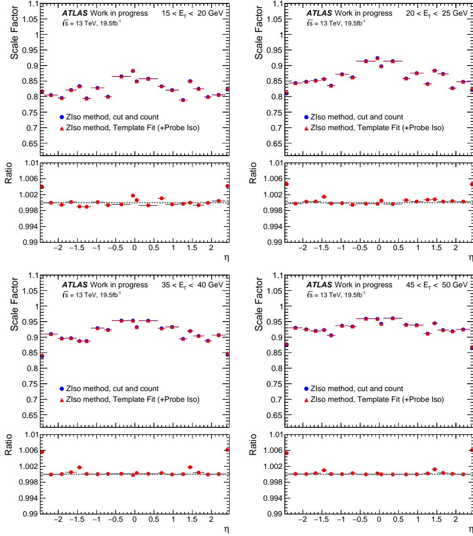
Figure 5.26 – Comparison of the Tight scale factor results for four E_T bins as a function of \eta for the cut-and-count Z_{\text{iso}} method and the template fit Z_{\text{iso}} method with a probe isolation cut at E_T^{\text{cone},r} < 0.5 applied.
