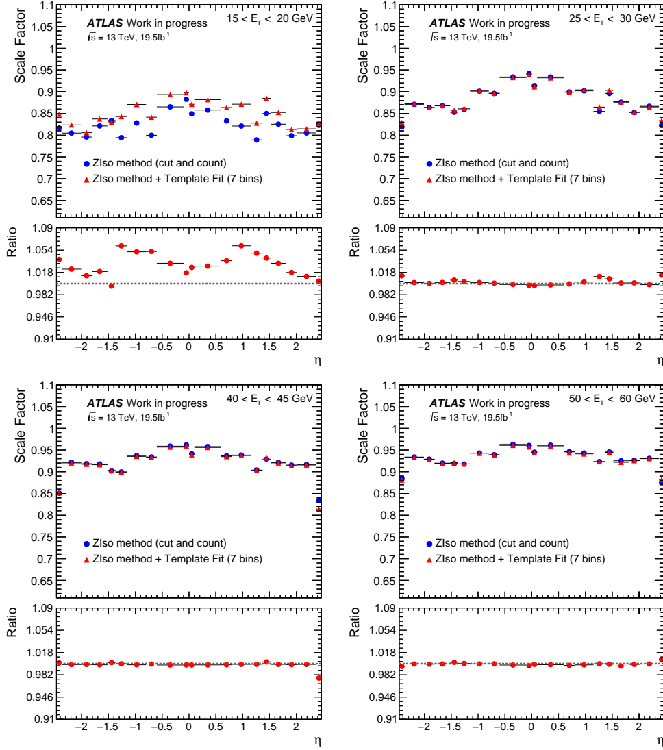
Figure 5.32 – Scale factor results obtained with a template fit to the isolation distribution divided into seven bins are indicated by the red triangles as a function of \eta for four bins in E_T . The results are compared to scale factor results obtained with the cut-and-count method (blue dots).
