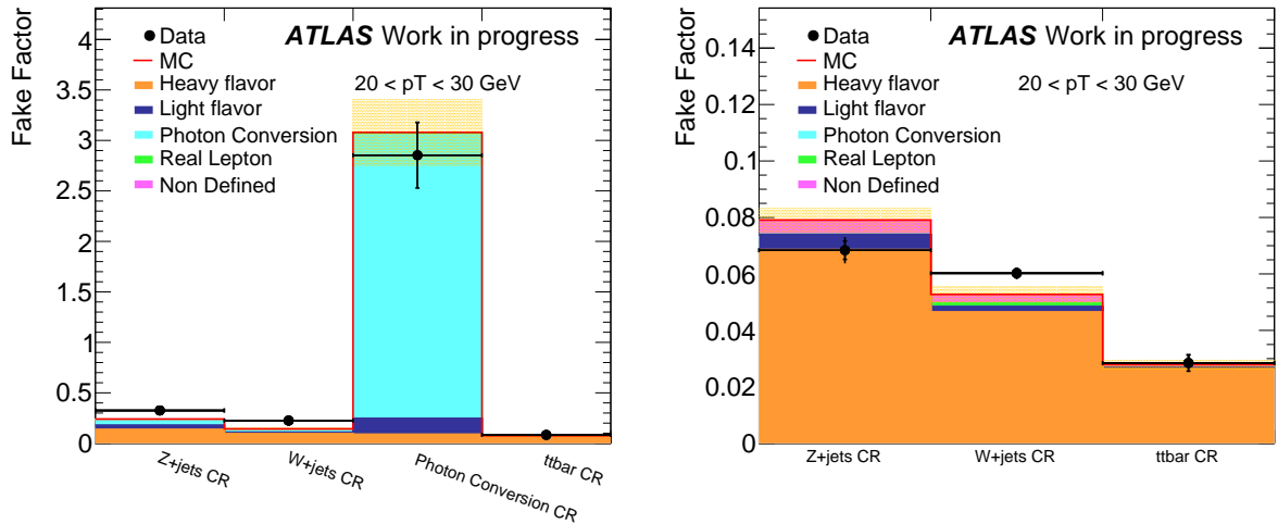
Figure 6.9 – Fake factor results for fake Z -type electrons (left) and Z -type muons (right) from all control regions for 20 < p_T < 30 GeV. Data fake factors are illustrated as black dots, the red histogram represents the MC fake factors. The difference between those two is expected as the identification and isolation cuts are not well modelled in MC for fake leptons. The coloured bars show the relative contribution of each fake lepton source, it is represented as the MC fake factor times the fake lepton source's relative contribution.
