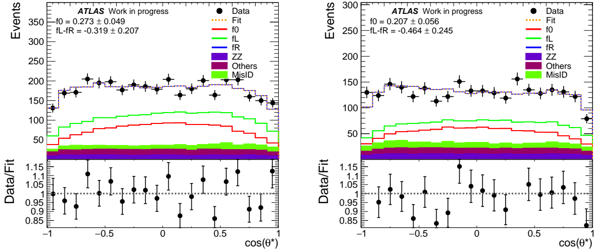
Figure 8.8 – Fit to the \cos(\theta^*) distribution in data to extract the Z-polarisation (in W^+Z events: left, in W^-Z events: right). The resulting polarisation fractions f_0 and f_L - f_R are displayed on the figure along with their total uncertainties. All background distributions and fitted polarisation templates are stacked in the plot. The ratio plot illustrates the agreement of the fit with data.
