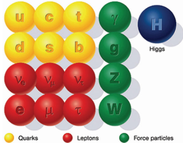
Figure 2.1 – Overview over all known particles in the Standard Model. Details are given in the text.
