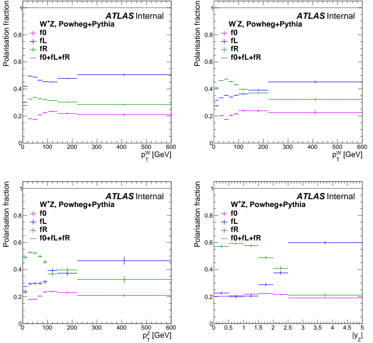
Figure 3.8 – Examples of the dependence of the polarisation fractions on the boson p_T and the boson rapidity. In the top row, the polarisation fractions as a function of p_T in the total phase-space are shown for W^+ (left) and W^- (right) bosons. In the bottom row, the polarisation of Z in W^+Z events as a function of the p_T of the Z boson is shown on the left and as a function of the Z rapidity on the right. From [82].
