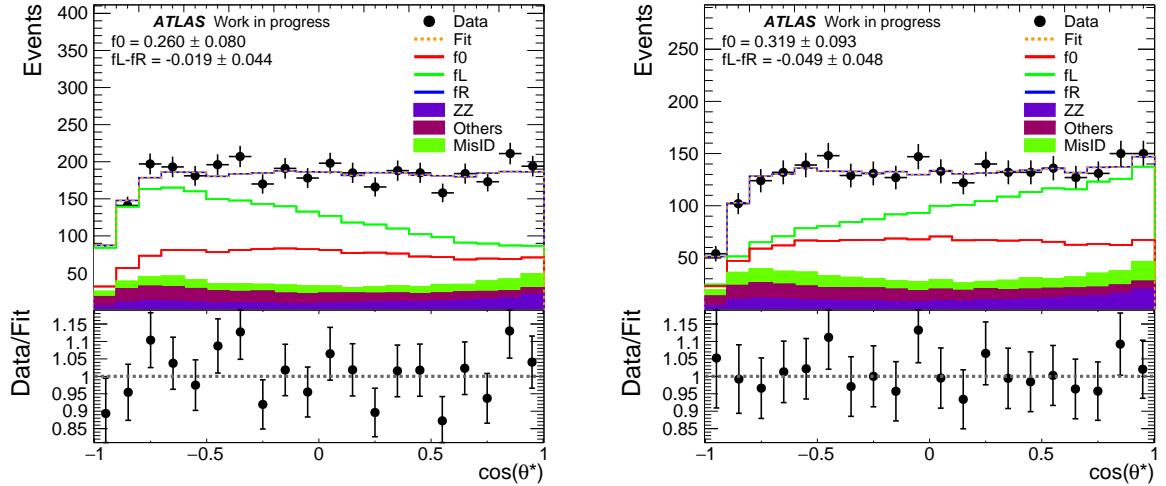
Figure 8.7 – Fit to the \cos(\theta^*) distribution in data to extract the W -polarisation ( W^+ -polarisation: left, W^- -polarisation: right). The resulting polarisation fractions f_0 and f_L - f_R along with their total uncertainties are displayed on the figure. All background distributions and fitted polarisation templates are stacked in the plot. The ratio plot illustrates the agreement of the fit with data.
