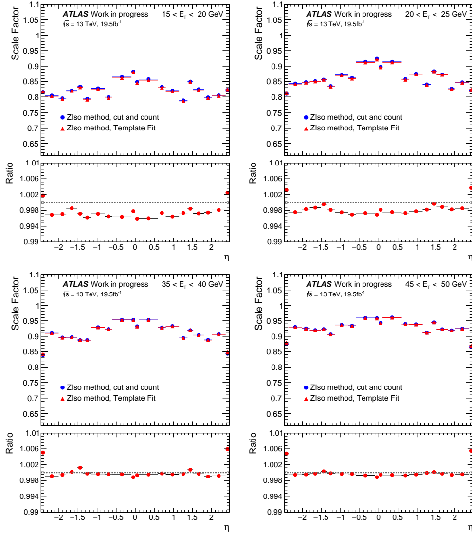
Figure 5.25 — Comparison of the scale factor results for the Tight working point obtained with the cut-and-count Z_{\text{iso}} method and the Z_{\text{iso}} template fit method for a fit of the model to data in two bins.
