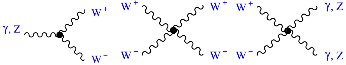
Figure 2.2 – Triple and quartic gauge coupling vertices. From [37].
