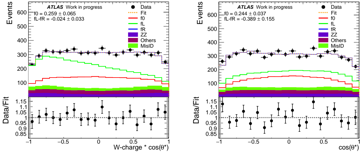
Figure 8.9 – Fit to the \cos(\theta^*) distribution in W^\pm Z events in data to extract the W-polarisation (left) and the Z-polarisation (right). The resulting polarisation fractions f_0 and f_L - f_R are displayed on the figure along with their total uncertainties. All background distributions and fitted polarisation templates are stacked in the plot. The ratio plot illustrates the agreement of the fit with data.
