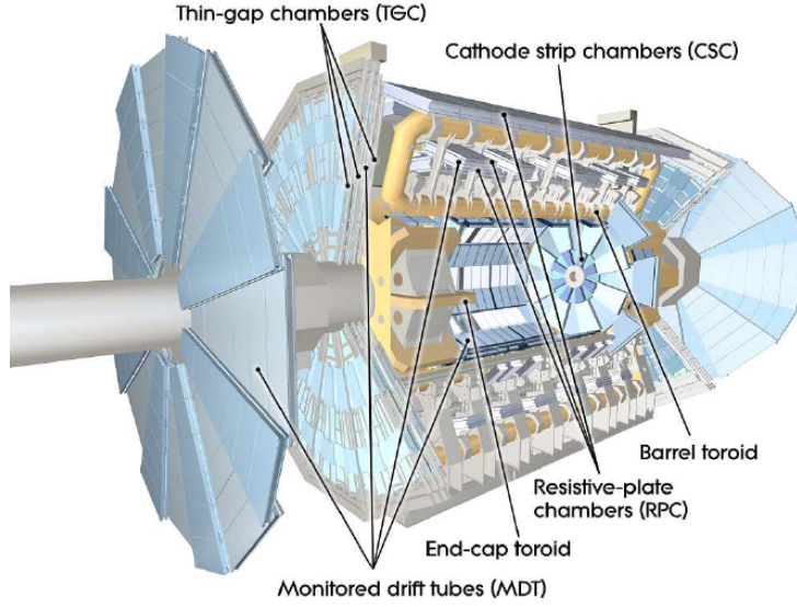
Figure 4.8 – Cut-away view of the ATLAS muons system. From [96].
