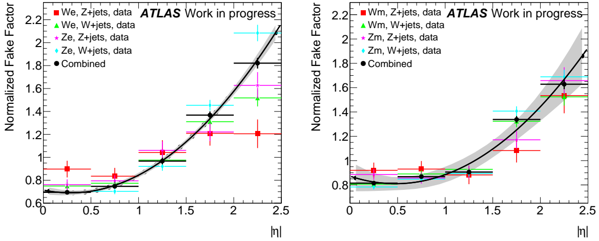
Figure 6.6 – Fit of a parabolic function to the weighted mean of W - and Z -type lepton fake factor distributions F_V(|\eta|) of the W +jets and Z +jets control regions (black dots). Electrons and muons are treated separately and displayed on the left and right, respectively. The shaded band around the fit result displays its 68% confidence interval. Full total uncertainties are displayed.
