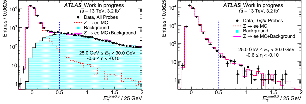
Figure 5.7 – Example of the probe isolation distribution of the selected data events (black dots) and the scaled background template representing the isolation distribution of fake electrons (blue shaded area). The Z \rightarrow ee MC simulation is plotted with red dots and the sum of MC and scaled background template is represented by the purple distribution which should match the data. The background template in this figure was scaled to data in the tail region E_T^{\text{cone},r}/25 \text{ GeV} > 0.5 (indicated by the vertical blue dotted line), real electrons in the tail of the isolation distribution were considered. The agreement to data is good for both reconstructed electrons (left) and Tight probes (right).
