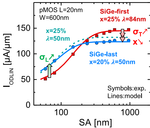
Figure 4.42: I_{ODLIN} vs. SA for SiGe-first and SiGe-last ( W=600\text{nm} and L=20\text{nm} ). Crossover is explained by both the lower initial stress from lower Ge concentration and the lower typical relaxation length in SiGe-last.
