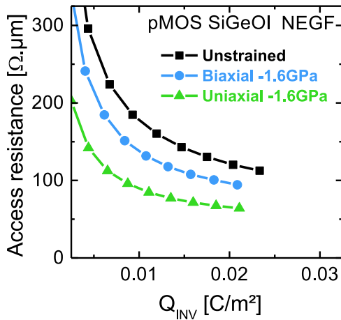
Figure 2.20: 2D NEGF simulations of SiGeOI pMOSFET access resistance under different stress configurations considering ballistic and phonon contributions. The access resistance is reduced under compressive stress. Especially, the longitudinal stress (i.e. parallel to the 110-oriented channel) is highly beneficial.
