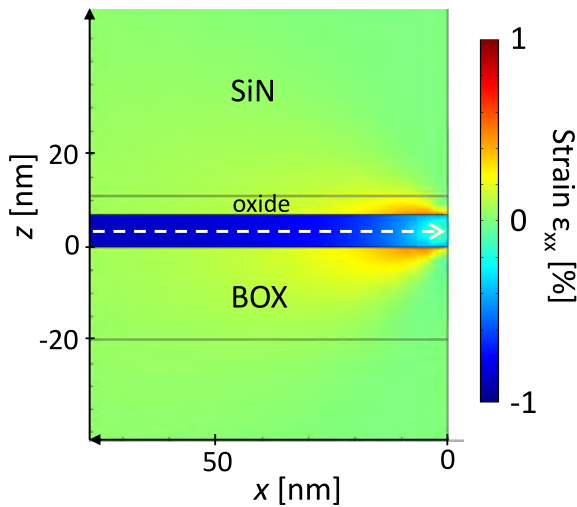
Figure 3.12: Strain \varepsilon_{xx} mapping of SiGeOI active area after patterning (with focus on the 50nm close to right side). The 55nm-thick SiN layer is considered unstressed. Strain relaxation because of free boundary condition is evidenced. The strain profiles are extracted in the middle of the SiGe layer (represented by the white arrow).
