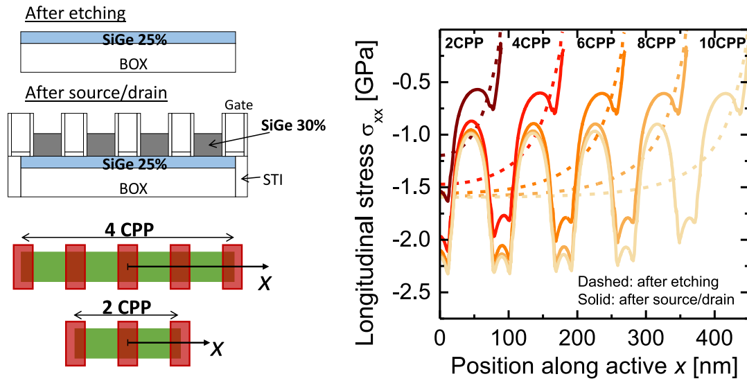
Figure 3.37: (left) Simulated structures with different active lengths (different numbers of CPP). (right) Simulated longitudinal stress profiles for different active lengths, after etching (dashed lines) and after source/drain epitaxy (solid lines). The additional stress from source/drain in the middle of the active area ( x=0 ) is deduced by subtracting the two curves and reported in Figure 3.38.
