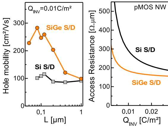
Figure 2.24: (left) Extracted hole mobility as a function of the gate length of pMOSFET \Omega -gate nanowires with either Si or SiGe source/drain. (right) Extracted access resistance on the same devices. SiGe source/drain leads to enhanced hole mobility, especially for short channel devices, and also yields lower access resistance.
