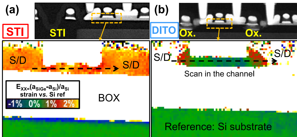
Figure 4.60: PED relative deformation mapping of a device (a) close to STI and (b) between two local oxidations.
