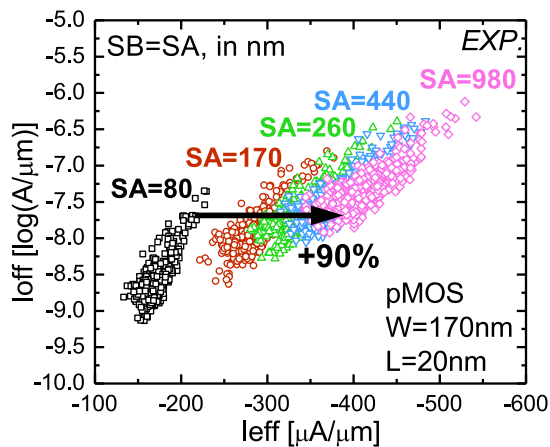
Figure 4.9: pFET I_{EFF}/I_{OFF} at V_{DD}=0.8\text{V} and for different gate-to-STI distances (SA). By increasing the active length, the effective current can be improved by up to +90% at the same leakage.
