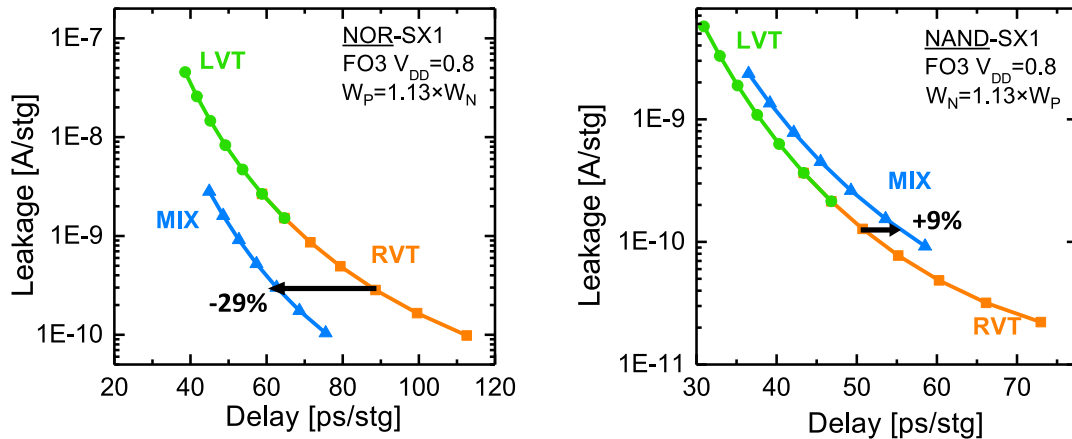
Figure 4.8: (left) NOR-SX1 and (right) NAND-SX1 simulated Leakage/Delay trade-off for the different VT flavors. The MIX flavor reduces the NOR delay by -29% at the same leakage. The NOR logic gate features pFET in series. Hence it is more sensitive to the leakage of the nFET and the speed of the pFET. Reducing the pFET V_T in such a cell improves the speed without a strong leakage penalty. It is the opposite for the NAND logic gate: the MIX flavor is thus irrelevant in this case.
