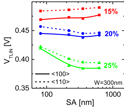
Figure 3.48: V_{TLIN} vs. SA for \langle 100 \rangle and \langle 110 \rangle SiGe channel of different Germanium concentrations. The higher the Germanium concentration, the lower the threshold voltage, as already observed [Cas12b; Sou13].
