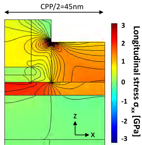
Figure 3.32: Simulated longitudinal stress \sigma_{xx} mapping in a pMOSFET with SiGe channel and SiGe source/drain. Only half of the structure is simulated for symmetry reasons.
