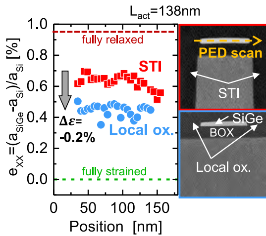
Figure 4.58: PED scan in SiGeOI isolated by STI or oxidation. A higher compressive strain is obtained by oxidation.
