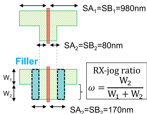
Figure 4.19: Schematics and definition of RX-jog ratio \omega and dedicated test structures (with and without filler cell).
