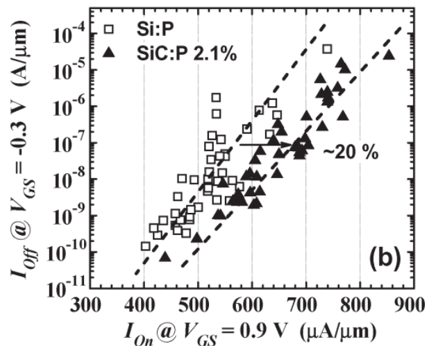
Figure 1.41: (left) Schematic of the tensile stress generated by SiC:P source/drain for nMOSFETs and (b) I_{ON}/I_{OFF} trade-off highlighting +20% ON-current with the introduction of Carbon in source/drain, from [Lio08]. The principle of this technique is the same as using SiGe source/drain stressor but since Carbon has a smaller lattice parameter than Silicon, a tensile stress is generated. Only few percents of Carbon lead to a significant tensile strain. The main challenge of this technique is to avoid silicon-carbide precipitation with anneals (the Carbon must be substitutionally incorporated for the Si:C to be stressed) [Tog12].
