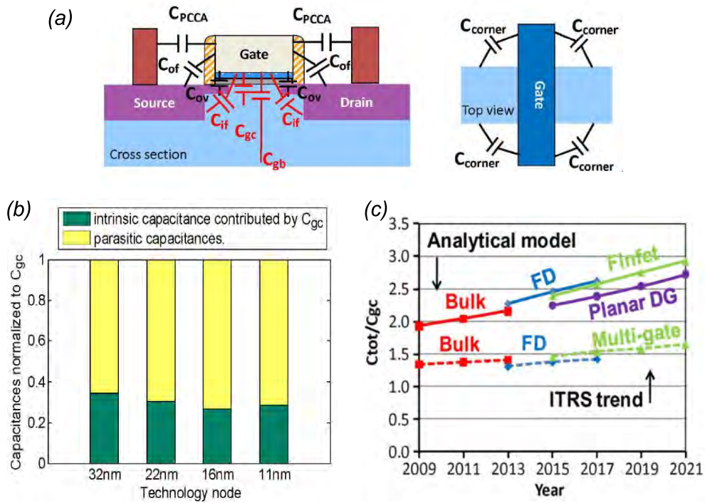
Figure 1.25: (a) Parasitic capacitances, from [Wei11]. (b) Parasitic capacitance contribution with respect to the intrinsic capacitance according to the technology node, from [Wei11]. (c) Total vs. intrinsic capacitance over the years for the different architectures, from [Lac12]. The parasitic capacitances become more and more dominant.
