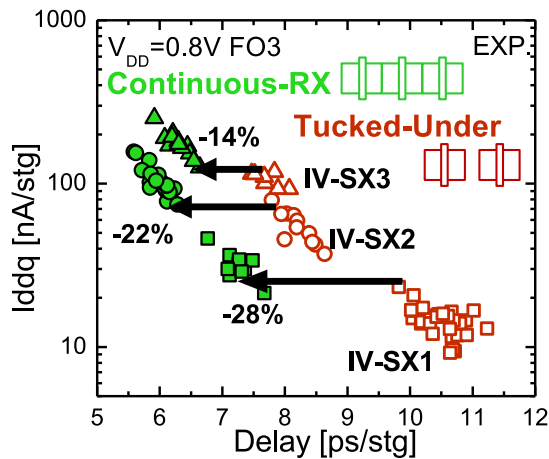
Figure 4.14: Experimental Delay/Leakage trade-off for ring-oscillators of inverters. Continuous-RX designs demonstrate high gain vs. Tucked-Under (-28% for 1-finger).
