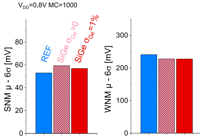
Figure 4.29: SRAM (left) SNM and (right) WNM \mu - 6\sigma at V_{DD}=0.8\text{V} after 1000 Monte Carlo simulations. Considering an additional source of variability for Ge concentration fluctuation does not impact the margins as the SRAM cell is more sensitive to local variability than global one.
