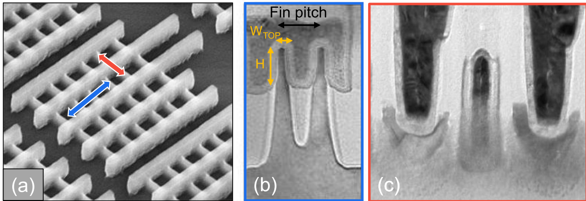
Figure 1.20: (a) FinFET SEM tilted top view, emphasizing the 3D architecture, from [Aut12]. (b) Cross-section in the gate of FinFET from 14nm node [Nat14], showing the FinFET height, top width and footprint. (c) Cross-section along the source/drain direction, from [Aut12].
