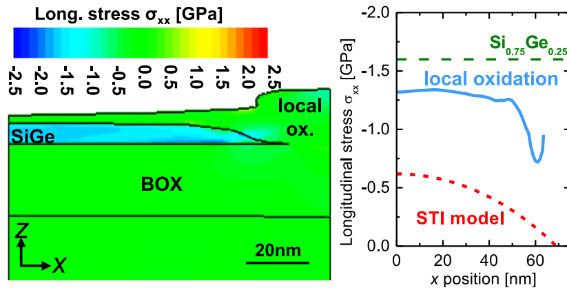
Figure 4.57: process simulation of local oxidation: (left) mapping of longitudinal stress after oxidation and (b) scan in the SiGe layer (blue line). Even though the stress is not fully maintained (lower value than the dashed green line), a high level of stress is expected (-1.3GPa). The STI model (dashed red line) is also plotted for comparison.
