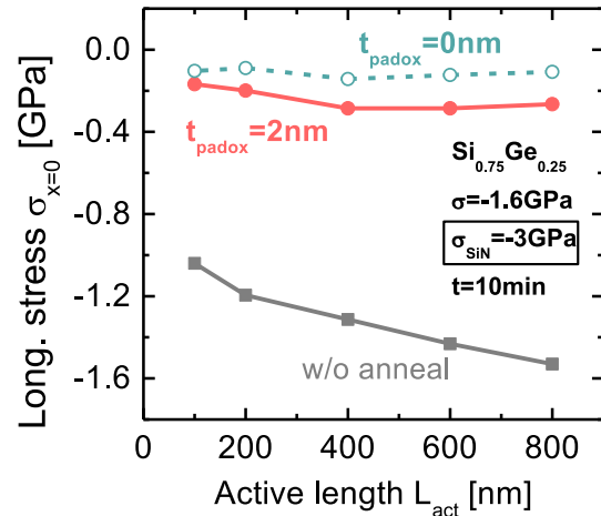
Figure 5.21: Simulated stress in the middle of the SiGe active area after BOX-creep with initially compressively stressed SiN layer. Strong relaxation of the SiGe compressive stress is expected.
