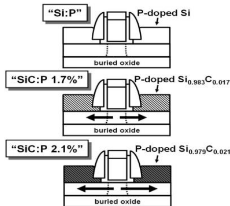
Figure 1.41: (left) Schematic of the tensile stress generated by SiC:P source/drain for nMOSFETs and (b) I_{ON}/I_{OFF} trade-off highlighting +20% ON-current with the introduction of Carbon in source/drain, from [Lio08]. The principle of this technique is the same as using SiGe source/drain stressor but since Carbon has a smaller lattice parameter than Silicon, a tensile stress is generated. Only few percents of Carbon lead to a significant tensile strain. The main challenge of this technique is to avoid silicon-carbide precipitation with anneals (the Carbon must be substitutionally incorporated for the Si:C to be stressed) [Tog12].
