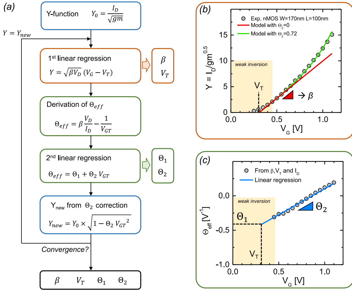
Figure 2.10: Y-function iterative procedure for extraction of parameters. Two successive linear regressions are performed until convergence is achieved.
