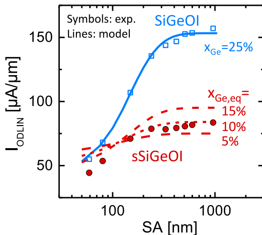
Figure 5.5: I_{ODLIN} current as a function of the gate-to-STI distance SA for both SiGeOI and sSiGeOI W=600\text{nm} L=20\text{nm} pFET devices. The sSiGeOI I_{ODLIN} current is degraded with respect to the reference SiGeOI because of lower initial compressive stress. The model, calibrated on the reference, enables to reproduce the sSiGeOI data assuming an equivalent Ge concentration of x_{Ge,eq}=10\% . The typical relaxation length is \lambda=82\text{nm} .
