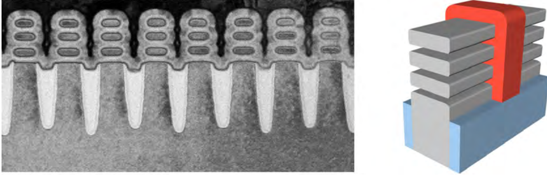
Figure 1.24: (left) Stacked nanosheets cross-section, from [Lou17] and (right) 3D view. The gate all around architecture enables a good electrostatic control. A high drive current is achieved by stacking the nanosheets and using a large width (hence the name nanosheet is preferred to nanowire).
