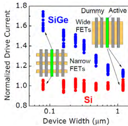
Figure 1.51: FDSOI device drive current improvement with SiGe active narrowing, from [Che12]. The enhancement is due to beneficial uniaxial stress configuration. Inset: optimized design by slicing a large active into several narrow actives.
