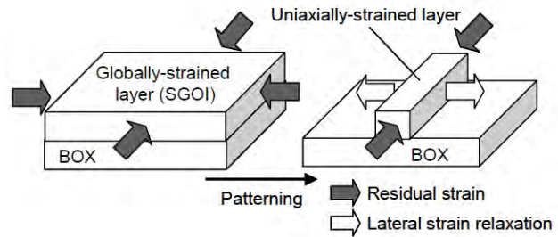
Figure 1.49: Illustration of patterning-induced SiGe strain relaxation, from [Iri05]. The patterning of SiGe on insulator (SGOI) active area shape changes the stress configuration from biaxial to uniaxial.
