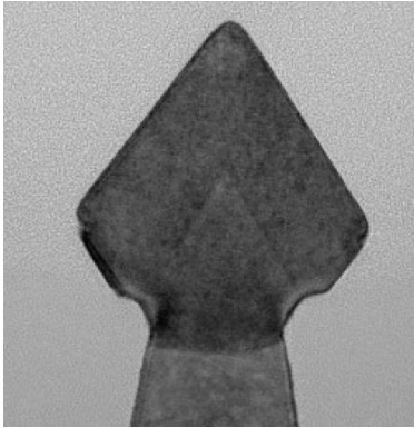
Figure 1.37: TEM cross-section of a FinFET in the source/drain area, showing the SiGe epitaxy, from [Aut12]. The compressive stress generated by SiGe source/drain has been introduced since the bulk 90nm technology [Gha03] and has been integrated into FinFET technologies as well as FDSOI technologies [Web15]. The diamond shape is due to the growth rate dependence with crystal orientation.
