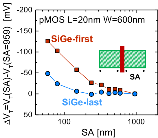
Figure 4.40: The threshold voltage shift \Delta V_T with respect to the long active configuration (SA=959nm). Higher V_T shift is observed for SiGe-first compared to SiGe-last.
