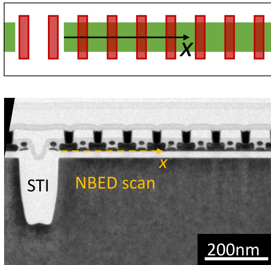
Figure 3.35: Layout and TEM image of the NBED measurement of Figure 3.36 realized after MEOL from the active edge ( x=0 ).
