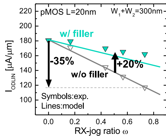
Figure 4.20: I_{ODLIN} as a function of the RX-jog ratio \omega with or without filler cell. Using a filler cell enables a higher stress in the channel, which is translated into a higher mobility.
