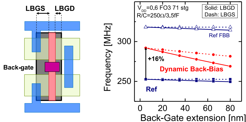
Figure C.38: (left) Layout of the 1-finger inverter with local back-gate. Definition of the back-gate extensions over front-gate on the source and drain sides, LBGs and LBGD, respectively. (right) Frequency as a function of the back-gate extensions. Under static bias, the back-gate extension does not significantly impact the performance. Under dynamic back-bias however, LBGs and particularly LBGD reductions enhance the frequency.
