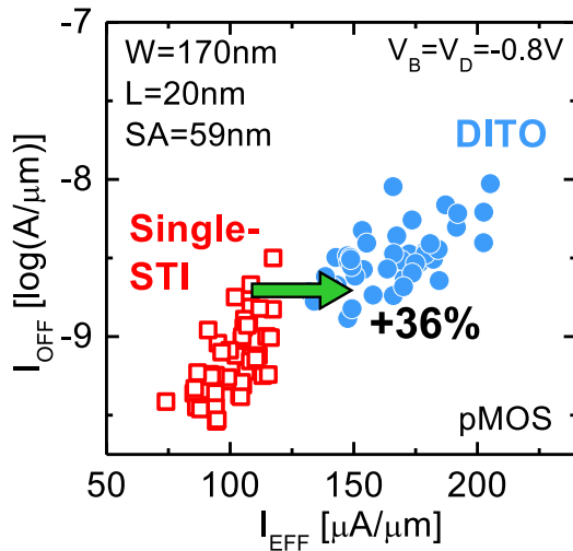
Figure 4.62: I_{\text{EFF}}/I_{\text{OFF}} trade-off for pMOSFETs showing +36% improvement with DITO over single-STI.
