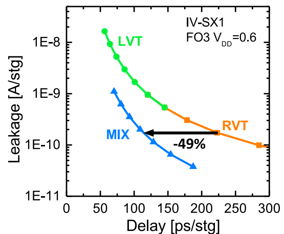
Figure 4.4: Simulated Leakage/Delay trade-off for 1-finger inverter (IV-SX1) at V_{DD}=0.6V and for different flavors: LVT, RVT and MIX. The MIX flavor delay is expected to be reduced by -49% at the same leakage with respect to RVT flavor. At low supply voltages, the gate overdrive ( V_{DD}-V_T ) is decisive. Hence the strong interest to have balanced threshold voltages.
