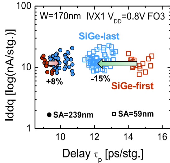
Figure 4.45: Experimental I_{\text{DDQ}}/\tau_p of a inverter ring oscillator of inverter (IVX1, L=20\text{nm} , W_n=W_p=170\text{nm} , V_{\text{DD}}=0.8\text{V} ) loaded with a fan-out 3. It demonstrates a delay increase with SiGe-last for long active regions (+8% for SA=239\text{nm} ) and a delay reduction for short active (-15% for SA=59\text{nm} )
