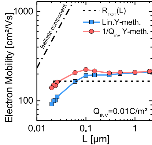
Figure 2.16: Extracted electron mobility at Q_{INV}=0.01\text{C}/\text{m}^2 with respect to the channel length according to the method used. The mobility drop obtained with the classical Y-function is mitigated with our proposed method.
