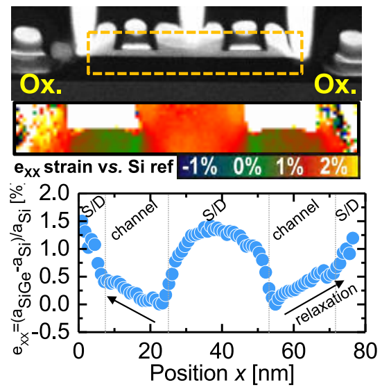
Figure 4.59: PED e_{XX} (top) mapping and (bottom) scan in a SiGeOI device constituted of two channels and isolated by local oxidation. The profile shows the impact of SiGe source/drain and evidences a slight relaxation close to the isolation ( e_{XX} increases, represented by the arrow). High level of stress is however evidenced in the channels ( e_{XX} = 0 \approx \sigma_L = -1.6 GPa).
