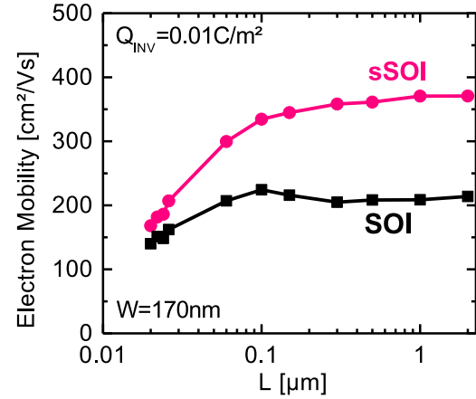
Figure 2.18: Extracted electron mobility \mu at Q_{INV}=0.01C/m^2 by our new 1/Q_{INV} Y-method (presented in section 2.2.3.b) as a function of the gate length L for W=170nm nFETs built on either SOI or sSOI substrates.
