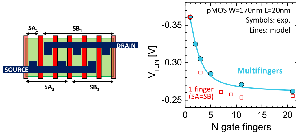
Figure 3.60: (left) multifinger layout with all the gate fingers connected in parallel. (right) V_{TLIN} as a function of the number of gate fingers. The 1-finger case is also plotted to highlight the impact of strain relaxation on fingers close to the active area edge. Multifinger model reproduces well the experimental data.
