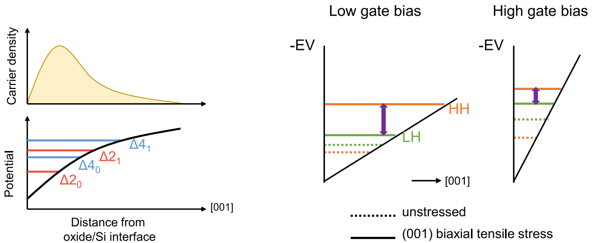
Figure 1.34: Schematic (top) carrier density and (bottom) band diagram in a MOSFET in inversion with respect to the distance from the oxide/Silicon interface. The electric confinement in the out-of-plane direction results in band splitting. \Delta_2 -valleys are preferentially populated in the conduction band (and HH in the valence band).
