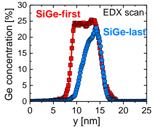
Figure 4.37: EDX scan of SiGe-first and SiGe-last across the channel thickness (see Figure 4.36). The bilayer of SiGe-last is evidenced with x_{\text{last}}=20\% , while SiGe-first Ge concentration is x_{\text{first}}=25\% .
