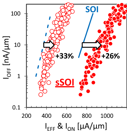
Figure 5.1: I_{EFF} & I_{ON} vs. I_{OFF} at V_{DD}=0.8 for sSOI W=170 nm nFETs compared to reference SOI in 14nm FDSOI technology. Performance improvement is demonstrated with sSOI, showing +26% I_{ON} and +33% I_{EFF} at the same leakage.
