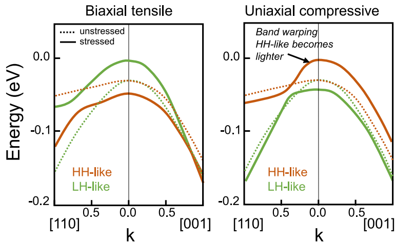
Figure 1.32: Relation of dispersion E(k) for the valence band in case of (left) biaxial tensile stress and (right) \langle 110 \rangle uniaxial compressive stress, compared with the unstrained reference (dotted lines), adapted from [Lee05; Nay94; Sun07]. The strain leads to band shifting, degeneracy lifting and also band warping.
