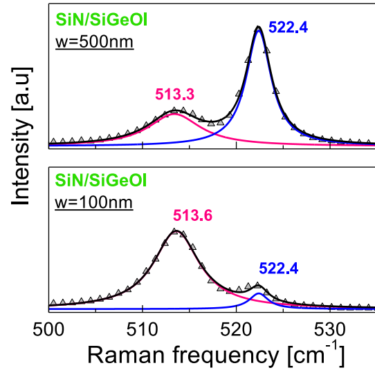
Figure 3.28: SiN/SiGeOI sample \mu Raman spectra for different stripe widths. The peak positions are determined using Lorentzian function fit.
