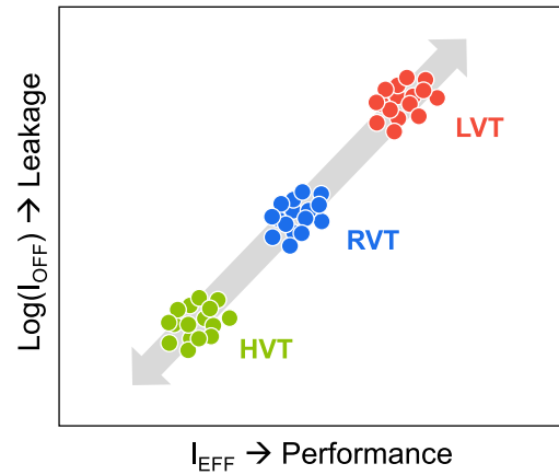
Figure 1.12: Performance/Leakage trade-off. A large range is covered thanks to multi V_T flavors (HVT=High- V_T , RVT=Regular- V_T and LVT=Low- V_T ).
