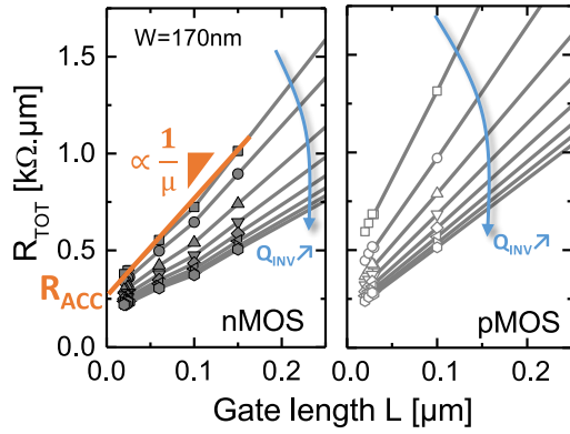
Figure 2.8: R_{TOT}(L) for (left) nMOS and (right) pMOS measured at different inversion charge Q_{INV} . The slope is inversely proportional to the mobility and the intercept gives the access resistance.
