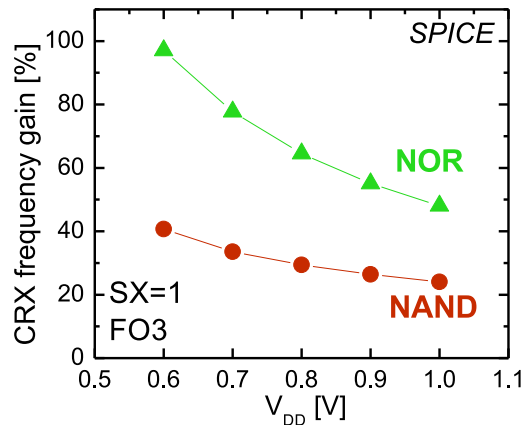
Figure 4.16: CRX frequency gain for NOR and NAND logic gates at different supply voltages. NOR are more impacted because more sensitive to pMOS performance, as they are built in series.
