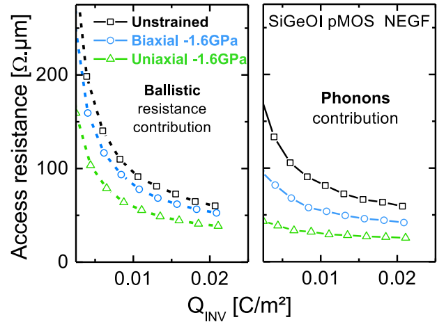
Figure 2.21: 2D NEGF simulations of SiGeOI pMOSFET access resistance under different stress configurations with (left) ballistic contribution only and (right) phonon contribution only. The ballistic resistance reduction is mainly due to the effective mass change, while the diffusive one is induced by subband splitting.
