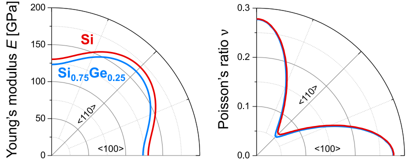
Figure 1.28: Equivalent (left) Young's Modulus and (right) Poisson's ratio of Silicon and SiGe with 25% of Germanium according to the crystal orientation. The plane is (001) oriented.
