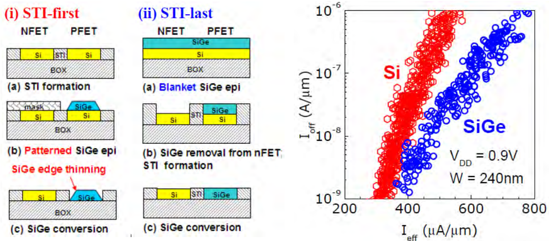
Figure 1.44: (left) Schematic of SiGe integration schemes in FDSOI technology and (right) I_{EFF}/I_{OFF} trade-off for Si and SiGe channel pMOSFETs, from [Che12]. The SiGeOI is fabricated by Ge-enrichment technique (see section 3.1.2.a). It can be done after, before, the STI formation in a so-called STI-first, STI-last, integration scheme, respectively a . The SiGe effective current at the same leakage is increased with respect to Si thanks to the compressive stress in SiGe.
