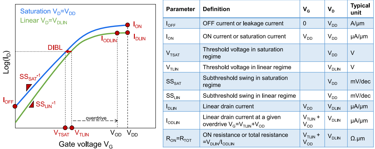
Figure 1.8: (left) MOSFET I_D(V_G) curves in linear and saturation regimes, also called transfer characteristics. (right) Table of the main electrical metrics of the MOSFET, also shown on the I_D(V_G) curve.
