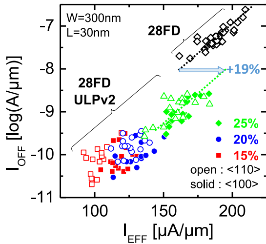
Figure 3.41: I_{EFF}/I_{OFF} trade-off for \langle 100 \rangle and \langle 110 \rangle SiGe channel pFETs of different Germanium concentrations. Performance is improved by 19% with respect to reference 28nm FDSOI technology. While the impact of Ge content is manifest, especially from V_T shift, the channel orientation does not play a significant role.
