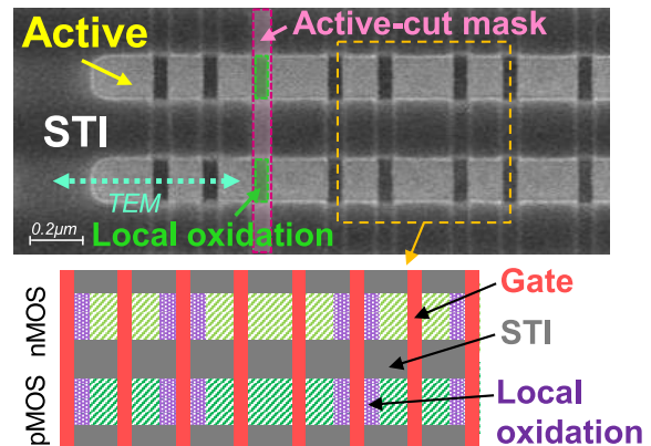
Figure 4.47: SEM top view of the DITO integration scheme after oxidation. Isolation of pMOS stripes from nMOS ones is made with STI while the isolation of transistors within the stripes is made of local oxidation. Corresponding layout is also illustrated showing the "Single-Diffusion-Break" scheme.
