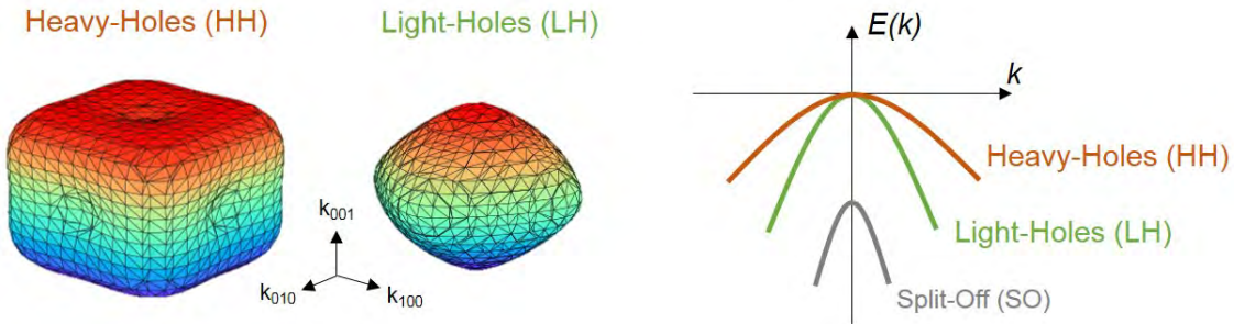
Figure 1.30: (left) Iso-energy surfaces of the two valence subbands at the \Gamma point, called "Heavy Holes" (HH) and "Light Holes", derived from equation 1.49. (right) Schematic of the relation of dispersion in the valence band. The effective mass is inversely proportional to the curvature, hence the "Heavy Holes" and "Light Holes" subband names.
