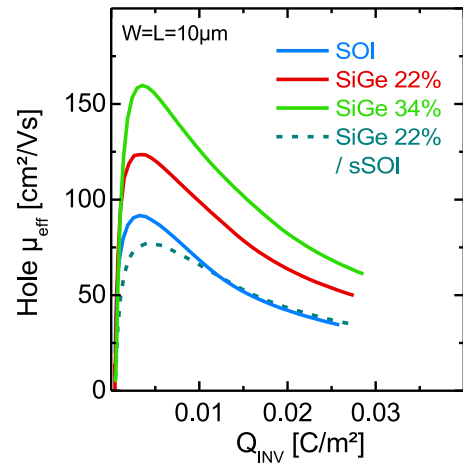
Figure 2.3: Effective hole mobility extracted by split-CV on long channel devices with different Germanium concentrations. The higher the Ge content, the higher the biaxial compressive strain and in turn the higher hole mobility. Similar mobility to SOI is obtained with 22% Ge integrated on sSOI substrate.
