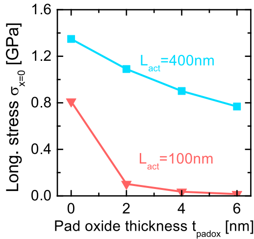
Figure 5.18: Impact of pad oxide thickness for two different active lengths. Strong impact of the presence of a pad oxide for L_{act}=100nm .
