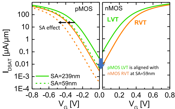
Figure 4.1: Experimental transfer characteristics of the two V_T flavors at V_{DD}=0.8V . Because of the V_T increase induced by stress relaxation, the LVT pFET is aligned with the RVT nFET at SA=59nm .
