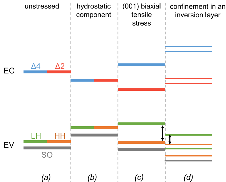
Figure 1.33: Diagrams of band splitting. (a) unstrained Silicon. (b) impact of a hydrostatic strain (i.e. change of volume), altering the band gap but no degeneracies are lifted. (c) impact of biaxial tensile stress, lifting the degeneracies ( \Delta_2 and LH subbands are more favorable). (d) impact of confinement (i.e. in an inversion layer).
