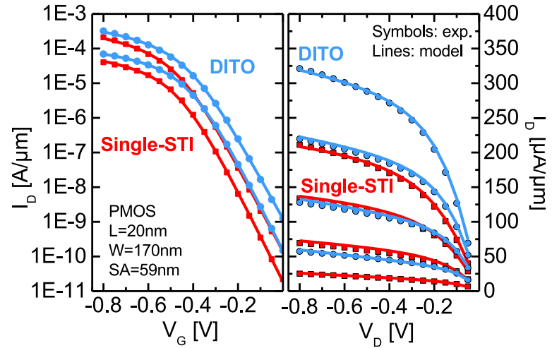
Figure 4.52: Transfer and output characteristics for pFET from DITO and single-STI integration schemes. Model from [Kha09].
