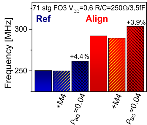
Figure 5.48: Inverters frequency with or without underlined M4 metal line (see the "Align&Bot.M4" layout of Figure 5.46) and for 2 back-gate resistivities \rho = 0.28\Omega\cdot\mu m (doped-Si) or \rho = 0.04\Omega\cdot\mu m (Cu). An underlying M4 metal line does not significantly impact the frequency. A Cu back-gate leads to +4% improvement for both the reference and the "Align" layouts.
