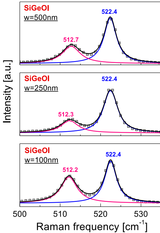
Figure 3.25: SiGeOI sample \mu Raman spectra for different stripe widths. The peak positions are determined using Lorentzian function fit. The pink line corresponds to the SiGe peak and the blue line to the Si bulk reference. The narrower the stripe, the lower frequency, because of the strain relaxation occurring at the edge.
