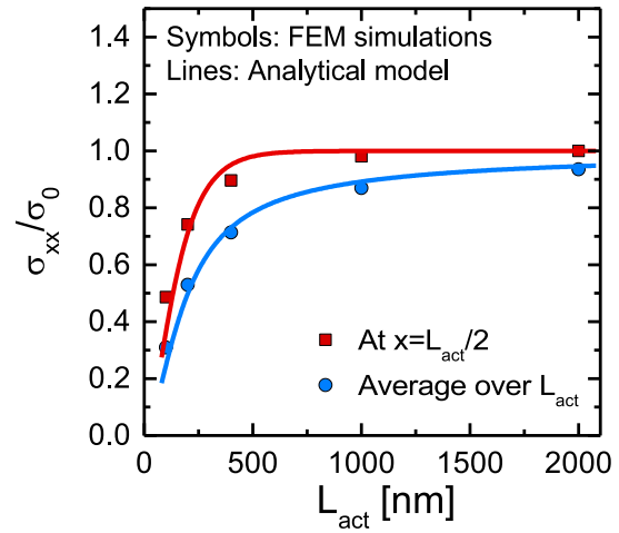
Figure 3.17: Patterned SiGeOI normalized stress at the center (i.e. at x = L_{act}/2 ) and mean stress given by FEM simulations and compared to the analytical model of Equation 3.19 using \lambda = 54\text{nm} . The analytical model enables to properly reproduce the impact of the relaxation on two edges.
