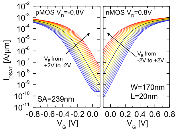
Figure 4.67: pFET and nFET I_D(V_G) at different V_B with 4V body bias range, enabling to shift the threshold voltage. Forward Back-Bias consists in positive, negative, V_B for nFET, pFET, respectively. Reverse Back-Bias is the opposite.
