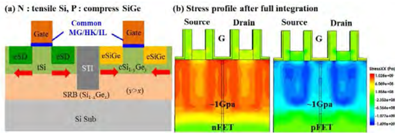
Figure 1.46: (left) Schematic of the dual stress integration technique using a Strain-Relaxed SiGe Buffer (SRB) and SiGe channel for pFET, and (right) inherent simulated stress mapping, from [Bae16]. The Si nFET channel is tensile strained because of the SRB. The SiGe pFET channel is compressively stressed under the condition that the Ge concentration in the channel is higher than the one in the SRB (i.e. y > x ).
