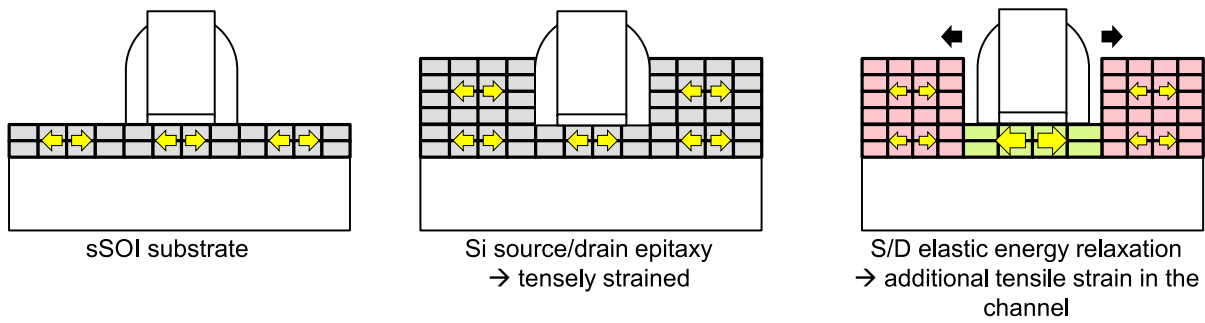
Figure 5.4: Illustration of the additional stress generated by Si epitaxy for devices built on a sSOI substrate. Since the raised source/drain are grown on a tensely strained substrate, they feature a tensile strain as well. As the elastic energy can partially relax in these regions because of the geometry, the channel region is dragged, generating a tensile stress.
