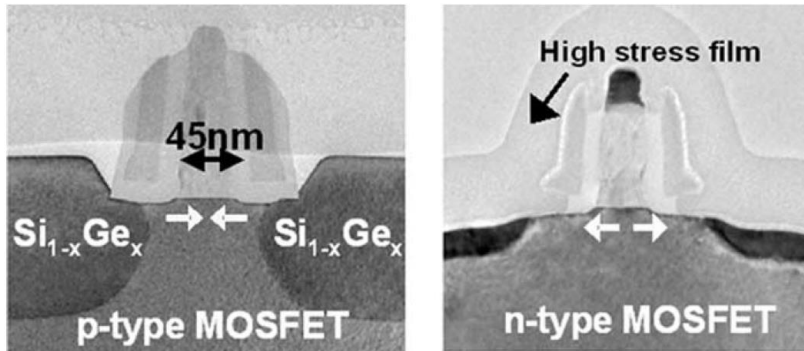
Figure 1.17: First stress introduction in Intel's 90nm technology [Gha03][Tho04]. Both pMOS and nMOS benefit from local stress introduction. Compressive stress from SiGe source/drain is used for the pMOS and tensile stress from a stressed SiN film is used for nMOS. Figure from [Tho04].
