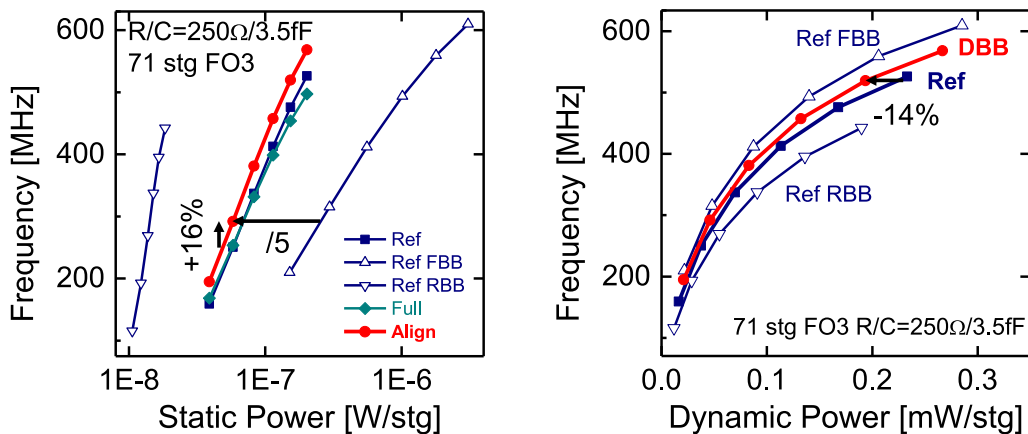
Figure 5.49: Frequency vs. (left) static power P_{STAT}=I_{DDQ}\cdot V_{DD} and (right) dynamic power P_{DYN}=I_{DYN}\cdot V_{DD} . The local back-gate "Align" configuration has same static power than the reference because of same bias configuration in OFF-state, but frequency is improved by +16%. The Dynamic Back-Bias of the "Align" case leads to 14% dynamic power saving at same frequency compared to the reference. The FBB regime is still the most relevant for dynamic power, but at the expense of a higher static power consumption.
