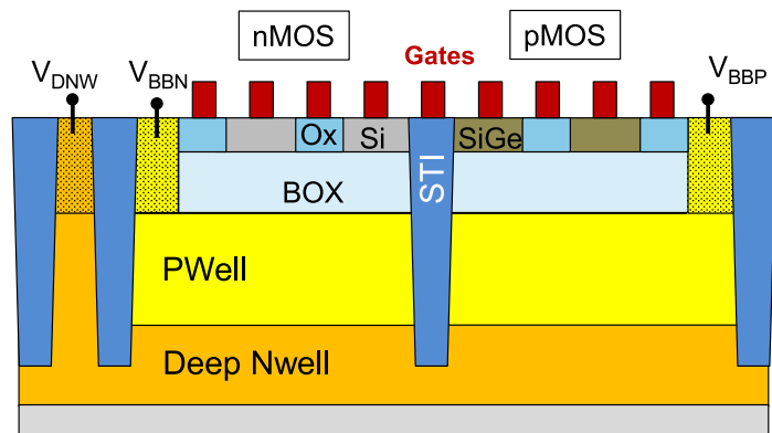
Figure 4.66: Cross-sectional scheme of the DITO integration enabling a full bidirectional back-bias (FBB and RBB). Deep trenches (STI) separate nMOS and pMOS back-planes while transistors of the same type are isolated with local oxidation.
