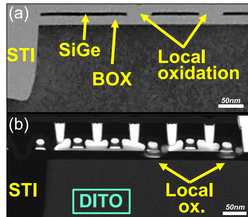
Figure 4.49: DITO TEM images (a) after the local oxidation module and (b) at the end of the process flow. In a "Single-Diffusion-Break" layout, a dummy gate is located above the local oxidation, as illustrated in the top-view of Figure 4.47.
