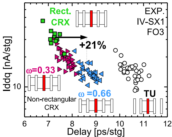
Figure 4.21: Delay/Leakage trade-off of 1-finger inverters with different RX-jog ratios. The higher the RX-jog ratio, the more the performance is degraded. This is due to the partial stress relaxation.
