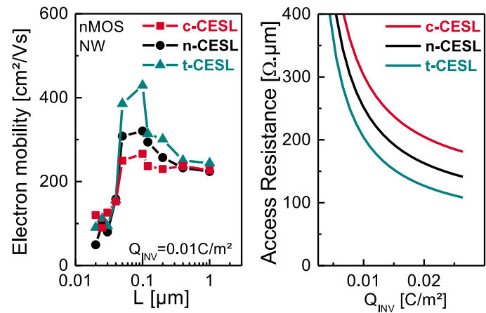
Figure 2.23: (left) Extracted electron mobility for \Omega -gate nMOSFET nanowires according to the gate length. (right) Extracted access resistance as a function of the inversion charge for the same devices. As for mobility, the CESL stress impacts the access resistance. A tensile-CESL (compressive CESL) is beneficial (detrimental, respectively).
