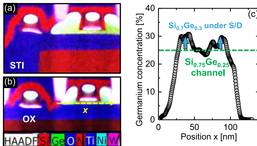
Figure 4.50: EDX mapping of a device close to (a) an STI isolation and (b) a local oxidation. (c) scan of Germanium concentration for a device located between two local oxidations. The Germanium concentration is 25% in the channel and close to 30% in the source/drain region
