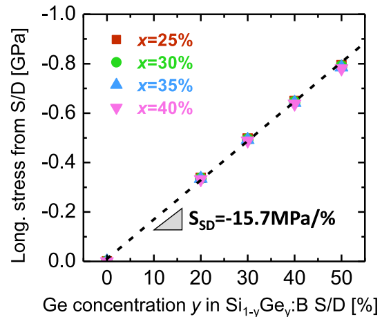
Figure 3.34: Simulated additional longitudinal stress from the source/drain only according to the Ge concentration in the source/drain and for different Ge concentrations in the channel. The additional stress related to the source/drain only depends on y_{Ge} , with sensitivity S_{SD} = -15.7\text{MPa}/\% , because the in-plane lattice parameter of the channel (i.e. substrate) is the one of Silicon, whatever its Germanium concentration. The simulation is for a non-patterned channel.
