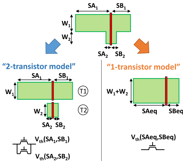
Figure 3.57: Illustration of the two approaches used to model the device built on a non-rectangular active area, i.e. with presence of a RX-jog. The so-called "2-transistor" model considers two transistors in parallel, each one with its own gate-to-STI distances SA and SB. The "1-transistor" model assumes equivalent gate-to-STI distances SAeq and SBeq (see equation 3.43).
