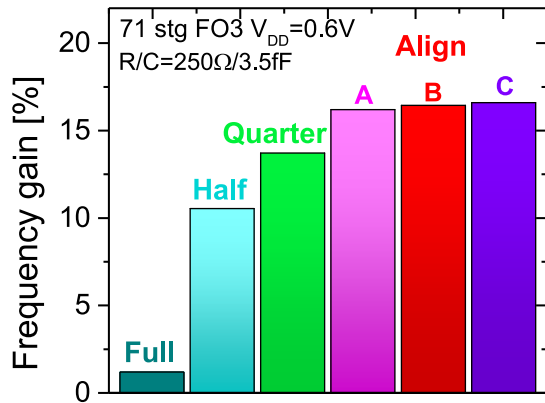
Figure 5.47: Frequency gain of the different inverter layouts vs. the Ref. The conditions of reference are V_{DD}=0.6V , fan-out 3, back-end network RC network with R_w=250\Omega and wire capacitance C_w=3.5fF . Frequency in double-gate mode can be improved by up to +16% for the optimized "Align" layouts.
