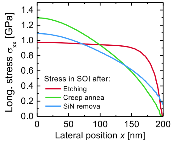
Figure 5.15: Stress profiles for the different BOX-creep process steps, extracted from Figure 5.12. After SiN removal, tensile stress is maintained in the SOI layer ( \sigma_{xx} = 1.1\text{GPa} in the middle, i.e. at x=0 ).
