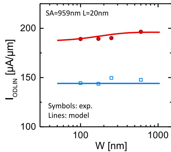
Figure 5.3: I_{ODLIN} current as a function of the active width for both SOI and sSOI SA=959 nm L=20 nm nFET devices. The sSOI I_{ODLIN} slightly varies with W . Even though the transverse stress is partially relaxed for narrow active, \langle 110 \rangle -oriented channel electron mobility is not sensitive to the transverse stress.
