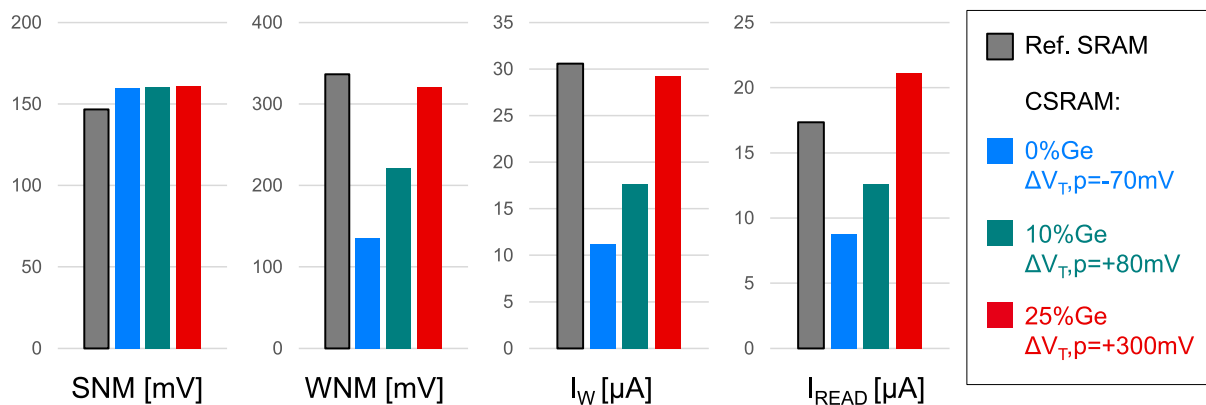
Figure 4.33: Reference SRAM and CSRAM metrics at V_{\text{DD}}=0.8\text{V} , benchmarked at same leakage obtained by an additional V_{\text{T}} shift, given in the legend. CSRAM improves the read current without significantly altering the other parameters.
