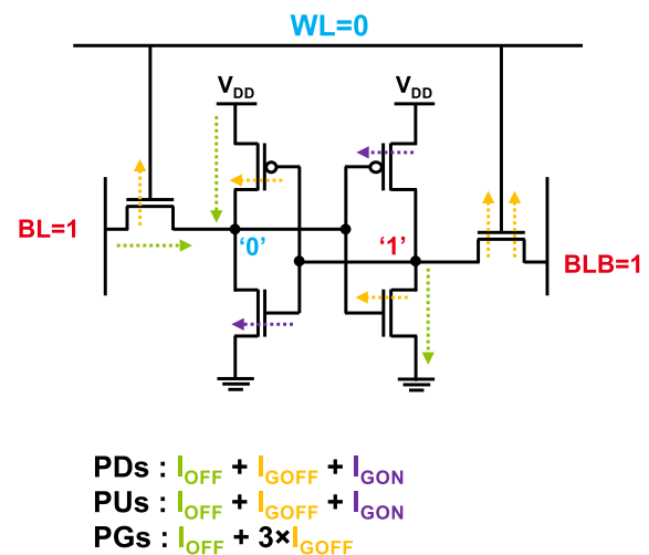
Figure B.8: SRAM leakage current extraction, measured when WL=0 and BL=BLB=1 . The stand-by leakage can be approximated from the leakage of each transistor of the bitcell.
