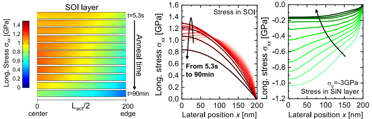
Figure 5.13: Simulated stress (left) mapping and (right) profiles during the BOX-creep annealing. From step to step, the anneal duration is multiplied by two. The compressive stress in SiN decreases and the tensile stress in SOI increases, due to the elastic energy transfer.
