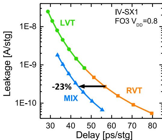
Figure 4.3: Simulated Leakage/Delay trade-off for a 1-finger inverter (IV-SX1) at V_{DD}=0.8V and for different flavors: LVT, RVT and MIX. The trend is obtained by simulating different V_T variations, equally to nFET and pFET. A -23% delay reduction at the same leakage is observed with the MIX flavor compared to RVT.
