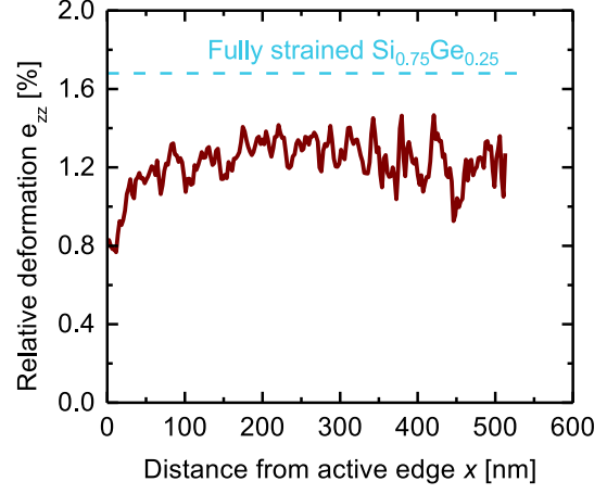
Figure 3.9: SiGeOI active area relative deformation e_{zz} profile after etching measured by NBED. The measured value is lower than expected for a pseudomorphic Si_{0.75}Ge_{0.25} (see the dashed line). This is attributed to the thin lamella effect, enabling relaxation in the y transverse direction.
