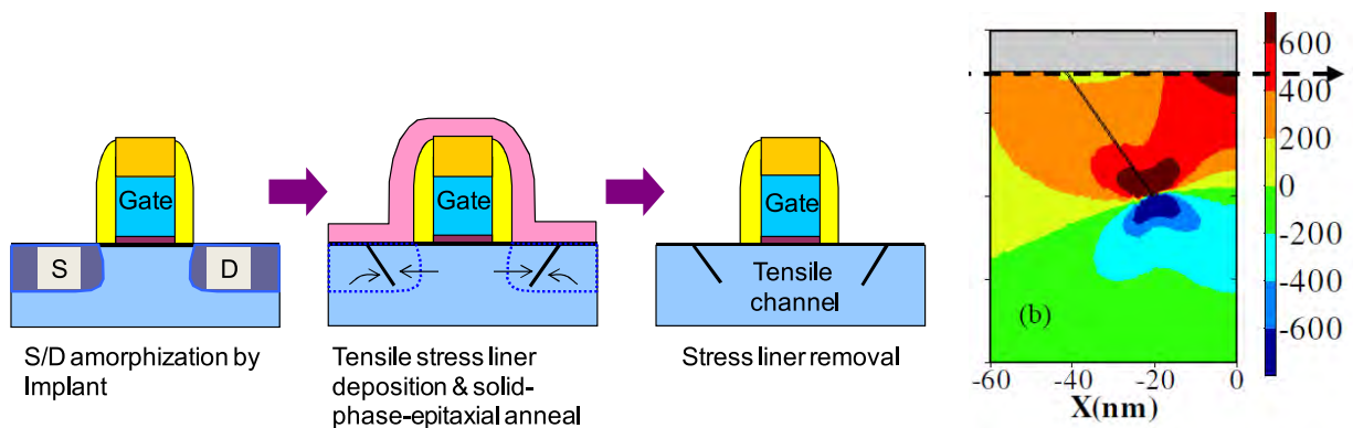
Figure 1.42: Principle of the Stress Memorization Technique (SMT), from [Lim10]. The SMT generates a tensile stress from the edge dislocation induced by Solid Phase Epitaxial Regrowth (SPER), as shown in Figure 1.43.
