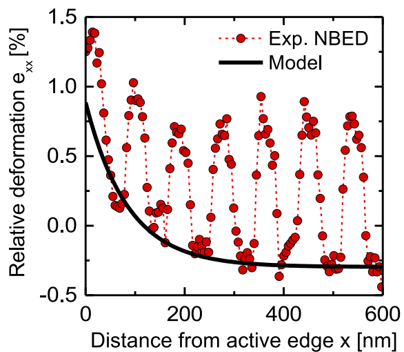
Figure 3.39: NBED and model relative deformation with source/drain stress taken into account. The model well reproduces the experimental data in the channels, i.e. under the gates (which are the region of interest for electrical behavior of the device). The typical relaxation length is \lambda = 84\text{nm} (the same as for the relaxation without source/drain of Figure 3.18).
