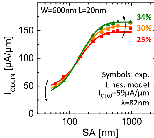
Figure 3.63: I_{ODLIN} vs. gate-to-STI SA (=SB) for W=600\text{nm} L=20\text{nm} pMOS with SiGe channels of different Germanium concentrations. The model represented by the lines well reproduces the experimental data assuming the same typical relaxation length. Especially, the crossover is explained by the stress configuration. For long active areas, the higher the Germanium content, the higher mobility due to beneficial uniaxial longitudinal strain configuration. For short active areas however, the main strain component is transverse, which is detrimental. Hence the higher mobility for lower Germanium content (i.e lower strain).
