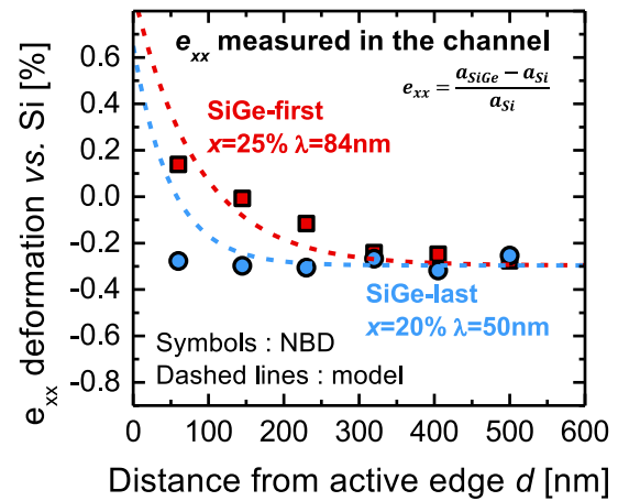
Figure 4.41: Deformation vs. Silicon reference e_{xx} measured by Nano-Beam Electron Diffraction (NBED) below the dummy gate and at the end of the process as a function of the distance from the active edge d . Higher strain relaxation for SiGe-first compared to SiGe-last is evidenced.
