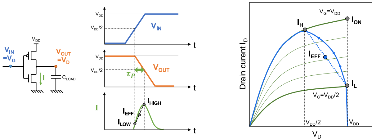
Figure 1.9: Illustration of the effective drive current in an inverter [Na02]. I_{EFF} is a DC approximation of the average drain current during the switching delay \tau_P (also called propagation delay).
