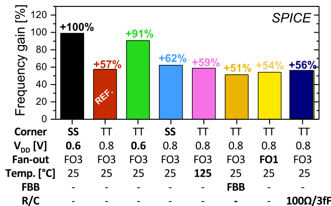
Figure 4.15: Simulated frequency gain expected by CRX design for various conditions. The major impact is V_{DD} reduction.
