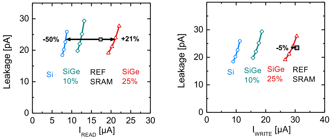
Figure 4.32: (left) Read current and (right) write current vs. cell leakage for different SRAM configurations at V_{\text{DD}}=0.8\text{V} . The \text{Si}_{0.75}\text{Ge}_{0.25} CSRAM read current outperforms the reference SRAM by 21% thanks to the higher hole mobility w.r.t. electron.
