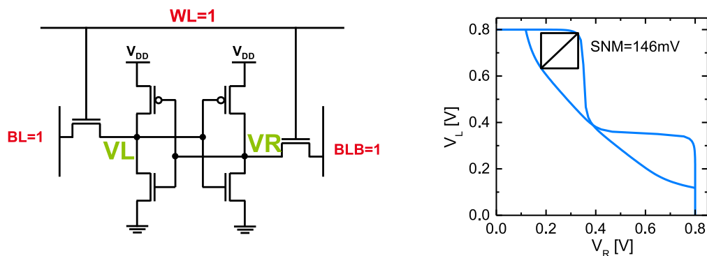
Figure B.4: (left) SRAM SNM extraction, consisting of two voltage transfer characteristics VR(VL) vs. VL(VR) while WL=BL=BLB=1. The SNM is given by the side of the smallest square embedded between the two curves in the so-called butterfly curve (right).
