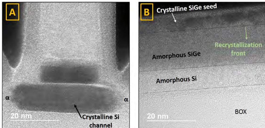
Figure 5.33: High resolution TEM after the SDRASS amorphization of the (A) channel region and (B) source/drain region. The channel is perfectly crystalline while the SOI in B region is amorphous after implantation. The top of the SiGe layer is crystalline and will act as a seed for recrystallization during the annealing.
