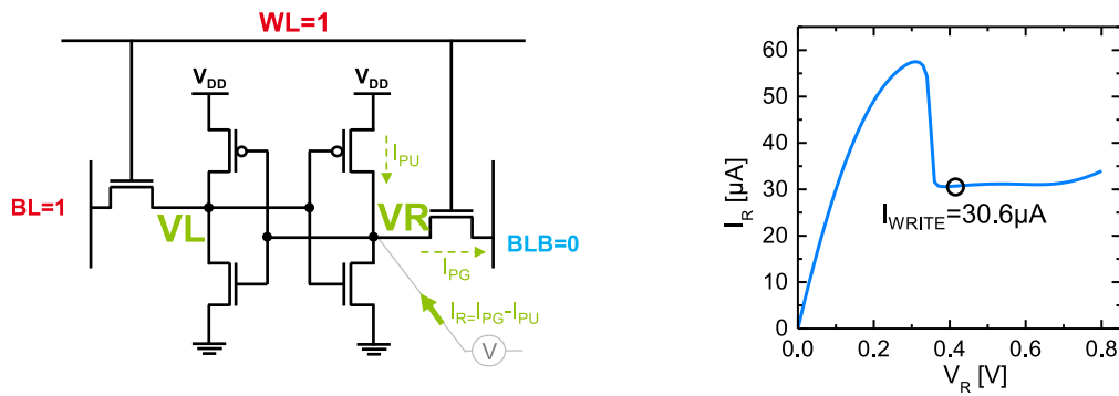
Figure B.6: (left) SRAM write current extraction, from sweeping the internal node voltage V_R and measuring the current externally sourced while WL=BL=1 and BLB=0 . The write current I_W is defined as the minimum current past the trip point of the inverter (right).
