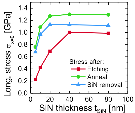
Figure 5.17: Impact of SiN thickness. Saturation of the final level of stress in the SOI. This is because a thick enough SiN totally relaxes and thus fully transfers its lattice deformation (i.e. strain) into the SOI.
