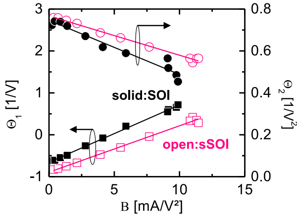
Figure 2.17: Extraction of parameters using \Theta_1(B) and \Theta_2(B) plots for both SOI and sSOI nMOSFETs. Extracted parameters of mobility and access resistance from linear regressions are presented in Table 2.2.
