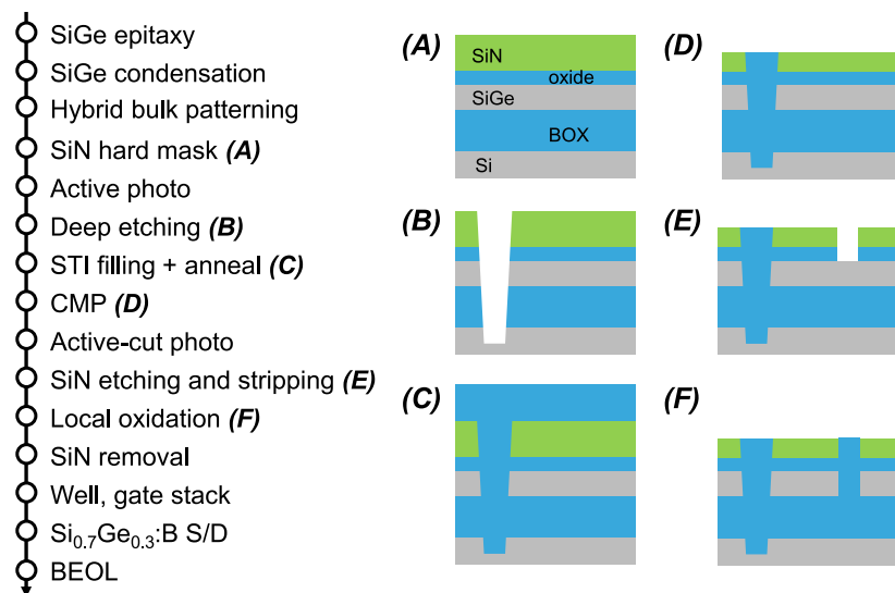
Figure 4.46: Process flow of DITO. The local oxidation is performed after the STI and CMP, reusing the SiN hardmask
