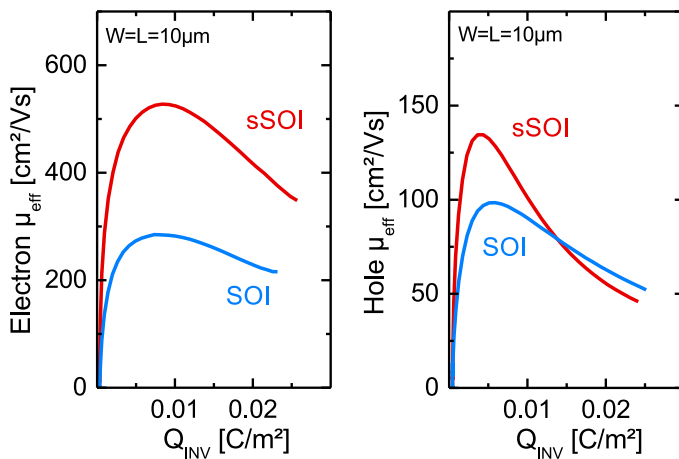
Figure 2.2: Effective (left) electron and (right) hole mobility extracted by split-CV on long channel devices built either on SOI or sSOI. The biaxial tensile strain improves the electron mobility. The hole mobility is enhanced at low inversion charge only.
