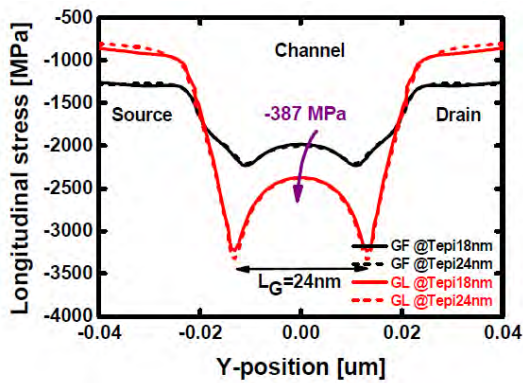
Figure 1.39: Stress profile for Gate-First and Gate-Last FDSOI technology embedding SiGe source/drain stressor, from [Idr15]. In Gate-First integration scheme, the gate holds the structure. The stress transfer is more efficient (-387MPa achieved) in a Gate-Last scheme thanks to the dummy gate removal.
