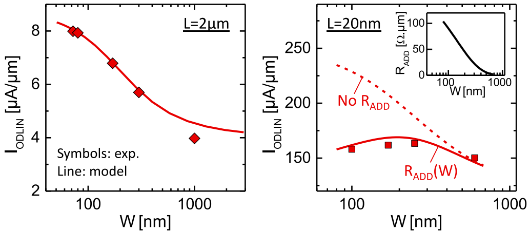
Figure 3.62: I_{ODLIN} vs. active width W for (left) long channel L=2\mu\text{m} and (right) short channel L=20\text{nm} . While the model considering transverse stress relaxation enables to well reproduce long channel I_{ODLIN} increase, it fails for short channel. This can be attributed to a higher access resistance for narrow devices (see inset). Such access resistance behavior could result from a faceted SiGe source/drain epitaxy (discussed in Figure 3.44).
