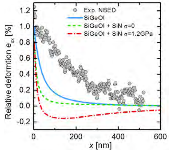
Figure 3.13: SiGeOI active area relative deformation e_{xx} profile after etching measured by NBED compared to elastic simulations considering different stacks. The strong relaxation observed experimentally is not consistent with simulations. Besides, the SiN hard mask should prevent the relaxation, especially if it is intrinsically tensely stressed.
