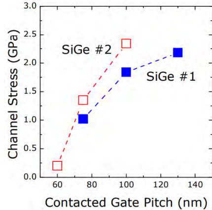
Figure 1.38: Stress generated by SiGe source/drain with respect to CPP (also called Contacted Gate Pitch CGP), from [Kha12]. As the volume of embedded SiGe diminishes, the strain transfer drops. Local stressors are less and less efficient as the CPP scales down.
