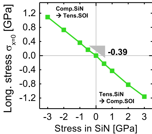
Figure 5.16: Simulated stress in the middle of the active area according to the initial stress in the SiN layer. Good proportionality is observed making BOX-creep technique suitable for both compressive and tensile stress generation in the SOI layer.
