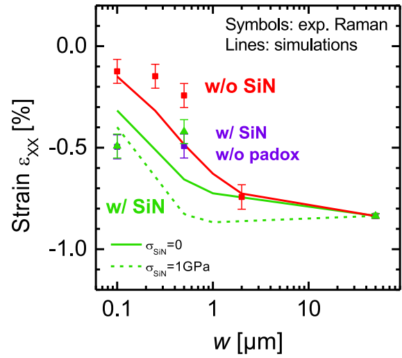
Figure 3.30: Extracted mean strain \varepsilon_{XX} according to the stripe width w for SiGeOI with and without SiN. The SiN layer enables to better maintain the compressive strain in the SiGe layer, especially for w=100\text{nm} . The lines correspond to FEM simulations assuming an unstressed (solid) and a 1GPa tensely stressed (dashed) SiN layer.
