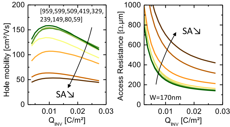
Figure 3.54: (left) Mobility and (right) access resistance vs. the inversion charge Q_{inv} for SiGeOI pMOSFETs of different L_{act} , extracted from linear regressions of Figure 3.53.
