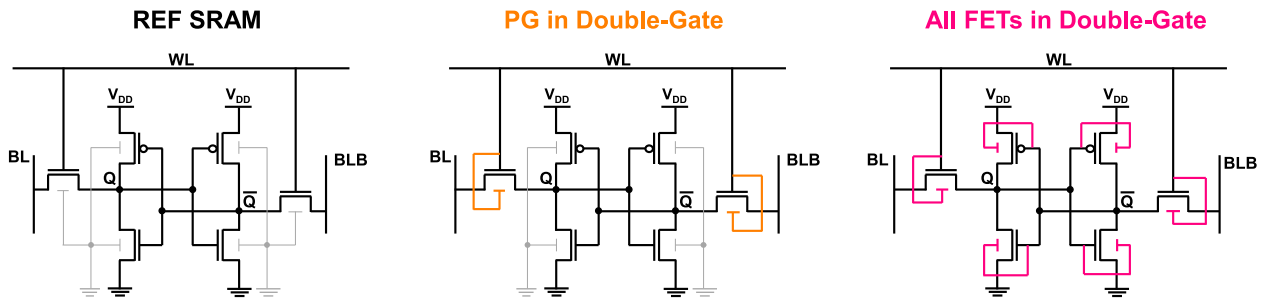
Figure 5.54: Schematics of the three 6T-SRAM configurations investigated. In the reference, back-bias for all FETs is grounded. Two cases of double-gate mode are assessed: only the Pass-Gate or all FETs in double-gate mode.
