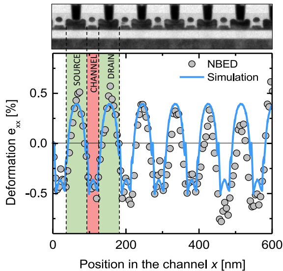
Figure 3.31: Relative deformation e_{xx} profile at the end of the process flow measured by NBED. The evidenced additional strain from SiGe source/drain is consistent with elastic simulations.
