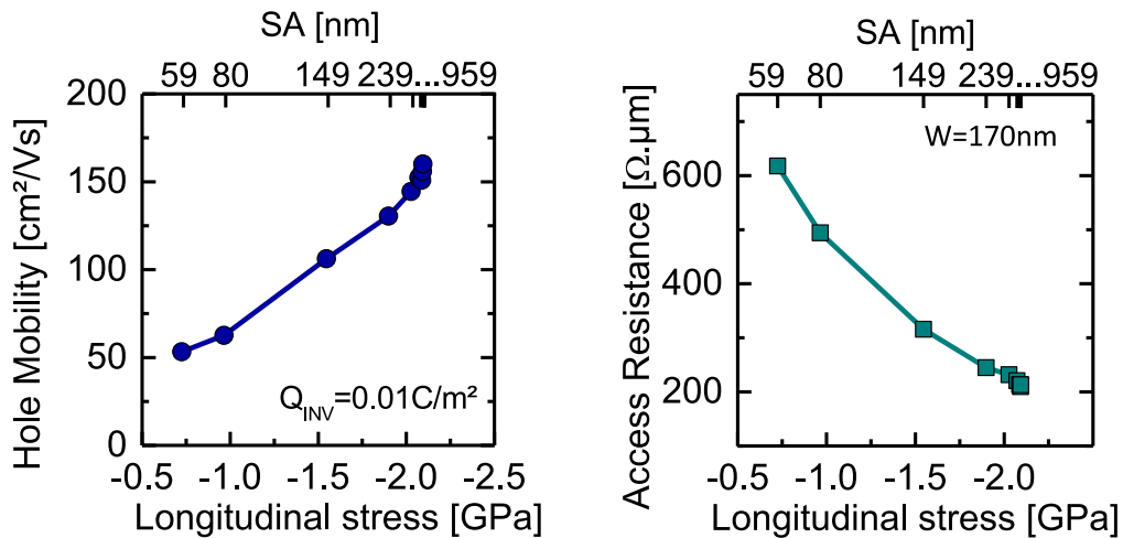
Figure 3.55: Extracted mobility and access resistance at Q_{inv} according to the longitudinal stress of each active length L_{act} . The value of stress is deduced from the relaxation model. The longitudinal stress impacts both the mobility and the access resistance. This result is consistent with Chapter 2.
