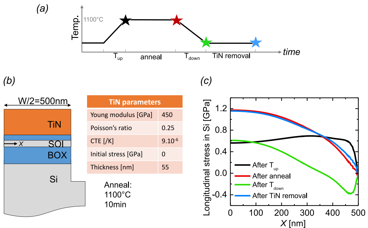
Figure 5.30: Principle of BOX-creep technique taking advantage of coefficient of thermal expansion mismatch. Mechanical simulation assuming TiN material. (a) Temperature along the different process steps (temperature ramp-up, anneal, temperature ramp down and TiN removal). (b) Mechanical simulation structure and parameters related to TiN (other parameters are the ones used in section 5.2.2). The TiN stress after deposition is considered null. (c) Longitudinal stress generated in the SOI along the different process steps. After TiN removal, tensile stress is expected.
