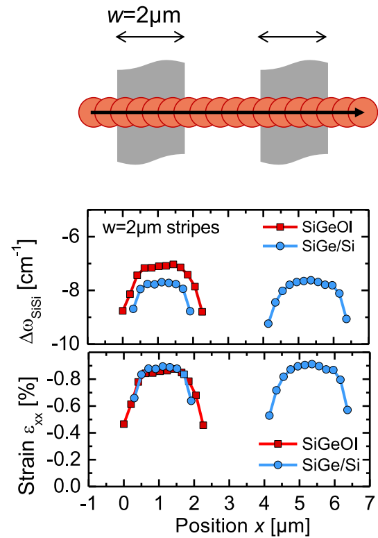
Figure 3.24: Raman scans perpendicular to the 2\mu\text{m} -wide stripes for both the SiGeOI and the bilayer samples. (top) Raman frequency shift and (bottom) extracted strain assuming relaxation in one direction. As for Figure 3.23, the \mu\text{Raman} resolution does not allow a precise measurement of the relaxation profile.
