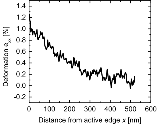
Figure 3.8: SiGeOI active area relative deformation e_{xx} profile after etching measured by NBED. The profile shows a progressive relaxation of the SiGeOI layer until it is fully strained at a distance of approximately 300nm from the edge.
