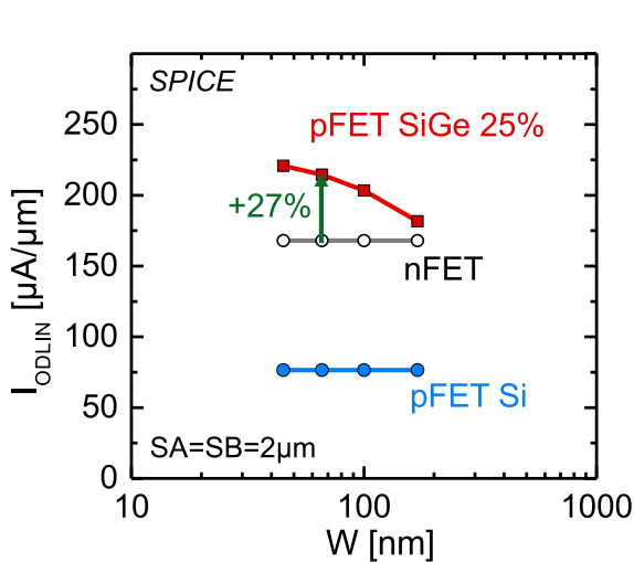
Figure 4.30: I_{ODLIN} vs. active with W from SPICE model at SA=SB=2\mu m and L=20nm . The introduction of SiGe leads higher hole mobility than electron, especially for short active area featuring the optimized longitudinal stress configuration. As a result, SiGe pFET I_{ODLIN} is expected to outperform nFET by +27% at W=66nm .
