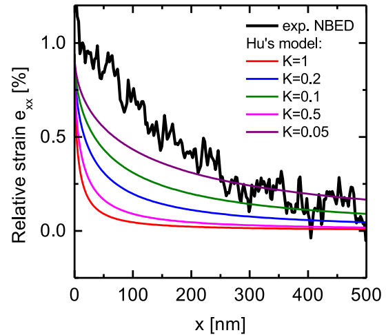
Figure 3.15: Hu's model compared to NBED profile of a patterned SiGeOI. A rigidity factor lower than K=0.05 (i.e. SiGe 20 times more rigid than the substrate) is needed to fit the experimental data. This reinforces the fact that the relaxation profile can not be explained by purely elastic models.
