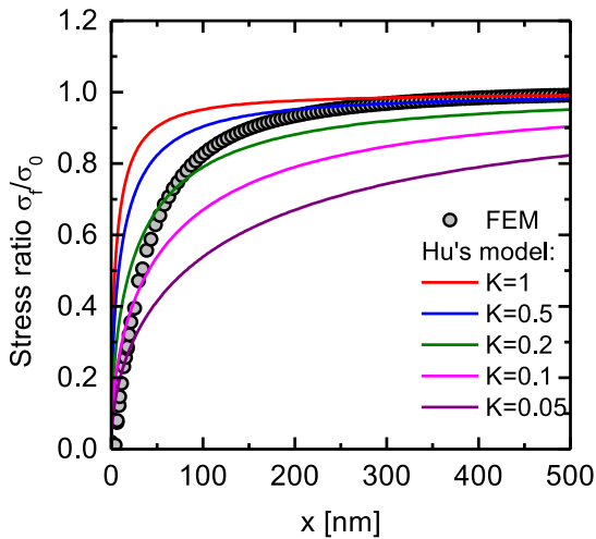
Figure 3.14: Hu's model compared to simulation of a patterned SiGeOI layer with deep trenches. The model does not perfectly reproduce the simulation because of both the impact of the BOX and the deep trenches etching (and not mesa).
