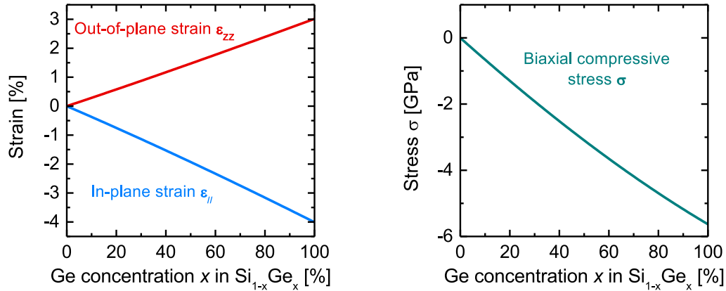
Figure 3.5: (left) In-plane and out-of-plane strains and (right) biaxial stress in pseudomorphic SiGe according to its Germanium concentration.
