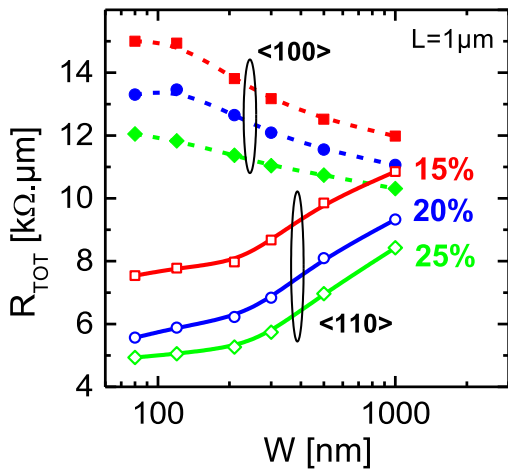
Figure 3.45: R_{TOT} vs. W for L=1\mu\text{m} \langle 100 \rangle and \langle 110 \rangle SiGe channel of different Germanium concentrations. The narrower the active, the higher the mobility for \langle 110 \rangle and the lower mobility for \langle 100 \rangle . This can be explained by the transverse stress relaxation. The transverse stress is detrimental for \langle 110 \rangle channel, hence the gain when this stress component is reduced. It is the opposite for \langle 100 \rangle channels.
