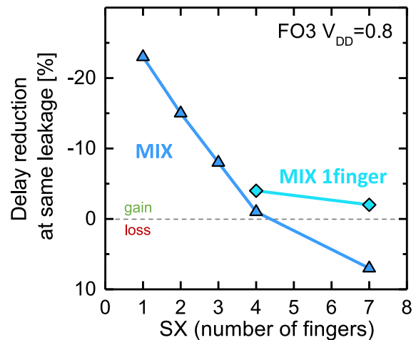
Figure 4.6: Delay gain at same leakage according to the inverter drive (SX, i.e. number of fingers). The higher drive, the lower gain because of longer active area. MIX flavor is even irrelevant for IV-SX7, degrading the delay by 7%. The MIX 1finger flavor (see Figure 4.7) improves the speed of IV-SX4 and IV-SX7.
