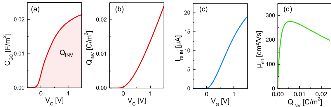
Figure 2.1: The CV-split technique. (a) C_{GC} vs. V_G . The integral gives the inversion charge Q_{INV} , shown in (b). (c) Linear drain current. (d) Extracted effective mobility \mu_{eff} vs. Q_{INV} .
