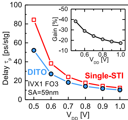
Figure 4.64: \tau_P vs. V_{DD} for ring-oscillators of 1-finger inverters. The lower the supply voltage, the higher the gain because DITO not only impacts the hole mobility but also allows to maintain a low pMOS V_T .
