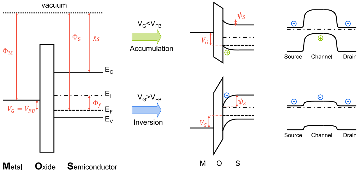
Figure 1.7: (left) Band diagram of the MOS structure under flat band condition. \phi_M and \phi_S are the metal and semiconductor work functions, respectively. \chi_S is the electron affinity. \phi_f is the Fermi potential. E_F is the Fermi level. E_i is the intrinsic Fermi level. E_C is the bottom of the conduction band and E_V the top of the valence band. (right) Band diagrams of a MOSFET in (top) accumulation or OFF state, i.e. no current from source to drain, and (bottom) inversion or ON state, i.e. carriers are free to flow from source to drain because of the reduced potential barrier.
