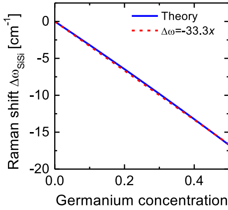
Figure 3.20: Raman frequency shift according to the Germanium concentration in a fully strained SiGe layer. Good approximation is given by \Delta\omega_{SiSi} = -33.3x_{Ge} for x_{Ge} below 0.5.
