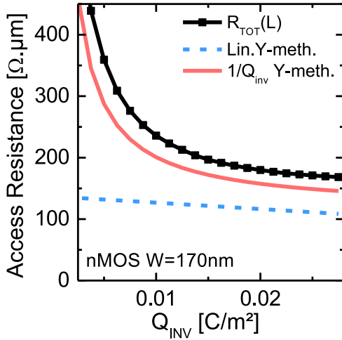
Figure 2.15: Extracted access resistance with respect to the inversion charge according to the method used. Our new methodology gives consistent result with the R_{TOT}(L) method without assuming a constant mobility.
