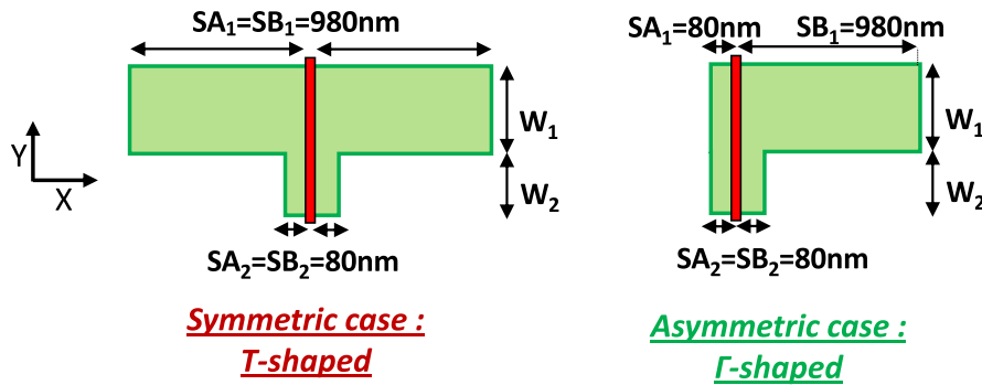
Figure 3.56: Scheme of non-rectangular layouts, i.e. with the presence of a least one RX-jog. Symmetric case (T-shaped) on the left and asymmetric case ( \Gamma -shaped) on the right.
