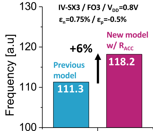
Figure 2.27: Three-finger inverter ring-oscillator frequency considering additional strains with respect to the previous planar FDSOI model ([Poi15], 14nm technology). The access resistance dependence with strain contributes to +6% frequency improvement.
