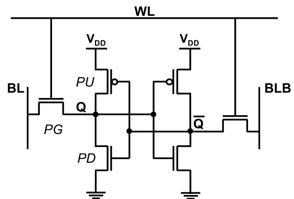
Figure B.1: SRAM bitcell schematic. The SRAM bitcell consists in two cross-coupled inverters, made of Pull-Up (PU) pFET and Pull-Down (PD) nFET transistors. The memory point is accessed by two Pass-Gate (PG) nFET transistors, both connected to the Word Line (WL) and to either the Bit Line (BL) or the second Bit Line (BLB).
