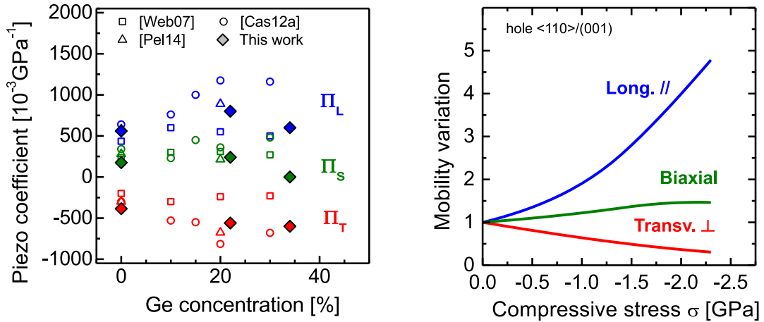
Figure 2.6: (left) Piezoresistive coefficients extracted on \langle 110 \rangle -oriented SiGe pFET according to the Germanium concentration. Results are compared with data from [Cas12a; Pel14; Web07]. (right) Hole mobility variation with compressive stress derived from equation 2.9. The longitudinal compressive stress is highly beneficial for hole mobility while the transverse stress is detrimental.
