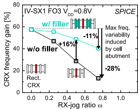
Figure 4.22: Simulated CRX frequency gain for IV-SX1 as a function of the RX-jog ratio showing the interest of a filler cell to limit the variability induced by standard cell abutment.
