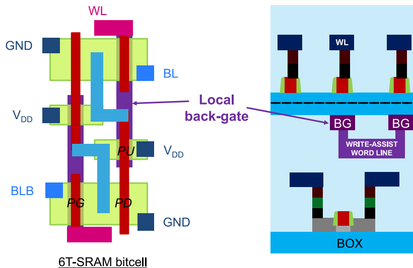
Figure 5.57: (left) Typical layout of an SRAM bitcell with the local back-gate layer in purple and (right) illustration of the 3D stack where the word line for write assist is embedded in an interlayer connection.
