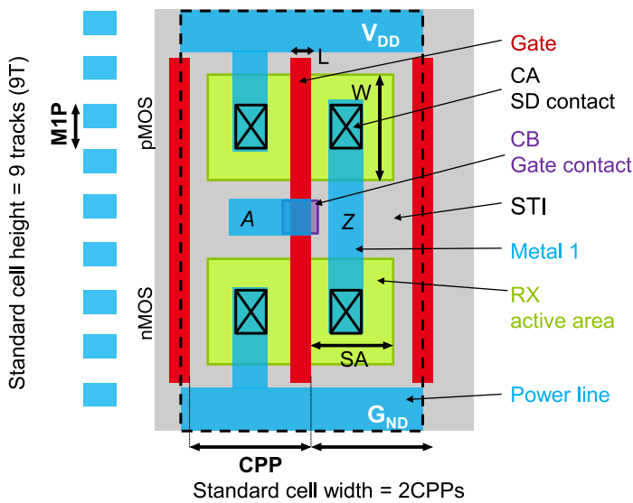
Figure 1.5: Layout of the 1-finger inverter standard cell. The pMOS and nMOS are designed between the two power rails. The standard cell height is expressed as a function of the number of Metal-1 pitches and its width is expressed as a function of the number of poly pitches (CPPs).
