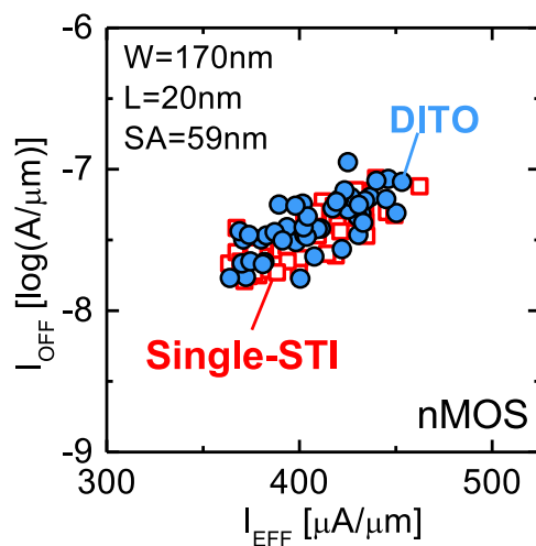
Figure 4.51: I_{\text{EFF}}/I_{\text{OFF}} trade-off for nFETs. Same results are obtained for single-STI and DITO.
