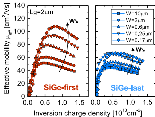
Figure 4.38: Hole effective mobility as a function of the inversion charge density for SiGe-first (left) and SiGe-last (right) for a long channel device ( L=2\mu\text{m} ) and for different channel widths W .
