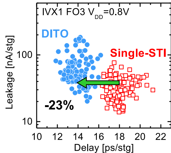
Figure 4.63: I_{\text{DDQ}}/\tau_P for ring-oscillators of 1-finger inverters. DITO leads to 23% delay reduction over single-STI at same leakage.
