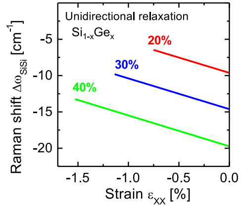
Figure 3.21: Raman frequency shift according to the level of strain in the X direction. The strain in the Y direction is assumed to be fully maintained since the SiGe stripes are considered infinite. The Raman frequency shift depends both on the level of strain in the X direction and on the Germanium concentration.
