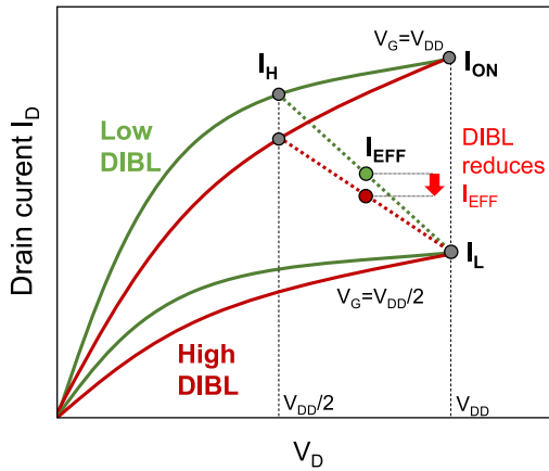
Figure 1.11: Illustration of the impact of the DIBL on the effective current I_{EFF} . A weak electrostatic control, i.e. high DIBL, is translated into I_{EFF} degradation (same leakage is considered).
