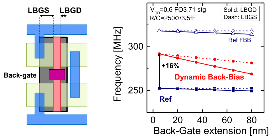
Figure 5.45: (left) Layout of the 1-finger inverter with local back-gate. Definition of the back-gate extensions over front-gate on the source and drain sides, LBGS and LBGD, respectively. (right) Frequency as a function of the back-gate extensions. Under static bias, the back-gate extension does not significantly impact the performance. Under dynamic back-bias however, LBGS and particularly LBGD reductions enhance the frequency.
