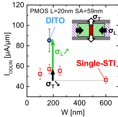
Figure 4.55: I_{ODLIN} vs. W evidencing the interest of DITO to optimize the strain configuration i.e. relaxing the transverse component while maintaining the longitudinal one.
