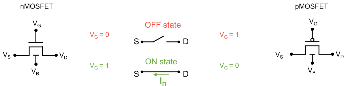
Figure 1.1: Schematic of the MOSFET, made of 4 terminals: Gate, Source, Drain and Body. The MOSFET is considered of a switch whose state ON or OFF is controlled by the gate voltage V_G . An nMOSFET (pMOSFET) is OFF if V_G = "0" ( V_G = "1" ) and turned ON if V_G = "1" ( V_G = "0" ), respectively. The n- and p-MOSFETs behave complementary, hence the name CMOS technology.
