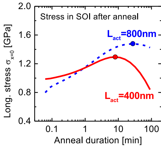
Figure 5.14: Stress in the middle of the active area according to the anneal duration. An optimal anneal duration is evidenced, which depends on the active length.
