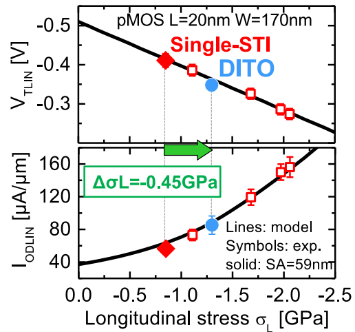
Figure 4.56: I_{ODLIN} and V_{TLIN} as a function of (left) SA and (right) the extracted stress from the model described in section 3.2.3. Both I_{ODLIN} and V_{TLIN} shifts at SA=59nm are consistent with an additional compressive stress of \Delta\sigma_L = -0.45 GPa.
