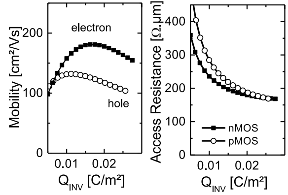
Figure 2.9: (left) \mu(Q_{INV}) and (right) R_{ACC}(Q_{INV}) for nMOS and pMOS, extracted from the R_{TOT}(L) plot of Figure 2.8. A strong access resistance dependence with inversion charge is evidenced.
