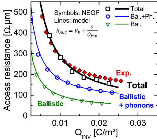
Figure 2.12: Comparison of the access resistance with respect to the inversion charge between a 3D NEGF simulation (black squares) and experiment (red diamonds) for a SiGe pMOS from 14nm FD-SOI technology. The ballistic component and the ballistic+phonon contributions to the access resistance are also plotted. The lines show the fit with equation 2.32.
