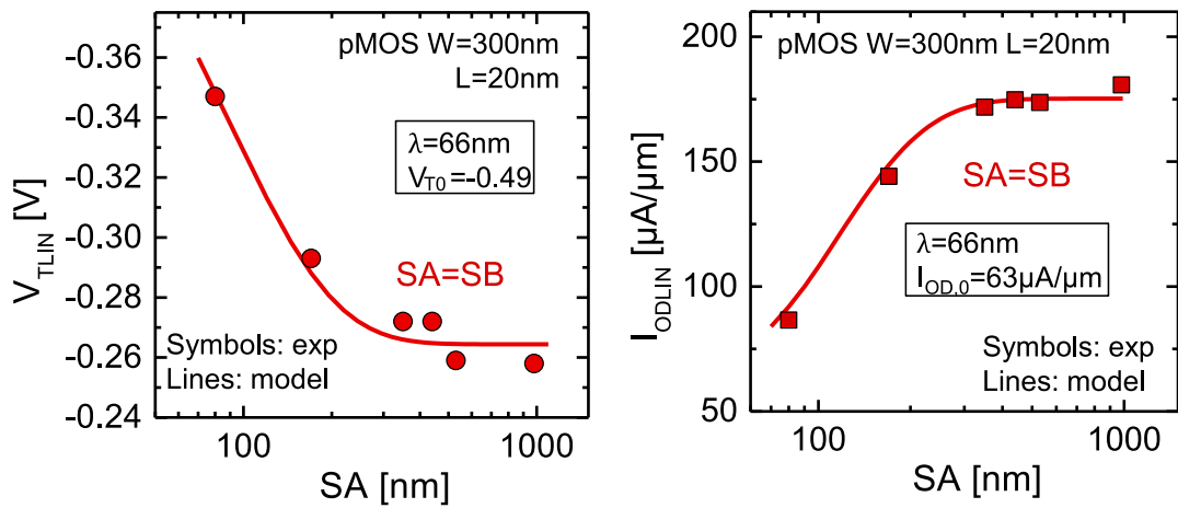
Figure 3.50: (left) V_{TLIN} and (right) I_{ODLIN} as a function of the gate-to-STI distance SA (=SB) for a W=300\text{nm} L=20\text{nm} pMOS device. The threshold voltage increases and I_{ODLIN} decreases for short active areas. This is due to a lower strain coming from the relaxation on the active edges. The model described in section 3.2.3 enables to reproduce the layout effect with a typical relaxation length \lambda=66\text{nm} . The used stress sensitivity is S_\sigma = 110\text{mV/GPa} .
