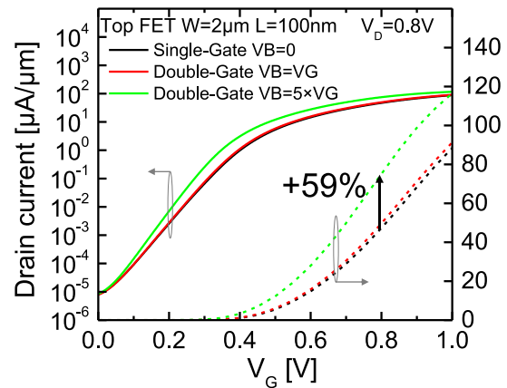
Figure 5.42: Top-tier nMOS I_D(V_G) in log. and linear scales in single- or double-gate modes. Because of the poor electrostatic coupling with the 100\text{nm} BOX, the double-gate mode V_B=V_G is closely similar to the single gate mode. In order to first-order emulate a 20\text{nm} -thick BOX, V_B=5\times V_G is applied, this time leading to +59\% I_{ON} over single gate mode.
