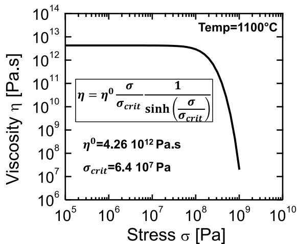
Figure 5.11: SiO 2 model of viscosity at T=1100°C used for BOX-creep simulations, based on a Garofalo's model [Eyr36; Gar65; Hu91] with parameters from [Sen96].
