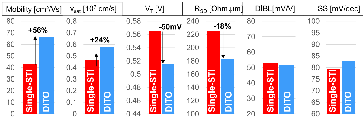
Figure 4.53: Extracted parameters from virtual source model [Kha09]. DITO leads to +56% mobility, +24% saturation velocity, -50mV threshold voltage and -18% access resistance. Similar DIBL and subthreshold swing obtained with DITO, highlighting no impact on electrostatics.
