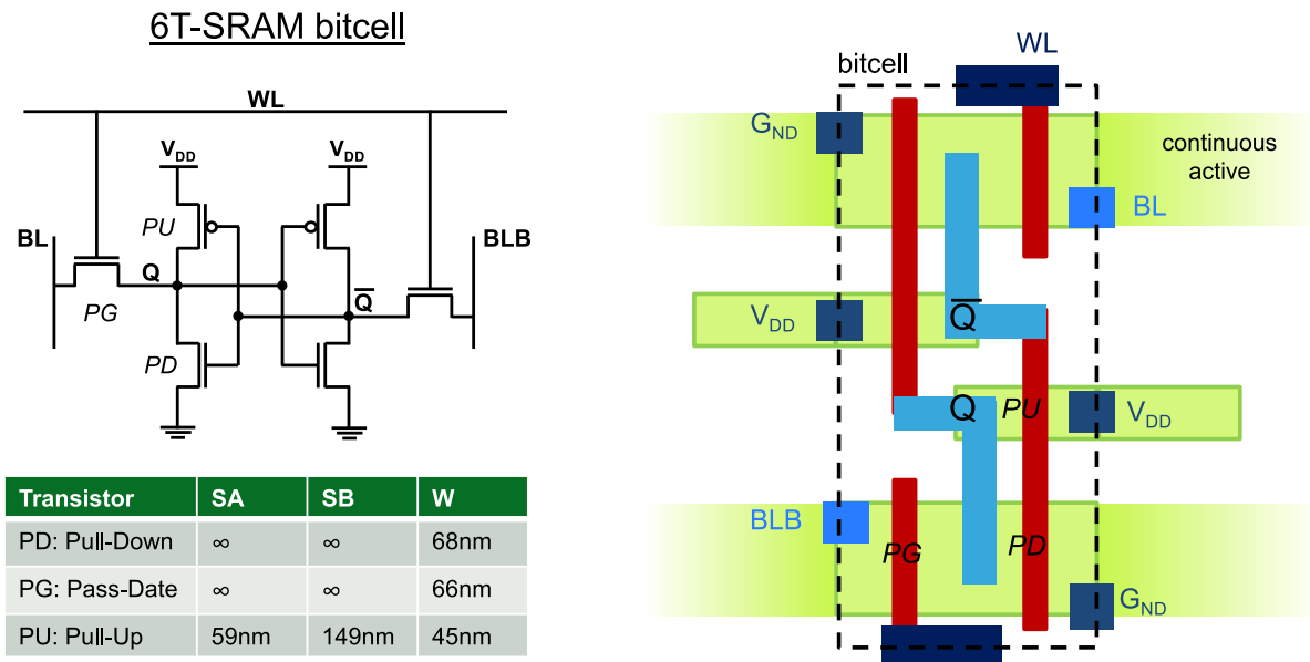
Figure 4.26: 6T-SRAM (left) schematic and (right) typical layout. An SRAM cell consists in two cross-coupled inverters made of Pull-Down (PD) and Pull-Up (PU) and two access transistors, also called Pass-Gate (PG).
