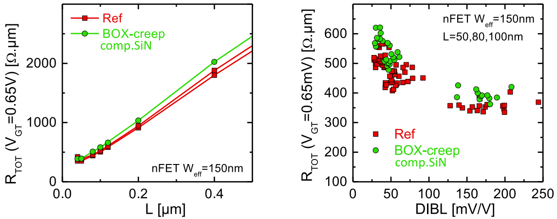
Figure 5.27: R_{TOT} vs. (left) gate length L and (right) DIBL for nFET with BOX-creep (15min anneal at 1100^\circ\text{C} with PECVD SiN \sigma_0 \approx -3\text{GPa} ) compared to the reference, i.e. without anneal (two wafers). While the electrostatic control is not impacted by the BOX-creep, the total resistance is degraded. This result is not consistent with a tensile stress generation into the SOI.
