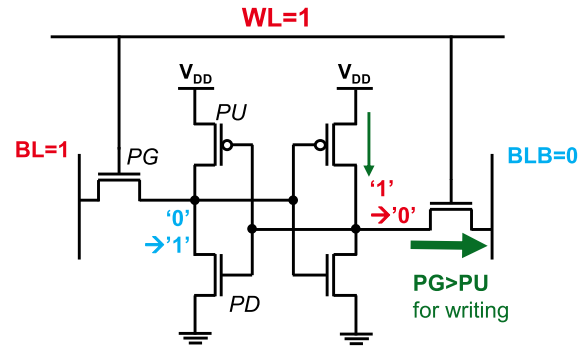
Figure B.3: SRAM writing operation. The bit flip is not possible where the internal node is at '0' (on the left side in this example) because of the read criterion PD>PG , discussed in Figure B.2. The writing operation imposes the PG>PU criterion, allowing the '1' to be flipped to '0'.
