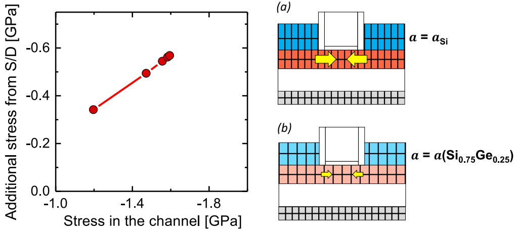
Figure 3.38: Simulated additional stress induced by the source/drain vs. stress in the channel after etching. Because of the \text{Si}_{0.75}\text{Ge}_{0.25}\text{OI} channel stress relaxation after patterning, \text{Si}_{0.7}\text{Ge}_{0.3} source/drain are grown on a substrate with a larger lattice parameter than Si. As a result, the lower the stress in the channel, the lower the additional stress from source/drain, as illustrated on the right.
