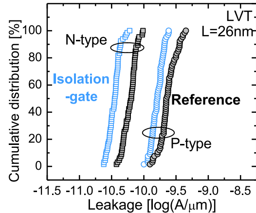
Figure 4.12: Cumulative distribution of the isolation-gate OFF-state leakage compared to reference.
