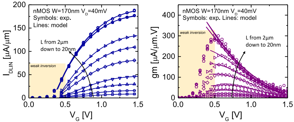
Figure 2.11: (left) I_D(V_G) and (right) g_m(V_G) experimental data fitted with Y-function method for nMOS of various gate lengths. The model well reproduces the experimental data in strong inversion regime.
