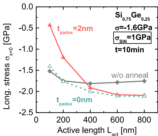
Figure 5.20: Simulated stress in the middle of the SiGe active area after BOX-creep with initially tensely stressed SiN layer. Without pad oxide, BOX-creep results in a slight increase of compressive stress in SiGe. With a pad oxide however, BOX-creep is detrimental as it allows the SiGe layer to relax. This is because the pad oxide creeping prevents the strain from SiN to be transferred.
