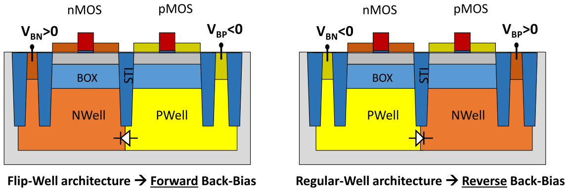
Figure 3.3: Illustration of Flip-well and Regular-well architectures. Flip-well architecture allows Forward-Back-Bias (FBB) while Regular-well allows Reverse-Back-Bias (RBB) because of the PN junction.
