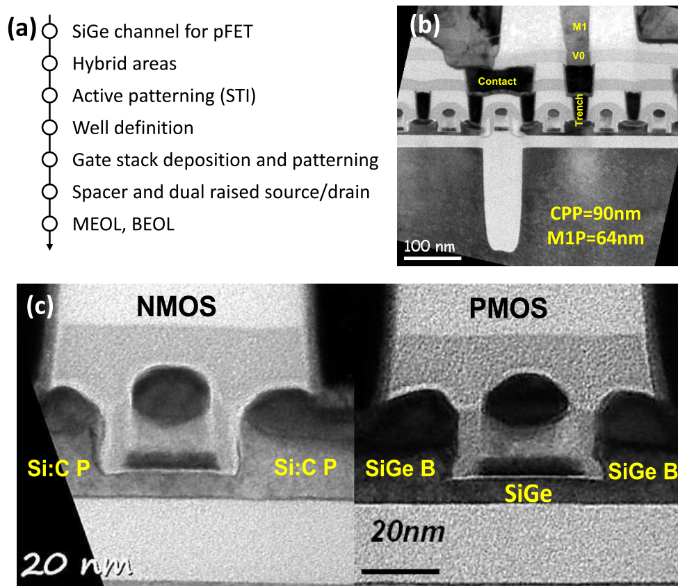
Figure 3.2: (a) Simplified process flow of 14nm FDSOI technology. SiGe channel integration for pFET is performed prior to the definition of active areas. Junctions made of dual raised source/drain are fabricated after the gate, i.e. gate-first scheme. (b) TEM image at the end of the process flow showing MEOL interconnections. Contacted Poly Pitch is 90nm and first level of metal M1 pitch is 64nm. (c) Focus on nFET and pFET nominal devices, emphasizing the dual channel and dual raised in-situ doped source and drain.
