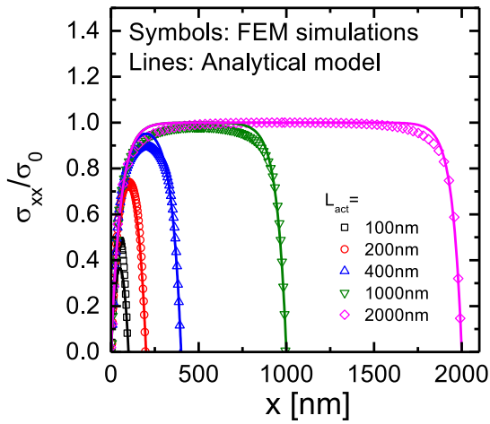
Figure 3.16: Normalized stress along patterned SiGeOI of various active lengths given by FEM simulations and compared to the analytical model of Equation 3.19 using \lambda = 54\text{nm} .
