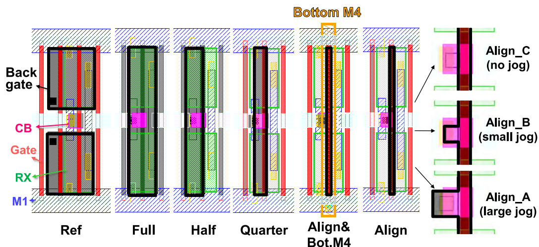
Figure 5.46: Different top level inverter layouts exploiting the double-gate mode vs. Ref, whose back-gate is at a given static bias (no back-bias, FBB or RBB). Optimization of the back-gate and shared contact shapes.
