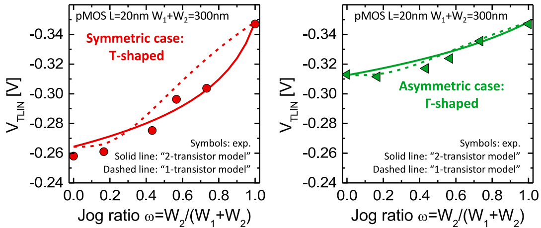
Figure 3.58: pMOS V_{TLIN} as a function of the jog ratio for two different cases of non-rectangular active area: symmetric (left) and asymmetric (right). Experimental data are well reproduced by the two different model approaches.
