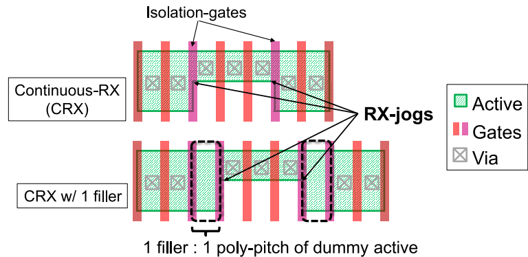
Figure 4.17: Layout of CRX in presence of RX-jogs, without and with a filler cell.
