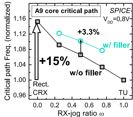
Figure 4.24: CRX frequency gain for a critical path of an A9 core according to the jog ratio (considered to be the same for each standard cell of the critical path). The relevance of a filler cell introduction is translated by +3.3% freq at \omega=0.5 .
