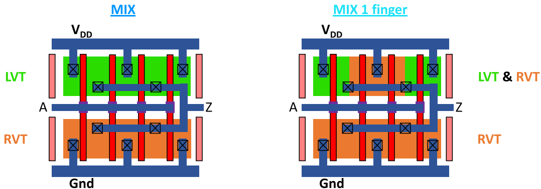
Figure 4.7: Illustration of the "MIX 1finger" flavor, consisting in changing the RVT pFET fingers close to the active edge to LVT. These fingers are the one the more impacted by the SiGeOI stress relaxation. This can be done by an implant mask for example.
