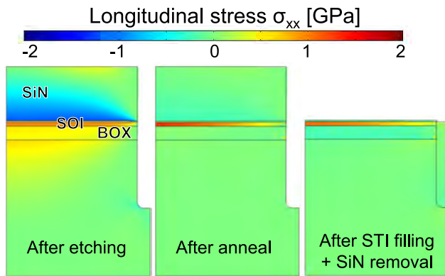
Figure 5.12: Simulated stress mapping along BOX-creep process steps. Using a compressive SiN leads to a tensile stress generated in the SOI layer. The stress is still present after SiN removal. The SiN layer is highly relaxed after anneal, hence the small impact of its removal on the SOI stress.
