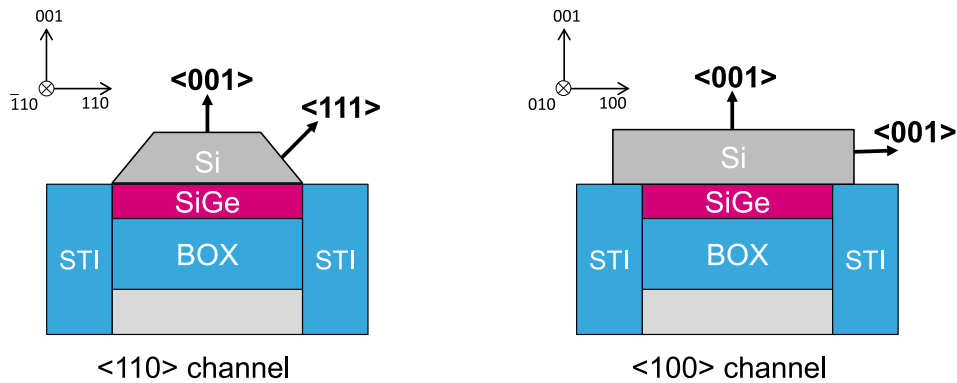
Figure 3.44: Illustration of different raised source/drain facets for \langle 100 \rangle and \langle 110 \rangle oriented channels. The cut is along W. The growth rate along the \langle 111 \rangle oriented crystallographic plan is slower than \langle 001 \rangle [Tun65]. This could lead to a degraded silicidation on the sides, responsible for a higher access resistance. The facets after SiGe epitaxy for \langle 110 \rangle oriented channels can be observed on a TEM image of devices fabricated at LETI in Figure 5.35.
