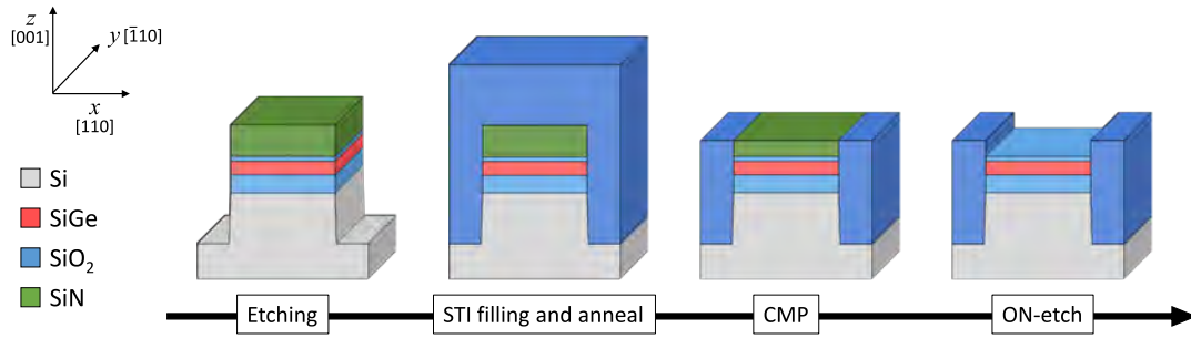
Figure 3.7: Illustration of the process steps of the STI module, defining the active area. Focus is made on pFET area with SiGe channel previously obtained by condensation technique.
