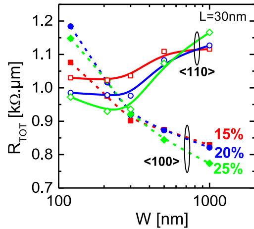
Figure 3.46: R_{TOT} vs. W for L=30\text{nm} \langle 100 \rangle and \langle 110 \rangle SiGe channel of different Germanium concentrations. As for long channels, the active narrowing is beneficial for \langle 110 \rangle channel while it is detrimental for \langle 100 \rangle channel. This can be explained by the transverse stress relaxation. For large W , \langle 110 \rangle orientation is degraded compared to \langle 100 \rangle , which is not the case for long channel. This change of behavior from long to short channel is attributed to a different access resistance (see Figure 3.44).
