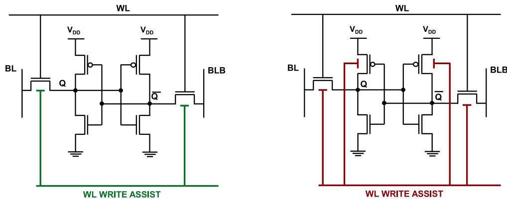
Figure 5.56: SRAM schematics with local back-gate connected to a second word line, dedicated to write-assist. Two configurations are presented. Either only the PG is connected to the write-assist word line or both the PG and the PU are connected.
