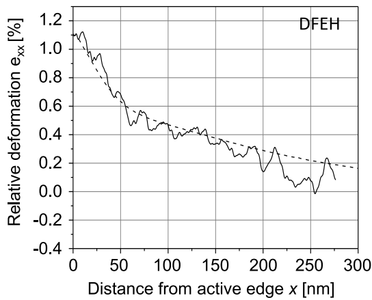
Figure 3.10: SiGeOI active area relative deformation e_{xx} profile measured by DFEH after etching. Courtesy of Victor Boureau [Bou16b].
