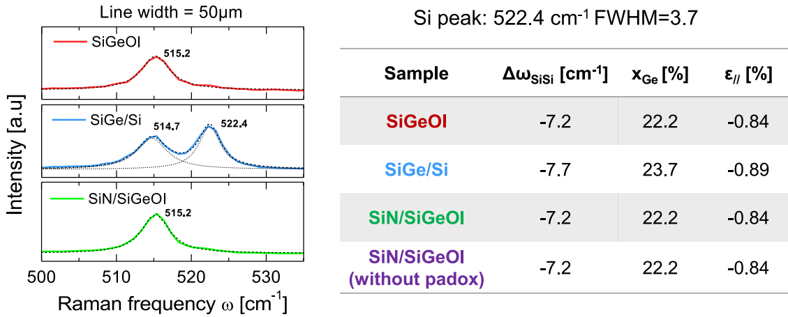
Figure 3.22: (left) Raman spectra for a wide SiGe stripe of w=50\mu\text{m} , equivalent to blanket wafer configuration. (right) Table summarizing the in-plane strain and associated Germanium concentration extracted from the Raman frequency shift \Delta\omega_{\text{SiSi}} with respect to the Si reference measured at \omega_0=522.4\text{cm}^{-1} with Full Width at Half Maximum of \text{FWHM}=3.7\text{cm}^{-1} .
