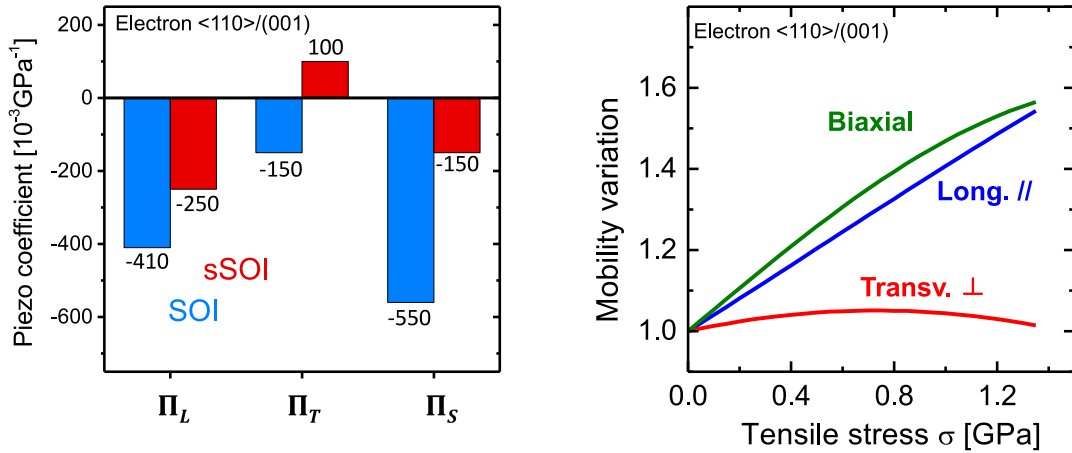
Figure 2.5: (left) \Pi_L , \Pi_T and \Pi_S piezoresistive coefficients extracted on \langle 110 \rangle -oriented nFET fabricated on SOI and sSOI. (right) Electron mobility variation with tensile stress derived from equation 2.9. The electron mobility enhancement under biaxial strain is mainly due to the longitudinal component.
