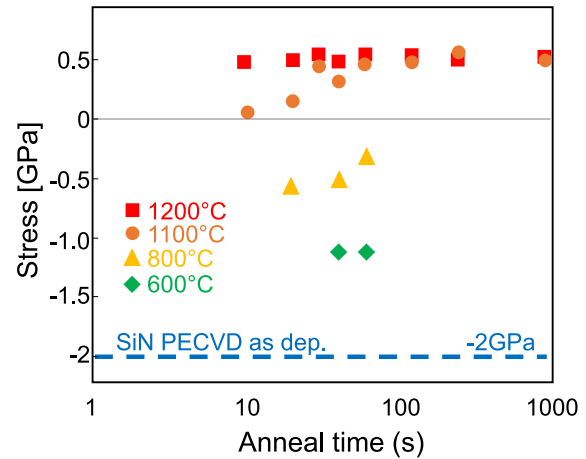
Figure 5.29: Evolution of PECVD SiN stress according to the anneal time, for different anneal temperatures, from [Bon16a]. The compressive stress obtained after deposition (-2GPa) rapidly decreases. After 10 seconds at 1100°C, the SiN is totally relaxed. For longer anneal, the SiN stress becomes tensile.
