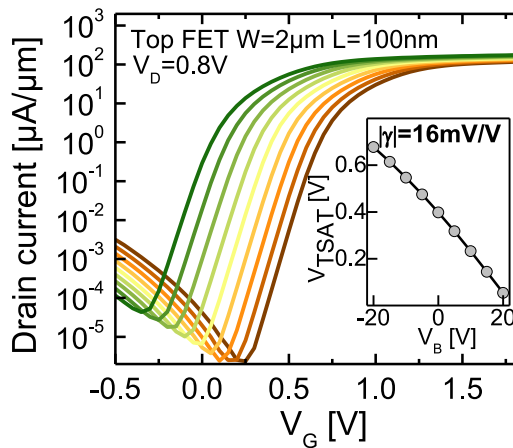
Figure 5.41: Top-tier nMOS transfer characteristics I_D(V_G) in saturation for different back-biases V_B ranging from -20\text{V} to +20\text{V} . Inset: V_{TSAT}(V_B) showing sensitivity \gamma=16\text{mV/V} . The back-bias V_B is applied on the gate of the bottom transistor (see Figure 5.40).
