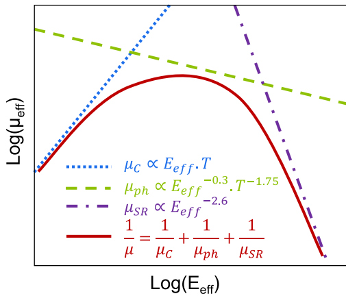
Figure 1.13: Illustration of the electron effective mobility dependence with the transverse electric field. The total mobility is derived from the three components (remote Coulomb, phonons, surface roughness) according to Matthiessen's law. The dependence with temperature and field is specific to each scattering mechanism [Che96; Tak94b].
