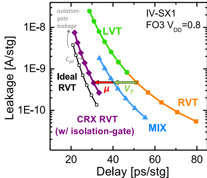
Figure 4.25: I_{ddq}/\tau_p trade-off of IV-SX1 at V_{DD}=0.8V simulated from SPICE for different design configurations. By re-balancing the V_T , the MIX approach yields a reduced delay with respect to reference RVT cell. The performance is however lower than the CRX approach because of the degraded mobility. The CRX performance is close to ideal. The increase of leakage is due to the isolation-gate and the performance loss is due to increased parasitic capacitance.
