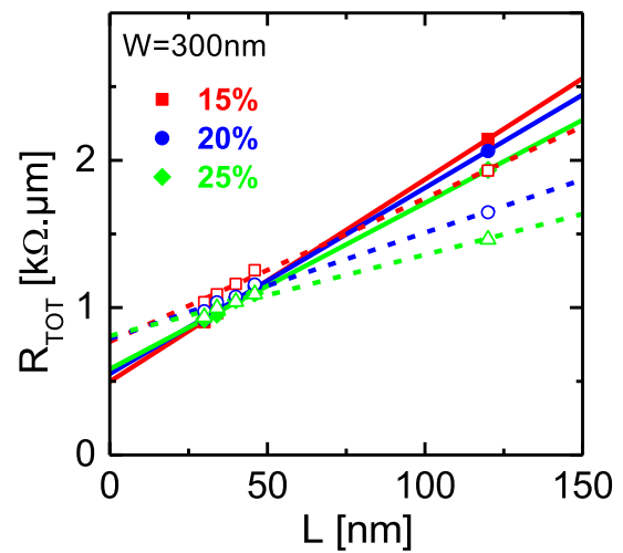
Figure 3.42: R_{TOT} vs. L for \langle 100 \rangle and \langle 110 \rangle SiGe channel pFETs of different Germanium concentrations. The slope and intercept give the \beta factor ( \beta = \frac{W}{L} \mu C_{ox} ) and access resistance R_{ACC} , respectively (see Chapter 2).
