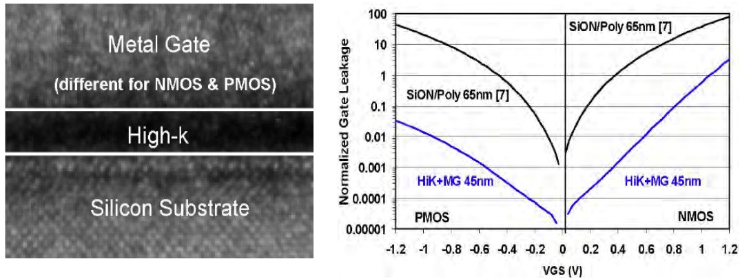
Figure 1.18: High- \kappa introduction at the 45nm node, from [Mis07]. (left) Gate stack with high- \kappa dielectric and metal gate. (right) Gate leakage reduction with high- \kappa introduction because of a thicker oxide at a constant capacitance.
