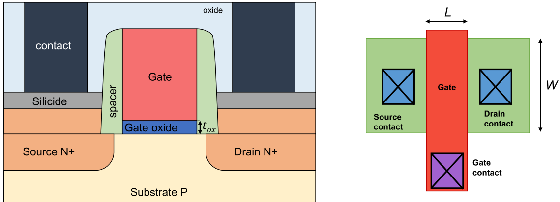
Figure 1.6: Illustration of typical MOSFET (left) cross-section and (right) top-view, i.e. layout.
