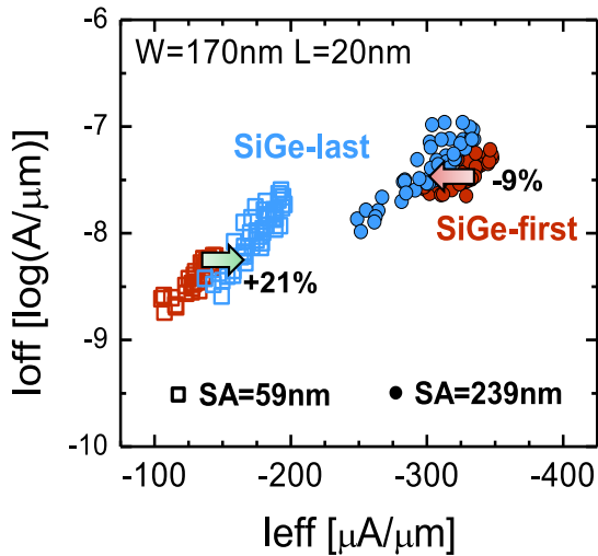
Figure 4.44: Experimental I_{\text{EFF}}/I_{\text{OFF}} trade-off demonstrating higher performance of SiGe-last for short active ( SA=59\text{nm} ) but lower perf. for long active ( SA=239\text{nm} ) regions at L=20\text{nm} gate length and W=170\text{nm} active width
