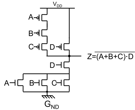
Figure 1.3: Schematic of the OR-AND-INVERT-31 (OAI-31) compound gate. The logic function is achieved by relevantly building the pull-down and pull-up networks. Transistors in series in the pull-up network are in parallel in the pull-down network and vice versa.
