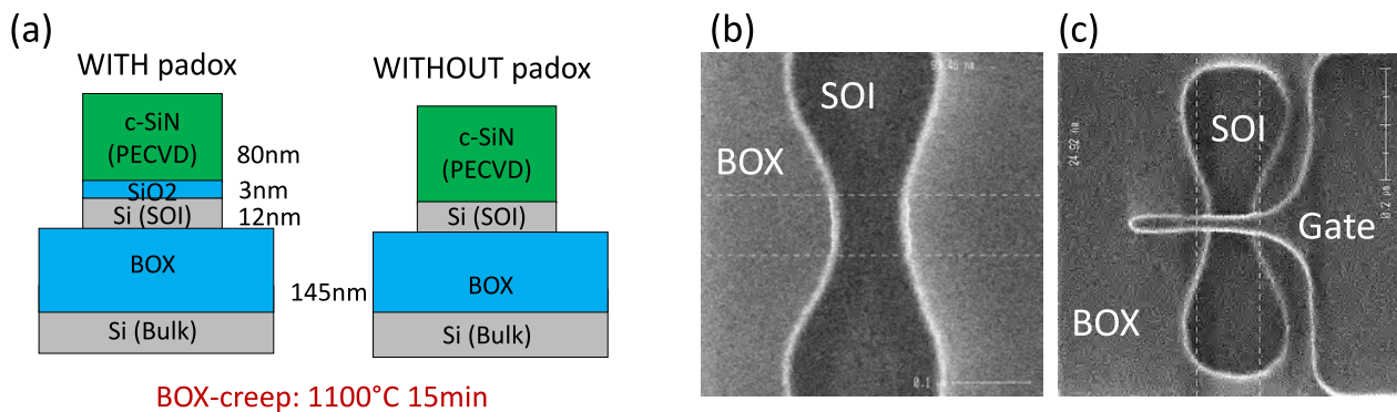
Figure 5.25: Presentation of BOX-creep technique integrated into LETI's device route. (a) Stack after active patterning for the two configurations with and without pad oxide. The etching is mesa (and not deep trenches as in STI). The buried oxide is 145nm thick. SEM top view after (b) SiN removal and (c) gate patterning.
