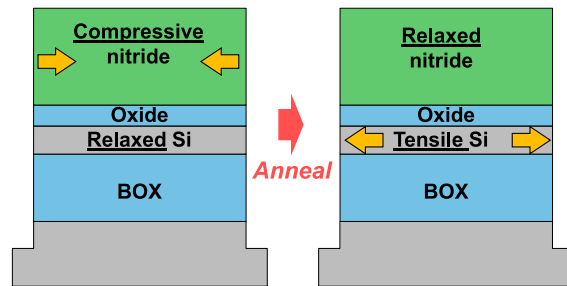
Figure 5.9: BOX-creep principle. Strain transfer from SiN layer into SOI by an anneal at high temperature. Low viscosity of SiO 2 allows the SiN to relax, dragging the underneath SOI. In this case, the use of a compressive SiN is translated into a tensile SOI after annealing.
