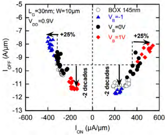
Figure 1.23: Impact of back-bias on FDSOI I_{ON}/I_{OFF} trade-off, from [And10]. The BOX thickness is 10nm. A positive (negative) back-bias on nMOS (pMOS, respectively) shifts the V_T toward low value, resulting in an increased ON current at the expense of high leakage. This is called Forward Back-Bias (FBB). It is the opposite for Reverse Back-Bias (RBB).
