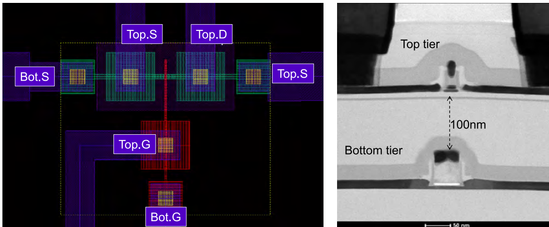
Figure 5.40: (left) Layout of the tested stacked devices. The poly-Si gate of the bottom transistor can be used as a back-gate electrode for the top level one. (right) TEM picture showing the two stacked transistors. The Inter-Layer Dielectric, also called BOX, is approximately 100nm-thick.
