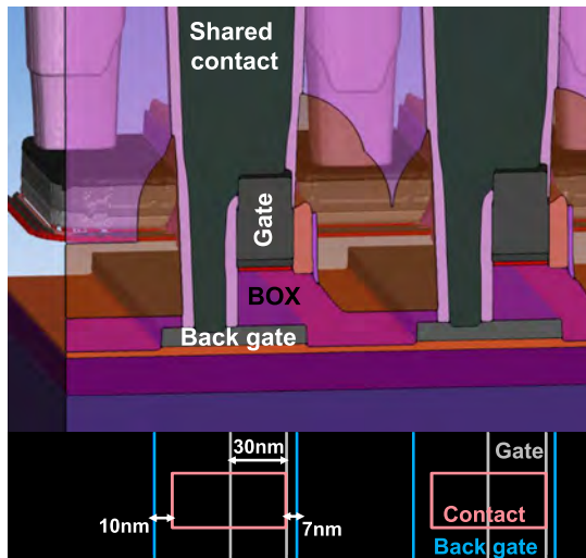
Figure 5.43: Coventor process simulation of the 3D shared contact between the front-gate and the local back-gate. Back-gate extension over the front-gate helps the realization of the shared contact. 28nm design rules are considered.
