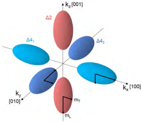
Figure 1.29: Iso-energy ellipsoids of the conduction band ( \Delta valleys). The \Delta_2 valleys correspond to the out-of-plane direction (i.e. the orientation of confinement) and \Delta_4 valleys correspond to the in-plane valleys. The transverse and longitudinal effective masses are represented.
