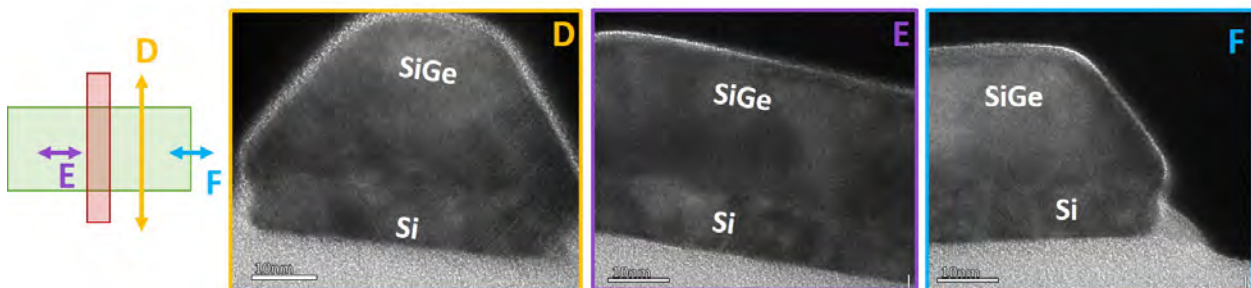
Figure 5.35: TEM after the SDRASS annealing in different source/drain regions. Cut D is transverse. After annealing, the SiGe/Si bilayer is crystalline with defects, especially in the Si layer.
