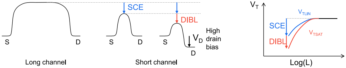
Figure 1.10: Top of the band schematic. The potential barrier is lowered for short channel (Short Channel Effect, SCE) and under a drain bias (Drain-Induced Barrier Lowering, DIBL).
