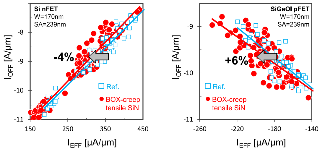
Figure 5.23: I_{EFF}/I_{OFF} trade-off for W=170\text{nm} SA=239\text{nm} (left) nFET and (right) pFET from 14nm FDSOI technology at V_{DD}=0.8\text{V} . The BOX-creep consists in an anneal at 1100^\circ\text{C} for 15min after active patterning. The SiN tensile stress is approximately 1.2GPa. The drive current of nFET is degraded by -4% at the same leakage, while the one of pFET is enhanced by 6%. This result is consistent with the generation of a compressive stress in the channel.
