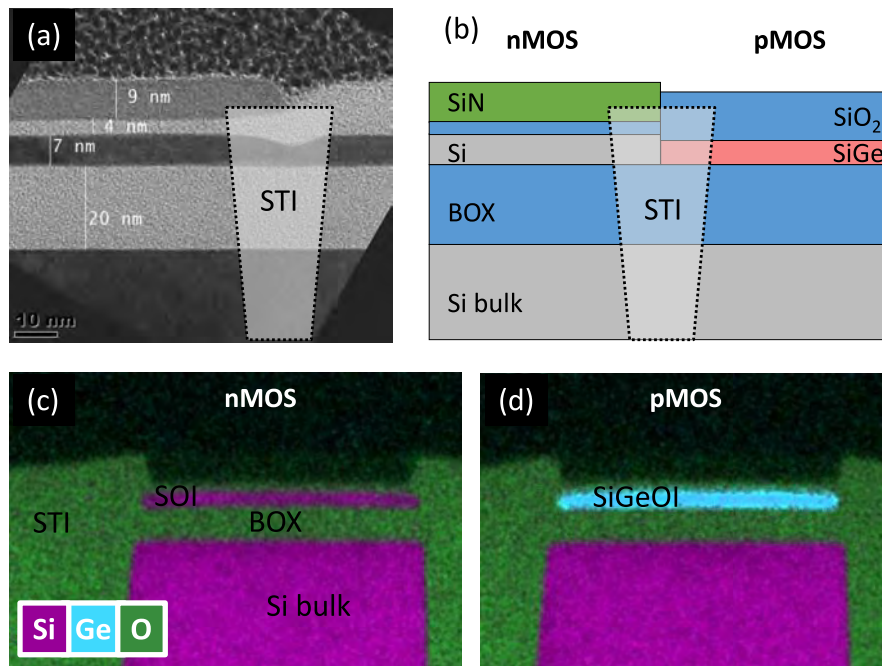
Figure 3.6: (a) TEM and (b) scheme of the SOI/SiGeOI border before STI fabrication. The nMOS area is protected by a SiN hard mask, allowing local introduction of SiGe by condensation. EDX mappings after STI in the (c) SOI and (d) SiGeOI regions.
