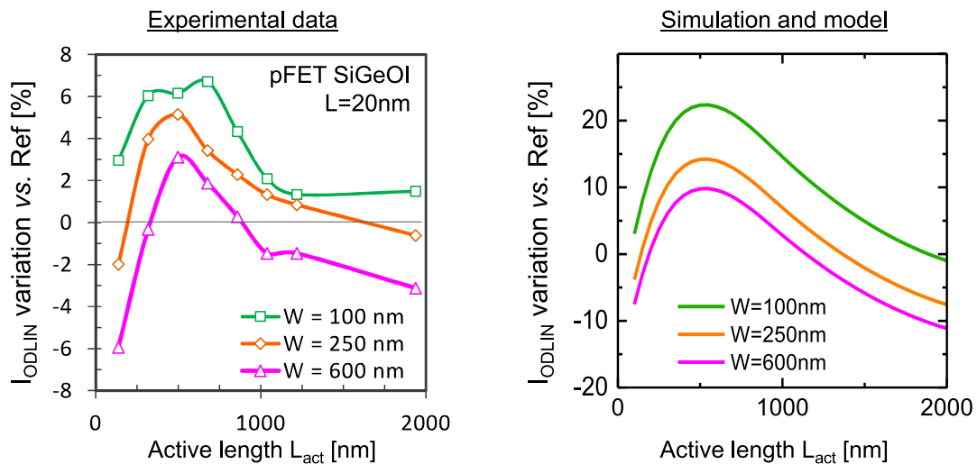
Figure 5.24: 14nm FDSOI BOX-creep pFET I_{ODLIN} variation w.r.t the reference according to the active length for different widths from (left) experimental measurements and (right) simulation and model. The highest gain is achieved for W=100\text{nm} and L_{act}\approx 500\text{nm} . The trend is qualitatively reproduced by the mechanical simulation and mobility model.
