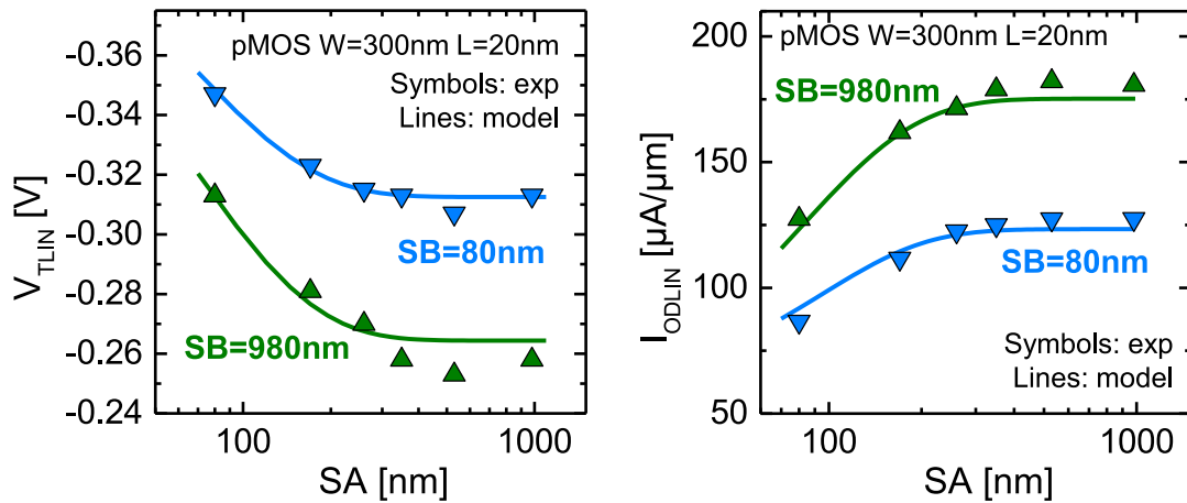
Figure 3.52: (left) V_{TLIN} and (right) I_{ODLIN} as a function of the gate-to-STI distance SA while SB value is fixed at either 980nm or 80nm for a W=300\text{nm} L=20\text{nm} pMOS device. The behavior is similar to the symmetric case of Figure 3.50, this time showing the impact of one edge proximity. The model parameters are the same as for Figure 3.50 (especially \lambda = 66\text{nm} ).
