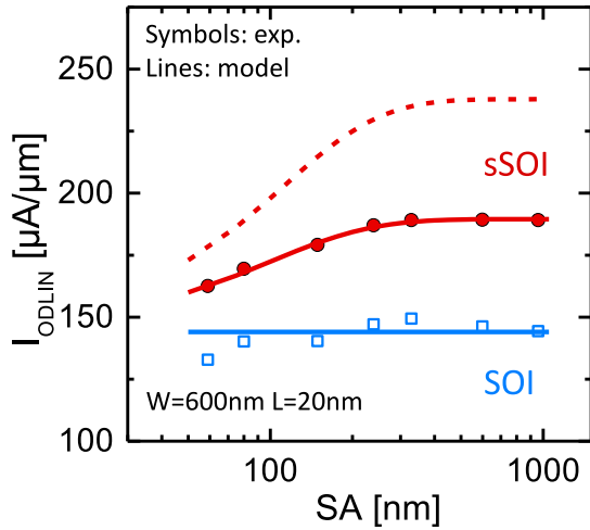
Figure 5.2: I_{ODLIN} current as a function of the gate-to-STI distance SA for both SOI and sSOI W=600 nm L=20 nm nFET devices. The sSOI I_{ODLIN} decrease for short active layout is attributed to the longitudinal stress relaxation. The model overestimates the gain (dashed line). In order to reproduce the experimental data, an access resistance of R_{ACC}=132 \Omega \cdot \mu m must be considered (solid line). The used typical relaxation length is \lambda=86 nm.
