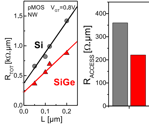
Figure 2.25: (left) R_{TOT}(L) at V_{GT}=0.8V for \Omega -gate pFET nanowires featuring Si or SiGe channel. (right) Extracted access resistance from the intercept of the linear regression. The access resistance is reduced by 39% from Si to SiGe channel.
