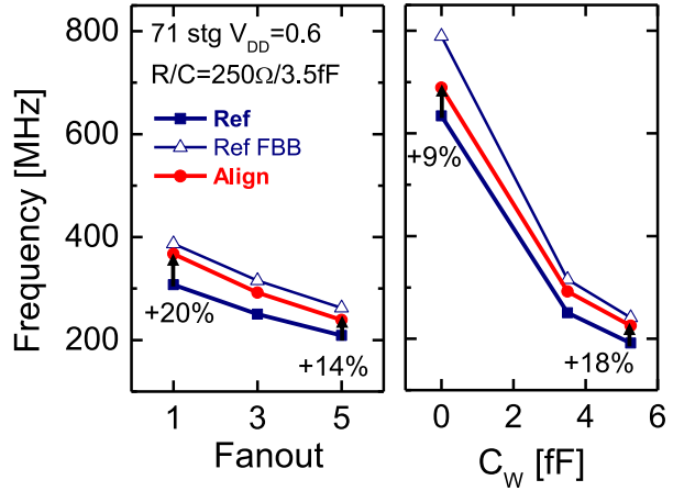
Figure 5.53: Frequency vs. (left) Fanout and (right) back-end wire capacitance C_w . The higher the fanout, the lower the gain with DBB because of the C_{EFF} degradation. The higher the back-end load, the higher frequency gain, thanks to the improved R_{EFF} .
