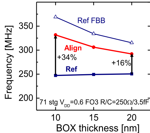
Figure 5.51: Frequency vs. top-tier BOX thickness for the "Align" layout (DBB) compared to the reference with or without FBB. The thinner the BOX, the higher the gain from Dynamic-Back-Bias, due to a better electrostatic coupling.
