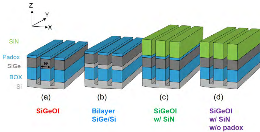
Figure 3.19: Sketches of the four different samples investigated: (a) the reference condensed SiGe directly on insulator, (b) The SiGe/Si bilayer case, i.e. without condensation, (c) reference SiGeOI before SiN hard mask removal, (d) same case as (c) but without pad oxide. The SiGe stripes of width w in the X direction [110] are 2mm long in the Y direction, which is long enough to be considered as infinite. The vertical direction Z is oriented along the [001] direction.
