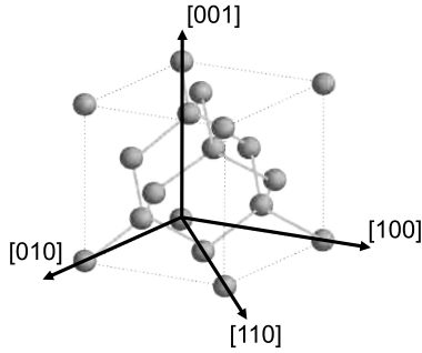
Figure 1.27: Lattice of Silicon. Silicon has a diamond cubic lattice structure.
