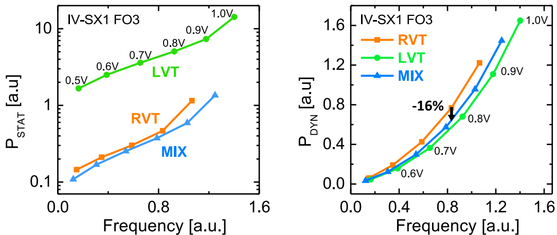
Figure 4.5: (left) P_{STAT} and (right) P_{DYN} vs. Frequency for RVT, LVT and dMIX flavors for different V_{DD} . The MIX flavor has similar P_{STAT} to RVT and achieves -16% dynamic consumption at same frequency.
