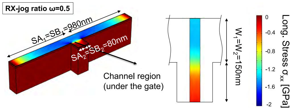
Figure 4.18: Mechanical simulation of an active area with RX-jog showing a partial stress relaxation.
