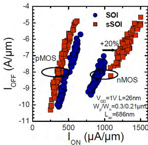
Figure 1.45: I_{ON}/I_{OFF} trade-off for both nMOS and pMOS fabricated on SOI or sSOI substrate, from [And14]. The tensile strain of sSOI results in an improvement of nMOS performance but decreases the pMOS saturation current. This figure highlights the challenge of stress co-integration. In order to enhance the pMOS performance, the tensile stress must be compensated for, by integrating SiGe of high Germanium content [And14; Cas12b; Cas12c].
