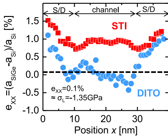
Figure 4.61: Relative deformation in SiGe active area extracted from PED mapping of Figure 4.60. Higher compressive strain observed for the device isolated by oxidation (compressive stress evaluated at \sigma_L = -1.35\text{GPa} ).
