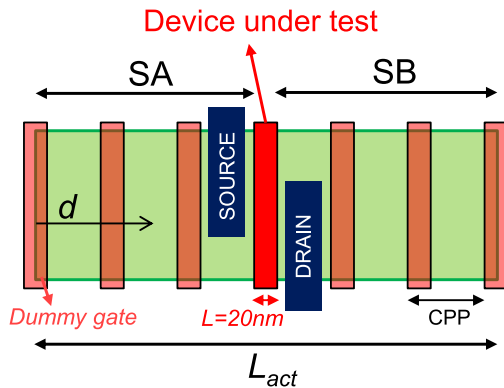
Figure 3.40: Definition of investigated parameters in Local Layout Effects study. SA/SB are the gate-to-STI distances from left and right sides, respectively. The active length L_{act} varies with the number of dummy gates used in the layout.
