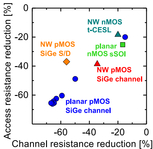
Figure 2.26: Correlation plot of access resistance variation with respect to channel resistance variation. The reference is unstrained device (except for the "planar pMOS SiGe channel", discussed in Figure 3.53). The access resistance is impacted by strain to the same extent as the mobility is.
