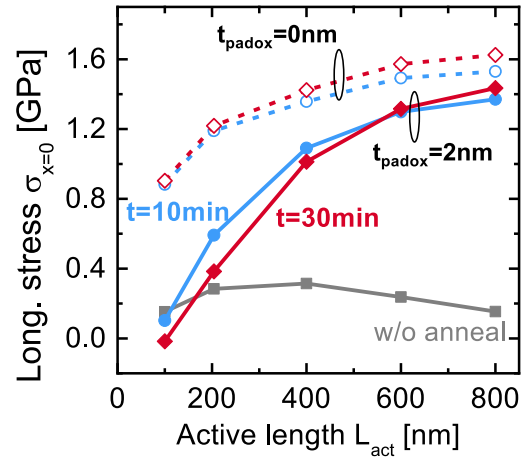
Figure 5.19: Impact of the layout dimension. The loss of efficiency for short active lengths is mainly due to the pad oxide creeping since the stress is highly increased when the pad oxide is not present.
