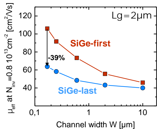
Figure 4.39: Long channel hole effective mobility at N_{\text{inv}}=0.8 \cdot 10^{13} \text{cm}^{-2} according to the channel width. Gain from biaxial to uniaxial stress configuration is higher for SiGe-first than for SiGe-last.
