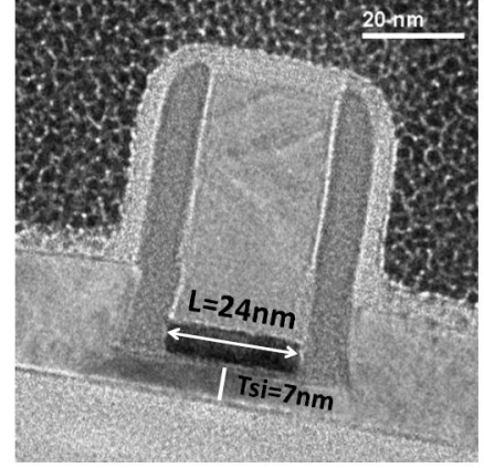
Figure 1.22: Cross-section of a FDSOI transistor from 28nm technology. The film thickness t_{Si} is 7nm. Figure from [Pla12].
