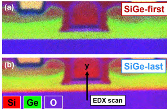
Figure 4.36: Energy-dispersive X-ray spectroscopy (EDX) mapping of (a) SiGe-first and (b) SiGe-last at the end of the process flow. A SiGe/Si bilayer is evidenced in the SiGe-last approach.
