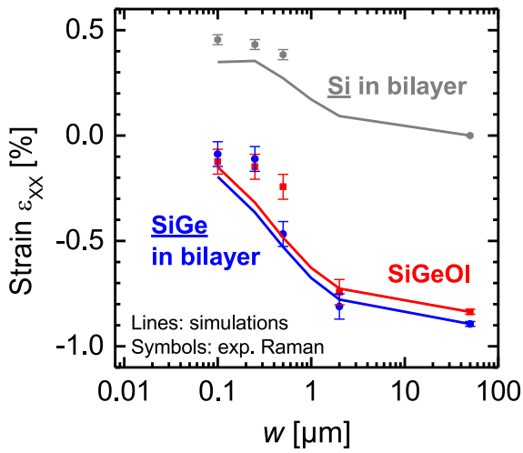
Figure 3.29: Extracted mean strain \varepsilon_{XX} according to the stripe width w for SiGeOI and SiGe/Si bilayer. The lines correspond to FEM mechanical simulations. The SiGe compressive strain decreases when the stripe width is reduced for both samples because of the relaxation on edges. The SOI of the bilayer shows an increased uniaxial tensile strain for reduced stripe widths.
