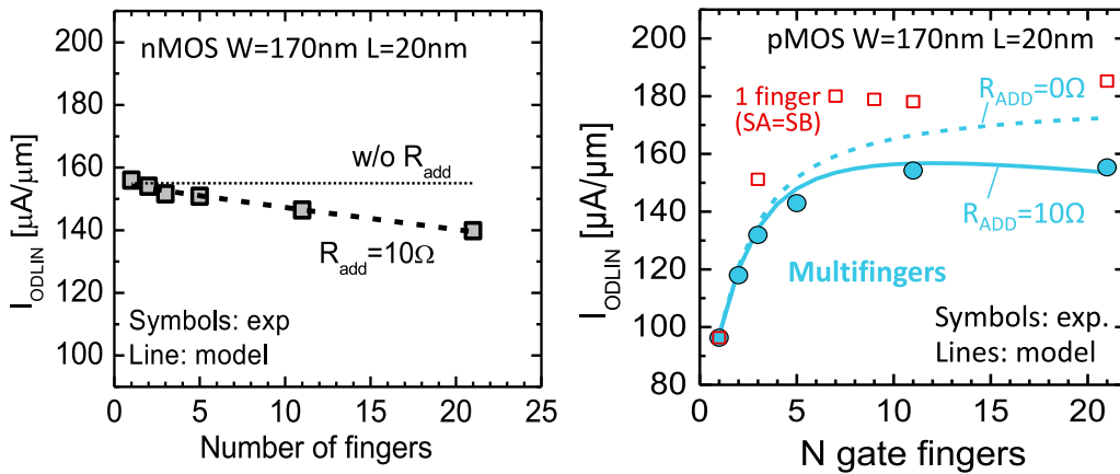
Figure 3.61: Multifinger (left) nMOS and (right) pMOS I_{ODLIN} as a function of the number of gate fingers. The multifinger model reproduces well the experimental data, provided that an additional parasitic series resistance is considered, consistently with nMOS results.
