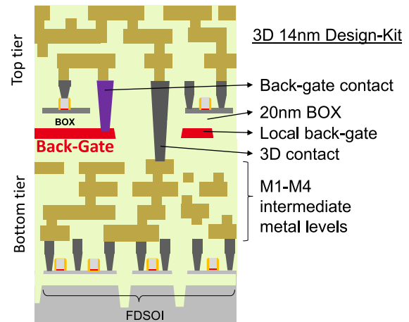
Figure 5.44: Schematic stack of the 3D 14nm Design Kit used for SPICE simulations. It features 4 intermediate metal levels, a 20nm-thick BOX and a 3D-dedicated parasitic extraction model.
