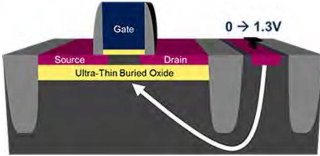
Figure 1.21: FDSOI transistor schematic, from STMicroelectronics. The transistor is built on a Silicon On Insulator (SOI) substrate. The thin Silicon film and buried oxide (BOX) allow a good electrostatic control. The channel-body coupling due the BOX enables a high back-bias efficiency.
