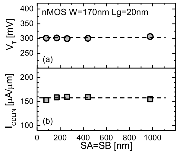
Figure 3.49: (a) V_{TLIN} and (b) I_{ODLIN} as a function of the gate-to-STI distance SA (=SB) for a W=170\text{nm} L=20\text{nm} nMOS device. No layout effect is observed because nMOS channel is unstrained. This result also shows that possible stress generated by STI proximity is not significant.
