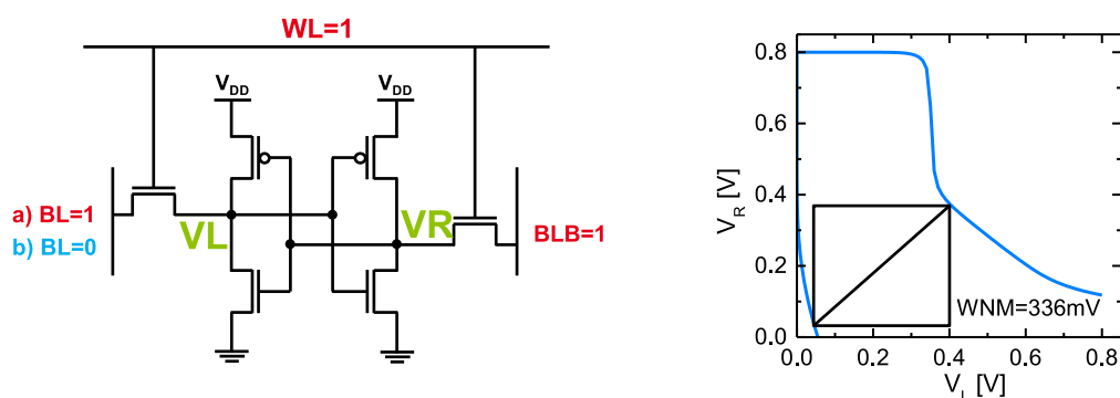
Figure B.5: (left) SRAM WNM extraction, consisting of two voltage transfer characteristics VR(VL) vs. VL(VR) while WL=BLB=1 and BL=1(=0). The WNM is given by the side of the smallest square embedded between the two curves (right).
