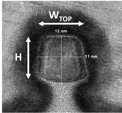
Figure 2.22: TEM cross-section of \Omega -gate-shaped nanowires investigated in this work. The section is defined by the sidewall height H and the top width W_{TOP} . The narrow section ensures a good electrostatic control.
