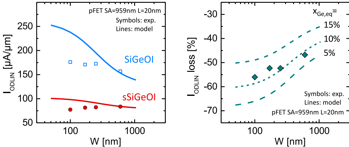
Figure 5.6: (left) I_{ODLIN} vs. W and (right) I_{ODLIN} loss from SiGeOI to sSiGeOI SA=959nm L=20nm pFETs. Even though the model fails to reproduce the impact of active narrowing (parasitic access resistance), the I_{ODLIN} variation from SiGeOI to sSiGeOI is well captured, assuming an equivalent Germanium concentration of x_{Ge,eq}=10\% .
