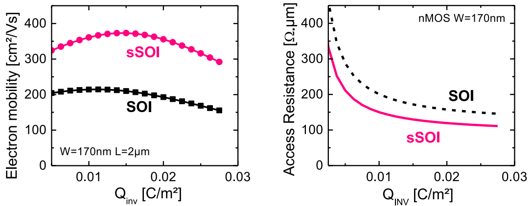
Figure 2.19: Extraction by our new 1/Q_{INV} Y-method of (left) electron mobility as a function of the inversion charge for L=2\mu\text{m} W=170\text{nm} nMOS built on SOI and sSOI substrates and (right) access resistance vs. inversion charge. Tensile strain from sSOI substrate yields both an enhancement of the electron mobility and a reduction of the access resistance (-25% at Q_{INV}=0.01\text{C}/\text{m}^2 ).
