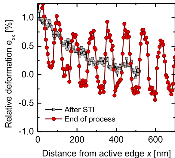
Figure 3.36: Relative deformation e_{xx} profile at the end of the process flow measured by NBED and compared with the profile after etching. Even though SiGe source/drain induces an additional compressive strain, the channels close to the active edge suffer from the relaxation occurring during the patterning.
