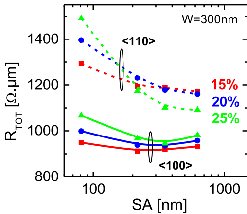
Figure 3.47: R_{TOT} vs. SA for \langle 100 \rangle and \langle 110 \rangle SiGe channel of different Germanium concentrations. \langle 110 \rangle oriented channels suffer from longitudinal stress relaxation while \langle 100 \rangle oriented ones are less sensitive.
