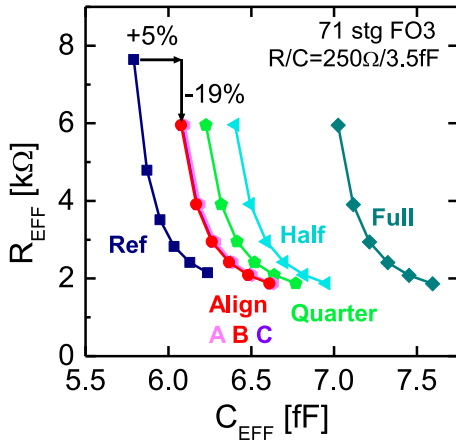
Figure 5.52: Effective resistance R_{EFF} = V_{DD}/2I_{DYN} vs. effective capacitance C_{EFF} = \tau_P/R_{EFF} for the studied layout configurations (see Figure 5.46). Cells operating in double-gate mode suffer from a larger capacitance (from both the active back-gate and parasitic source/drain overlap). The R_{EFF} gain for optimized layouts, especially "Align" cases, counterbalances the C_{EFF} degradation
