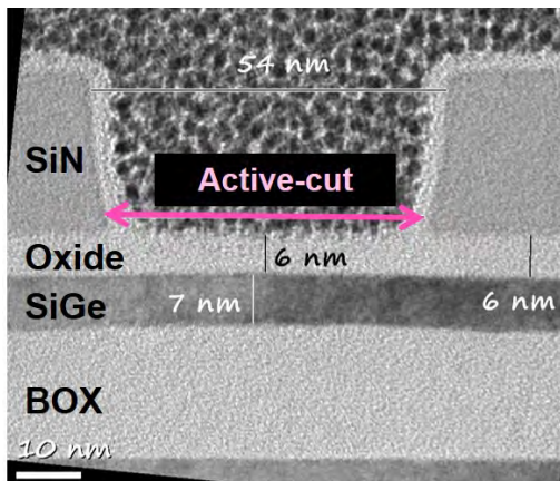
Figure 4.48: TEM picture after "active-cut" etching, corresponding of step (E) of Figure 4.46. The SiN hard mask is reused after CMP. The "active-cut" consists in the minimum distance of isolation in a "Single-Diffusion-Break" layout.
