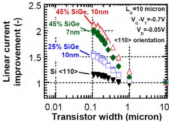
Figure 1.50: Bulk device linear drain current improvement with SiGe active narrowing, from [Ene10]. The enhancement is due to beneficial uniaxial stress configuration.
