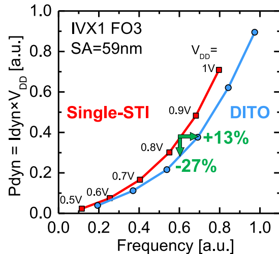
Figure 4.65: P_{dyn} vs. Frequency for DITO and single-STI at different supply voltages V_{DD} . DITO enables to reduce the dynamic consumption by -27% at a given frequency or improves the speed by +13% at same dynamic power.
