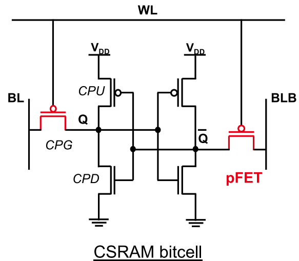
Figure 4.31: Complementary SRAM (CSRAM) bitcell layout. The Pass-Gates consist in pFETs instead of nFETs as in the reference. Such a CSRAM bitcell operates reversely to a classical SRAM: the read operation criterion becomes CPU > CPG and the write one becomes CPG > CPD .
