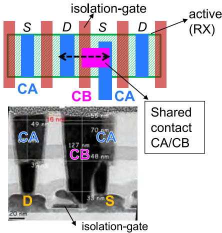
Figure 4.11: Isolation-gate layout construct and associated TEM image showing the shared contact.
