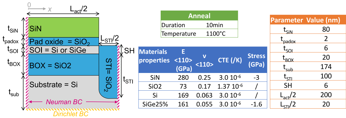
Figure 5.10: BOX-creep simulation half-structure and tables of reference parameters.
