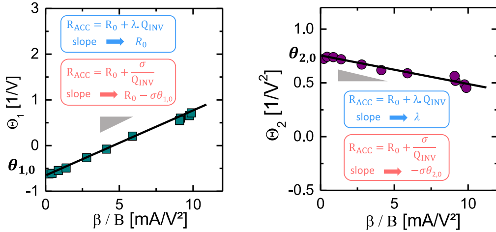
Figure 2.14: (left) \Theta_1 and (right) \Theta_2 vs. \beta (or B ). Linear regressions enable to extract the mobility and access resistance parameters, depending on the model of access resistance (either equation 2.17 or equation 2.32).
