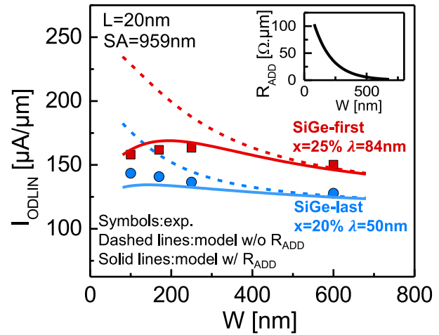
Figure 4.43: I_{ODLIN} vs. W for SiGe-first and SiGe-last short channel devices ( L=20\text{nm} ). The model well reproduces the behaviors if an additional series resistance is considered for both integrations. The additional access resistance is attributed to faceted source/drain epitaxy, as discussed in section 3.4 (Figure 3.44).
