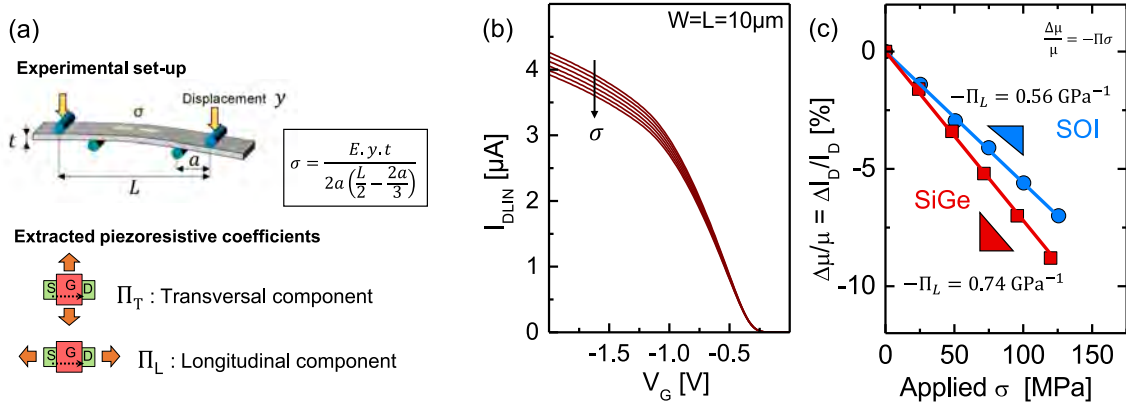
Figure 2.4: (a) Experimental set-up of wafer bending for piezoresistive coefficient extraction and definition of \Pi_L and \Pi_T . (b) Si pFET linear drain current vs. V_G for different externally applied stress. (c) Longitudinal piezoresistive coefficient extraction from linear regression of linear drain current relative variation w.r.t stress. \Pi_L of both Si and SiGe \langle 110 \rangle -oriented pFETs are extracted.
