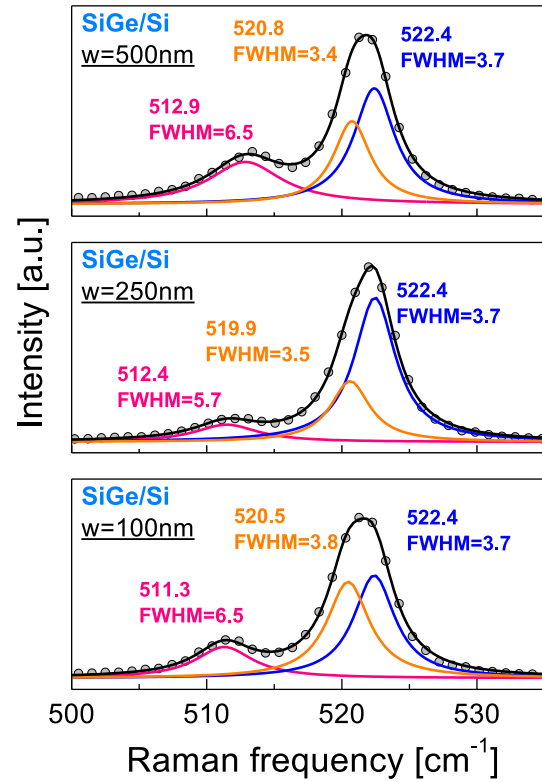
Figure 3.26: SiGe/Si bilayer sample \mu Raman spectra for different stripe widths. The peak positions are determined using Lorentzian function fit. Three regions are considered: the SiGe, the SOI and the Si bulk (see Figure 3.27). The pink line corresponds to the SiGe peak whose position tends toward low frequency when the stripe width is reduced, because of the strain relaxation. The Si bulk reference parameters are fixed (blue line). The SOI peak tends toward low frequency indicating a tensile strain.
