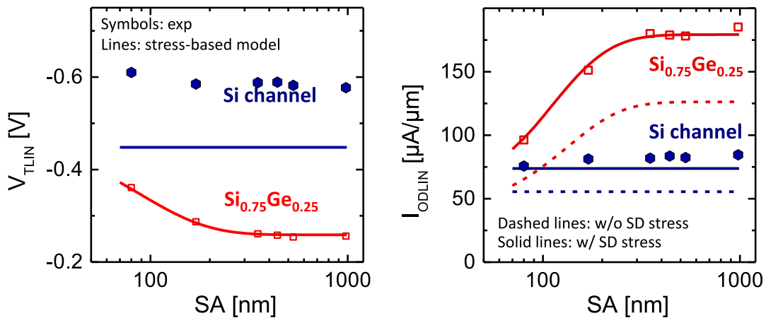
Figure 3.51: (left) V_{TLIN} and (right) I_{ODLIN} vs. gate-to-STI SA (=SB) for W=170\text{nm} L=20\text{nm} pMOS with SiGe and Si channels. The lines derive from the stress-based model calibrated on SiGe channel layout effects. The Si data are well predicted for I_{ODLIN} . The threshold voltage V_{TLIN} is however highly underestimated. This result suggests that the V_T shift with SiGe introduction is not only due to strain, as already evidenced in literature [Cas12b; Sou13].
