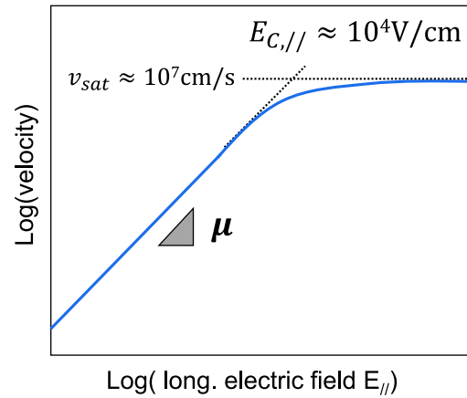
Figure 1.14: Carrier velocity as a function of the longitudinal electric field. Below the critical field, the velocity is directly proportional to the field through mobility. The velocity saturates under high field.
