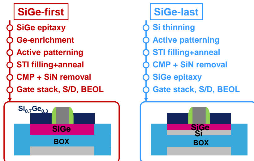
Figure 4.35: Process flow of SiGe-first and SiGe-last integration schemes. The SiGe-first integration scheme, i.e. the process of reference, uses the condensation technique prior to the active area patterning. On the opposite, the SiGe-last process consists in an epitaxy after the STI module, leading to a SiGe/Si bilayer.
