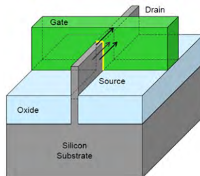
Figure 1.19: FinFET schematic. The FinFET is a 3D transistor where the gate is wrapped around the fin-shaped channel. A FinFET is also referred to as a tri-gate transistor. Figure from Intel.
