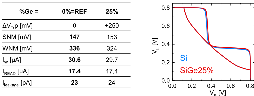
Figure 4.28: (left) SRAM metrics for Si and \text{Si}_{0.75}\text{Ge}_{0.25} PUs at same leakage, obtained thanks to an additional V_{\text{T}} shift of \Delta V_{\text{T},p}=+250\text{mV} and (right) SNM butterfly curve at V_{\text{DD}}=0.8\text{V} . No significant impact of SiGe because of the strong stress relaxation in the small active area of PU.
