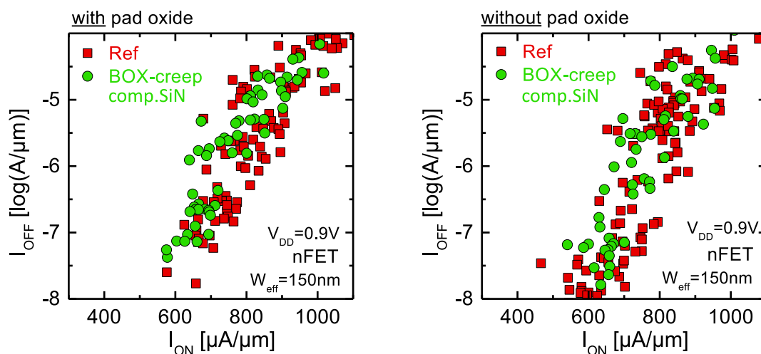
Figure 5.26: I_{ON}/I_{OFF} trade-off for nFET devices after BOX-creep (left) with a pad oxide and (right) without pad oxide. The SiN used for BOX-creep, deposited by PECVD, is compressively stressed ( \sigma_0 \approx -3\text{GPa} ). The anneal is performed at 1100°C for 15min. The BOX-creep technique has low impact on performance, suggesting an inefficient strain transfer.
