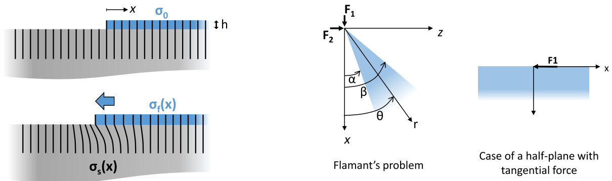
Figure A.1: (left) Illustration of Hu's model structure, consisting of a stressed film mesa etched [Hu79] [Hu91]. (right) Flamant's problem definition [Fla92] and particular case used for Hu's model derivation.
