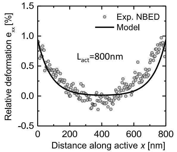
Figure 3.18: Relative deformation after etching from NBED measurement and analytical model for an active length of 800nm. The model well reproduces the experimental data assuming a typical relaxation length \lambda = 84\text{nm} .
