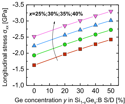
Figure 3.33: Simulated total longitudinal stress according to the Ge concentration in the source/drain y_{Ge} and for different Ge concentrations in the channel x_{Ge} . The simulation is for a non-patterned channel.
