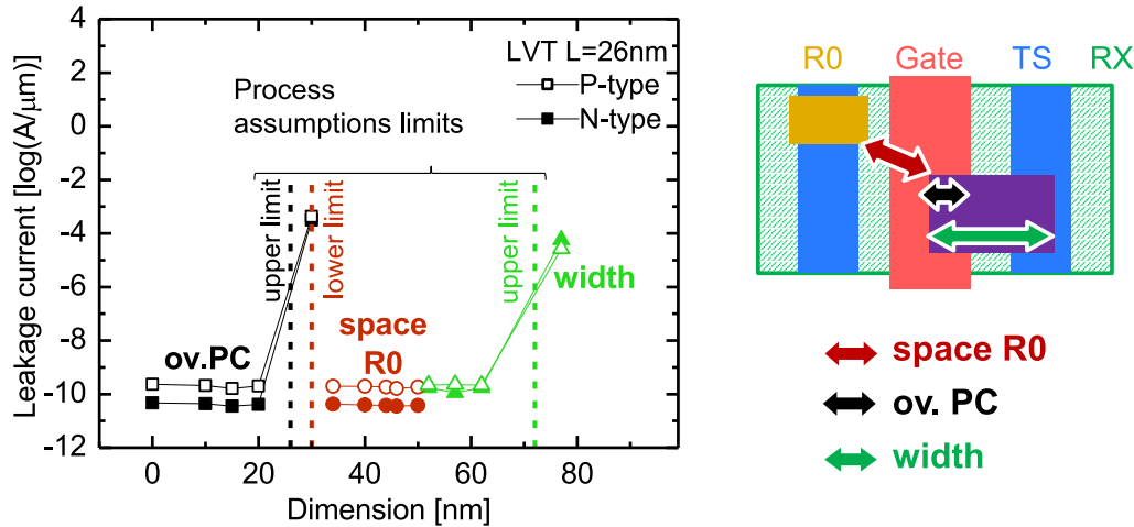
Figure 4.13: Isolation-gate leakage vs. critical dimension variation. No short-cut under process assumptions demonstrating the optimization of the design rules (width of the contact, distance to via and overlap on poly).
