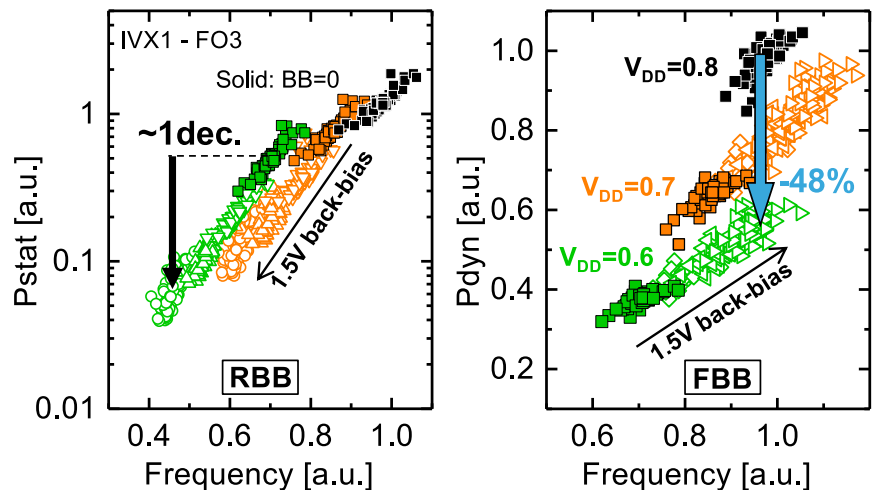
Figure 4.69: P_{STAT} and P_{DYN} as a function of the Frequency. Static power can be reduced by 1 decade under 1.5V RBB and FBB enables the dynamic power to be reduced by -48% at a given frequency.
