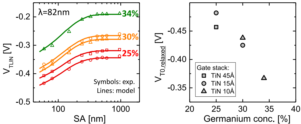
Figure 3.64: (left) V_{TLIN} vs. gate-to-STI SA (=SB) for W=600\text{nm} L=20\text{nm} pMOS with SiGe channels of different Germanium concentrations and different gate stacks (TiN thicknesses). The stress-based model reproduces the experimental data using the same typical relaxation length. (right) V_{T0,relaxed} extracted from the model as a function of the Germanium concentration for different gate stacks. Consistently with Figure 3.51, the threshold voltage shift induced by SiGe is not entirely explained by strain.
