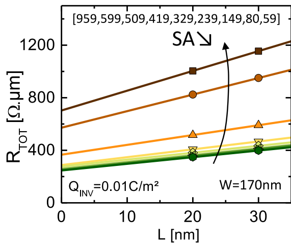
Figure 3.53: R_{tot} vs. L for SiGeOI pMOSFETs of different L_{act} . Slope and intercept of linear regressions give the mobility and the access resistance, respectively.
