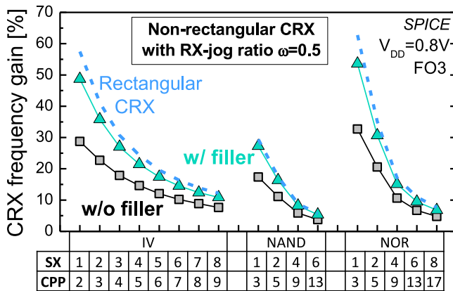
Figure 4.23: Simulated CRX gain for different standard cells (IV/NAND/NOR of different drive) with RX-jog ratio \omega = 0.5 compared to rectangular CRX (i.e. \omega = 0 ). The introduction of a filler cell yields gains close to ideal rectangular CRX.
