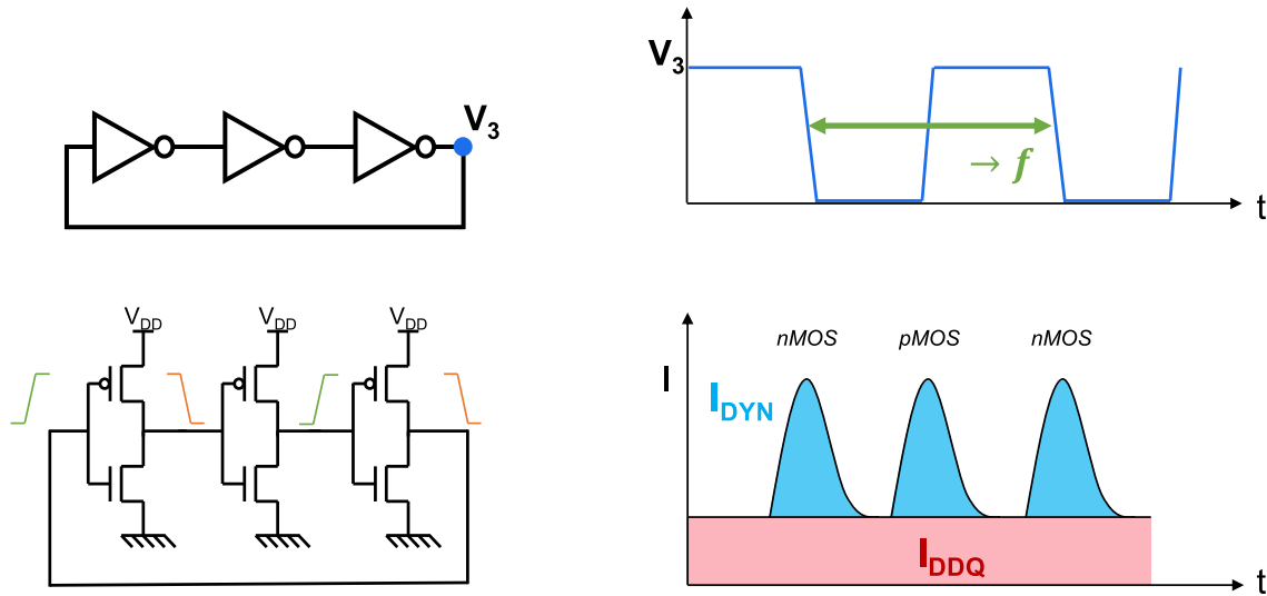
Figure 1.4: (left) symbolic and schematic views of a ring-oscillator made of three inverters. (right) Voltage at the output of the third inverter as a function of time, oscillating between "1" ( V_{DD} ) and "0" ( G_{ND} ) at a frequency f . The current flowing through an inverter is composed of the dynamic current I_{DYN} and the static current I_{DDQ} . The dynamic current is the drive current of either the pMOS or the nMOS to load the output capacitance (i.e. the gates from the next level inverter) during a switching and the static current is the leakage when the inverter is not active.
