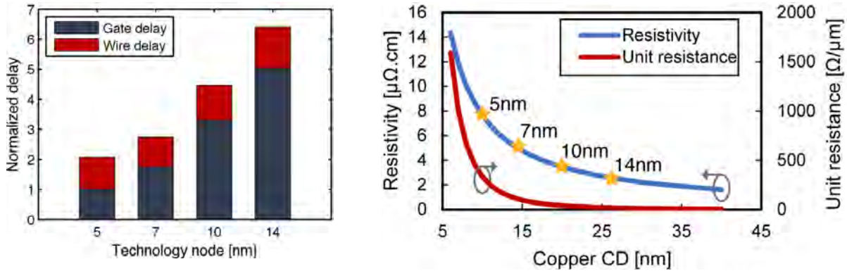
Figure 1.26: (left) Delay partitioning between gate (i.e. transistors) and wire (i.e. interconnections) according to the technology node, from [Huy17]. The interconnection delay becomes more predominant as the technology scales down. (right) Wire resistance and resistivity vs. critical dimension, from [Huy17]. The interconnection resistance rises dramatically when the dimensions are scaled down, especially because of the Copper resistivity increase.
