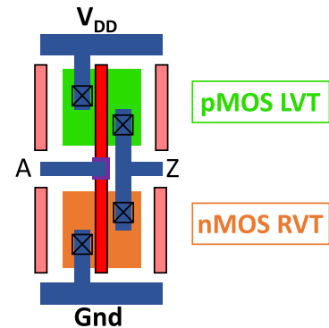
Figure 4.2: Layout of the 1-finger inverter for the MixVT flavor. The use of a LVT pFET compensates for the V_T increase due to the stress relaxation for short active.
