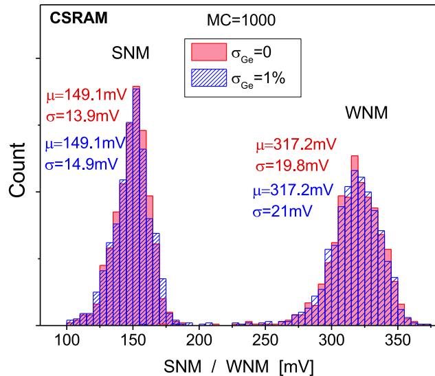
Figure 4.34: CSRAM SNM and WNM distributions at V_{DD}=0.8\text{V} with and without considering Ge concentration fluctuation.
