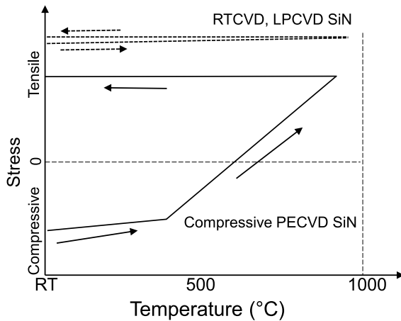
Figure 5.28: Evolution of stress in SiN according to the temperature, from [Ses12]. Both compressive SiN (PECVD) and tensile SiN (LPCVD) are considered. The PECVD SiN loses its compressive stress as the temperature increases. The stress can even be tensile after cooling.
