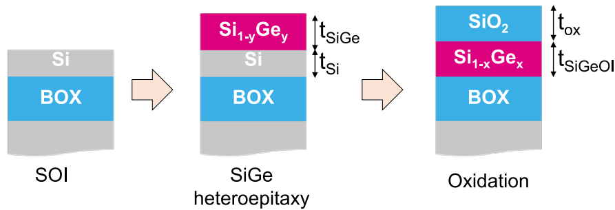
Figure 3.4: Schematic of condensation technique, constituted of two steps: a SiGe heteroepitaxy on a SOI substrate and an oxidation. Silicon atoms are preferentially oxidized. Germanium atoms are thus rejected in the underlying SiGe layer. Interdiffusion of Si and Ge finally leads to a SiGe layer directly on insulator (SiGeOI).
