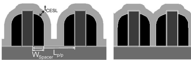
Figure 1.36: Schematic of the impact of contacted poly pitch reduction on the CESL morphology, from [Ene07]. The shorter the CPP, the lower the stress generated in the channel, making this technique irrelevant for aggressively scaled devices.
