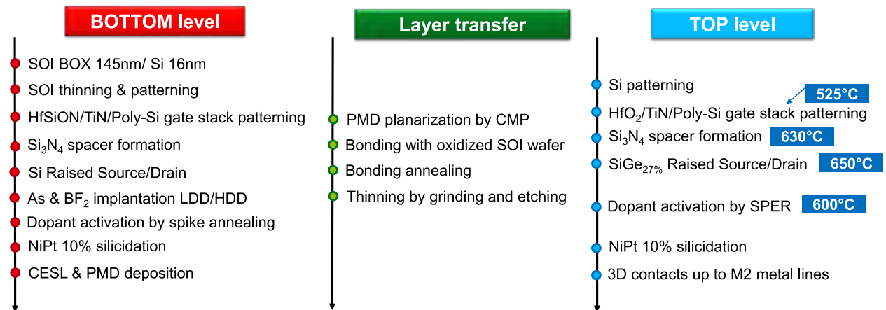
Figure 5.39: Process flow of the 3D-monolithic sequential integration, from [Bru16]. Low thermal budget is required for the second layer processing in order to maintain the stability of the first layer.
