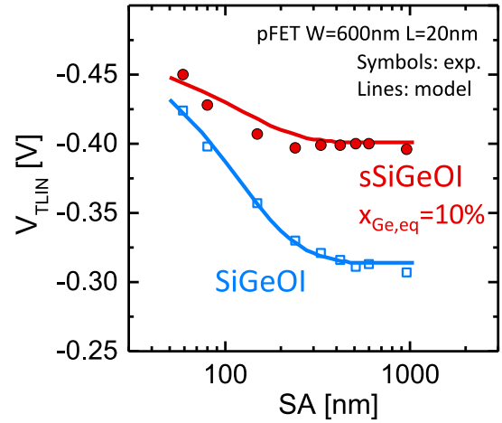
Figure 5.8: pFET V_{TLIN} vs. SA for SiGeOI and sSiGeOI. The lower strain in sSiGeOI yields increased V_{TLIN} and reduced layout effect compared to the SiGeOI reference. The lines correspond to the model, calibrated on the SiGeOI reference and assuming x_{Ge,eq}=10\% in sSiGeOI.
