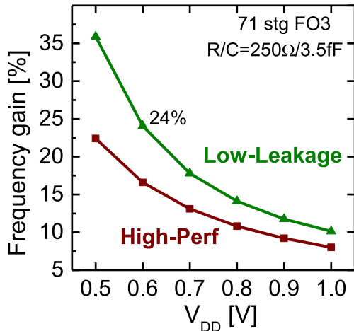
Figure 5.50: Frequency gain with respect to the reference according to the supply voltage V_{\text{DD}} for both the "High Performance" (HP) and "Low Leakage" (LL) cells. The better subthreshold swing in double-gate mode improves its efficiency at low gate overdrive V_{\text{DD}}-V_{\text{T}} . Reducing V_{\text{DD}} or increasing V_{\text{T}} (which is the case for LL cells) thus achieves higher frequency gain in double-gate mode over the single-gate reference.
