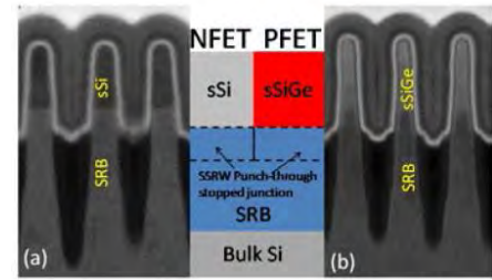
Figure 1.47: TEM cross-section of FinFETs fabricated on SRB, from [Xie16].
