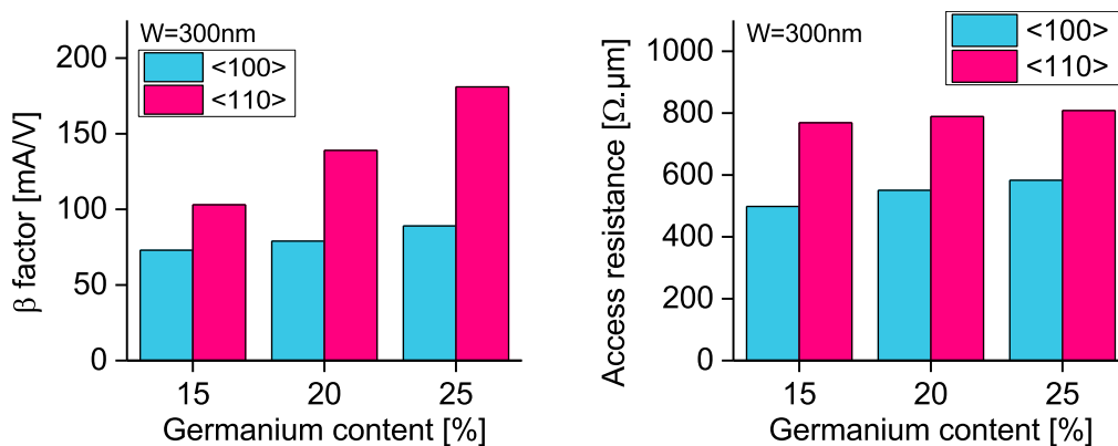
Figure 3.43: (left) \beta factor and (right) R_{ACC} for \langle 100 \rangle and \langle 110 \rangle SiGe channel pFETs of different Germanium concentrations. \langle 110 \rangle oriented channels benefit from a higher mobility thanks to the uniaxial longitudinal stress configuration. However, they also show a degraded access resistance with respect to \langle 100 \rangle oriented channel. This R_{ACC} degradation is attributed to the faceted source/drain epitaxy.
