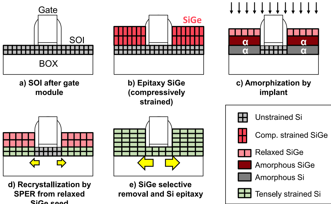
Figure 5.31: Process flow of the SDRASS technique. a) SOI device after gate module fabricated in a gate-first scheme. b) Heteroepitaxy of SiGe in the source/drain region. SiGe is compressively strained because of the lattice mismatch with Silicon. The Germanium concentration used in our experiment is 30%. c) Amorphization by Si implant at 40keV with a dose of 2.5 \cdot 10^{14} \text{ cm}^{-2} . This condition has been chosen according to the results of [Bon16b]. d) Recrystallization from the top seed of relaxed SiGe by Solid Phase Epitaxial Regrowth (SPER) consisting in an anneal at 600°C for 20min. The amorphous Silicon recrystallizes according to the lattice parameter of relaxed SiGe. It is thus tensely strained. e) SiGe selective removal by wet etching and epitaxy of Si for raised source and drain. This step allows a higher strain transfer into the channel thanks to the high volume of tensely strained source/drain.
