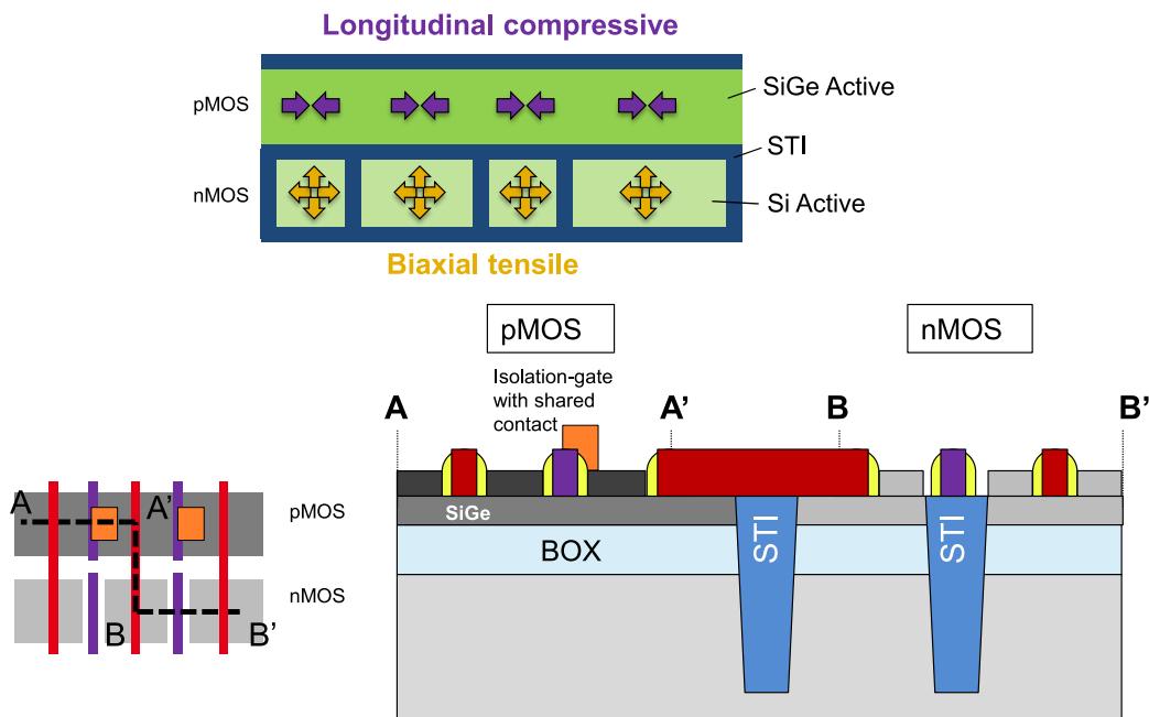
Figure 5.22: Illustration of stress configuration co-optimization by BOX-creep technique. A compressive SiN is used for the BOX-creep, introducing tensile stress after annealing. The isolation of nMOS is made with STI in both longitudinal and transverse directions to take benefit of the BOX-creep technique. The pMOS featuring SiGe channel is patterned only in the transverse direction, enabling the transverse stress to relax. Isolation-gates are used in the pMOS row as in a Continuous-RX approach (see section 4.2.2).
