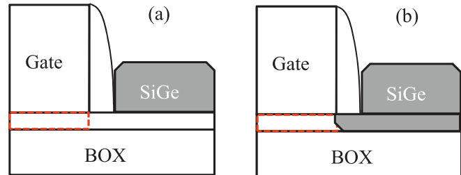
Figure 1.40: Schematic of the (b) Self-Aligned In-Plane Stressor (SAIPS) compared to the (a) conventional SiGe source/drain stressor, from [Mor16]. SAIPS induces an additional compressive stress in the channel from an increased volume of SiGe stressor, which is also better localized for transferring the stress into the channel.
