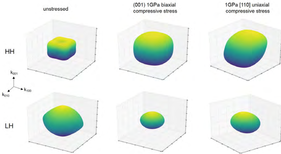
Figure 1.31: Energy iso-surfaces of (top) HH and (bottom) LH under different stress configuration: (left) unstressed, (middle) (001) biaxial compressive stress, (right) [110] uniaxial compressive stress.
