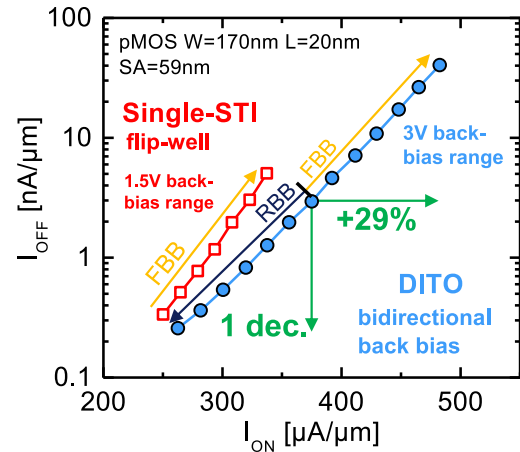
Figure 4.68: pFET I_{ON}/I_{OFF} trade-off at V_{DD}=0.8V for different back-biases. DITO enables a full back-bias operation while single-STI is limited to FBB in a flip-well architecture.
