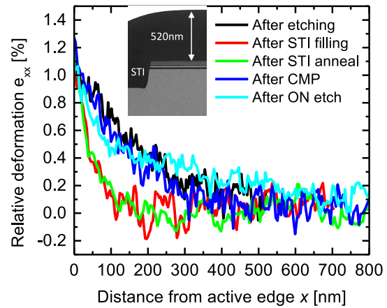
Figure 3.11: SiGeOI active area relative deformation e_{xx} profile measured by NBED after each process step of the STI module. Strain profile at the end of active area patterning is governed by the etching step that induces a strong relaxation. The change in profile after STI filling is attributed to a thermal stress from the thick (520nm) oxide layer on top of the structure (see TEM image after filling in inset).
