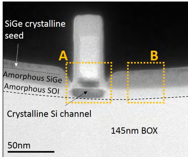
Figure 5.32: TEM after the SDRASS amorphization showing the top seed of crystalline SiGe in source/drain. The underlying SOI is amorphous while the channel is still crystalline since it is protected by the gate.
