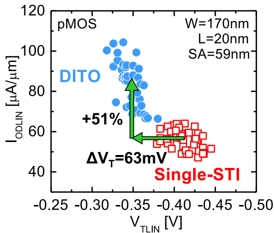
Figure 4.54: I_{ODLIN} vs. V_{TLIN} for DITO and single-STI. DITO improves I_{ODLIN} by +51% and reduces V_{TLIN} by -63mV.
