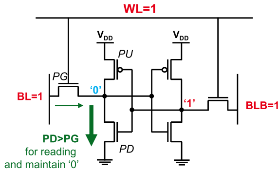
Figure B.2: SRAM reading operation. Both bit lines are precharged to '1'. The reading criterion PD>PG allows the internal node at '0' to be maintained.
