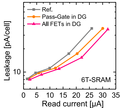
Figure 5.55: SRAM (left) table of metrics and (right) leakage vs. read current according to their double-gate configuration. The read and write currents are enhanced when the Pass-Gate is in double-gate mode, at the expense of a reduced SNM. All FETs in double-gate mode leads to +30% read and write currents without degrading the leakage.
