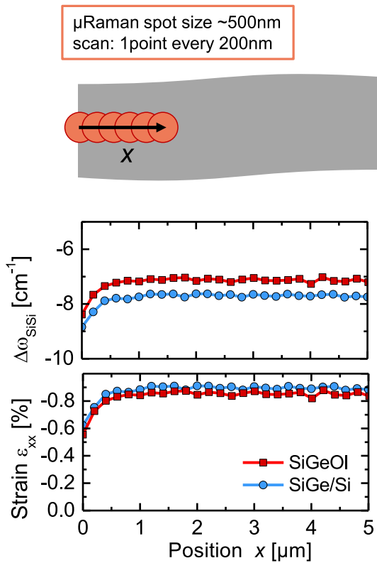
Figure 3.23: Raman scans close to the edge of the w=50\mu\text{m} stripe for both the SiGeOI and the bilayer samples. (top) Raman frequency shift and (bottom) extracted strain assuming relaxation in one direction. Raman spectra are measured every 200nm. The size of the spot is approximately 500nm, making it impossible to assess the relaxation profile with a sufficient resolution.
