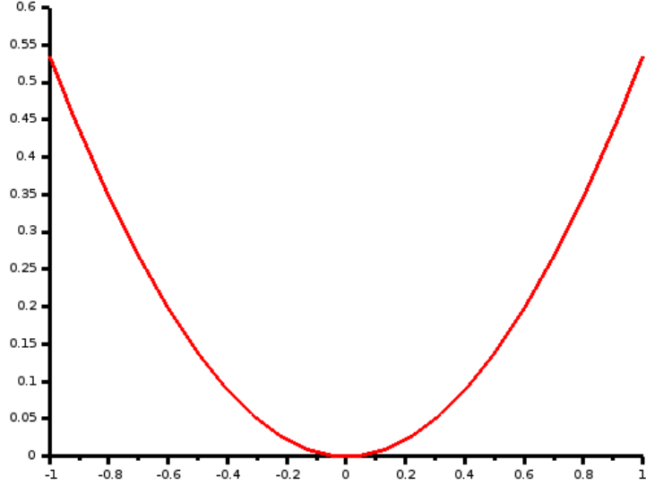
FIGURE 5.2: \Lambda^* for the first example.
