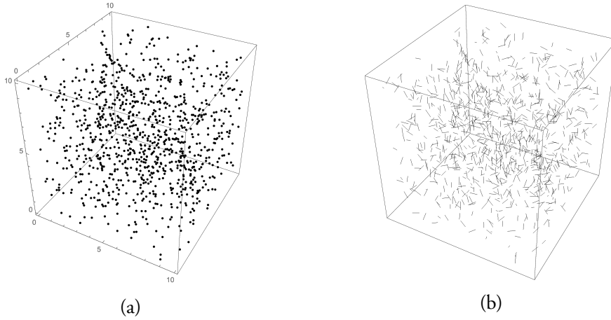
Figure 4.15: Distribution of fibers in 3D: (a) fiber midpoints; (b) whole fibers.
