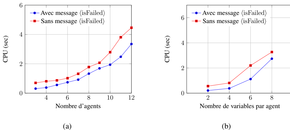
FIGURE 4.4 – Elimination du message \langle isFailed \rangle
