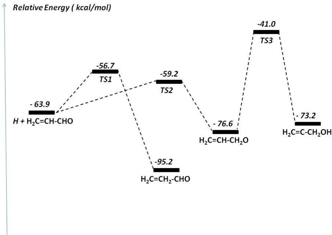
Figure VI-10: Relative energies of H_2C=CH_2-CHO , H_2C=CH-CH_2O and H_2C=C-CH_2OH and transitions states for H + H_2C=CH-CHO reaction according to Kwon et al. 28 TS1 and TS2 are the transitions states that lead to the reaction products H_2C=CH_2-CHO and H_2C=CH-CH_2O . TS3 is the transition state between the two isomeric forms H_2C=CH-CH_2O and H_2C=C-CH_2OH .
