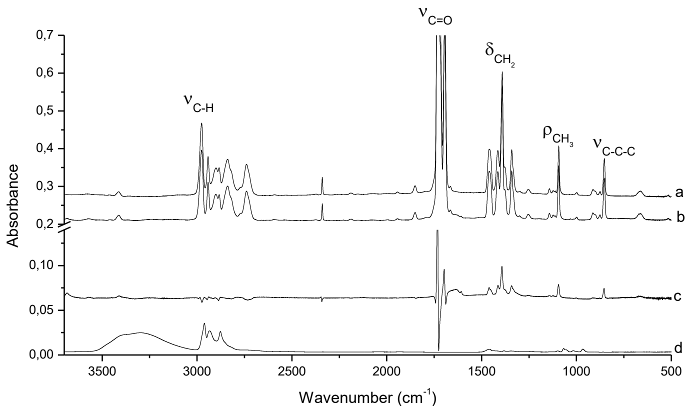
Figure VI-4: IR spectra of: a) Deposition of 4 \mu\text{mol} of propanal ( \text{CH}_3\text{CH}_2\text{CHO} ) on a mirror maintained at 10K. b) Hydrogenation of solid propanal at 10K. c) Difference spectrum: Spectrum (b) - spectrum (a). d) Deposition of 0.2 \mu\text{mol} of pure propanol ( \text{H}_3\text{C}-\text{CH}_2\text{CH}_2\text{OH} ) on a mirror maintained at 10 K (signal divided by approximately 10 in comparison with that of figure VI-2d).
