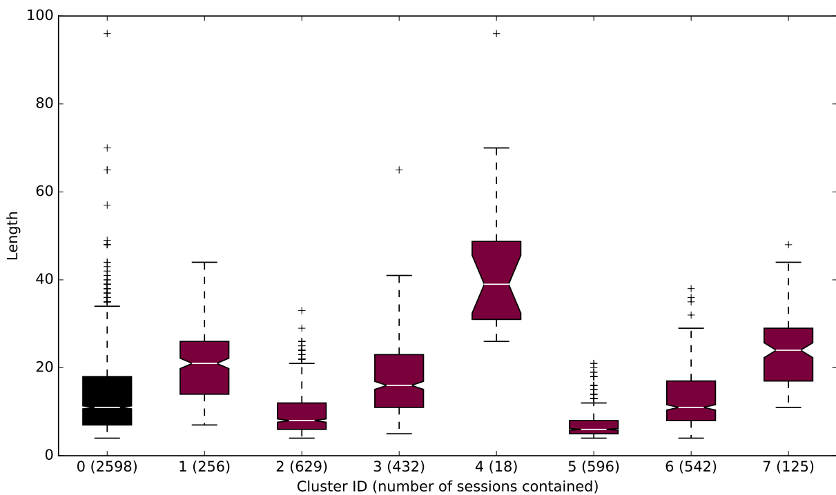
Figure I.3.15: System 50 session length distribution for each cluster. In parenthesis, the number of sessions contained in each cluster. Cluster 0 represents the whole dataset.
