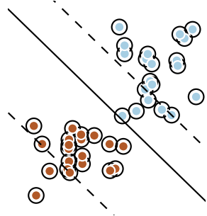
Figure 2.6: NuSVM example: We present two classes as blue and brown points. The NuSVM learns a hyperplane, a line in this two dimensional case, to discriminate the two classes. The nu parameter permits to regularize the algorithm by controlling the number of support vectors selected. For small value of nu , few observations are selected as support vectors, while for a large value of nu , all observations are selected.
