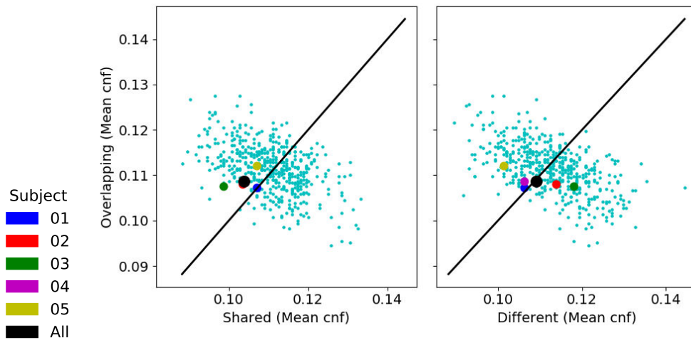
Figure A.14: Superposition test in aSTS : We present the relationship between the mean confusion of cell groups representing overlapping syllables, shared syllables and different syllables. The smaller cyan dots correspond to the shuffled models of all subjects. All other dots correspond to subjects. If the mean confusion values of a tested model is reflected as a dot above the black line in both plots, then we have evidence for superposition. A star means significance with a p-value < 0.05
