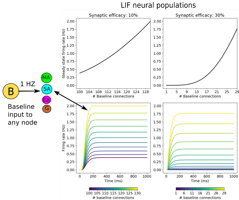
Figure 10.1: LIF Baseline neural dynamics: The plots at the top show how the steady state rate of a neural population relates to the number of baseline connections for a baseline input of 1Hz. The plots at the bottom show the temporal dynamics for different number of baseline connections.
