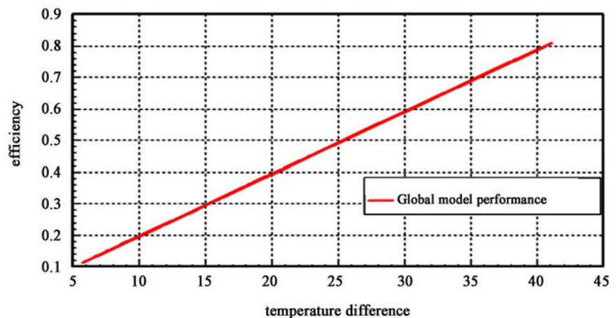
Figure 13. Performance of solar collector.
