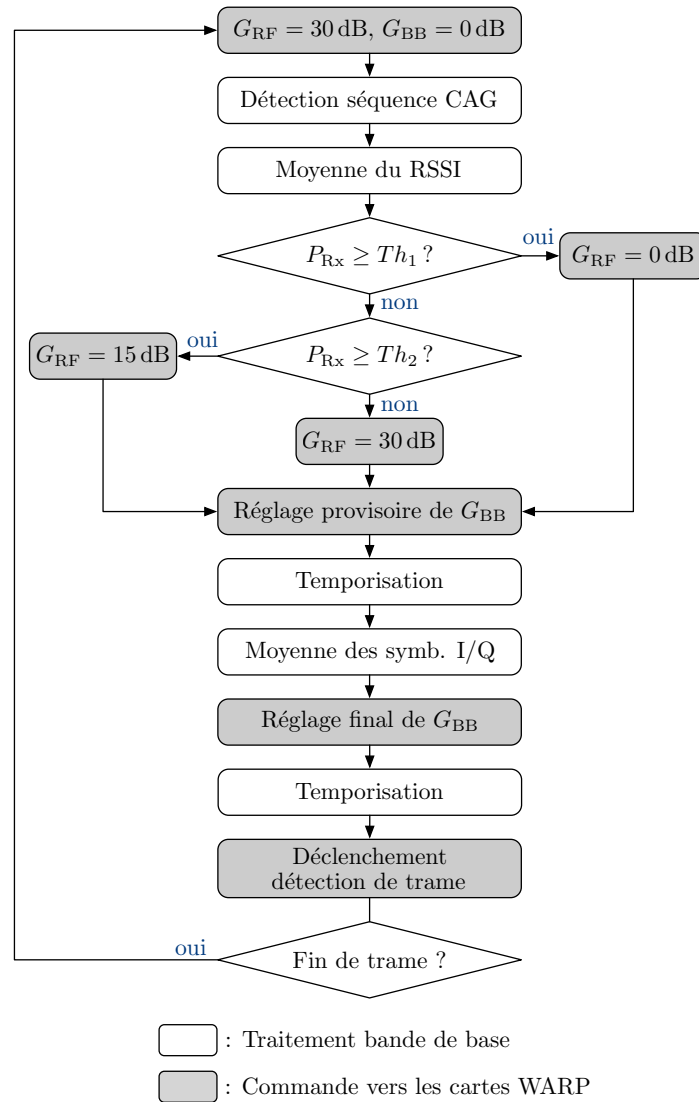
FIGURE 5.5 – Algorithme de CAG
