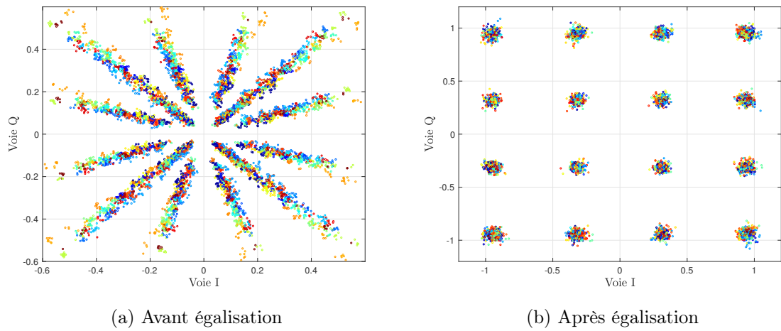
FIGURE 5.13 – Constellations 16 QAM reçues
