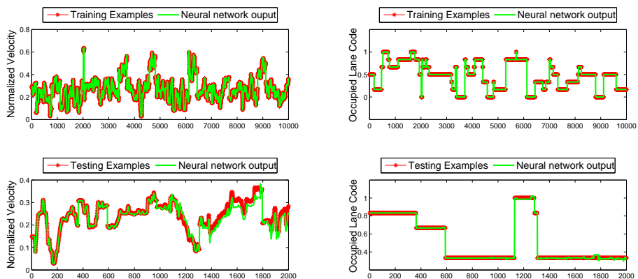
Figure 3.15: Result of Learned NN after HMM labeling by BFGS-algorithm
