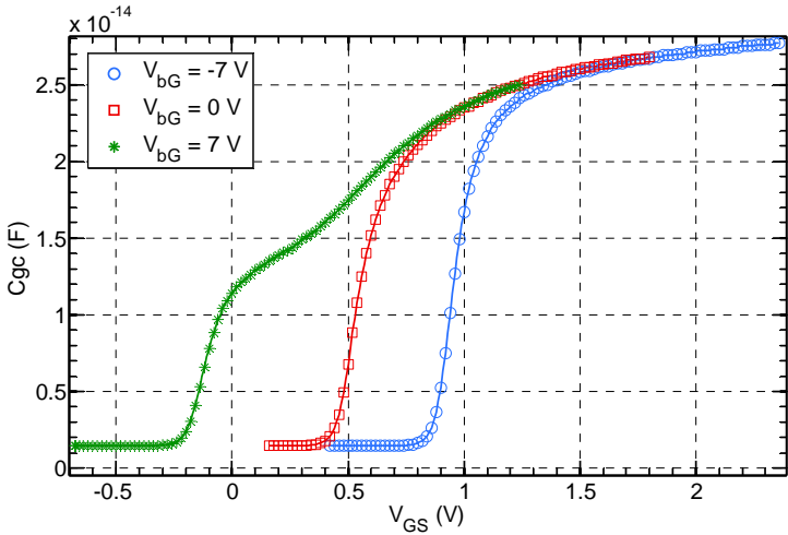
Fig. 2.5 TCAD simulations of the gate capacitance versus V_{GS} for three V_{bG} values (-7 V, 0 V, and 7 V) for L = 1 \mu\text{m} and V_{DS} = 1 \text{ V} .
