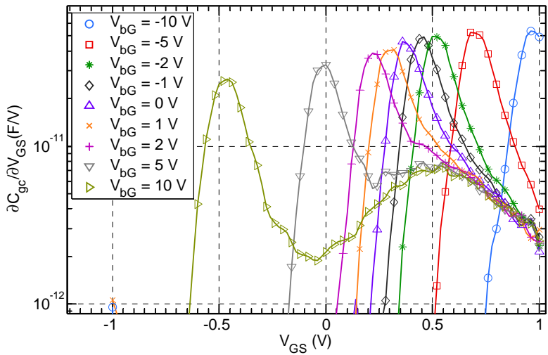
Fig. 2.4 Measured gate capacitance derivatives versus V_{GS} for various back gate voltages for NMOS ( L = 10 \mu\text{m} , W = 2 \mu\text{m} , MULT = 30 ).
