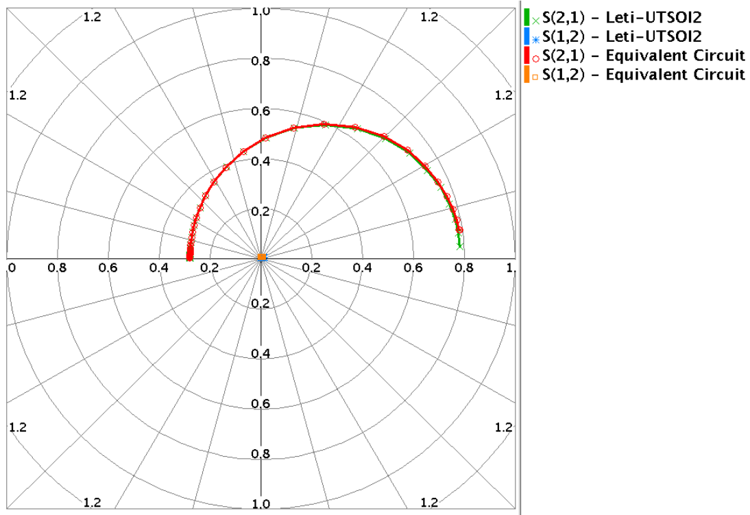
Fig. 2.33 Polar chart showing the input to output and output to input S-parameters simulated using the proposed equivalent circuit in Fig. 2.18 and the Leti-UTSOI2 of L = 1 \mu\text{m} NMOS in saturation ( V_{\text{DS}} = 1 \text{ V} ).
