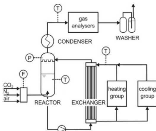
Figure 50: LEMEDES-CO 2 lab-scale equipment (F: flowmeter; T: temperature probe; P: pressure sensor).
