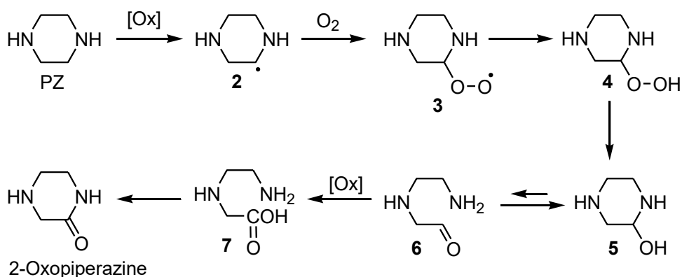
Figure 37: Formation of 2-oxopiperazine
