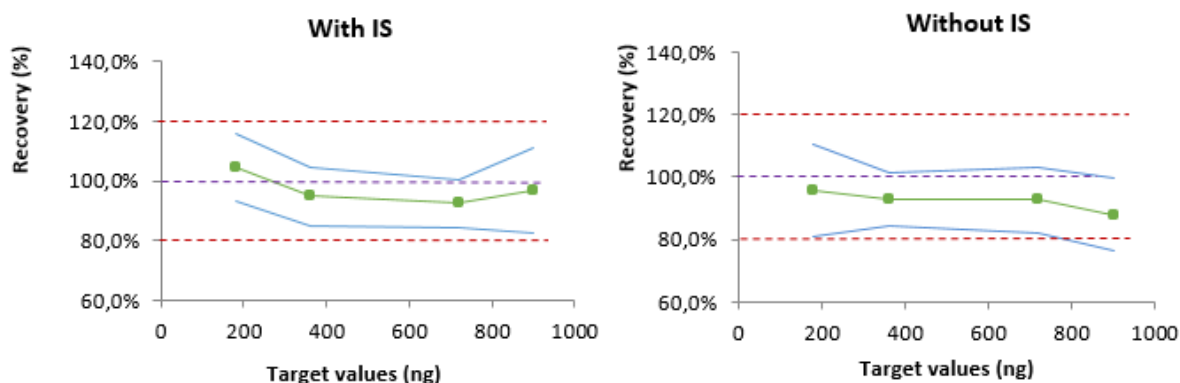
Figure 20: Evaluation of the interest of using NDMA-d 6 as internal standard
