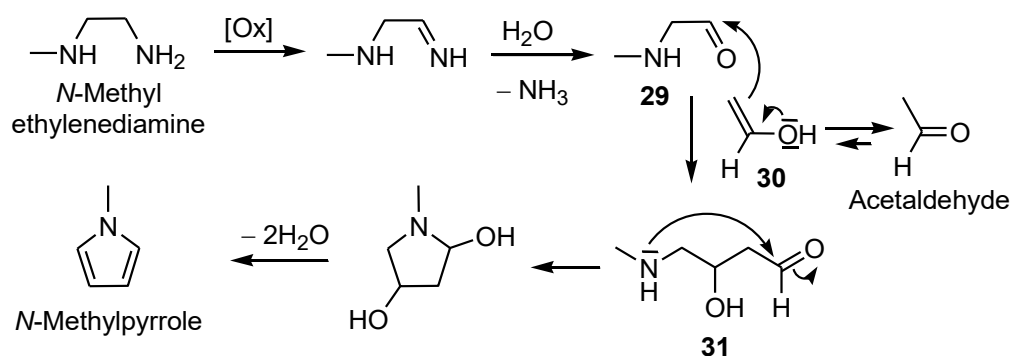
Figure 45: Formation of N -methylpyrrole
