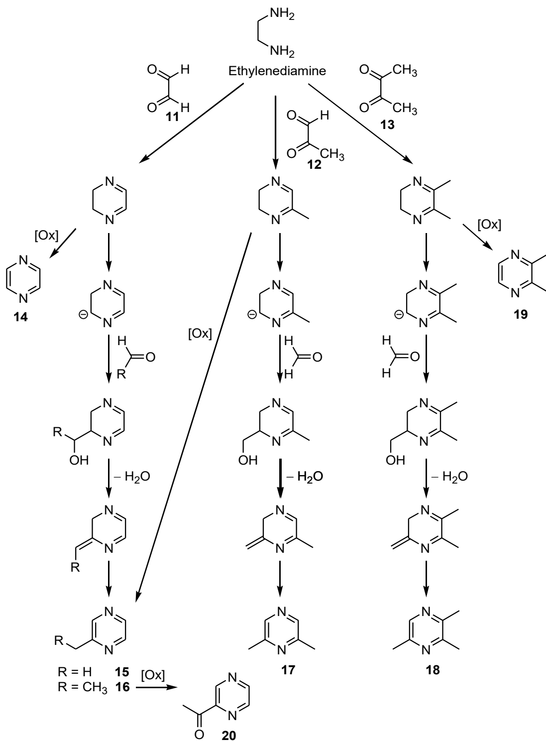
Figure 39: Formation of five alkyipyrazines
