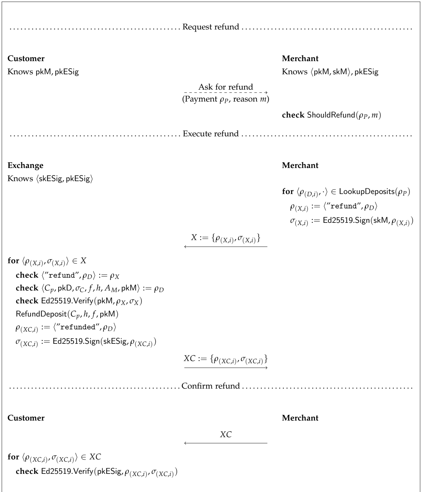
Figure 4.19.: Refund protocol
