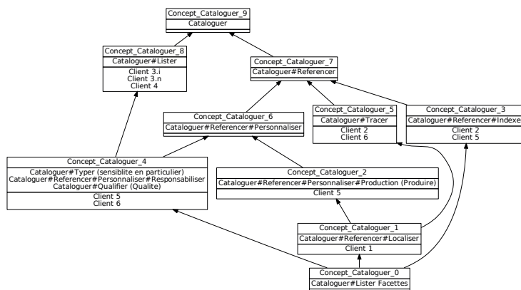
FIGURE 8.14: AC-Cataloguer-simple
