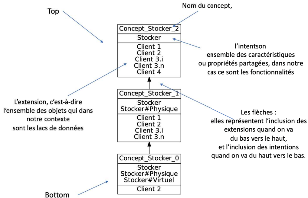
FIGURE 6.5: Un concept
