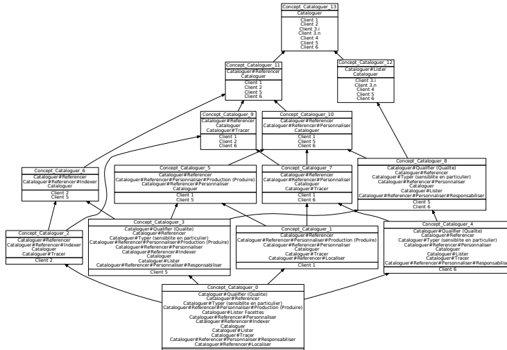
FIGURE 8.17: FCA-Cataloguer-plein
