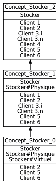
FIGURE 8.24: FCA-stocker-plein
