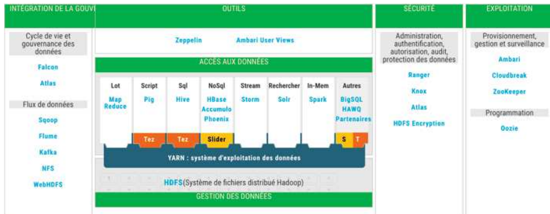
FIGURE 5.3: Plateforme HortonWorks
