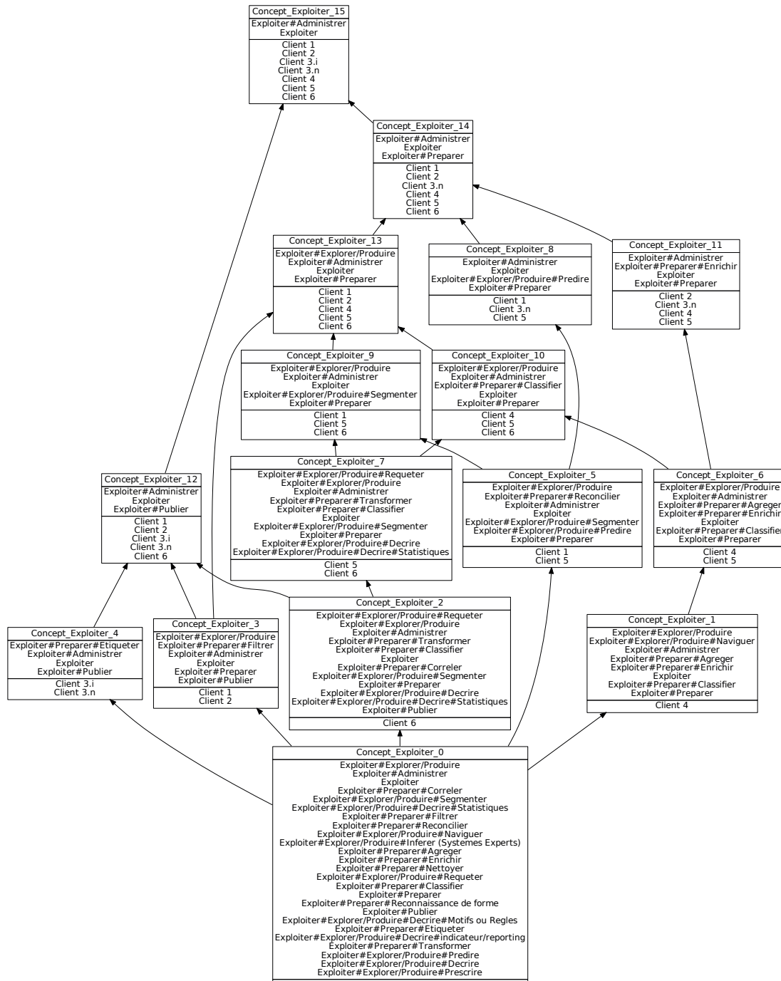
FIGURE 8.29: AC-Exploiter-plein
