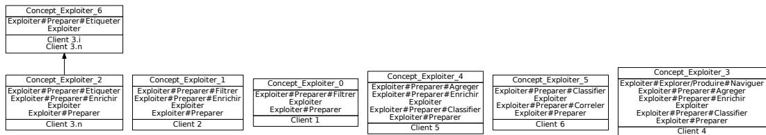
FIGURE 8.33: AOC-Exploiter-plein
