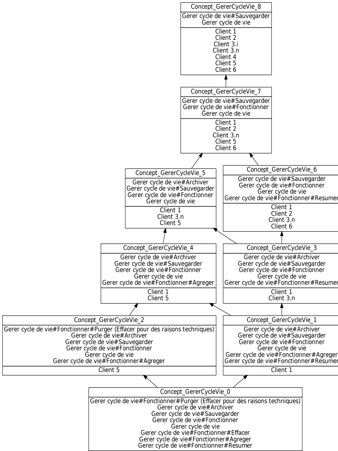
FIGURE 8.38: FCA-Gérer-plein
