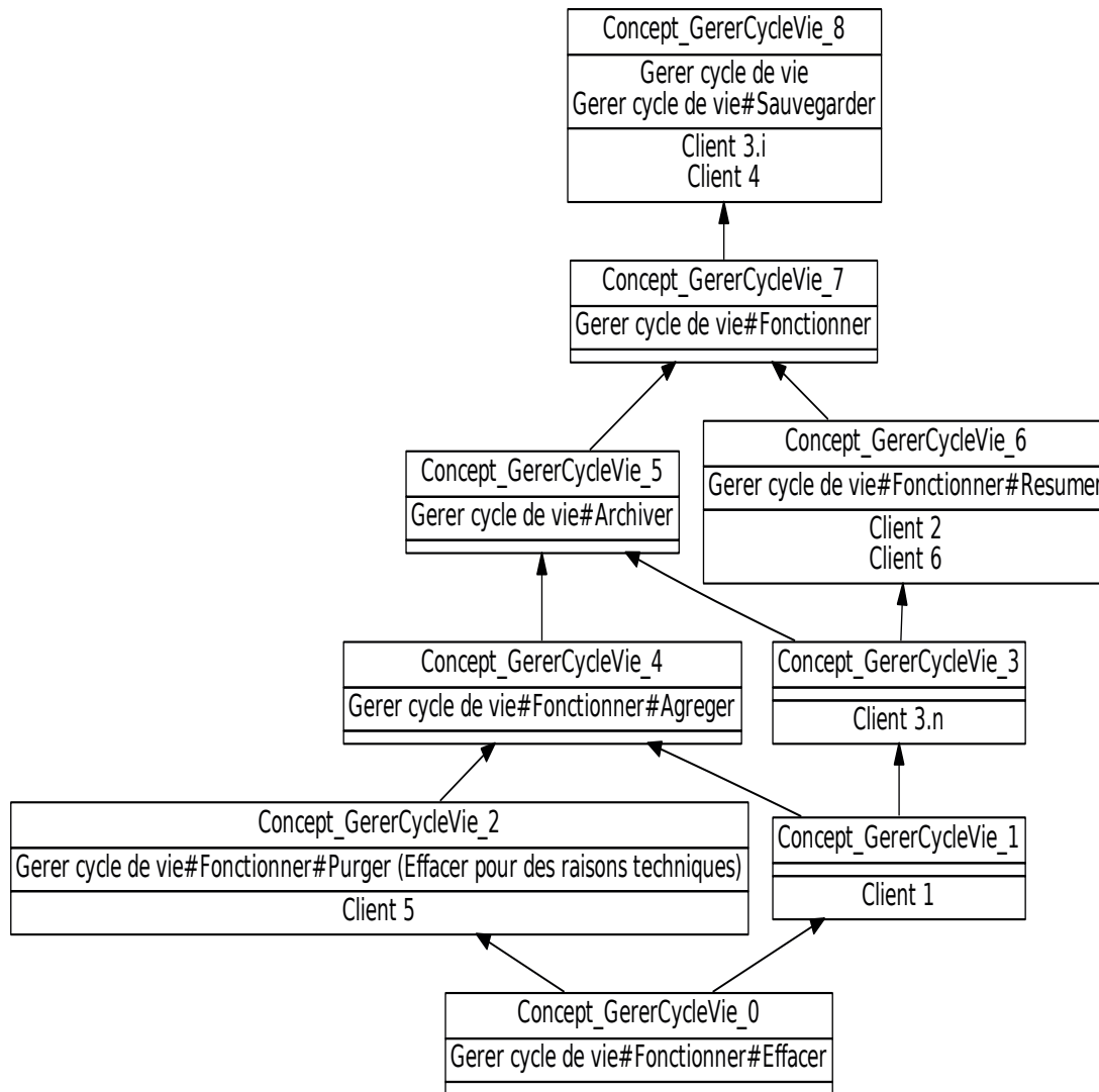
FIGURE 8.37: FCA-Gérer-simple
