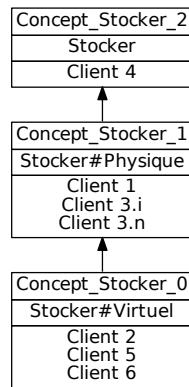
FIGURE 8.23: FCA-stocker-simple
