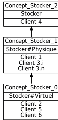
FIGURE 8.21: AC-stocker-simple
