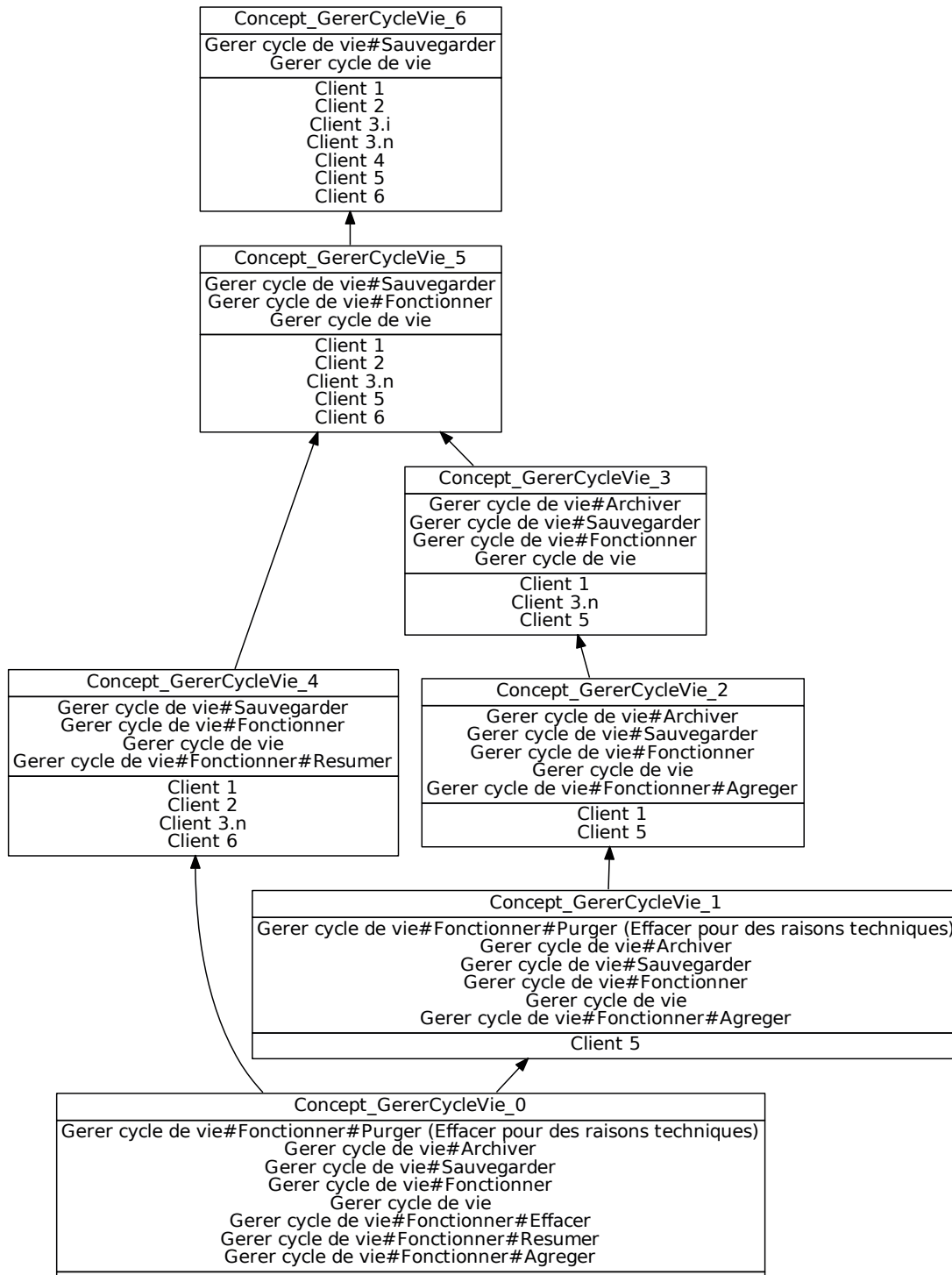
FIGURE 8.36: AC-Gérer-plein
