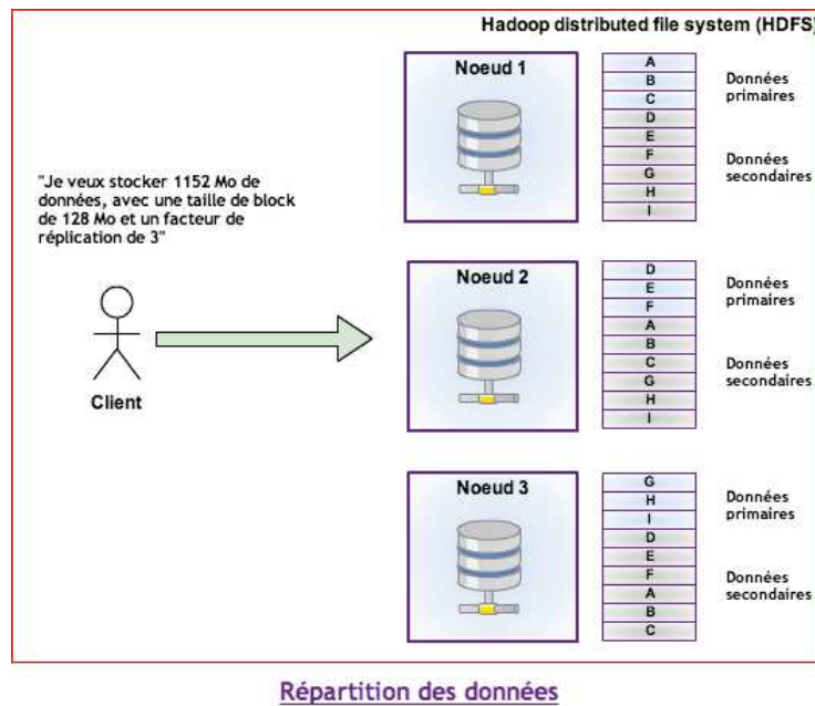
FIGURE 3.21: Apache Hadoop-Fichier HDFS
