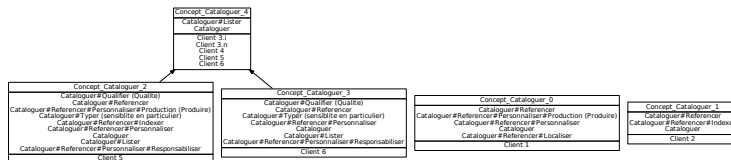
FIGURE 8.19: AOC-Cataloguer-plein
