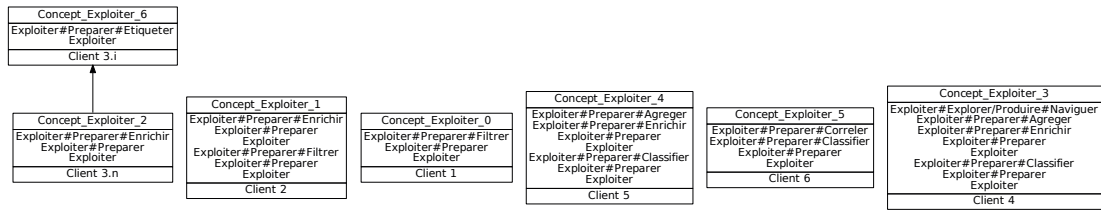
FIGURE 8.32: AOC-Exploiter-simple
