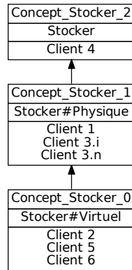
FIGURE 8.25: AOC-stocker-simple
