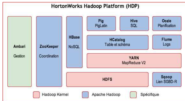
FIGURE 3.25: Distribution HortonWorks
