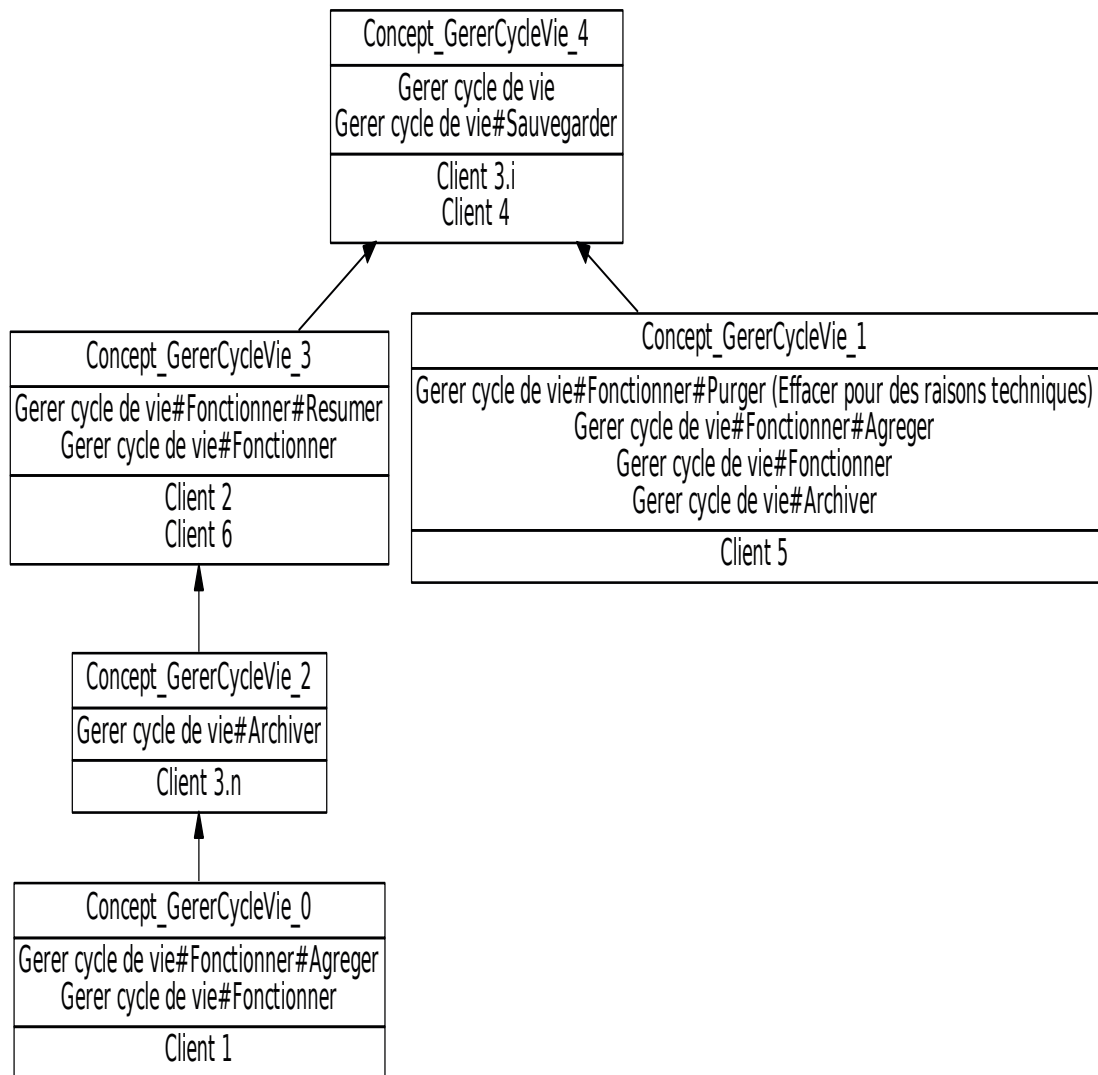
FIGURE 8.39: AOC-Gérer-simple
