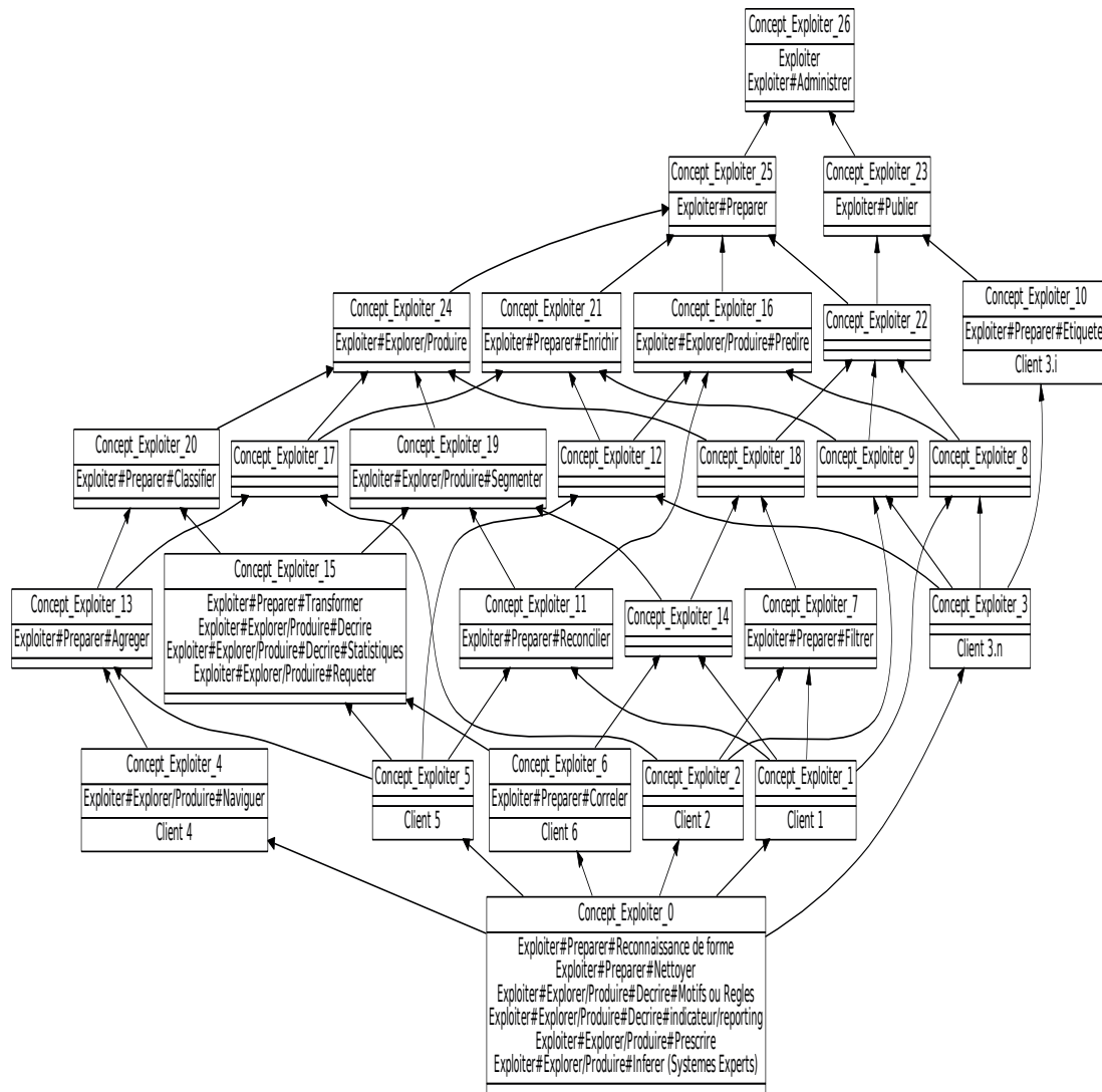
FIGURE 8.30: FCA-Exploiter-simple
