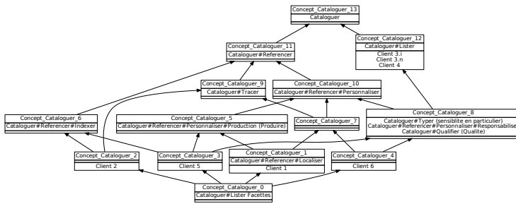
FIGURE 8.16: FCA-Cataloguer-simple
