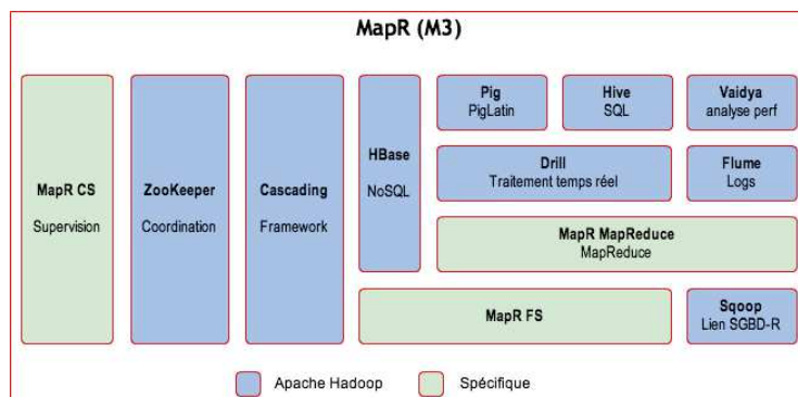
FIGURE 3.27: MapR
