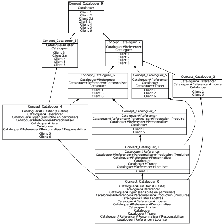
FIGURE 8.15: AC-Cataloguer-plein
