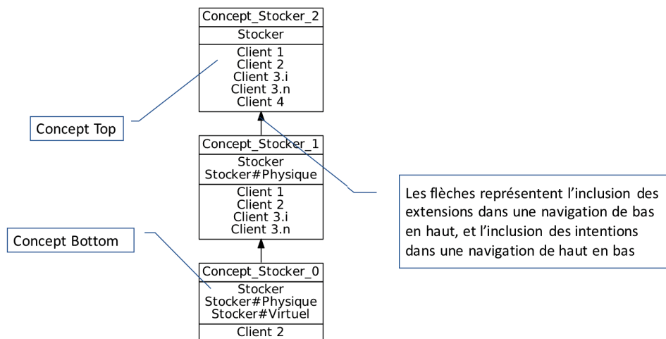
FIGURE 6.6: Un treillis de concepts
