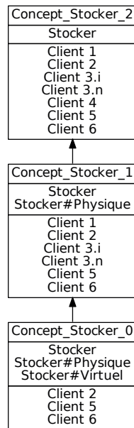
FIGURE 8.26: AOC-stocker-plein
