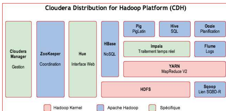
FIGURE 3.26: Distribution Cloudera
