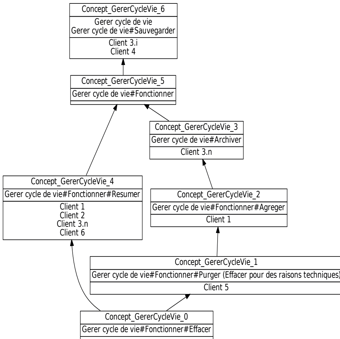
FIGURE 8.35: AC-Gérer-simple
