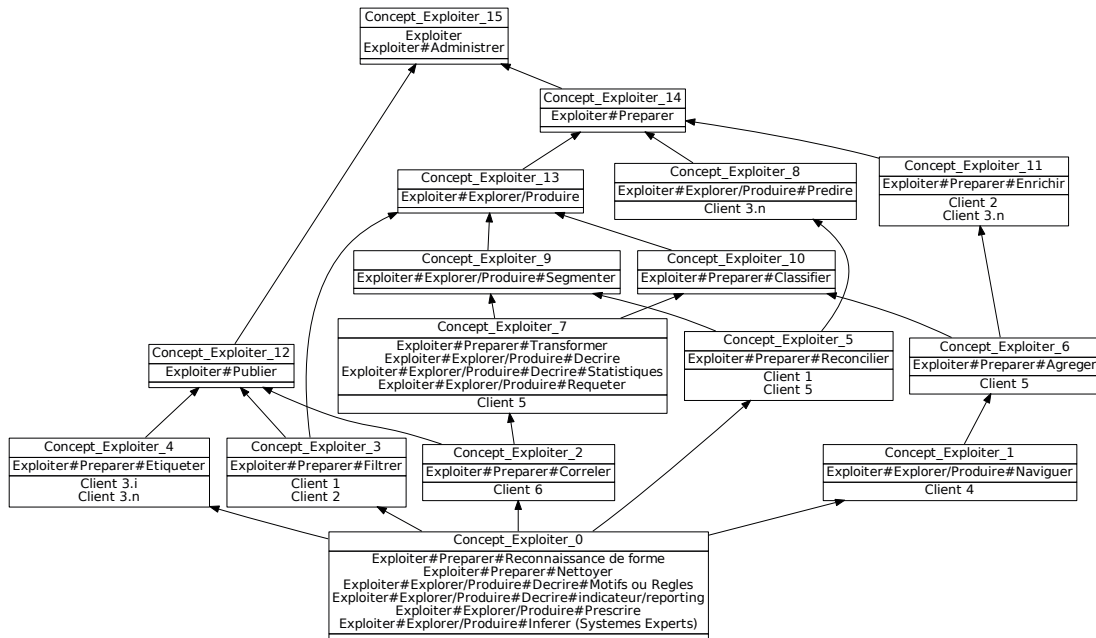
FIGURE 8.28: AC-Exploiter-simple
