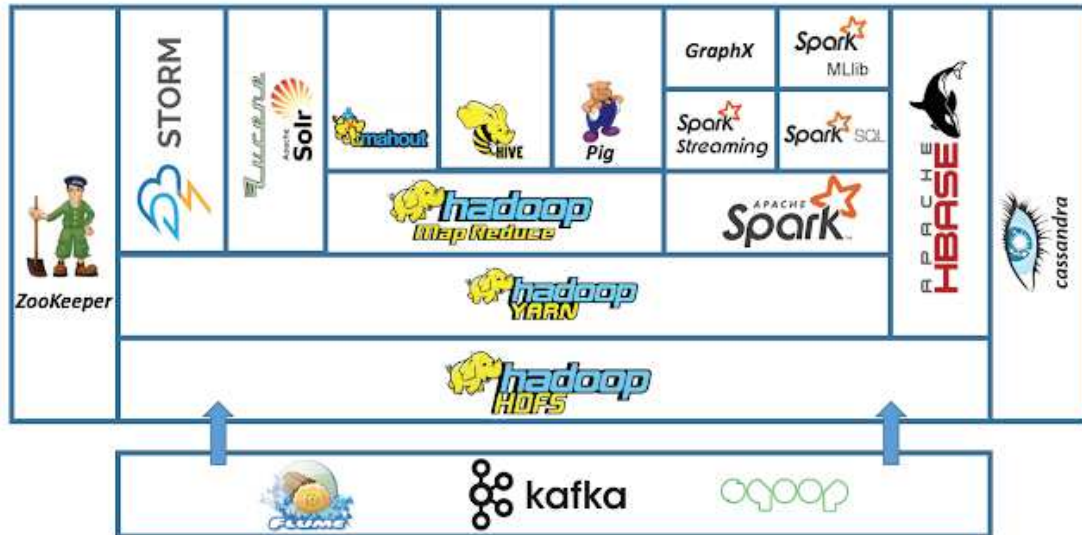
FIGURE 3.23: Un environnement Hadoop
