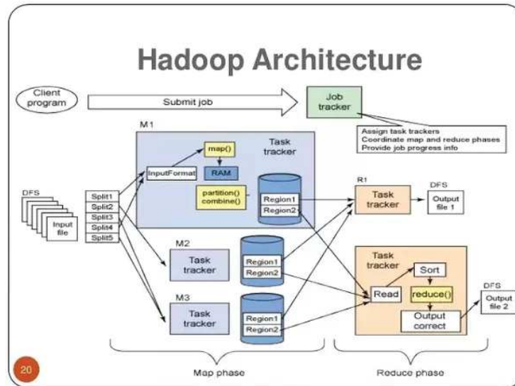
FIGURE 3.22: Architecture Apache Hadoop
