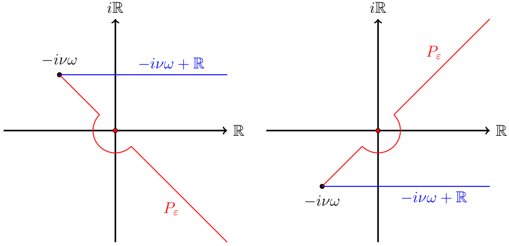
Figure I.3 – Paths of integration for z \mapsto e^{-z}/z in (I.65) and (I.66). On the left: \text{Im}(-i\nu\omega > 0) , which implies that y_1 < x_1 (the point of observation x is downstream of the source y ). On the right: \text{Im}(-i\nu\omega < 0) , which implies that y_1 > x_1 (the point of observation x is upstream of the source y ).
