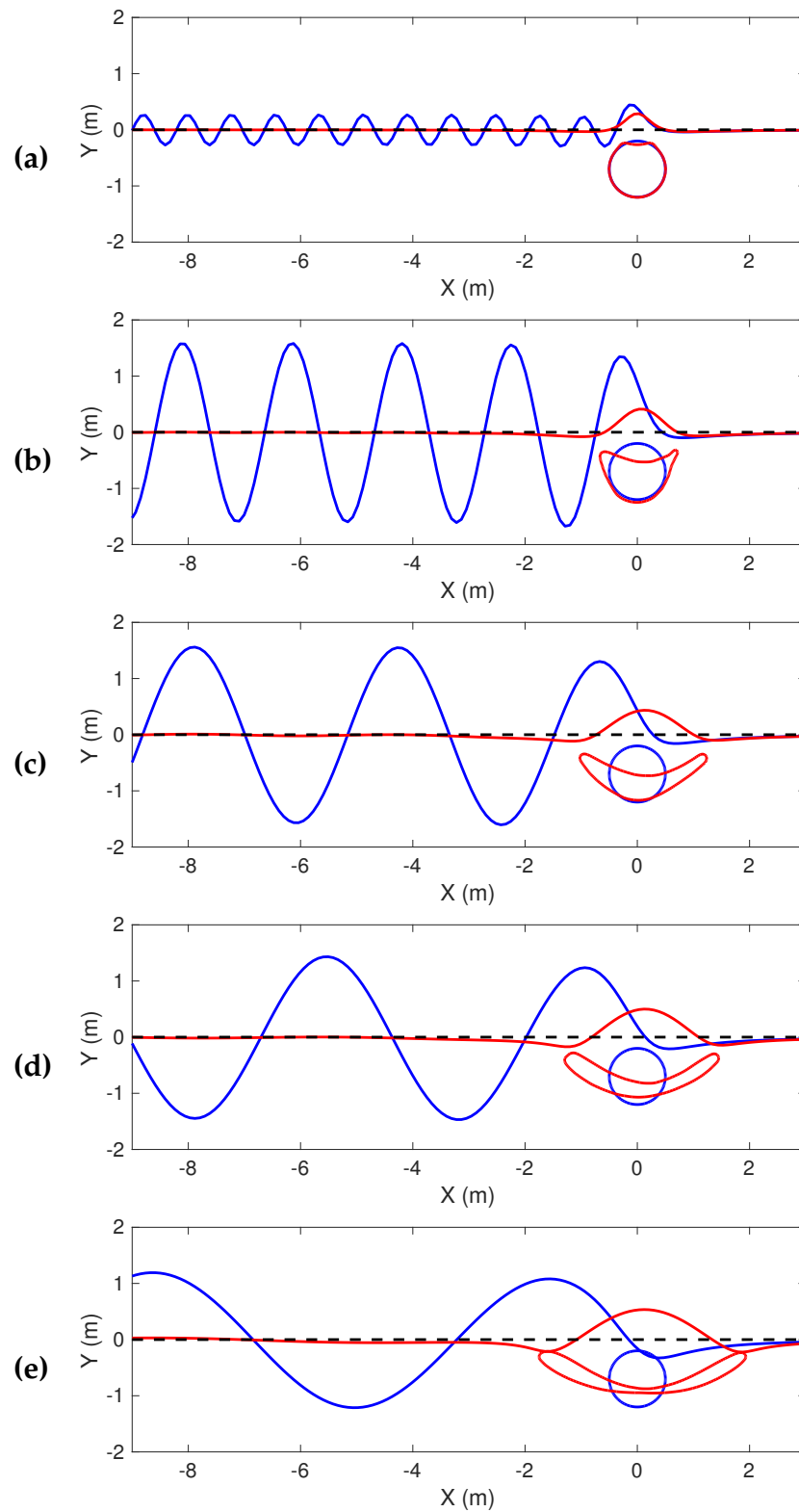
Figure IV.6 – Plots of the obstacles and corresponding free surface deformations. The blue curves represent the initial situation, the red curves represent the wake and obstacle at the end of the shape optimisation process. The horizontal dashed line represents the zero water level. The depth is fixed at 0.7; from top to bottom, we have: Fr = 0.4222, 0.6667, 0.9111, 1.0333, 1.2778
