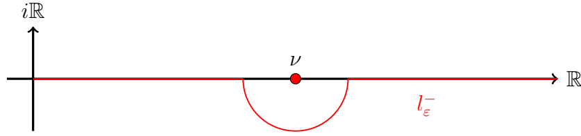
Figure I.2 – Path of integration for z \mapsto \frac{e^{-izw}}{z - \nu} in [50]
