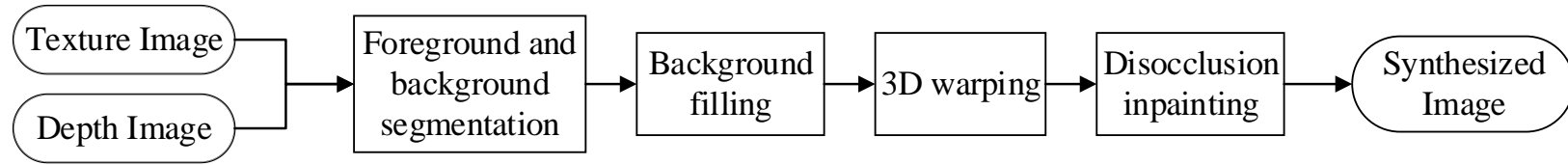
Figure 4.2: Block diagram of LDI
