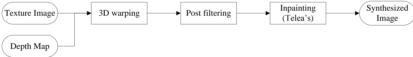
Figure 4.6: Block diagram of VSRS
