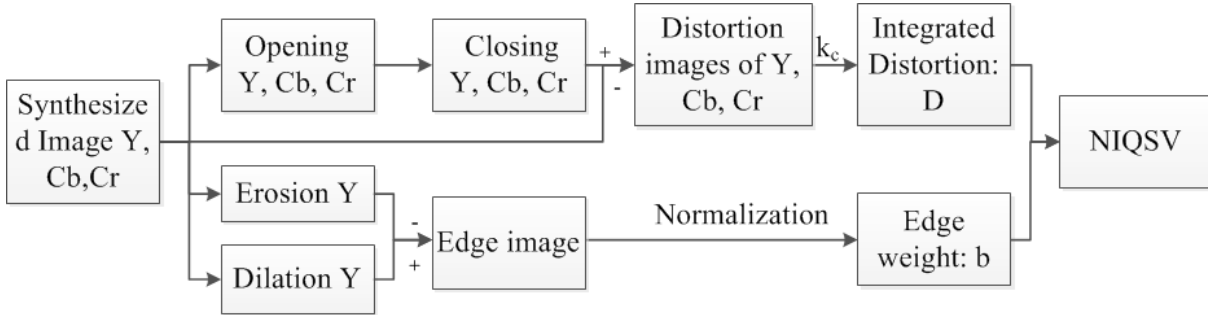
Figure 3.4: Block scheme of NIQSV
