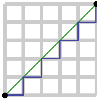
Figure 1.2 – Comparison of Manhattan Distance (blue) and Euclidean Distance (green)
