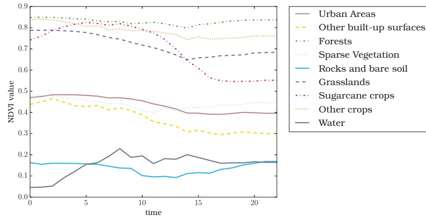
Figure 4.3 – TiSeLaC mean profiles per class (NDVI)
