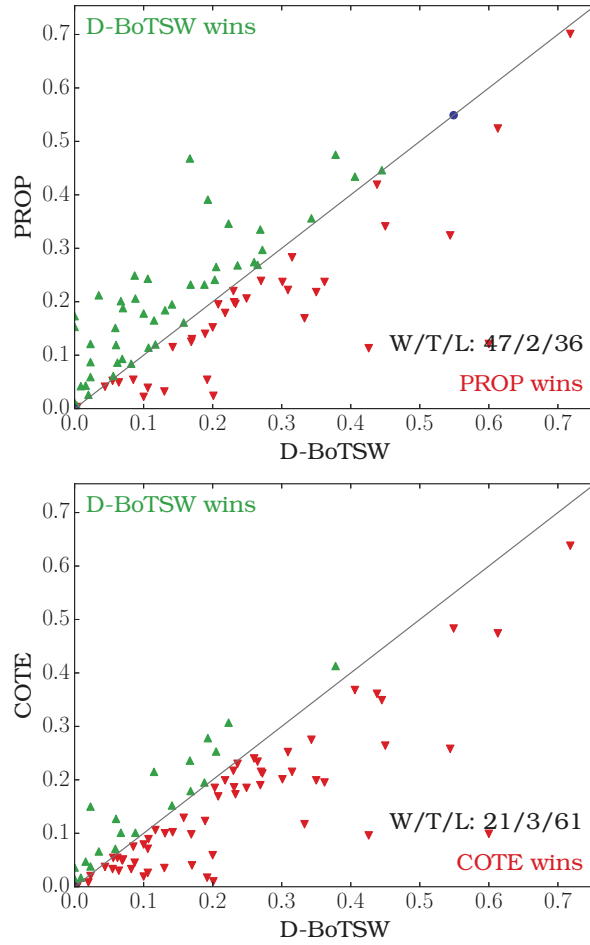
Figure 2.12 – Error rates for D-BoTSW ( \text{SSR} + \mathcal{L}_2 ) versus baseline ensemble classifiers (PROP and COTE).
