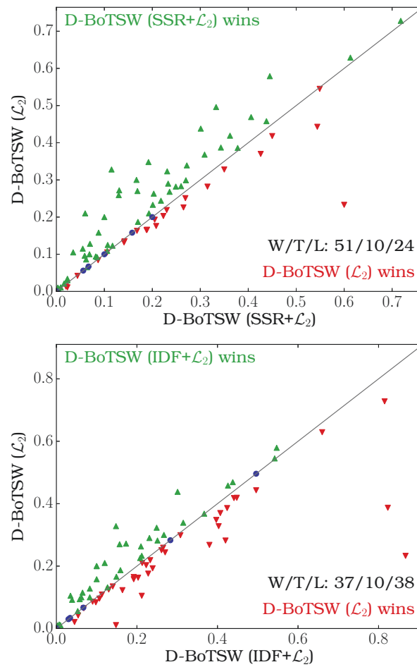
Figure 2.8 – Error rates of D-BoTSW with and without normalization.
