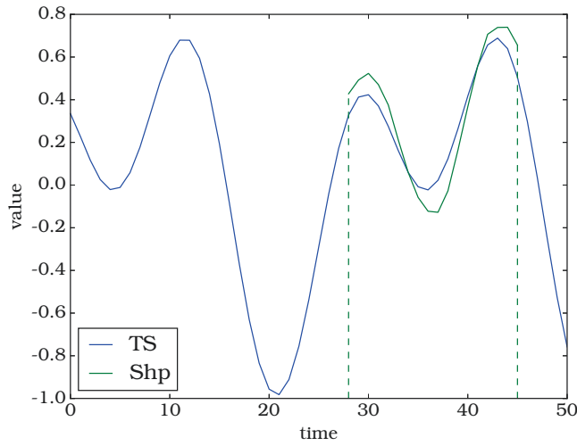
Figure 3.9 – Match between a time series \boldsymbol{x}_i and a shapelet \boldsymbol{s}_k (of length L = 18 ). Here j_k^* = 28 , i.e. the minimal distance between \boldsymbol{x}_i and \boldsymbol{s}_k is obtained for \tau_i^{j_k^*} = \tau_i^{28} . Thus \frac{\partial M_{i,k}}{\partial x_{i,j}} \neq 0 if j \in [j_k^*, j_k^* + L - 1] = [28, 45] , i.e. if j is one of the indices where \boldsymbol{x}_i matches with \boldsymbol{s}_k .
