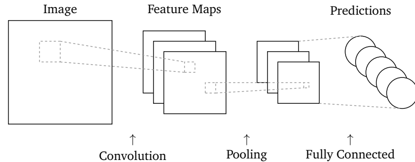
Figure 3.4 – Convolutional Neural Network overview, minimal example with three filters, five classes, and one layer of each type (convolution, pooling, fully connected).
