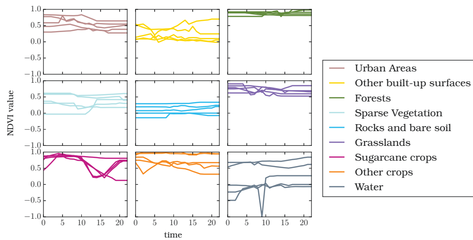
Figure 4.4 – Representation of five randomly selected time series per class from TiSeLaC dataset (NDVI)
