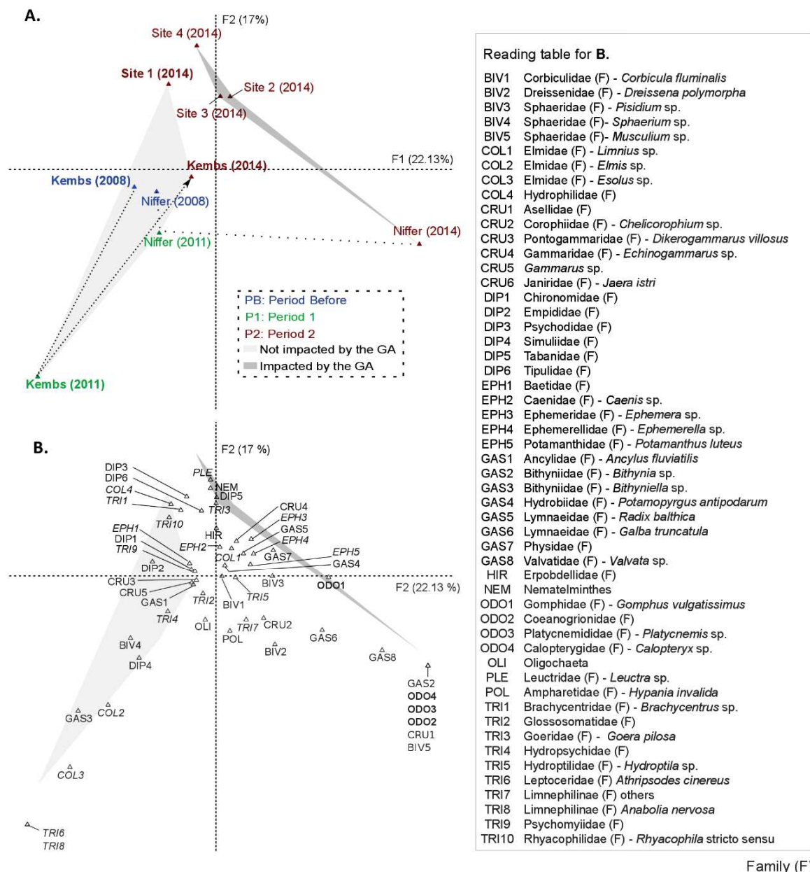
Figure 4.8: Factorial plane of a correspondence analysis based on all site data. A. The three periods are represented by different colours: PB in blue ( \blacktriangleleft December 2010), P1 in green (December 2010 \blacktriangleright ); i.e., after the gravel augmentation and the instream flow increase) and P2 in red (i.e., after the Q_{15} flood event in June 2013). Time trajectories are given for Niffer and Kembs site scores, whereas sites 1 (control, in bold), 2, 3 and 4, are each represented by a single point corresponding to the P2 data. B. Macroinvertebrate species observed in 2008, 2011 and 2014 (abundance data were \text{Log}_2(x+1) transformed). EPTC orders are represented in italic and Odonata in bold.
