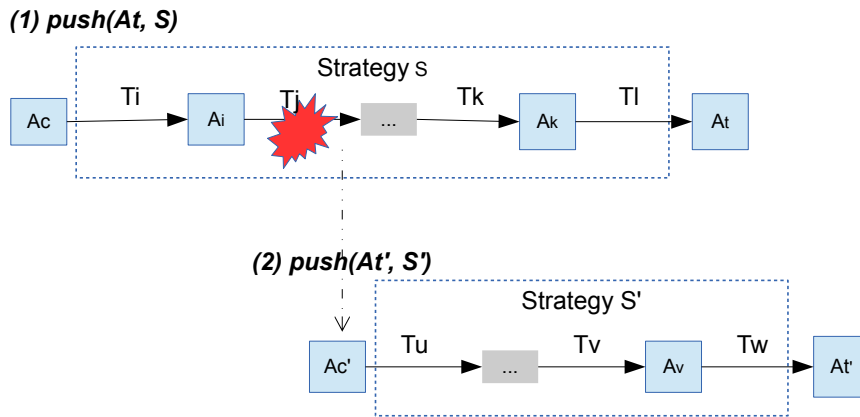
Figure 4.9: Management of failures at update time by adapting the strategy and the target
