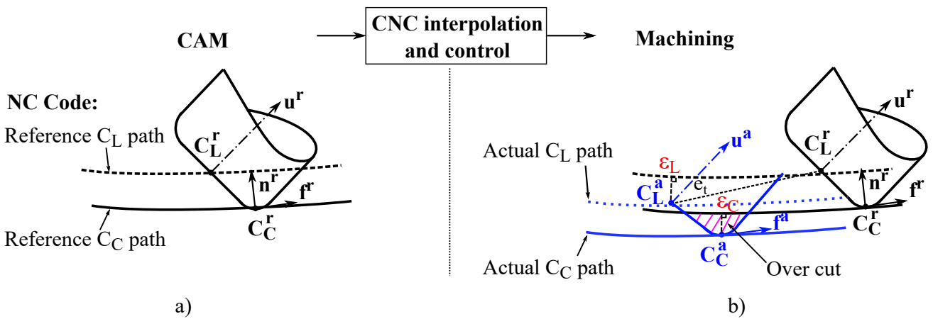
Figure 1.13: a) Reference tool positioning; b) Actual tool positioning with contour error
