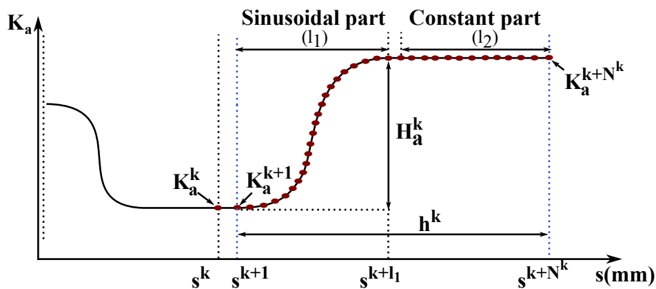
Figure 2.15: Gain prediction by predefined gain function
