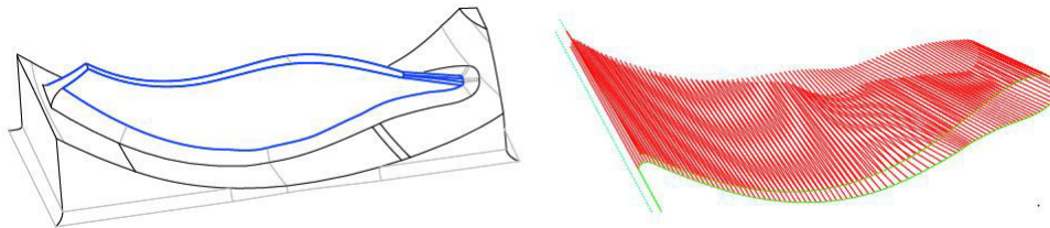
Figure 2.2: Definition of impeller surface and the machining trajectory [Pechard 2011]
