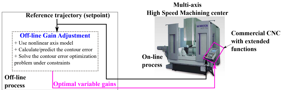
Figure 2.5: Proposed offline execution
