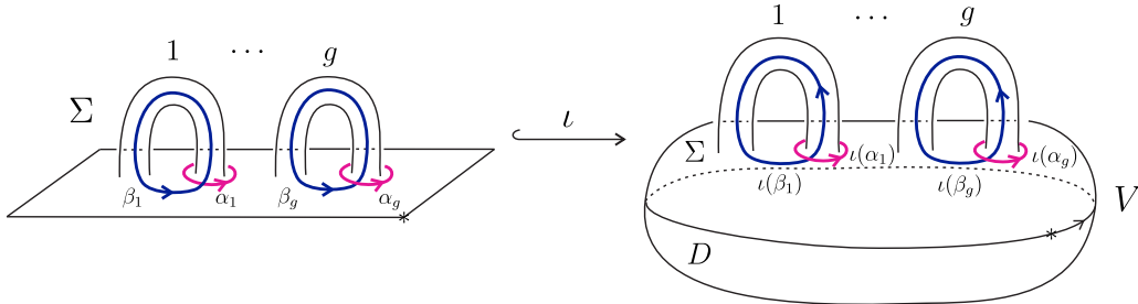
Figure 3.1: The inclusion \Sigma \hookrightarrow V .
