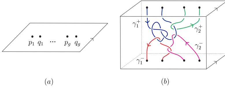
Figure 2.1: (b) bottom-top tangle of type (2, 2) in [-1, 1]^3 .
