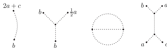
Figure 5.1: C -colored Jacobi diagrams of i\text{-deg} 0, 1, 2 and 2, respectively. Here C = \{a, b, c\}
