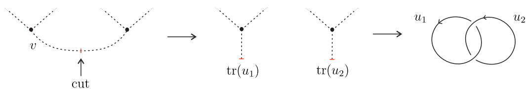
Figure 4.8: Starting the antidifferentiation process to realize v .
