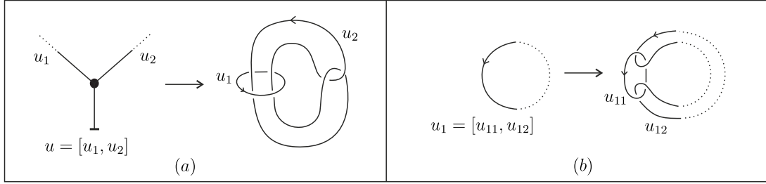
Figure 4.5: (a) Starting step and (b) recursive step.
