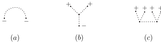
Figure 6.2: Tree-like Jacobi diagrams of \mathbf{a} -deg = 1.
