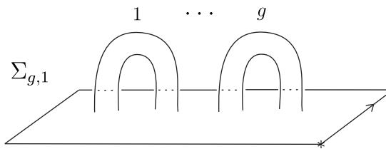
Figure 2.3: Surface \Sigma_{g,1} .
