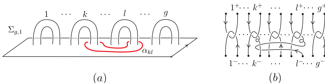
Figure 3.7: (a) Curve \alpha_{kl} and (b) bottom-top tangle presentation of c(t_{\alpha_{kl}}) .
