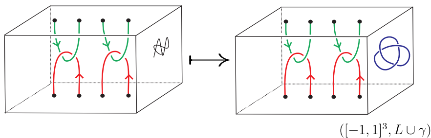
Figure 2.11: From (B, \gamma') to ([-1, 1]^3, L \cup \gamma) .
