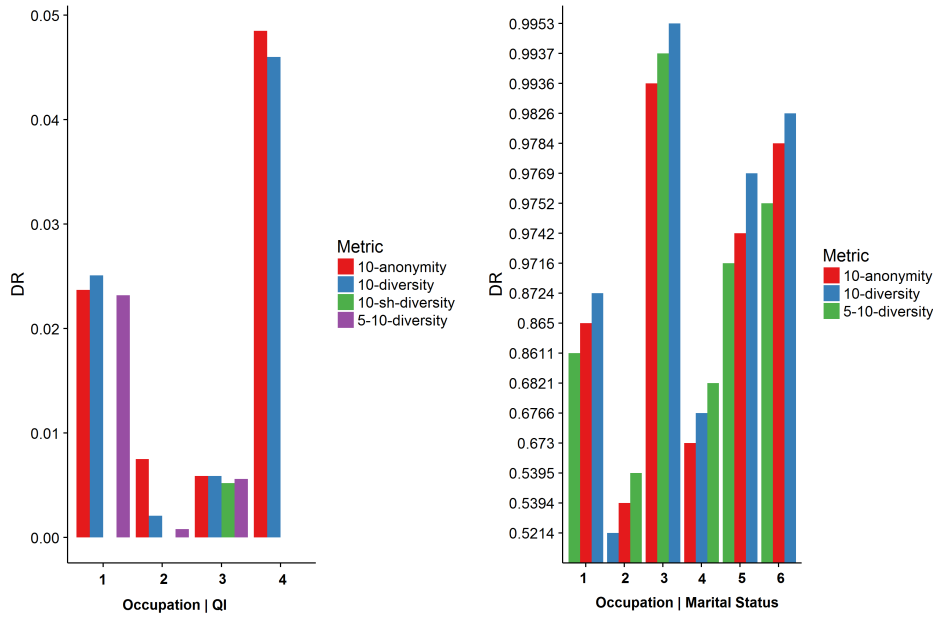
FIGURE 4.5: Homogeneity Attack measurements in the Adult dataset
