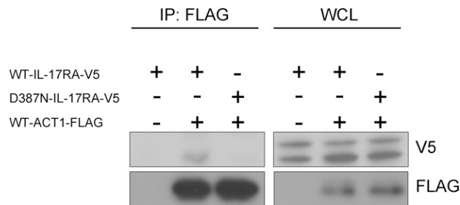
Fig. S2. The p.D387N IL-17RA allele impairs IL-17RA/ACT1 interaction. HEK293 cells were transiently transfected with a plasmid encoding FLAG-tagged ACT1 together with plasmids encoding V5-tagged WT-IL-17RA or D387N-IL-17RA. Whole-cell lysates (WCL) were subjected to immunoprecipitation with anti-FLAG antibody. Western blot analysis was performed with anti-FLAG and -V5 antibodies.
