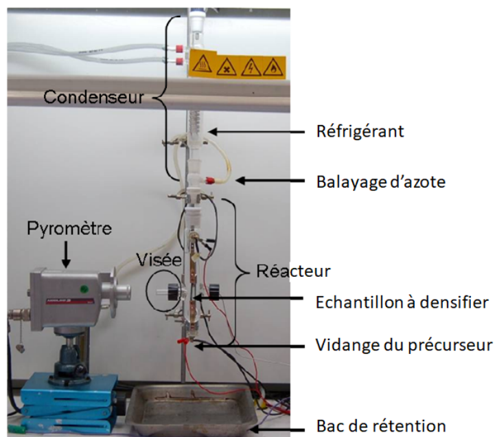
FIGURE I.3.4 – Photo du mini-kalamazoo [Serre_2013]
