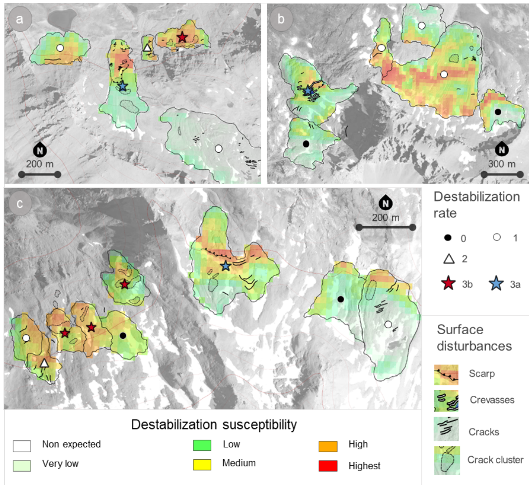
FIGURE 4.4: Examples of destabilization susceptibility map.
