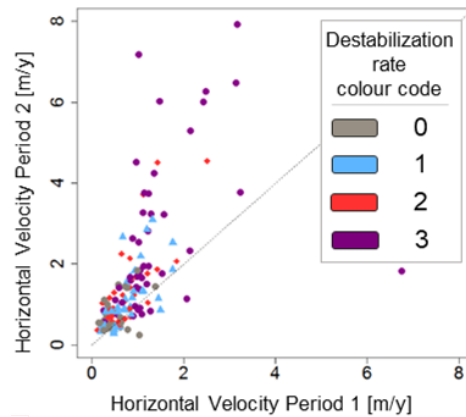
FIGURE 6.1: Fastest observable boulder velocity per rock glacier according to their destabilization rating in in the period 1 (2000 – 2004 to 2008 – 2009) and period 2 (2008 -2009 to 2012 -2013).
