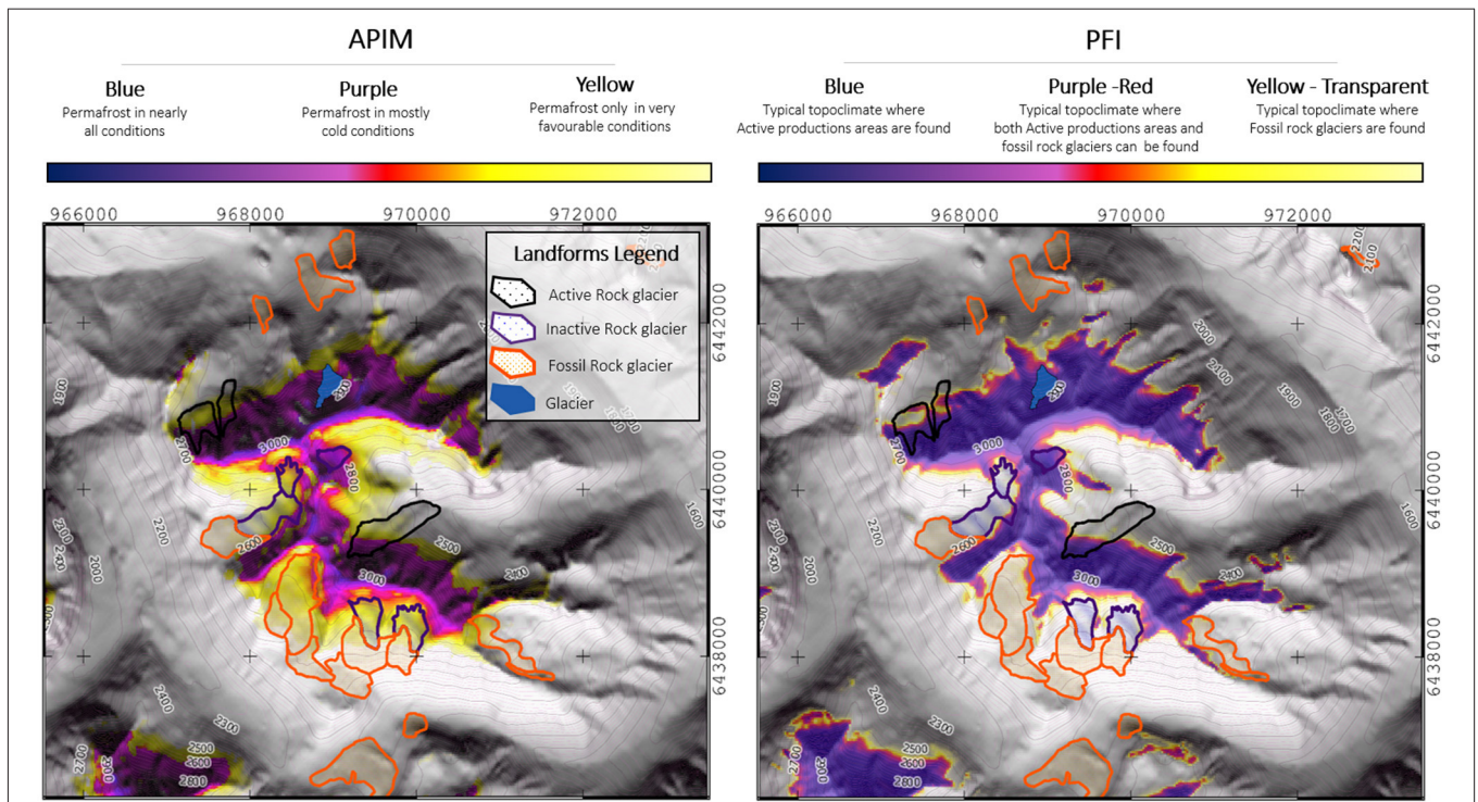
FIGURE 9 | Comparison between Alpine Permafrost Index Map (APIM) and Permafrost Favorability Index (PFI) in Massif du Combeynot. The PFI map is available as geotiff image in the Supplementary Materials.
