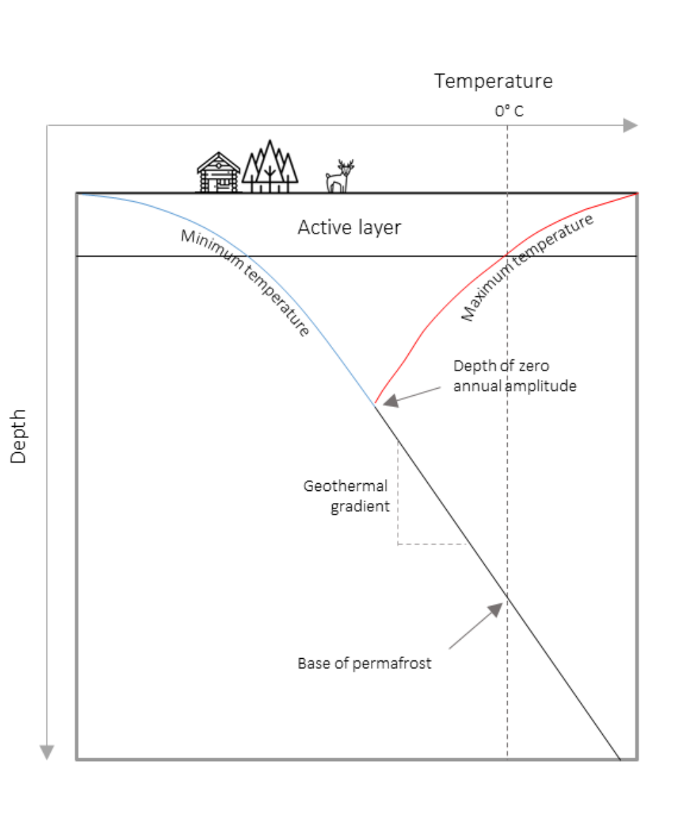
FIGURE 2.1: Conceptual scheme of the permafrost layers and characteristics (adapted from Osterkamp and Burn, 2003).
