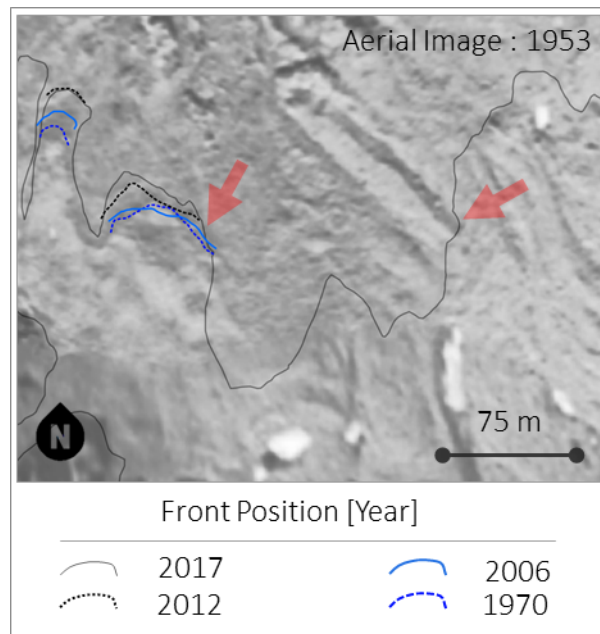
FIGURE 5.4: Evolution of the frontal position since 1970. Red arrows indicate the location of the western and eastern failures. It can be observed that the eastern failures was active already in 1953, while the western failure occurred on a spot only recently occupied by the rock glacier front.
