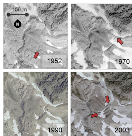
Figure 3. The evolution of the destabilization of the Pierre Brune rock glacier. The destabilization evidence, in this case a crack observable since 1952, evolved to a crevasse, observable in 1970. Afterwards, the landform was stable for 20 years as destabilization evidence did not further evolve. Between 1990 and 2003 the rock glacier experienced severe destabilization with the formation of new crevasses and a scarp at the location of the 1952 crack.
