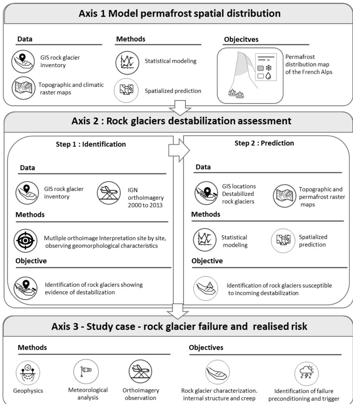
FIGURE 2.17: General workflow of the PhD project based on the three research axis, with specified objectives and methodologies.
