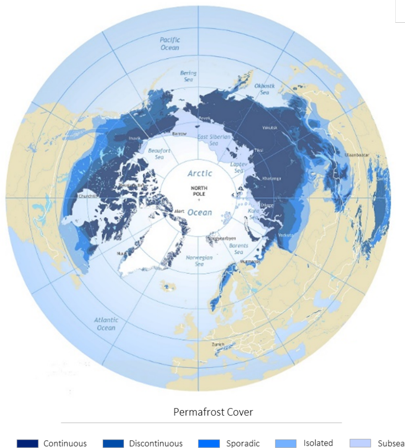
FIGURE 1.2: International Permafrost Association permafrost distribution map in the Northern Hemisphere (Brown et al., 1997).
