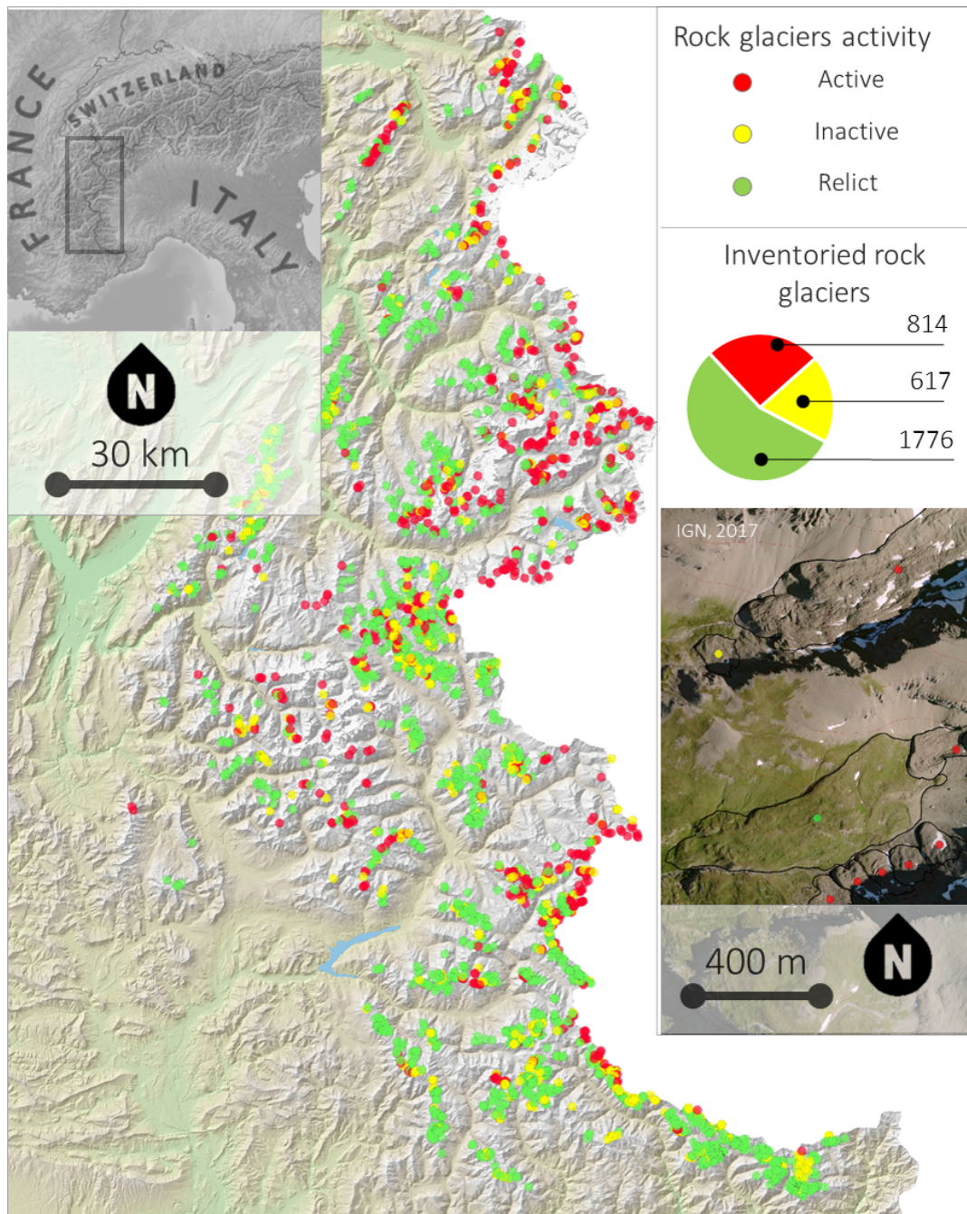
FIGURE 2.16: Rock glacier inventory as provided by the RTM
