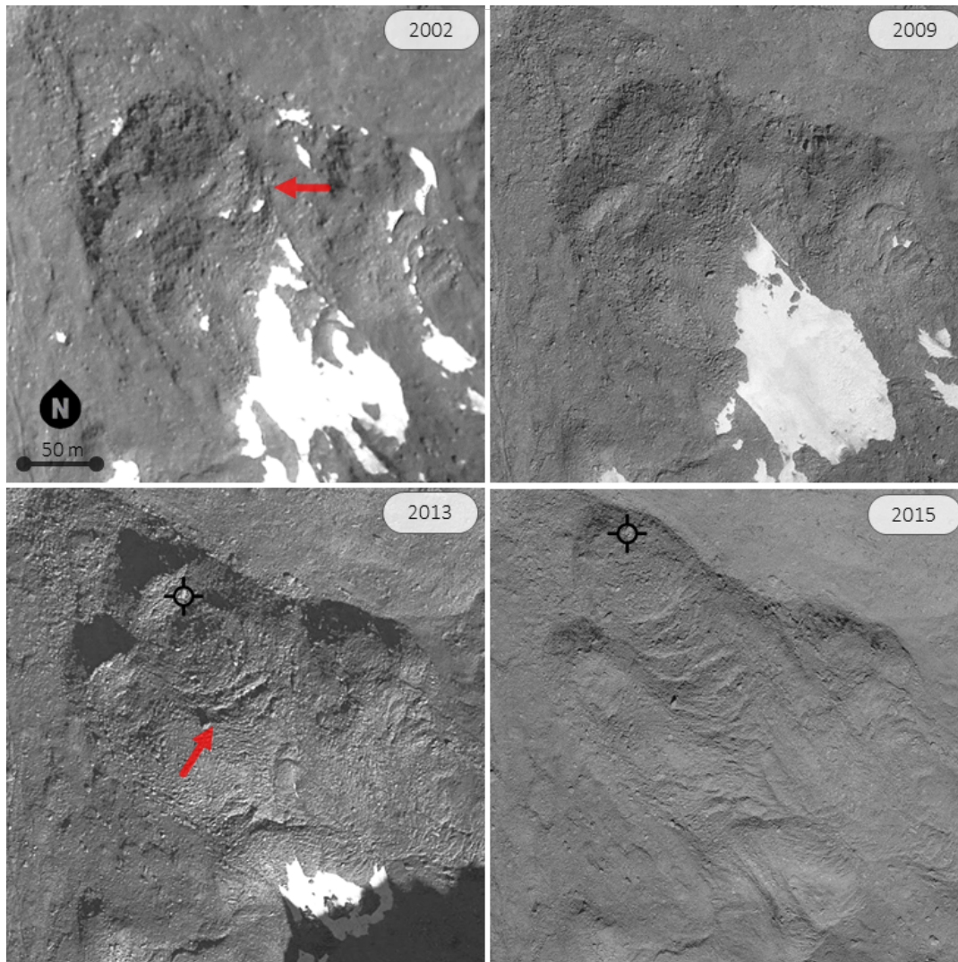
FIGURE 2.11: Example of rock glacier destabilization from the southern French Alps. A slightly pronounced scarp and cracks were observable since 2002 (red arrow) and slowly evolving until 2009. In 2013 the morphology two large crevasses were observable (red arrow). At this point the destabilization started, causing a displacement, measured on the black target on these orthoimages, of about 40 meters in two years
