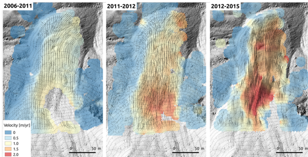
FIGURE 2.6: Spatial and temporal variability of permafrost creep on the Laurichard rock glacier of the Laurichard obtained with high resolution DEMs comparison (Bodin et al., 2018).
