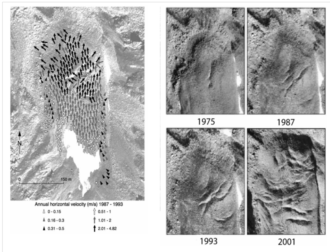
FIGURE 2.13: Creeping pattern of a destabilized rock glacier and evolution of surface disturbances, presented in Roer et al. (2008).
