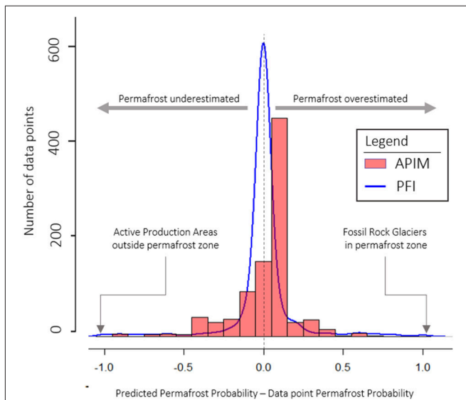
FIGURE 10 | Comparison between the residuals on our inventory with respect to Alpine Permafrost Index Map (APIM) and Permafrost Favorability Index (PFI). Since the PFI is calibrated on this inventory, residual distribution is not surprisingly centered to zero.
