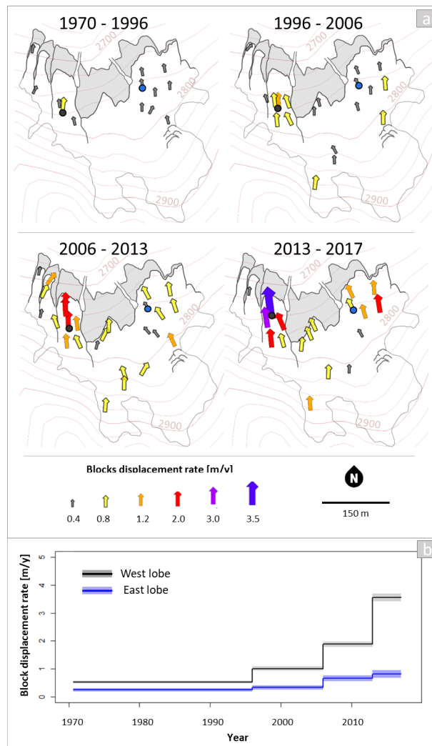
Figure 6. Overview of the historical dynamics of the Lou rock glacier presented as evolution of surface displacement rates retrieved by manual feature tracking on historical aerial imagery. In panel b is presented the graph of the evolution of the displacement rate on two boulders, one for the western lobe and one for the eastern lobe. Shaded areas size represent the mean error evaluated by apparent movements on stable areas. Boulder locations is identified by a dot in the maps in panel a.
