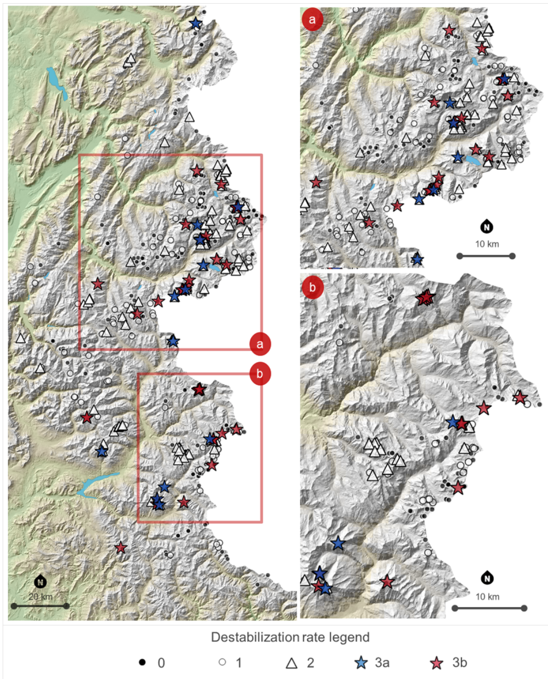
FIGURE 4.2: Active rock glaciers by destabilization rating in the French Alps, with focus on the Maurienne (a) and Ubaye (b) areas.
