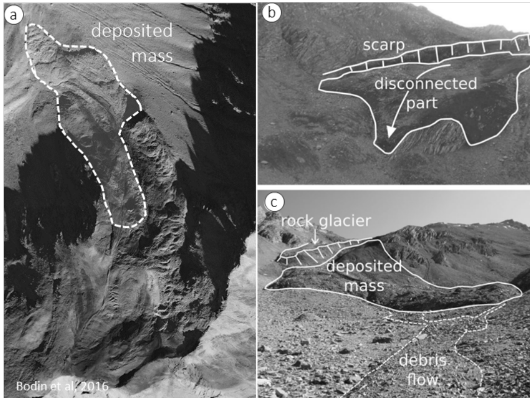
FIGURE 2.15: Bérard rock glacier collapse, from Bodin et al., 2016
