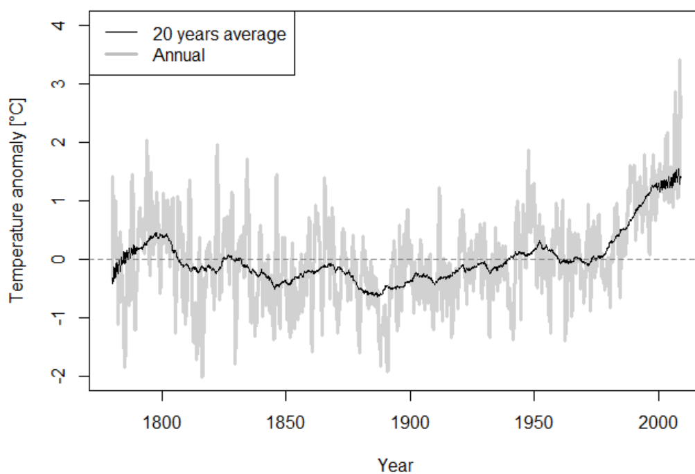
FIGURE 2.8: Mean annual temperature anomaly in the northern French Alps with respect to the period 1850 - 2006, obtained using Histalp data (Auer et al., 2007).
