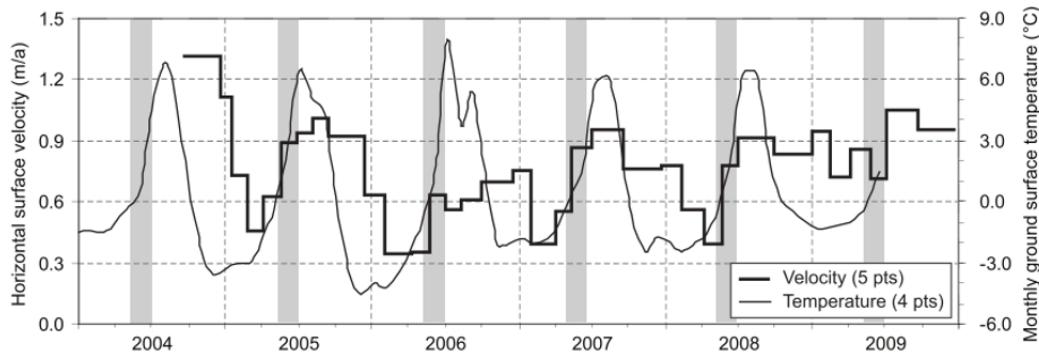
FIGURE 2.7: Temporal variability of the surface velocity at the seasonal scale in relation with ground temperature and snow melt periods (grey shaded areas), measured by Delaloye et al. (2010) at Becs-de-Bosson/Réchy rock glacier.
