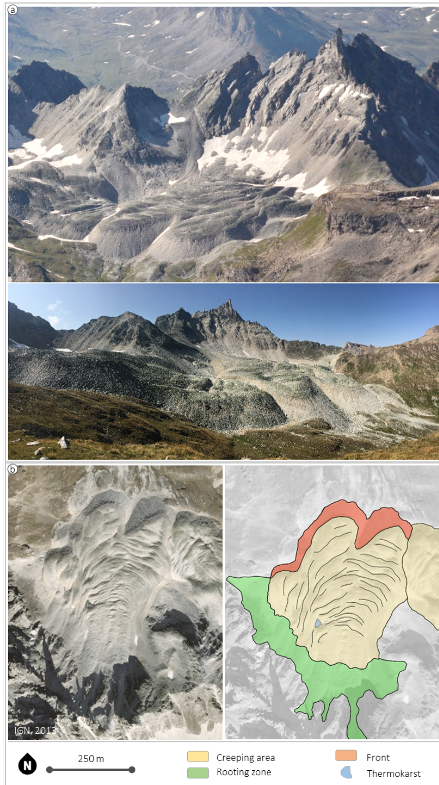
FIGURE 2.4: Overview of an active rock glacier, located in the Grande Sassiere natural reserve. On top (a) it is shown the appearance of the landform from the field, while on bottom (b) it is shown the appearance on orthoimage and general morphological characteristics.
