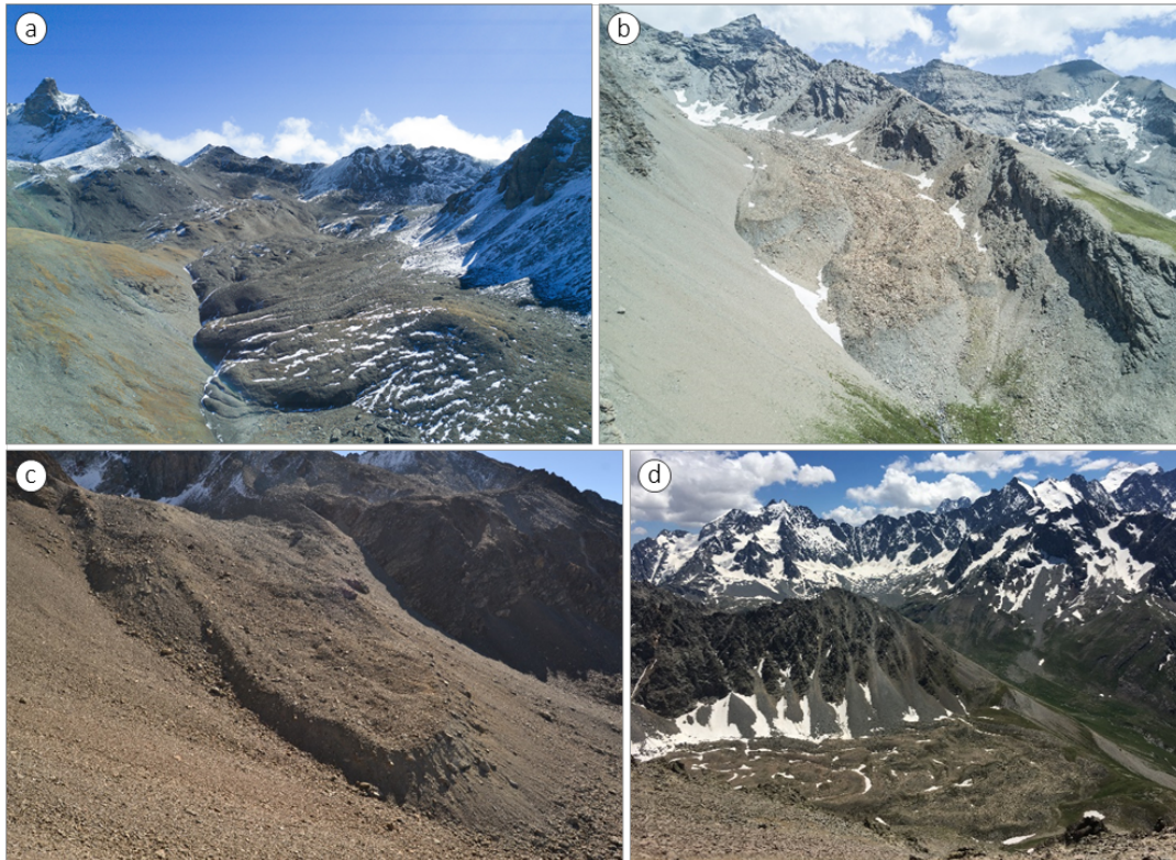
FIGURE 2.5: Different rock glaciers morphologies. Pebbly (a) and bouldery (b) rock glaciers. Inactive (c) and relict (d) rock glaciers.
