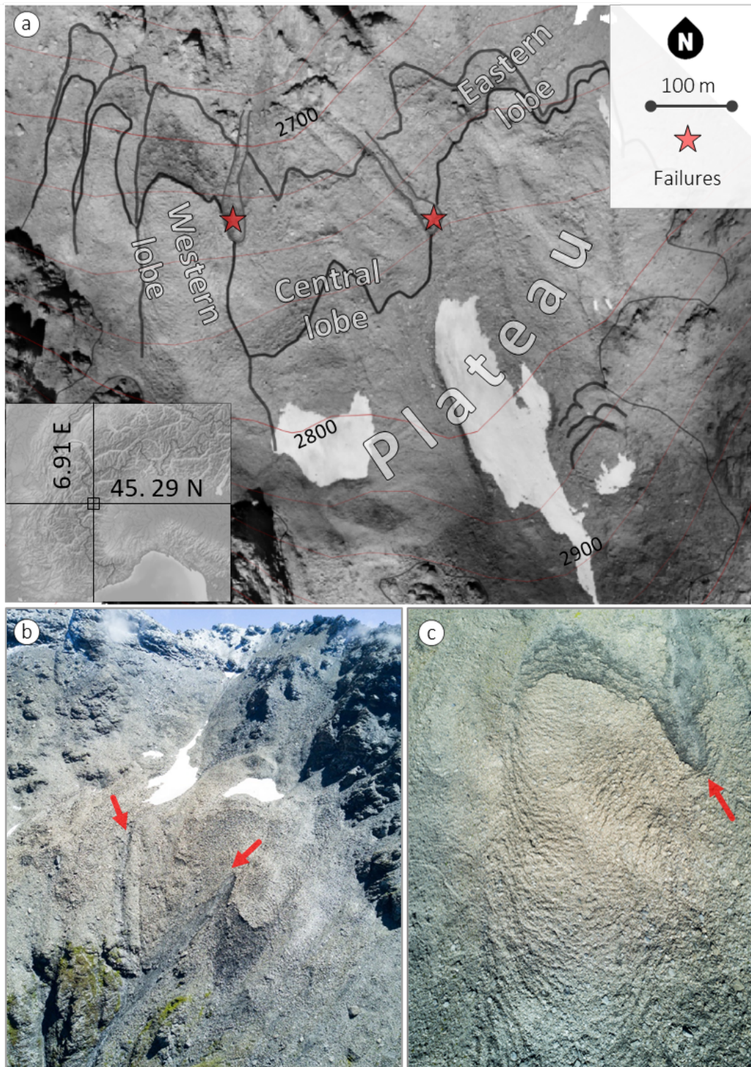
FIGURE 5.1: Presentation of the Lou rock glacier. In (a) overview of the landform on orthoimage. On bottom aerial images of the entire landform from South (b) and detail of the cracks on the western lobe (c). Red arrows indicate locations of the failures involved in the 2015 event.
