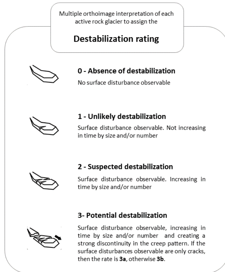
FIGURE 4.1: Destabilization rating, attributed by multiple orthoimages observations of the occurrence and evolution of the surface disturbances and creep pattern.
