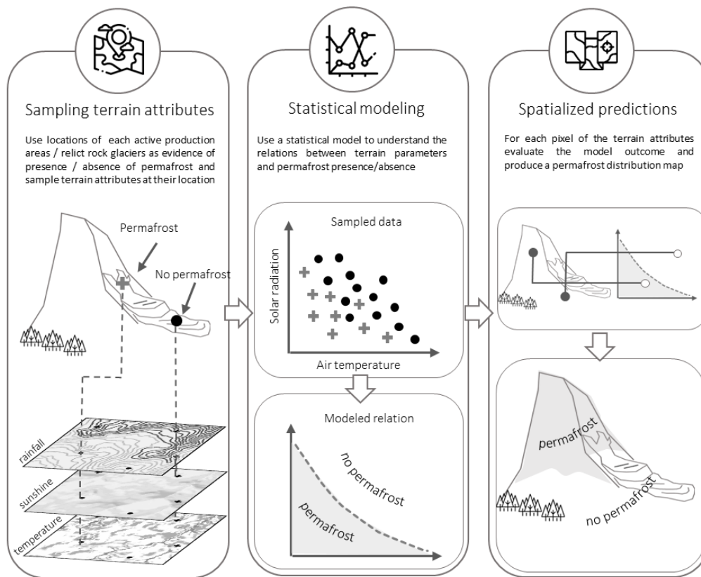
FIGURE 3.1: General workflow of statistical modeling applied to permafrost distribution prediction.
