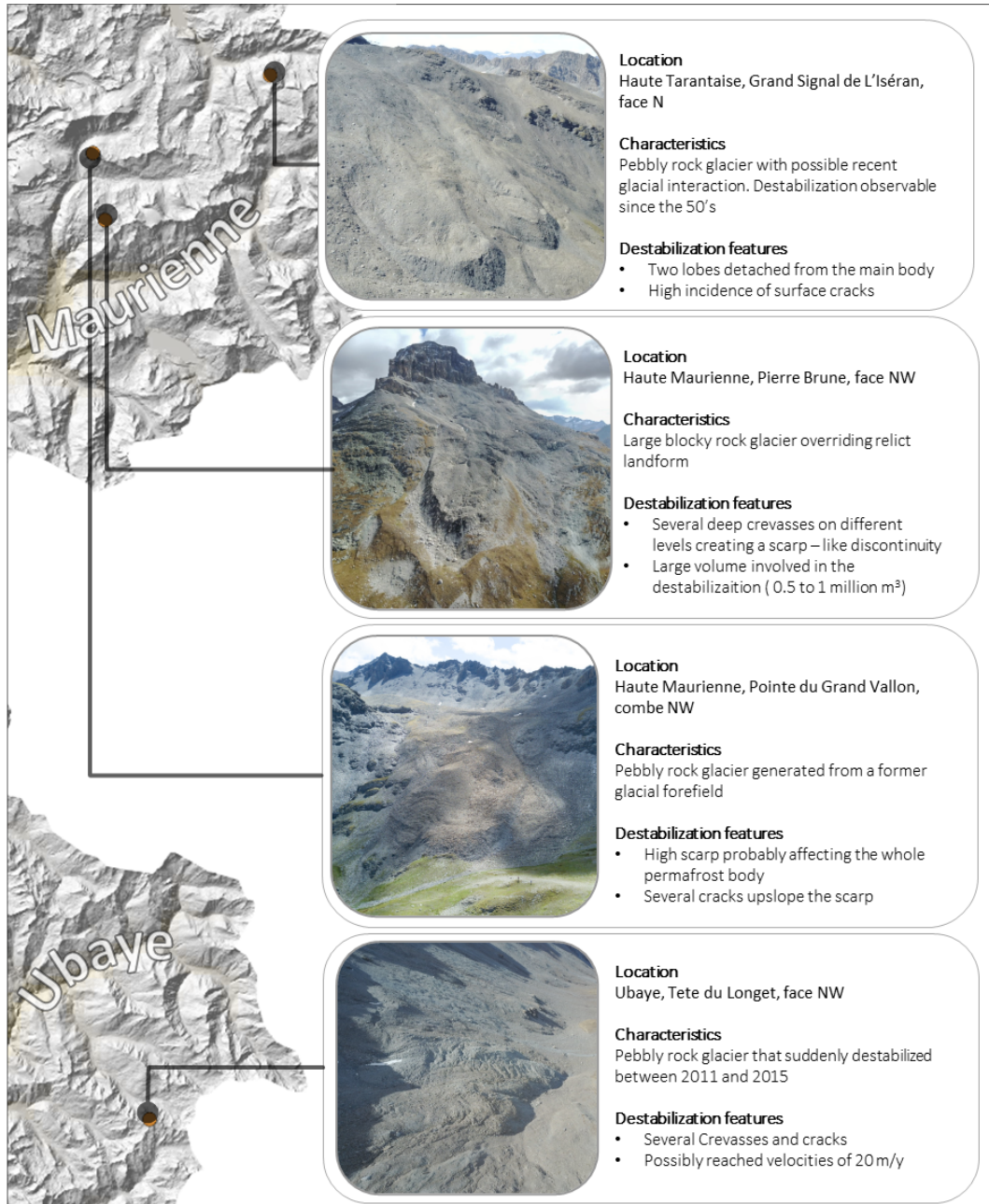
FIGURE 6.2: Localization and main characteristics of the destabilized rock glaciers that started to be monitored by yearly UAV surveys in summer 2017.
