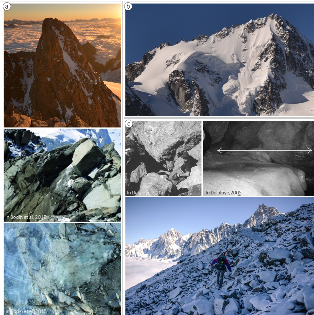
FIGURE 2.3: Examples of mountain permafrost in the European Alps. Bedrock permafrost (a) can be found in high mountain rockwalls and debris-free areas. Frozen water fills the joints of the bedrock. Frozen ground may cause the existence of hanging glaciers (b) by preventing basal sliding of the ice. Coarse debris (c) host permafrost at lower altitudes, thanks to the cooling effect due to ventilation of the active layer. Ice can be found within the ground matrix or in lenses.
