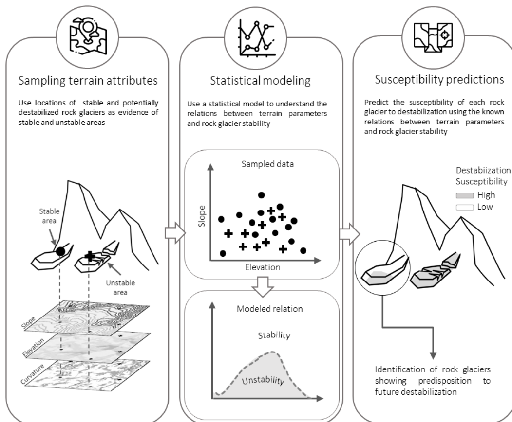
FIGURE 4.3: Conceptual scheme used to understand and predict rock glacier destabilization susceptibility.
