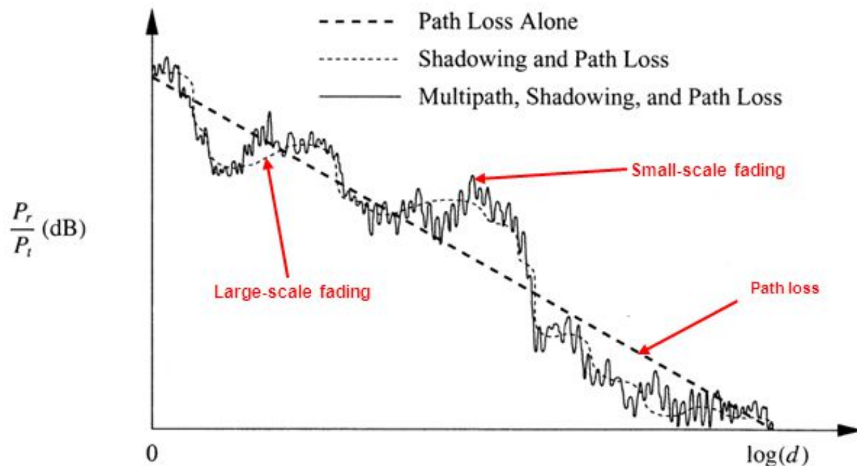
Figure 2.6: Fading phenomenon.
