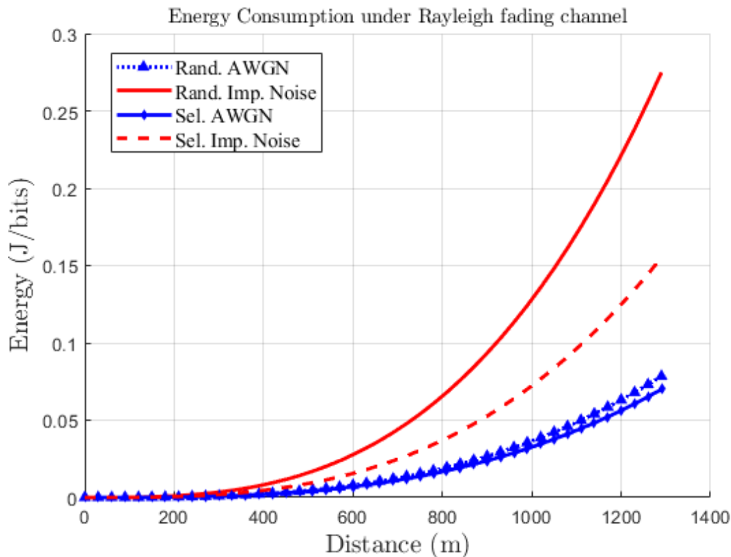
Figure 5.22: Energy consumption for \max-d_{min} precoding with FCSI under Rayleigh fading channel.
