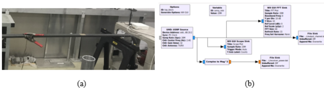
Figure 3.8: Setup for impulsive noise measurement in the laboratory.
