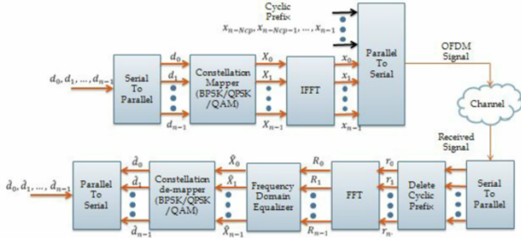
Figure 4.1: Architecture of a primary OFDM system [87].
