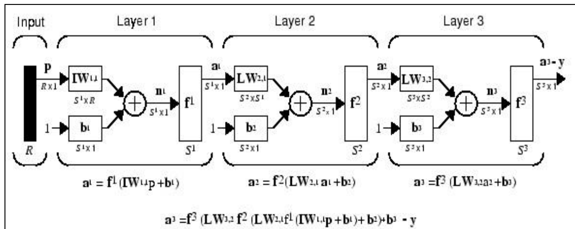
Fig. 10: MLP Diagram
