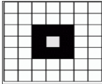
Fig. 53: Moore neighborhood
