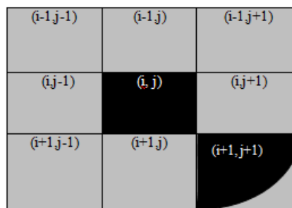
Fig. 61: Circular spreading
