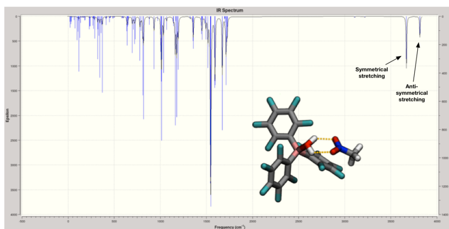
Figure B.2: Calculated IR spectrum for the most stable dimeric complex BCF:Nitromethane. Labels and arrows indicate the hydrogen stretching modes for each group of hydrogen bond.
