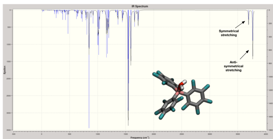
Figure B.3: Calculated IR spectrum for the BCF isolated. Labels and arrows indicate the hydrogen stretching modes.
