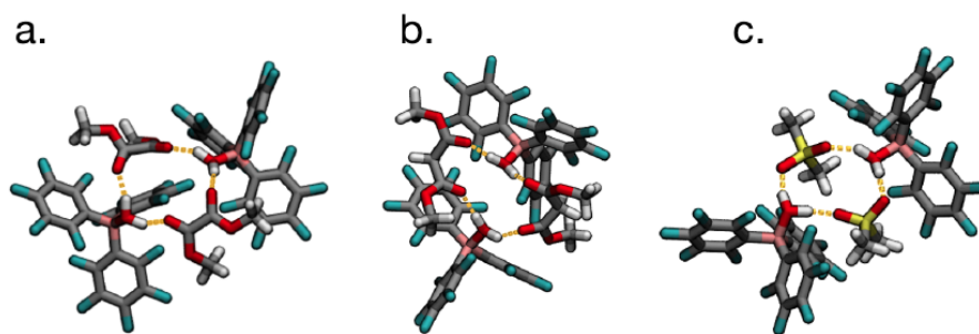
Figure B.6: DFT-optimized structures for the 2:2 self-assembly of BCF with: (a) dimethyl oxalate; (b) dimethyl malonate; and (c) dimethyl sulfone. These compounds correspond to entries 2-4 in Table 6.1.
