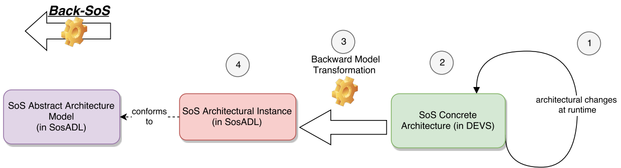
Figure 26 – Model discovery mechanism for SoS software architectures.
