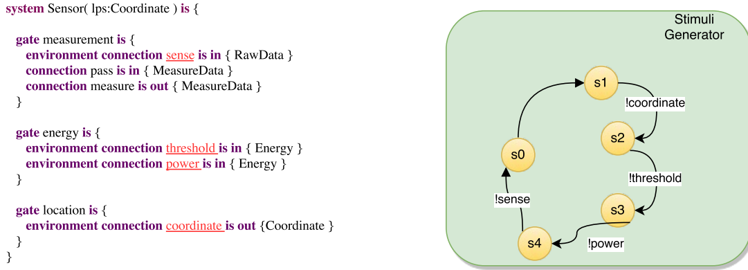
Figure 38 – Illustration of how an automaton is derived from SoSADL system specification to create a functional stimuli generator.
