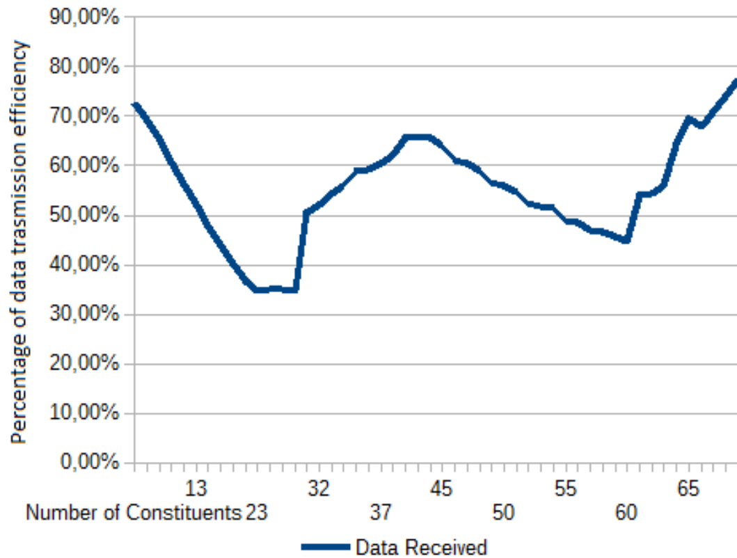
Figure 14 – Relation between data received in one or more gateways and SoS scale.
