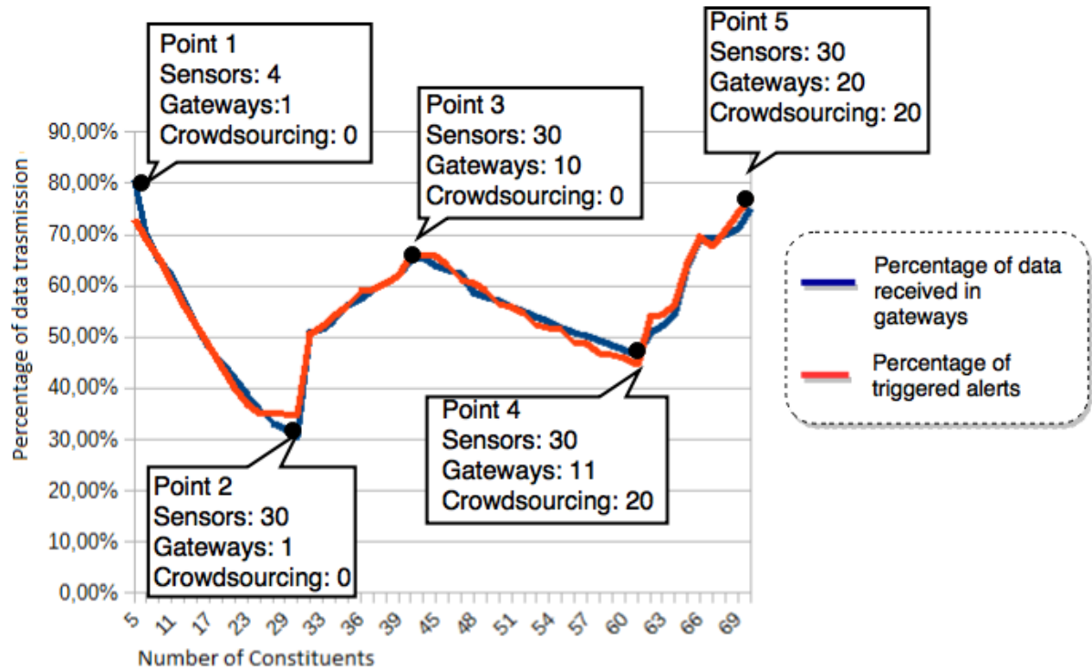
Figure 13 – Relation between percentage of data received in gateways and alerts triggered.
