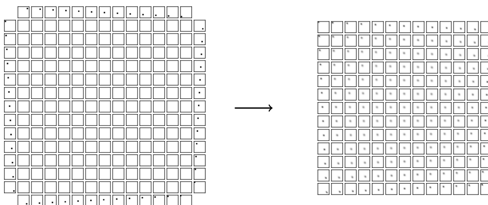
Figure 11.6: Left: boundary conditions which are supposed to look like Dirac masses. In practice, each probability distribution on the boundary is non zero on 4 = 2 \times 2 points of the grid \mathcal{G}_D^c \times \mathcal{G}_D^c . Right: solution of the Dirichlet problem with N = 13 , M = 17 . As one can see, the solution of the Dirichlet problem takes values in only very peaked probability distributions.
