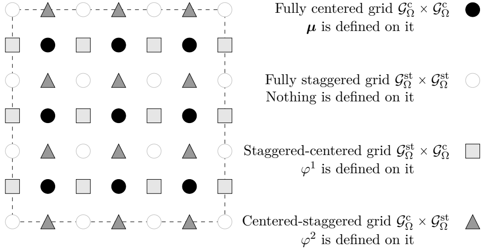
Figure 11.1: Example of the different grids considered on \Omega for the case N = 3 . We mention that the boundary values \mu are defined on the intersection of the staggered-centered and centered-staggered with the boundary of \Omega (displayed as a dashed line).
