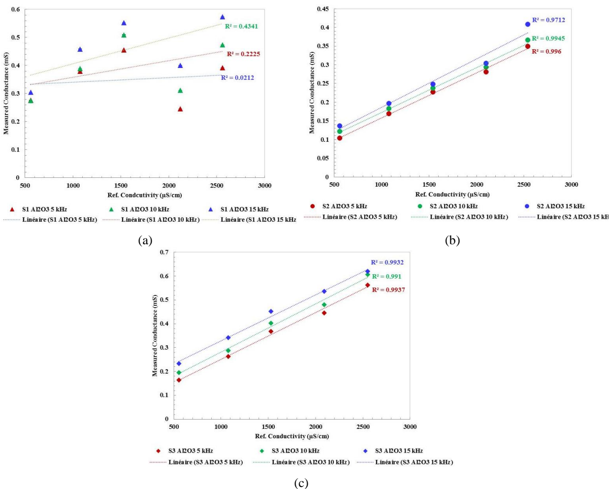
Figure 2-17: The response of the S1, S2 and S3 sensors under the considered five conductivity solutions at 5 kHz, 10 kHz and 15 kHz supply frequencies. Error bars are added in the plots, but not visible due to the small uncertainties.
