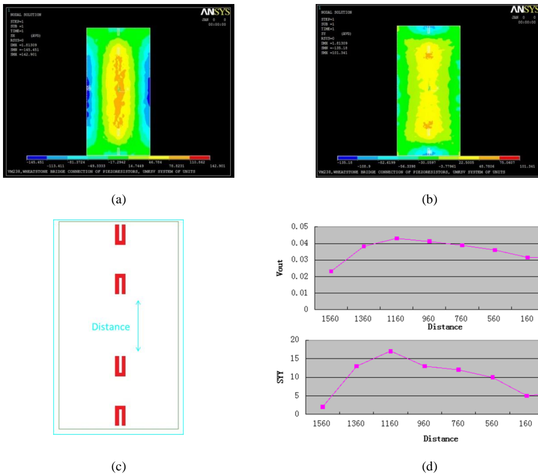
Figure Apn- 1: Example of FEM simulation results performed on the rectangular-shaped pressure sensor. The two upper contour plots show the distribution of the (a) S_{xx} and (b) S_{yy} stress components, (c) resistors distance on the membrane and (d) the lower right side curves show the effect of the position of the central resistances on the voltage at the output of the Wheatstone Bridge (dimensions are expressed herein micrometers).
