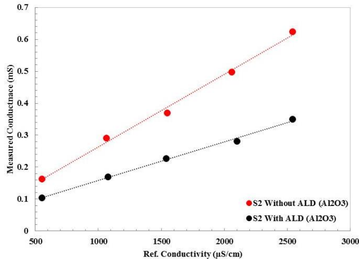
Figure 2-18: Conductivity sensor response at 5 kHz with and without coating layer made of \text{Al}_2\text{O}_3
