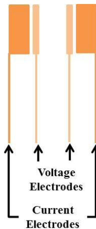
Figure 2-12: Current and voltage electrodes of the conductivity sensor
