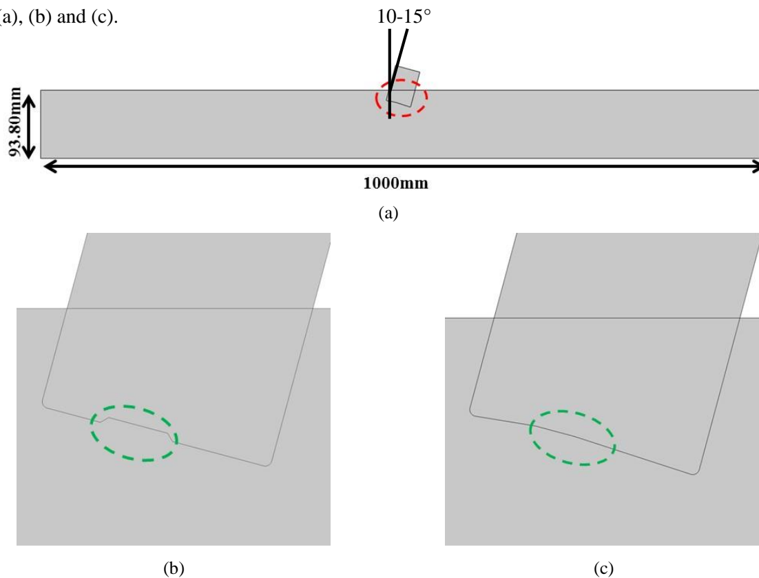
Figure 4-31: (a) The picture of the round-edged sensor node tilted at 15^\circ with respect to the normal and inserted into a water pipe, (b) the sensor node head chamfered with a 0.5 mm radius and (c) 1 mm radius.
