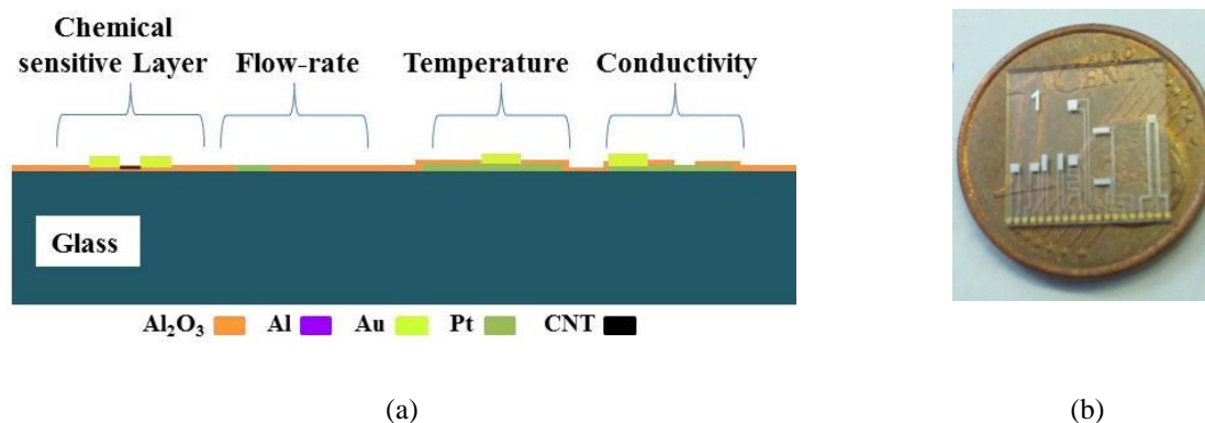
Figure 2-1: (a) Cross-section view of the multi-parameter sensor chip based on a glass substrate and (b) fabricated multi-parameter sensor chip on a glass substrate
