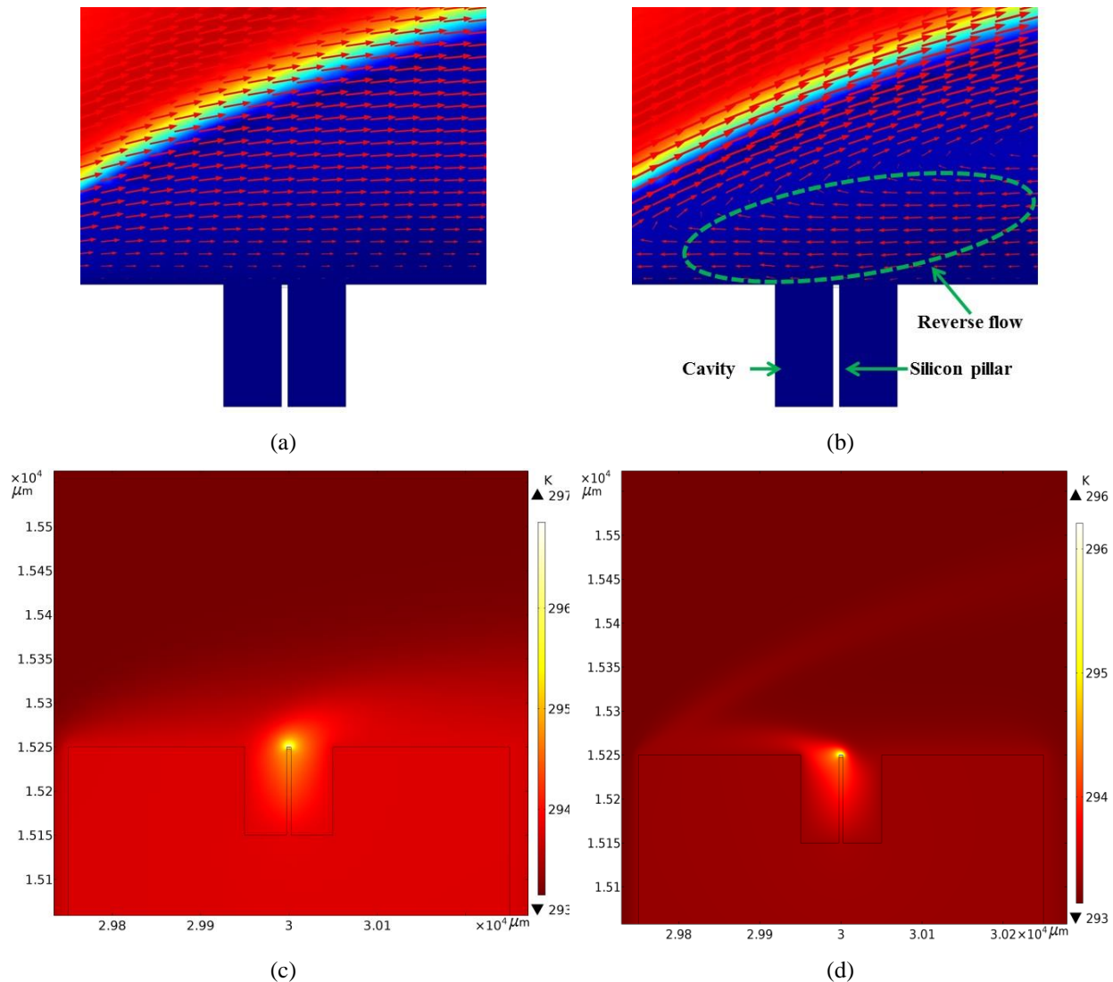
Figure 4-29: (a) Normal velocity profile for different fluid velocities, (b) reverse flow at the resistor vicinity causing the anomalous thermal behaviour within the velocity range highlighted by black circles in Figure 4-16 and Figure 4-25, (c) normal temperature profile and (d) the effect of reverse flow on the sensor temperature profile (flow direction is from left to right).
