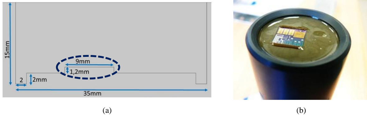
Figure 4-30: (a) The schematic diagram of the sensor node with dimensions and (b) photo of the real sensor node embedding the MPSC.
