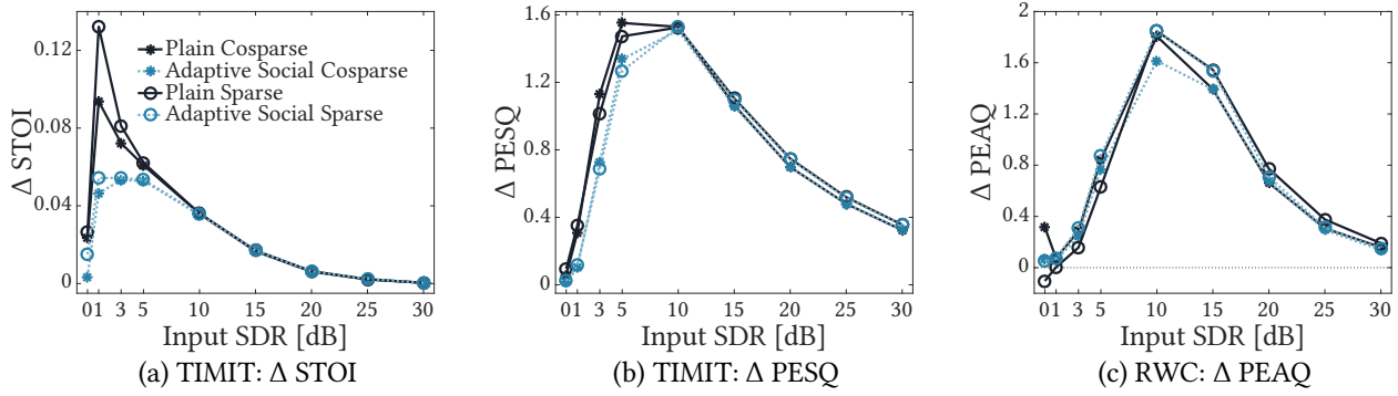
Figure 6.10 – Declipping: Objective Quality and Intelligibility Results
