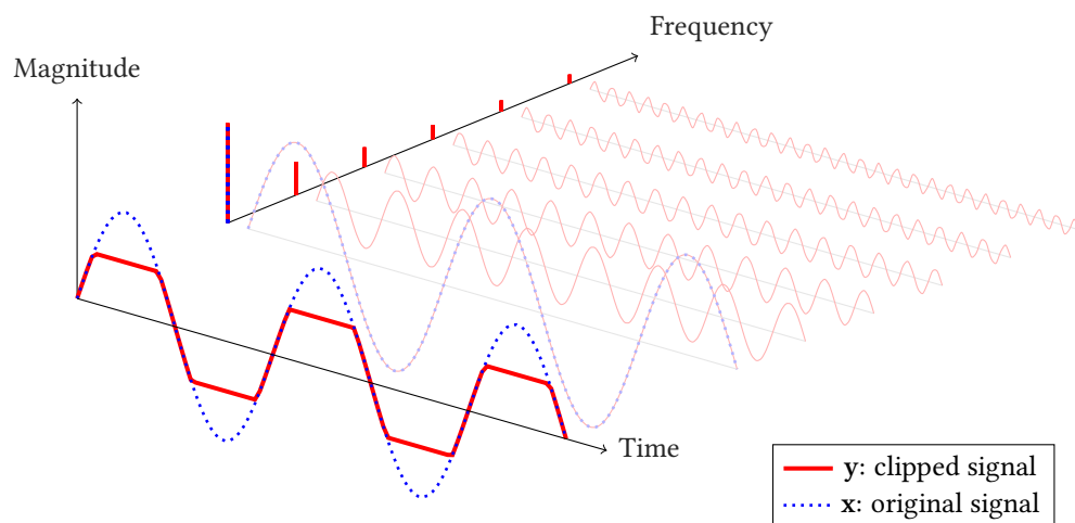
Figure 6.2 – Harmonic distortion
