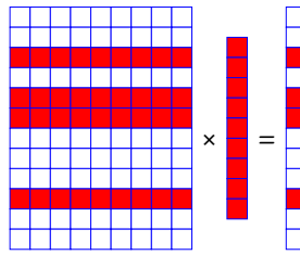
Figure 2.2 – Cosparse representation
