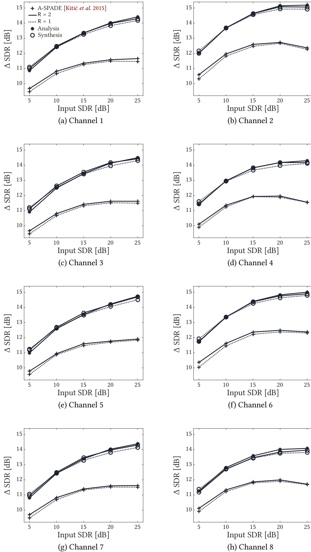
Figure 6.18 – VoiceHome2: Multichannel speech declipping (Numerical results \Delta \text{SDR} [dB])
