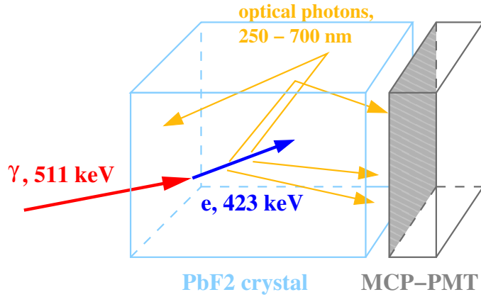
Figure 3.1: Schematic view of the 511 keV gamma detector with \text{PbF}_2 crystal using Cherenkov radiation.
