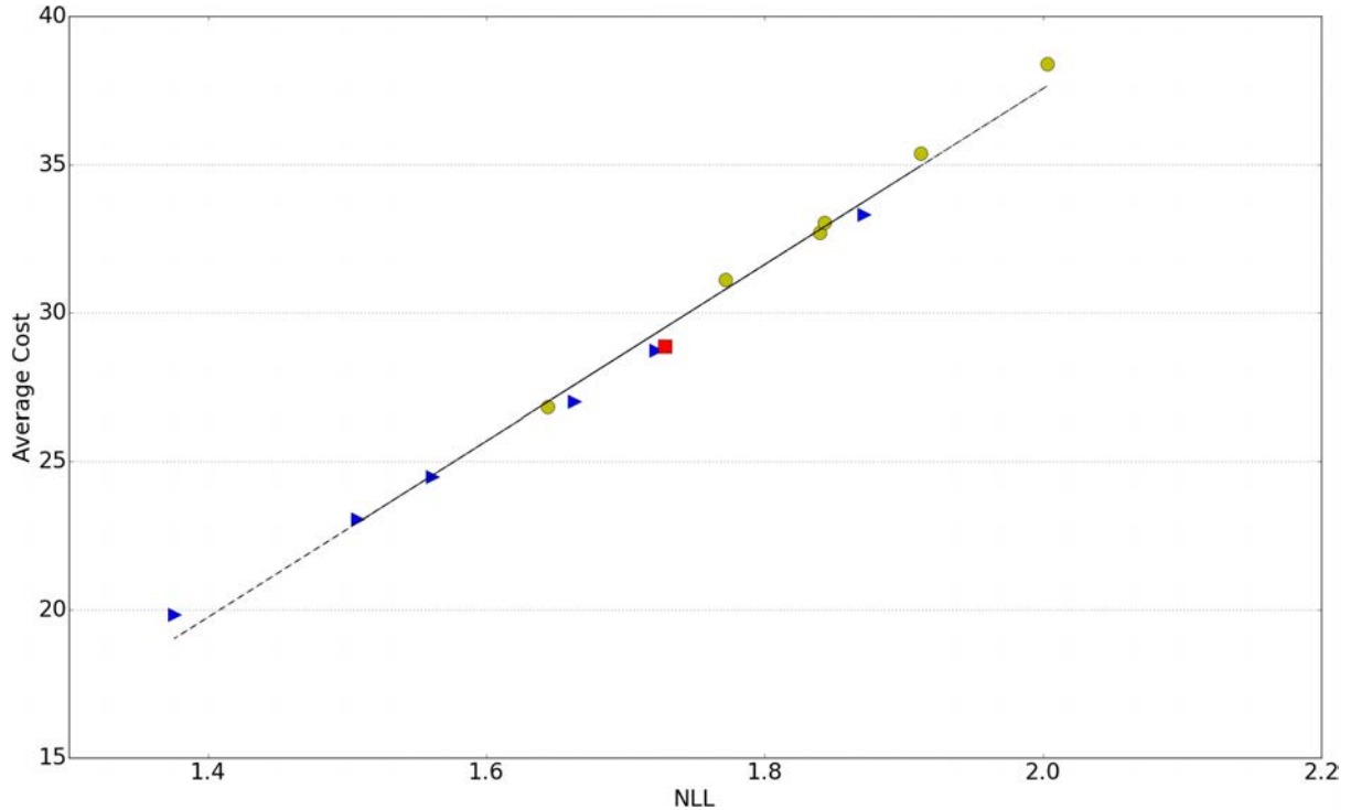
Figure 5.8: Graph of average sum of the optimal transport costs, function of the average cross-entropy on 727 sequences corpus for the Seq (red square), S\&C_{0...6} (blue triangles) and Sys_{0...6} (yellow circles) models. Correlation: 0.996, p -value: 9.76e^{-13} .
