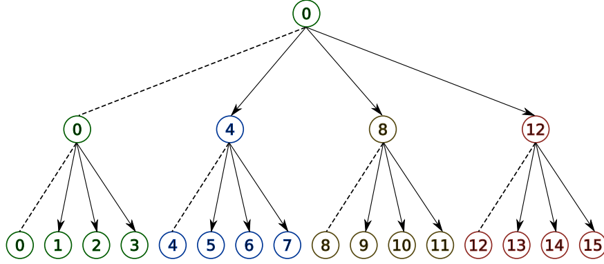
Figure 3.5: Representation of the relations used by a multi-scale analysis of a sequence of 16 elements in the Tree Systemic model. Here, the sub-sequence Y used in Equation 3.7 to pass from a scale to the upper one is (0, 4, 8, 12) .
