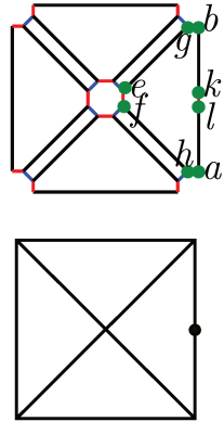
3-Insertion.Sommet(PN 2 )
