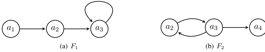
Figure 3.16: The Argumentation Frameworks F_1 and F_2
