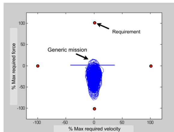
Fig. 5.3 Power requirements for an Airbus A320 aileron actuator [153]
