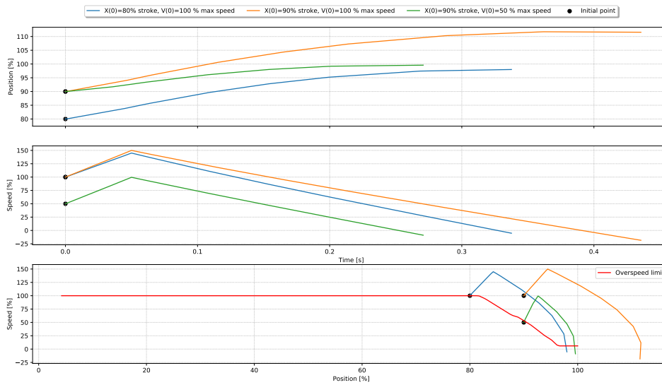
Fig. 6.26 Overspeed limit principle
