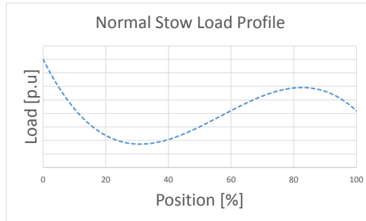
Fig. 6.8 Stow position dependent load profile shape
