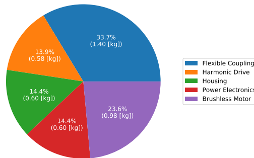
Fig. 5.30 Single EMA mass breakdown for five surfaces configuration
