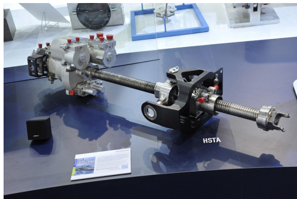
Fig. 1.10 Horizontal Stabilizer Trim electro-mechanical Actuator (Safran)
