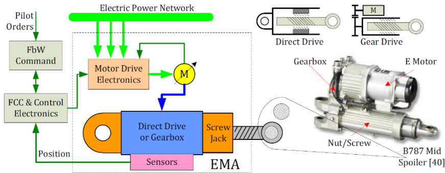
Fig. 1.6 Description of an EMA [240]
