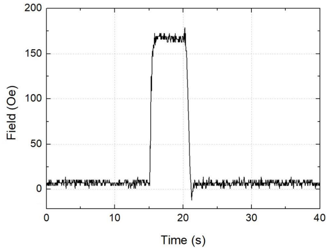
Figure 2-26 Field pulses signal with a duration of 5 \mu s.
