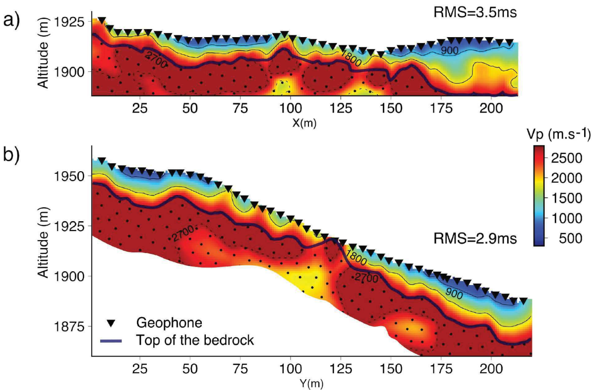
Figure 3.3: Inverted P-wave seismic velocity field for (a) profile 5 and (b) profile 11. In the bedrock (areas with the dots), the velocity is assumed to be homogeneous ( v_p=2700 \text{ m.s}^{-1} ).
