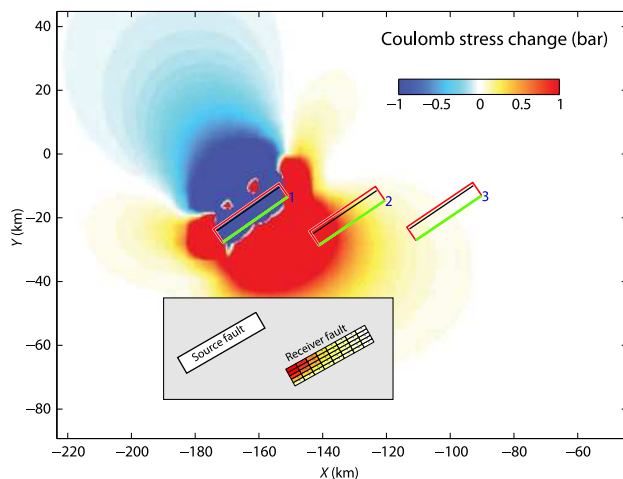
Figure 2. Conceptual model of a computed coulomb failure function ( \Delta CFF ) calculated on an en echelon thrust fault system (1, 2, and 3) comparable to the active structures of the Tell Atlas (see the Seismotectonics and Fault Parameters section for details). The kinematic of faulting and related block model is detailed in Meghraoui and Pondrelli (2012). The thin line indicates the fault tip, and the thick line is the intersection between the fault surface and the plane. Inset shows the stress loading on the fault plane, with 0.8 m average slip in agreement with an M_w 6.5 earthquake. The computation is made at 7 km depth with 235^\circ/60^\circ/70^\circ as strike/dip/rake and \mu' = 0.4 effective friction coefficient. The color version of this figure is available only in the electronic edition.
