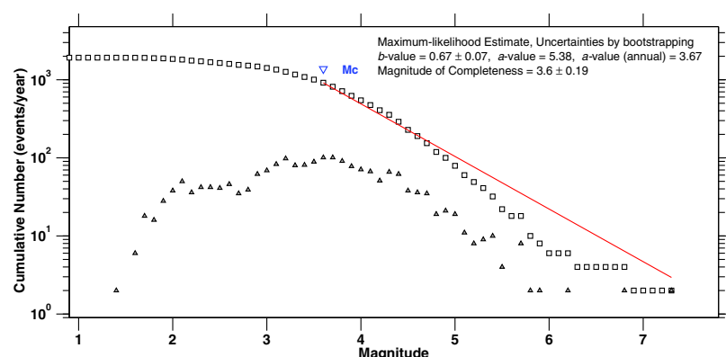
Figure 7. Cumulative number of earthquakes versus magnitude using different catalogs (Benouar, 1994; Ayadi and Bezzeghoud, 2015) using Zmap software (Wiemer, 2001) to obtain the magnitude of completeness = 3.6 \pm 0.19 using the maximum-likelihood estimate. Uncertainties by bootstrapping b -value = 0.67 \pm 0.07 , with a = 5.38 and a (annual) = 3.67. The noncumulative frequency magnitude distribution (triangles) is plotted in addition to the standard cumulative frequency-magnitude distribution (FMD, rectangles) to constrain the magnitude of completeness. The color version of this figure is available only in the electronic edition.
