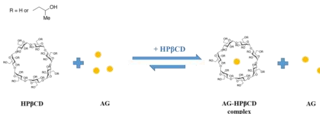
Figure 3.8: Shift of equilibrium between free AG and AG-HP \beta CD complex as concentration of HP \beta CD was increased.
