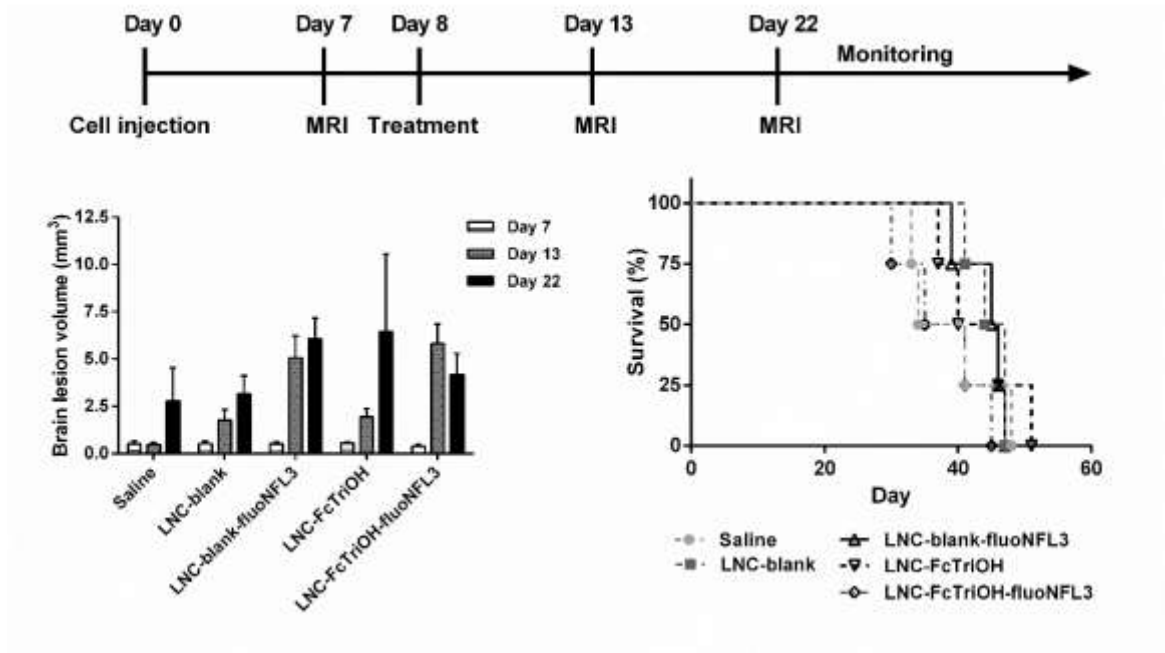
Figure 4.5: Brain lesion volumes calculated from manually selected region of interests in T2-weighted MR images, and Kaplan-Meier survival curves for U87MG tumor bearing mice treated with saline, or various LNCs administered by CED on day 8 after cell injection in the brain (n=4).
