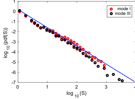
FIG. 9. Probability distribution of pinning size for mode I (red circles) and mode III (black circles) crack propagations. Blue line represents the power law \text{Pdf}(S) \propto S^{-\gamma} , with \gamma = 1.8 .
