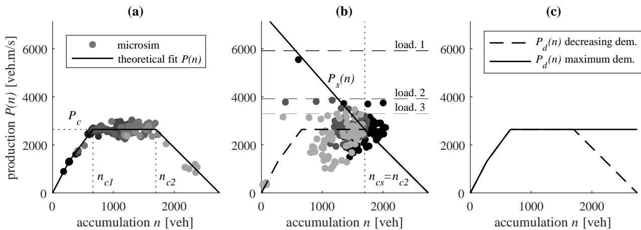
FIG. 5.3 – (a) Estimation of the production-MFD P(n) of the grid network using different loading scenarios in microsimulation, (b) the calibration of the entry production supply P_s(n) with three constant network loadings indicated by three different shades of gray, and (c) exit production demand P_d(n) for the two diverging approaches
