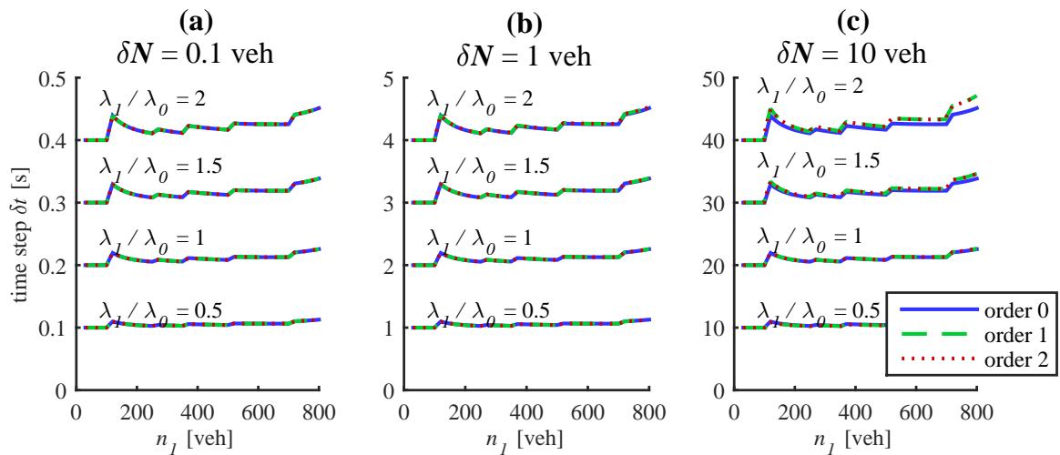
FIG. A.1 – Values of the time step \delta t calculated at different orders for V(n(t)) and for different accumulation n_1 and ratio of demand level \lambda_1/\lambda_0 . The difference n_1 - n_0 is equal to 20 veh in each case and \lambda_1 = 0.5 veh/s. (a) Case of a vehicle increment of \delta N = 0.1 veh, (b) \delta N = 1 veh, and (c) \delta N = 10 veh
