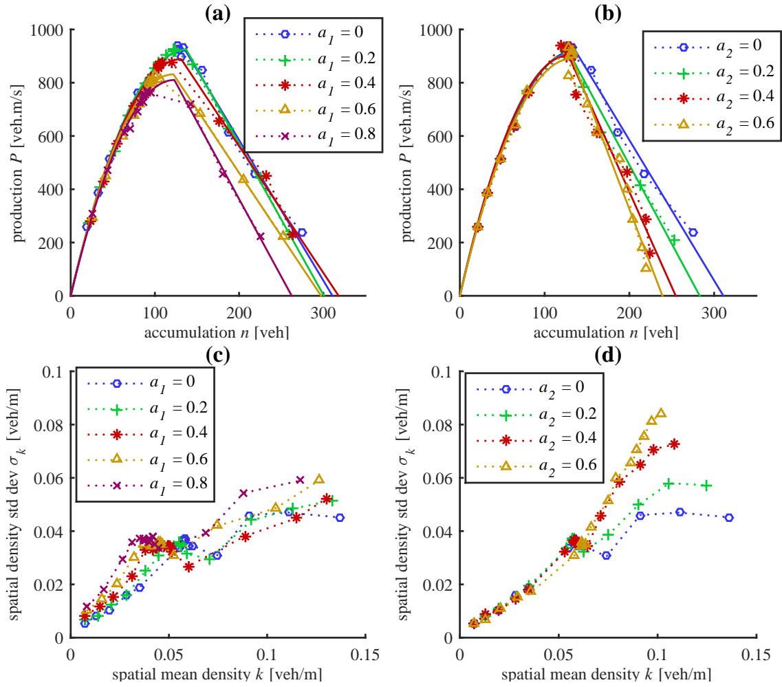
FIG. 3.5 – (a) MFD estimation for SC1 (heterogeneous demand / homogeneous supply), a_1 = 0 to 0.8. (b) MFD estimation for SC2 (homogeneous demand / heterogeneous supply), a_2 = 0 to 0.6. (c) Spatial heterogeneity (standard deviation) of link densities vs spatial mean link density in SC1 with a_1 = 0 to 0.8, and (d) in SC2 with a_2 = 0 to 0.6
