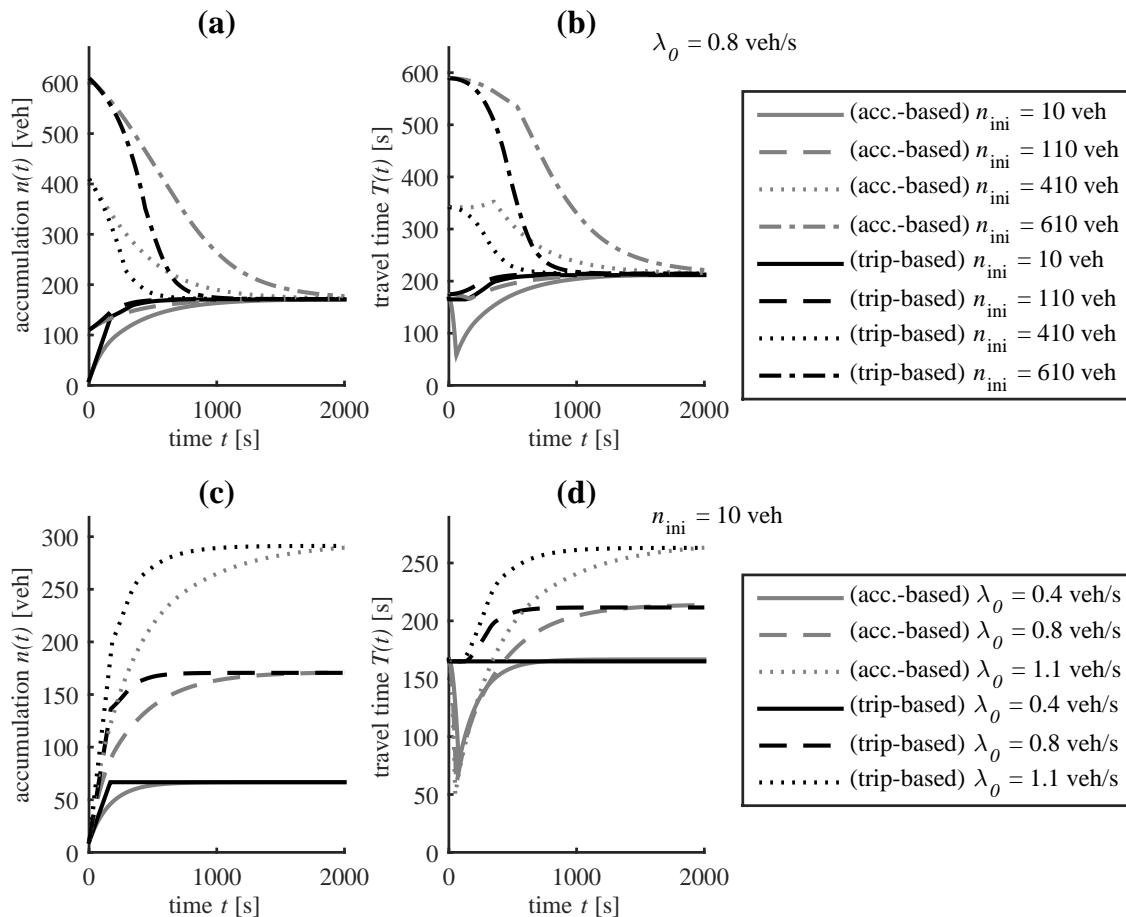
FIG. 2.7 – Comparison between accumulation-based and trip-based models. (a) Different initial conditions n_{ini} with demand \lambda_0 = 0.8 veh/s, evolution of accumulation n(t) and (b) travel time T(t) . (c) Different demand levels \lambda_0 with initial condition n_{ini} = 10 veh, evolution of accumulation n(t) and (d) travel time T(t)
