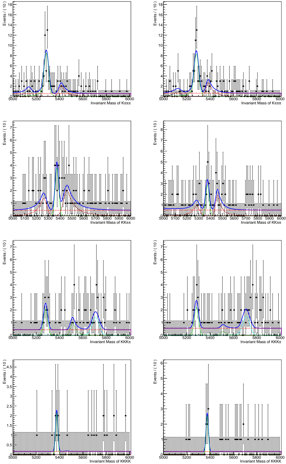
Figure 5.10: Invariant mass spectra of 2011 RHB events from [from top to bottom] X_b^0 \rightarrow p\pi\pi\pi as B^0 \rightarrow K\pi\pi\pi , X_b^0 \rightarrow pK\pi\pi as B_s^0 \rightarrow K\pi\pi K , X_b^0 \rightarrow pKK\pi as B^0 \rightarrow KKK\pi and X_b^0 \rightarrow pKKK as B_s^0 \rightarrow KKKK (left-column) with p and (right-column) \bar{p} separated.
