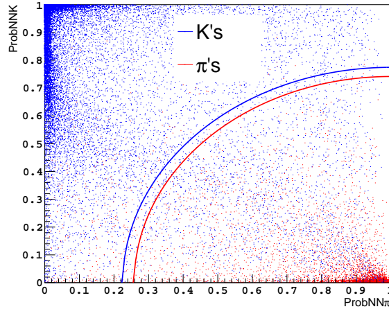
Figure 5.2: Illustration of the distribution of kaons and pions in the ProbNNK-vs-ProbNN \pi plane using MC-matched kaons and pions from MC-generated \Lambda_b^0 \rightarrow pK^-\pi^+\pi^- events.
