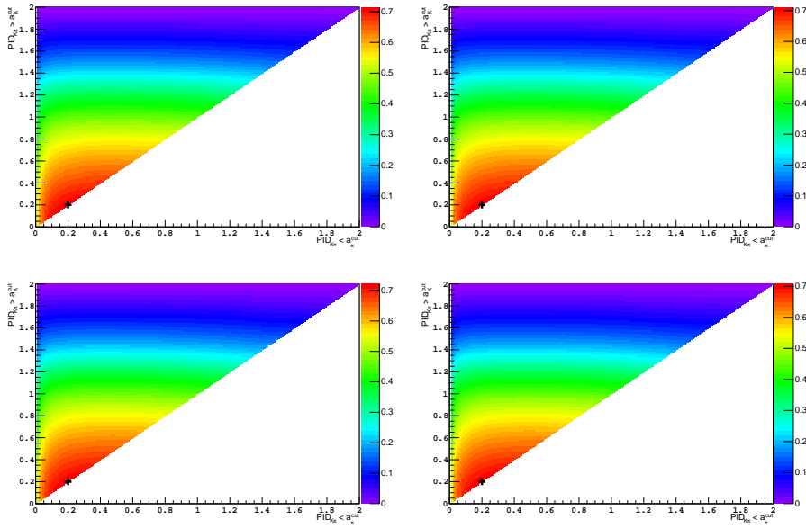
Figure A.6: Figure of merits of \text{PID}_{K\pi} optimization of \Lambda_b^0 \rightarrow pK^-K^+\pi^- for [top-left] 2011 MagDown, [top-right] 2011 MagUp, [bottom-left] 2012 MagDown and [bottom-right] 2012 MagUp.
