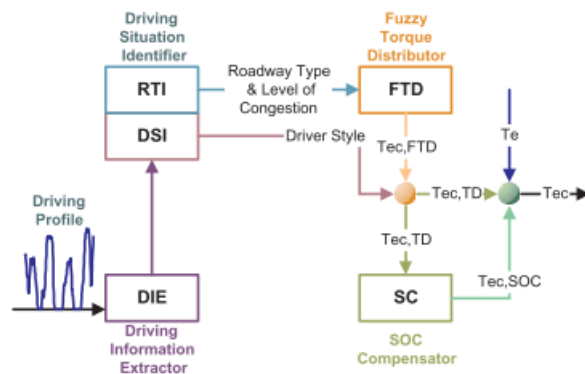
FIGURE 1.32 – IEMA architecture [129]
